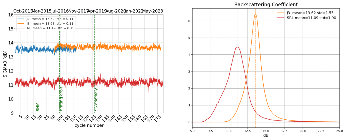
Figure 7: Daily monitoring of backscattering coefficient for Saral/AltiKa, Jason-2 and Jason-3 on the left and histogram for cycle 177 on the right (limited to 66° latitude).
