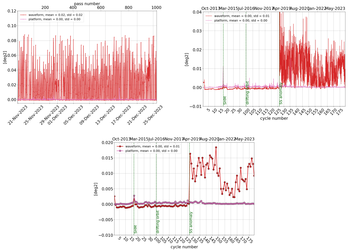
Figure 13: Monitoring per pass for cycle 177 (left), daily monitoring(right) and cyclic monitoring (bottom) of SARAL/AltiKa's mispointing angle: comparison between the one derived from waveform retracking and the one measured by platform startrackers.
