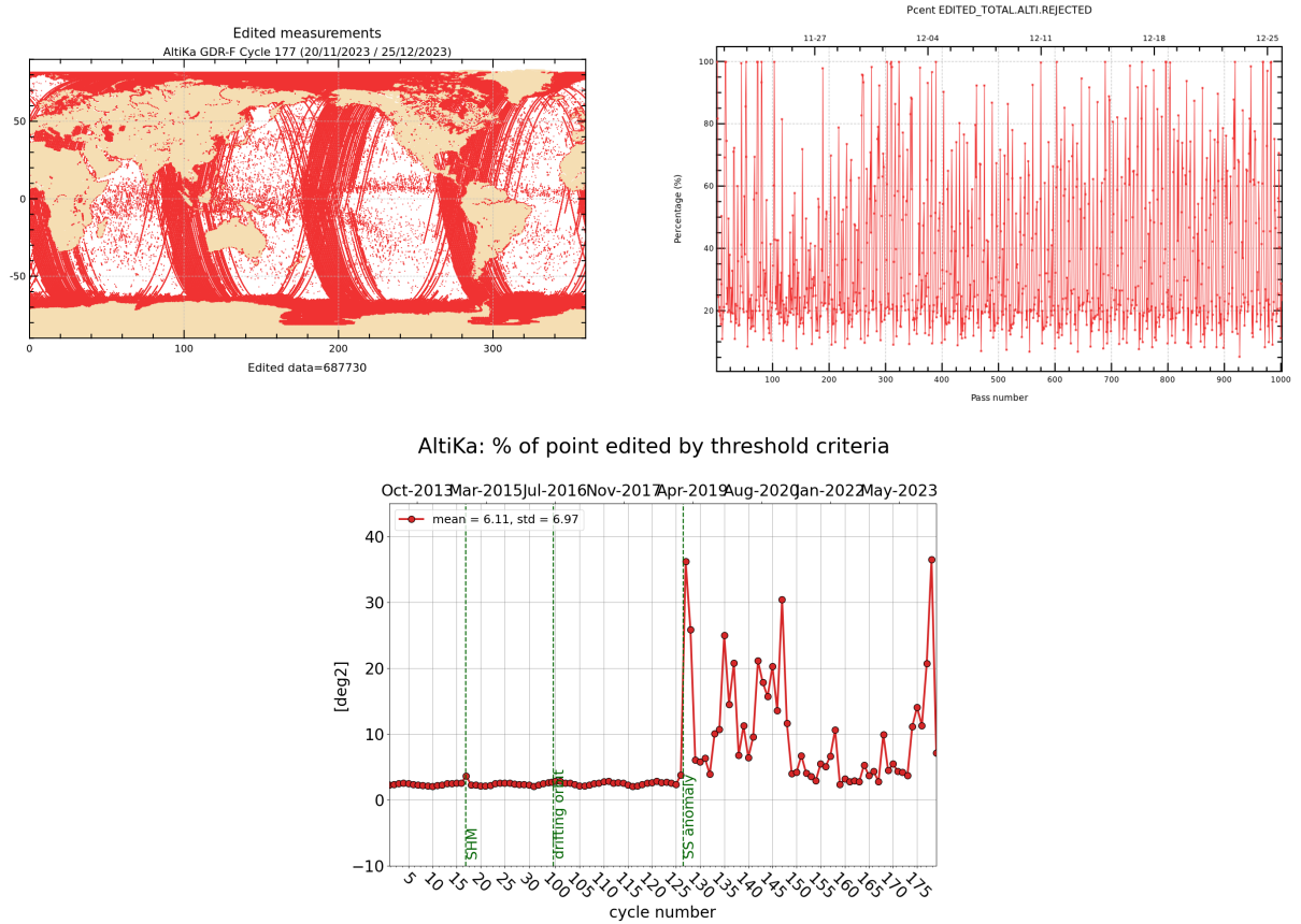
Figure 2: Rejected measurements on thresholds criteria : Cycle 177, map and monitoring of % of rejected measurements per track (top), whole time serie / % of rejected measurements per cycle (bottom).
