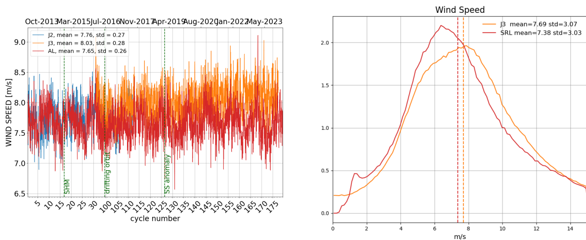
Figure 10: Daily monitoring of altimeter wind speed for Saral/AltiKa, Jason-2 and Jason-3 on the left and histogram for cycle 177 on the right (limited to 66° latitude).
