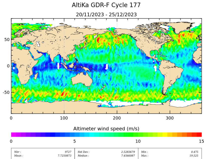
Figure 9: Altimeter wind speed for cycle 177.
