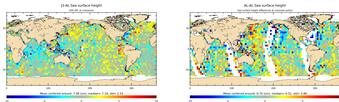
Figure 14: Mean of multi-mission SSH and mono-mission SSH differences at crossovers for cycle 177.
