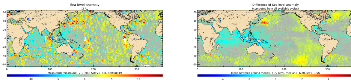
Figure 21: Jason-3 – Saral/AltiKa SLA differences for cycle 177 (left) and averaged over the whole Saral/AltiKa period (right).
