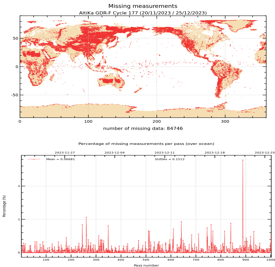
Figure 1: Map of missing measurements for cycle 177 on top. Monitoring of percentage of missing ocean measurements per pass on bottom.
