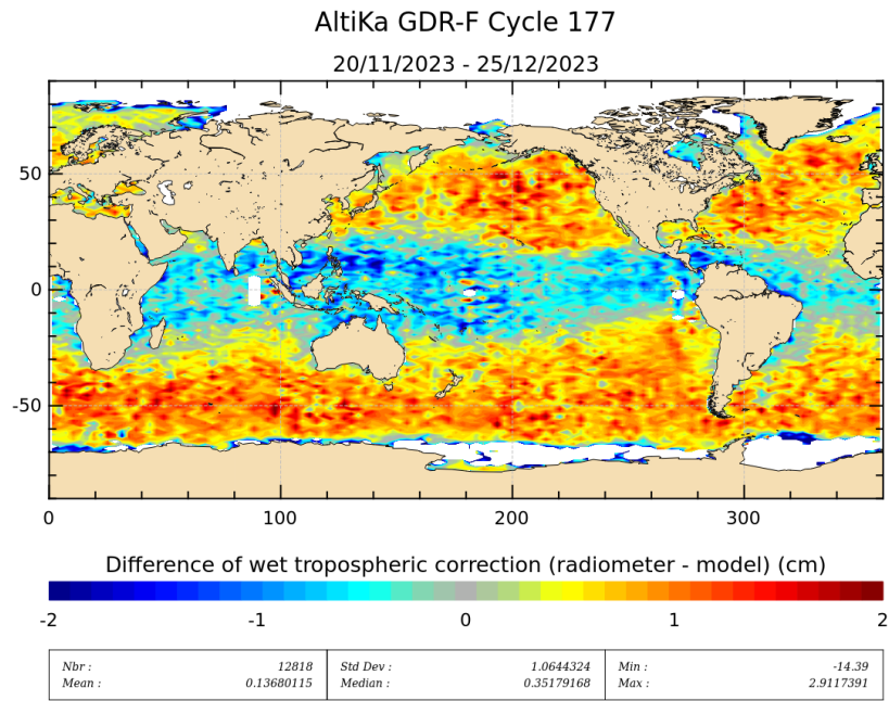
Figure 11: Mean of wet troposphere correction difference (Radiometer-ECMWF model) for cycle 177.
