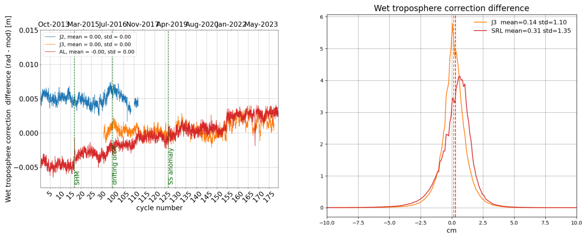
Figure 12: Daily monitoring of wet troposphere differences (Radiometer-ECMWF model) for Saral/AltiKa Jason-2 and Jason-3 (left) and histogram on the right (limited to 66° latitude) for cycle 177 .
