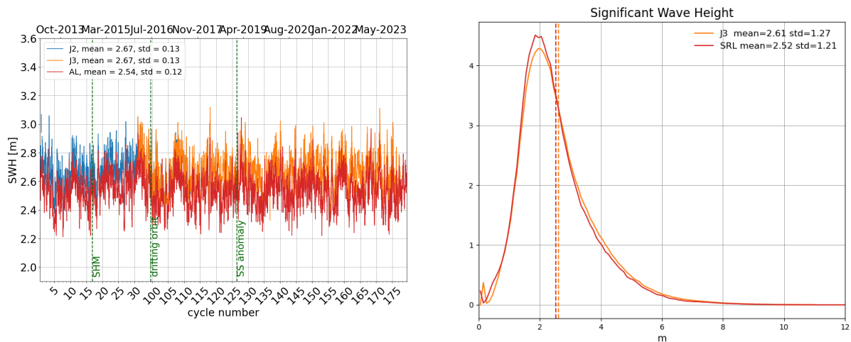
Figure 6: Daily monitoring of significant wave height for AltiKa (Ka-band) Jason-2 and Jason-3 (Ku-band) on the left and histogram for cycle 177 on the right (limited to 66^\circ latitude).
