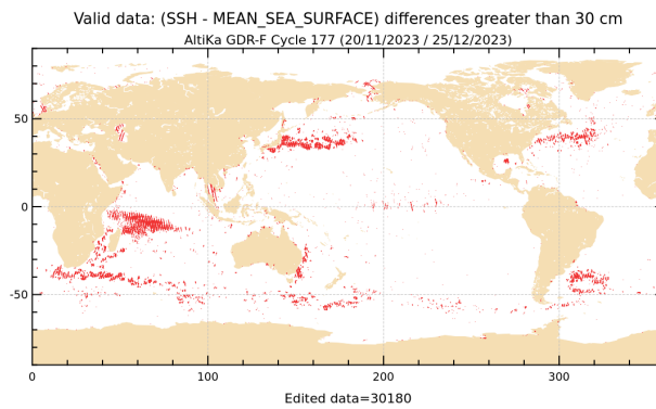
Figure 20: SLA higher than 30 cm for cycle 177.
