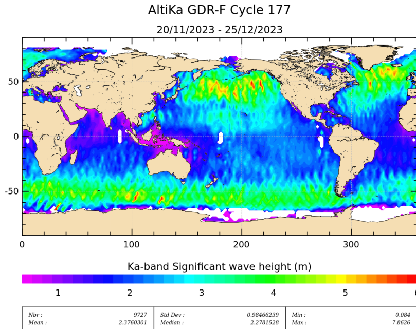
Figure 5: Significant wave height for cycle 177.
