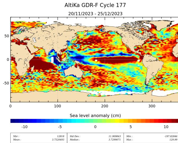
Figure 19: Sea level anomaly relative to MSS for cycle 177.
