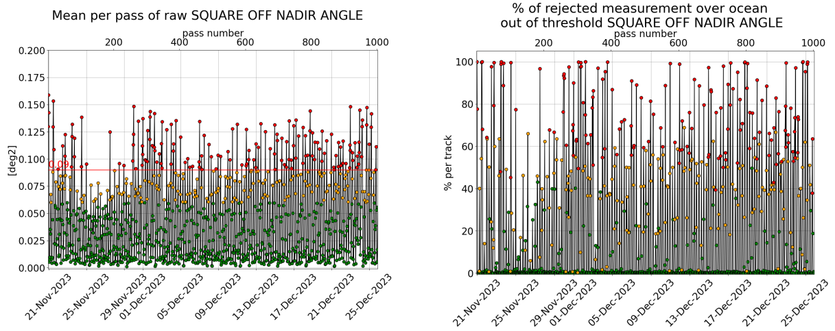
Figure 3: [left] Mispointing cycle 177, [right] Percentage of rejected measurement by threshold on square off-nadir angle.
