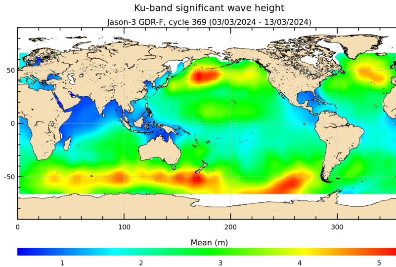
FIGURE 5 – Significant wave height for cycle 369.
