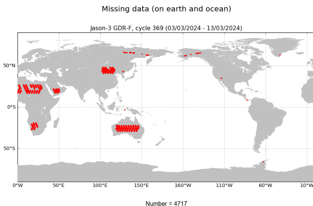
FIGURE 1 – Missing measurements for cycle 369.
