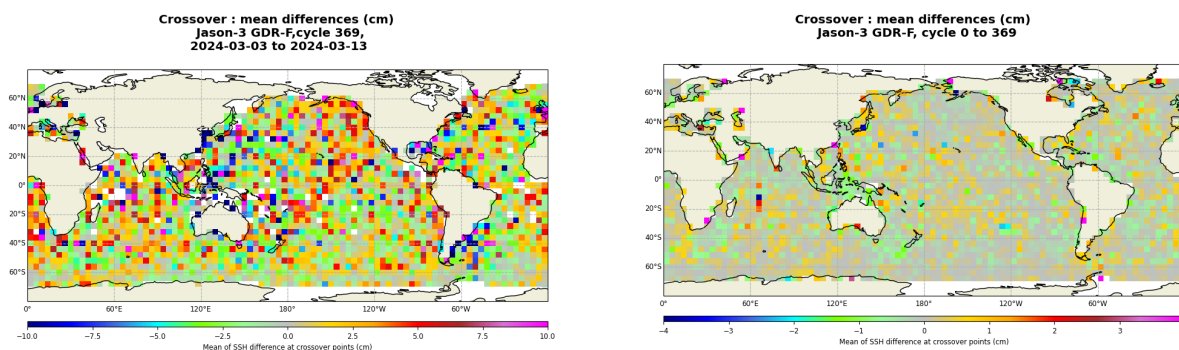
FIGURE 13 – Mean SSH at crossovers for cycle 369 (left) and over the whole Jason-3 period (right).
