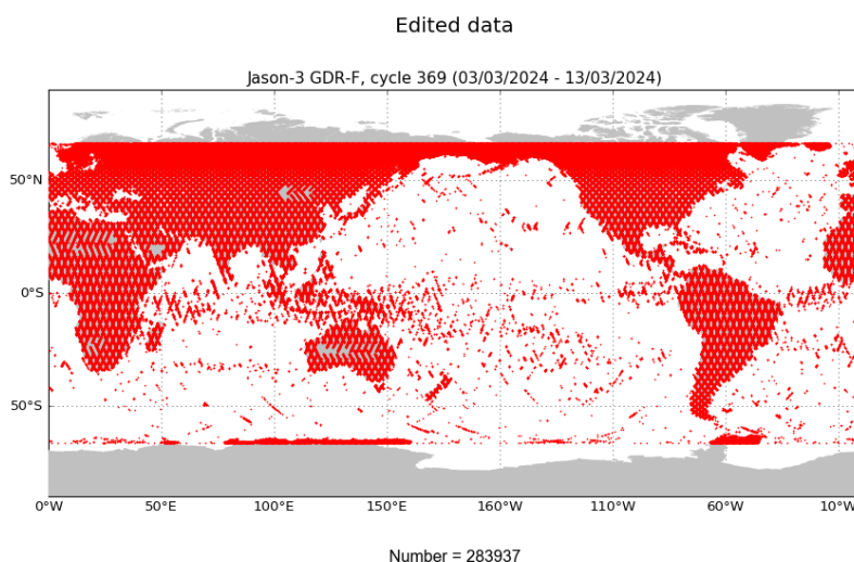
FIGURE 2 – Edited measurements for cycle 369.
