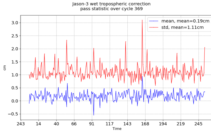
FIGURE 11 – Pass monitoring of wet troposphere differences between radiometer and ECMWF model for Jason-3 cycle 369
