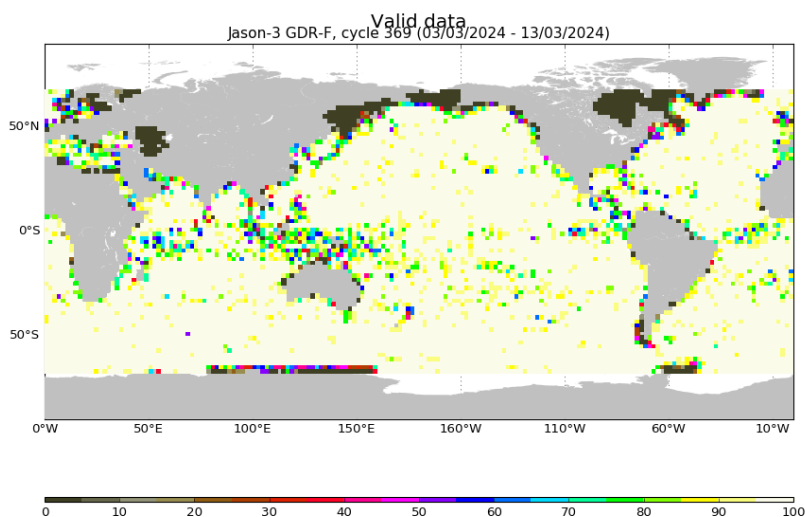
FIGURE 3 – Percentage of valid measurements for cycle 369.
