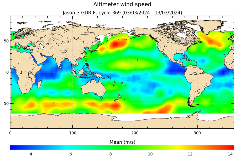
FIGURE 9 – Altimeter wind speed for cycle 369.
