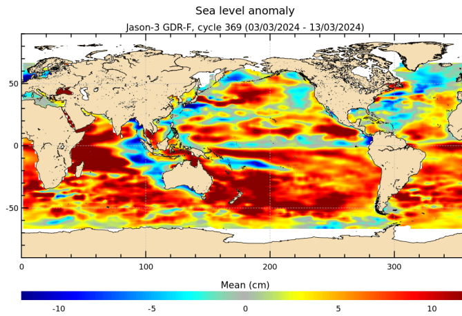
FIGURE 18 – Sea level anomaly relative to MSS for cycle 369.
