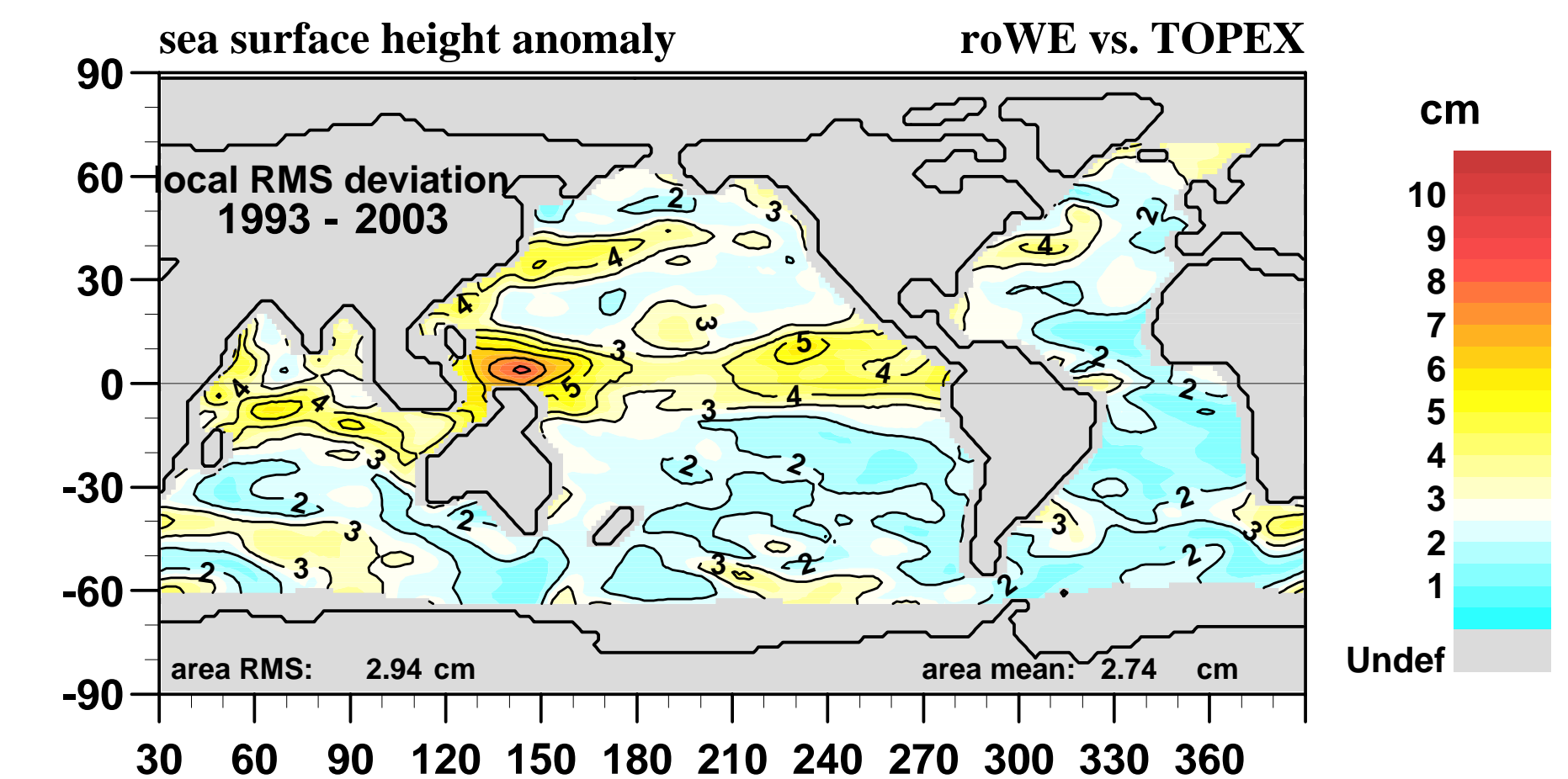
Fig. 1: Local temporal RMS difference between the modeled SSHA and the TOPEX/Poseidon data.
