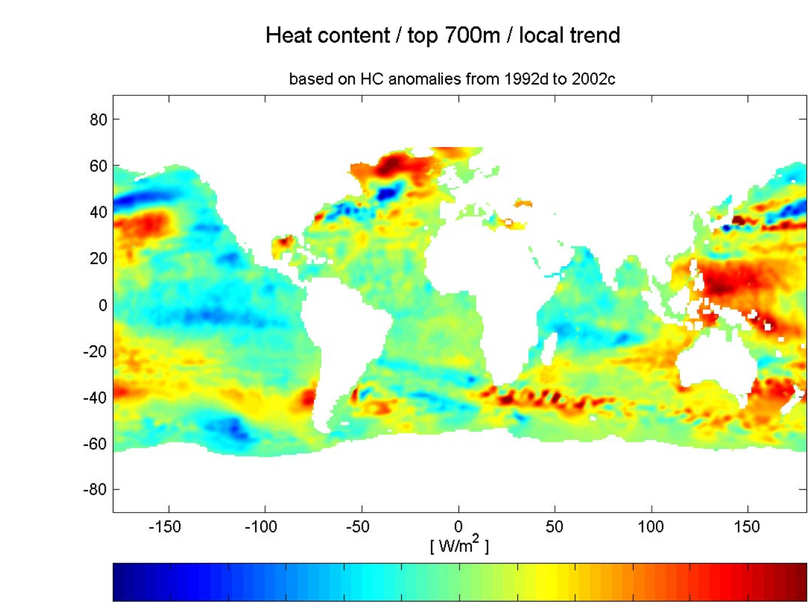
Fig. 5: Local linear trend of the upper ocean heat content [0-700m] as derived from the WOA01 annual anomalies (top) and from the Willis analysis (bottom).
