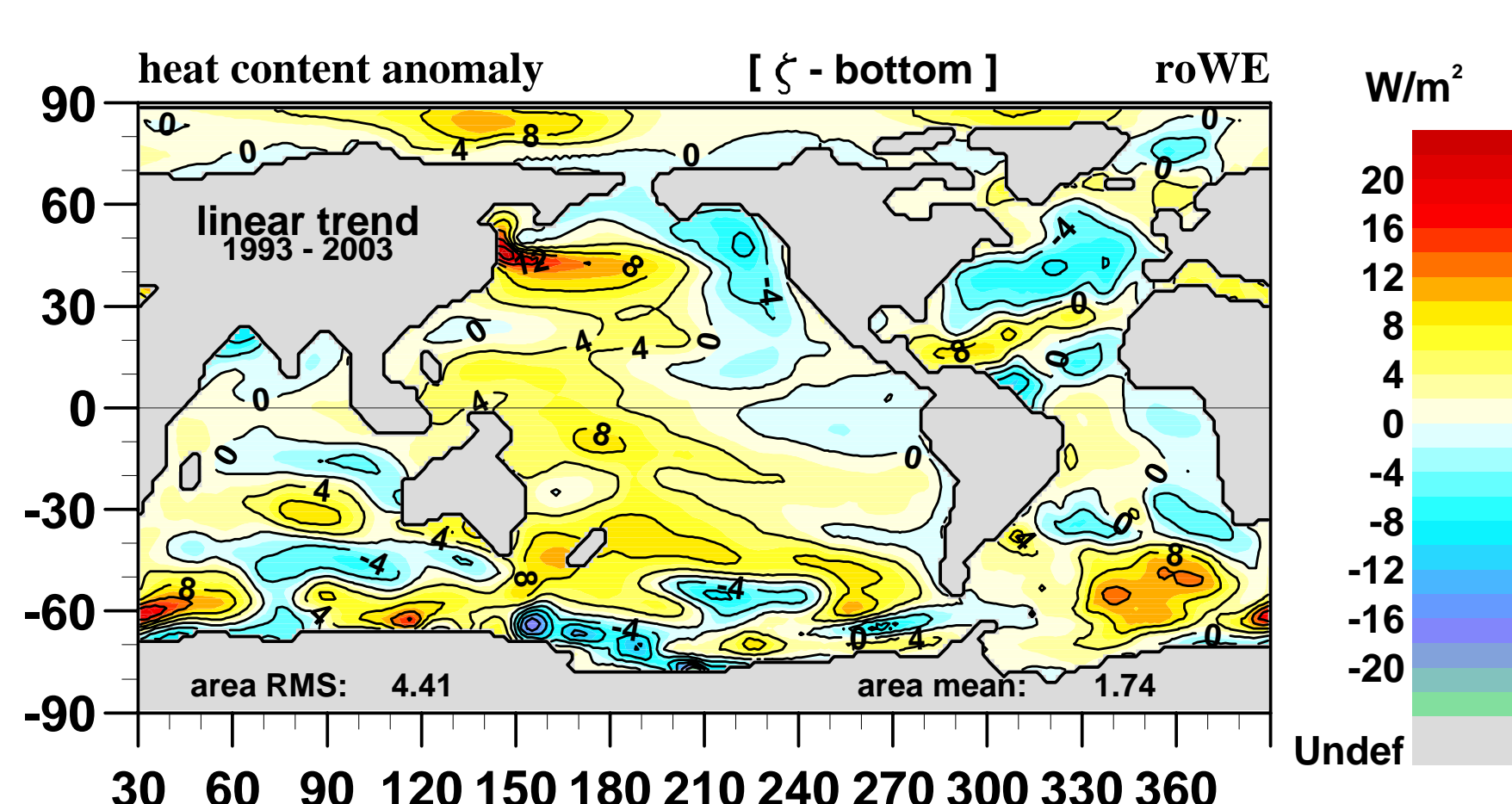
Fig. 6: Modeled local linear trend of the oceans heat content (total water column).
