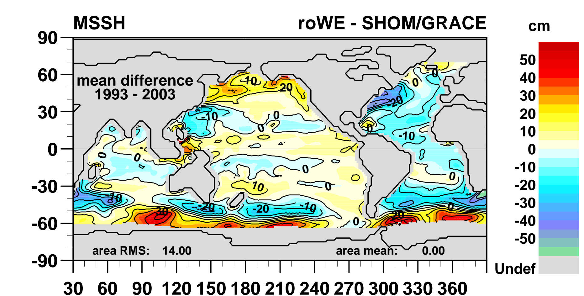
Fig. 2: Modeled temporal mean sea level compared to the SHOM98.2 mean sea surface height referenced to the GRACE geoid
