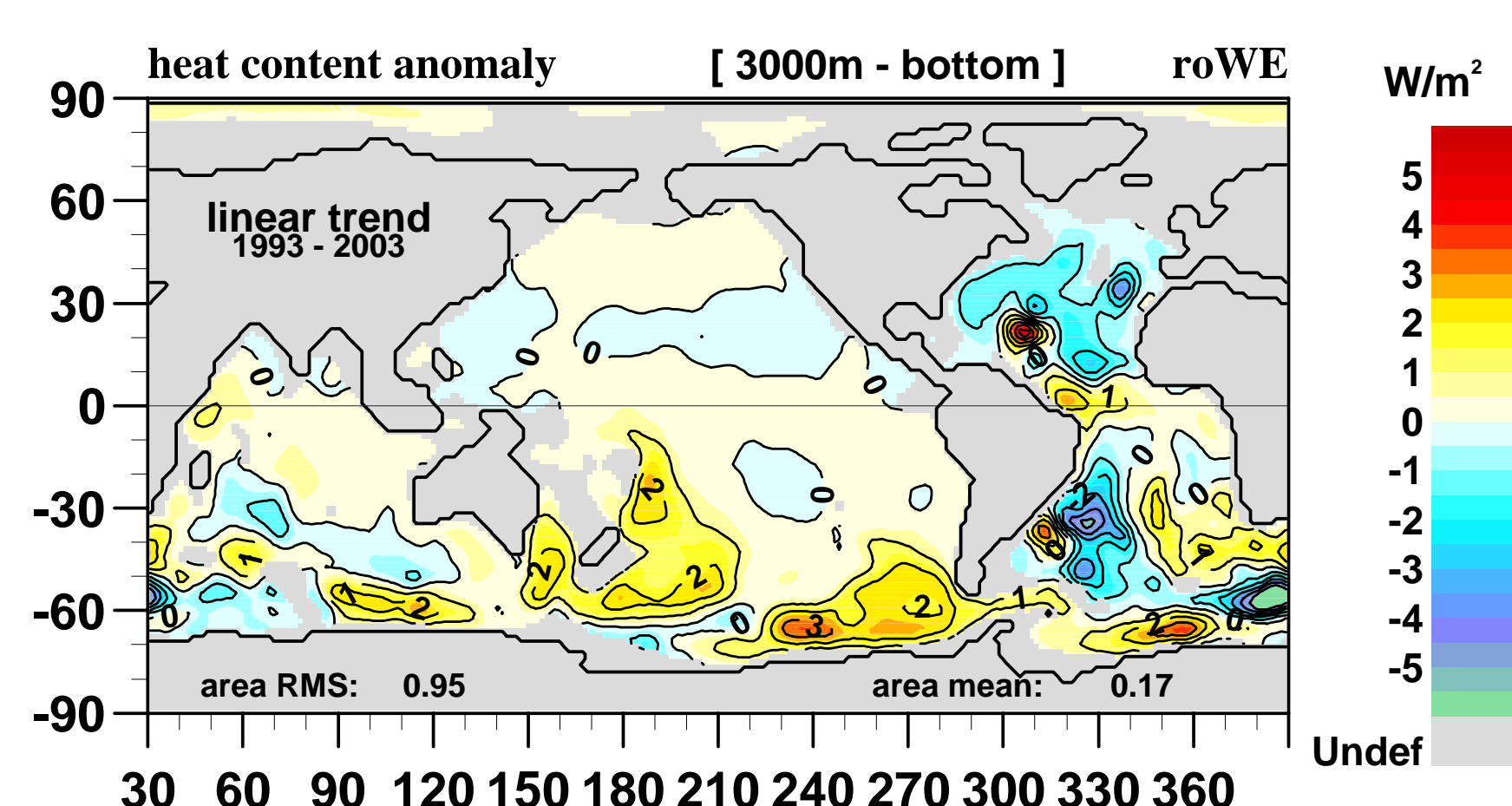
Fig. 4: Modeled local linear trend of the oceans heat content for the depth ranges: [ \zeta -700m] = top, [700-3000m] = middle and [3000m-bottom] = bottom panel.
