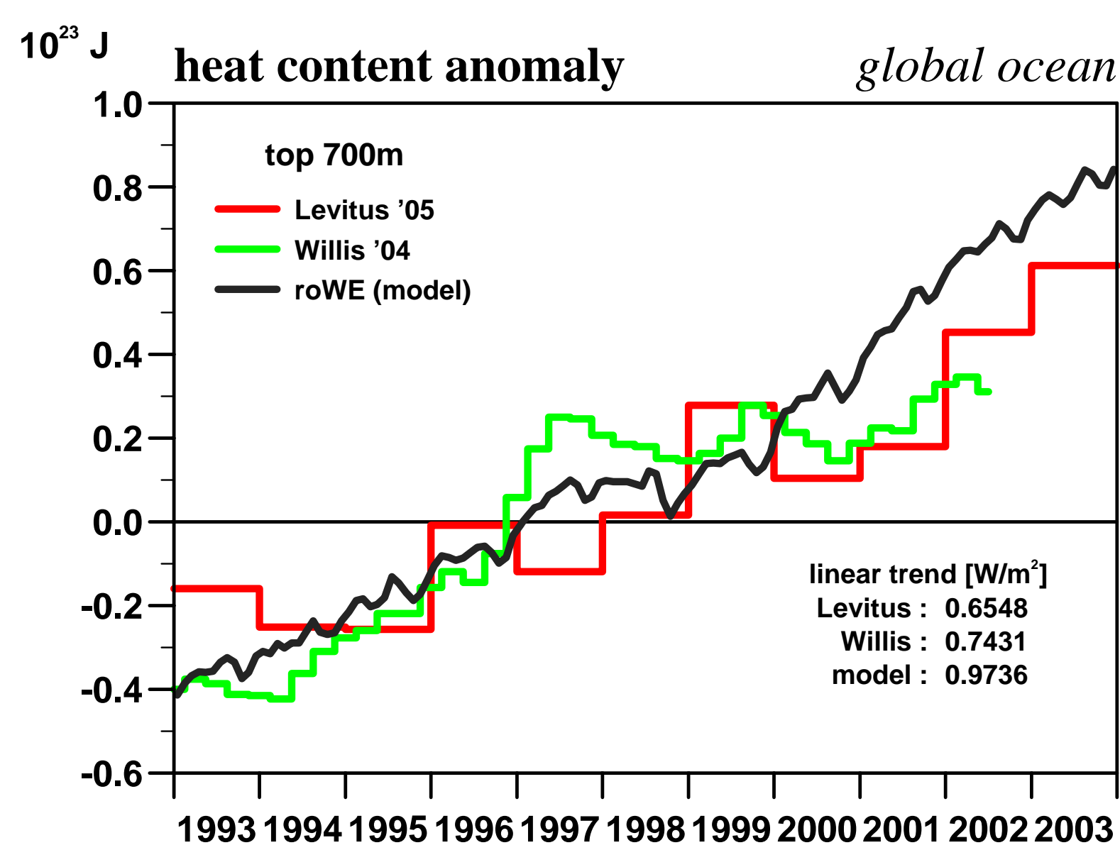
Fig. 3: Global ocean heat content anomaly for the depth range [ \zeta -700m] compared to the WOA01 annual anomaly data (Levitus, red line) and to the Willis data (green line).
