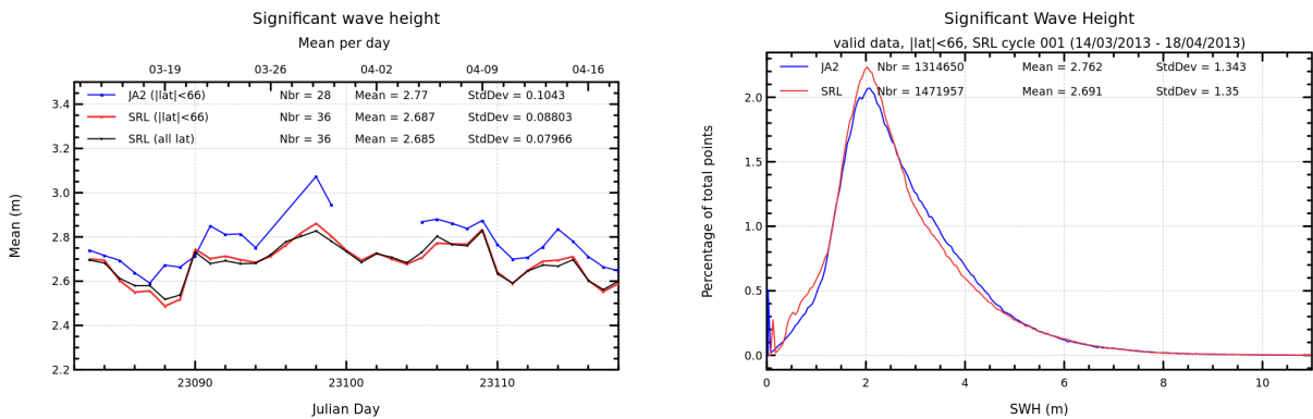
FIGURE 6 – Daily monitoring of significant wave height for AltiKa (Ka-band) and Jason-2 (Ku-band) on the left and histogram for cycle 001 on the right (limited to 66° latitude).
