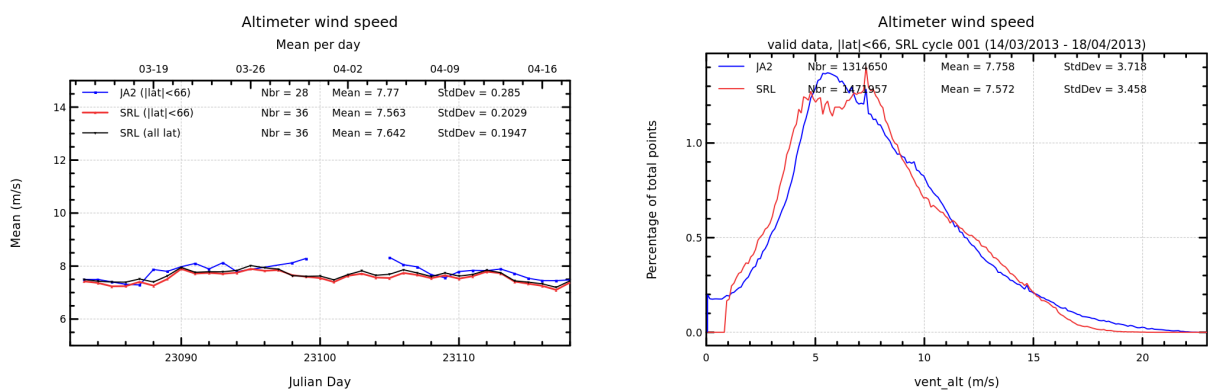
FIGURE 10 – Daily monitoring of altimeter wind speed for Saral/AltiKa and Jason-2 on the left and histogram for cycle 001 on the right (limited to 66° latitude).
