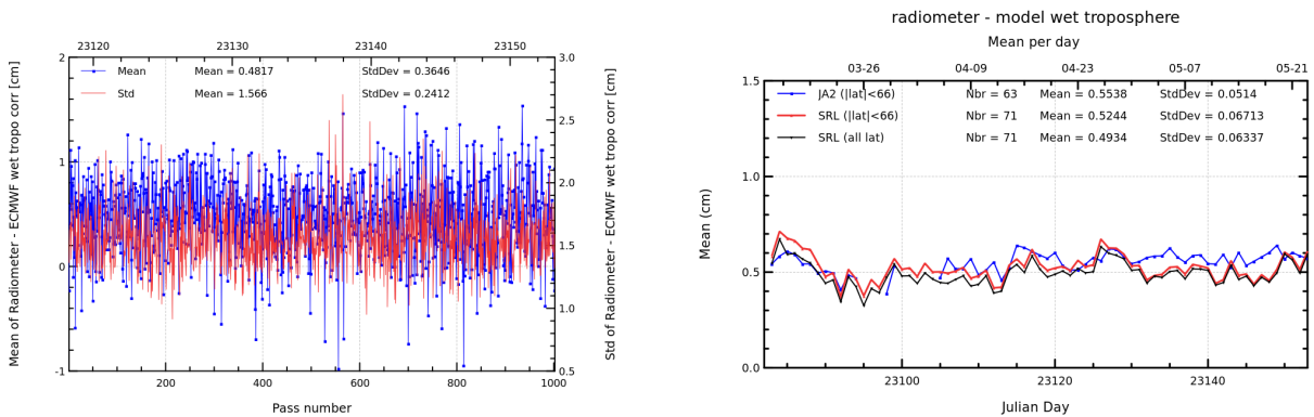
FIGURE 12 – Pass monitoring of wet troposphere differences between radiometer and ECMWF model for Saral/AltiKa cycle 002 (left) and daily monitoring of wet troposphere differences between radiometer and ECMWF model (right).
