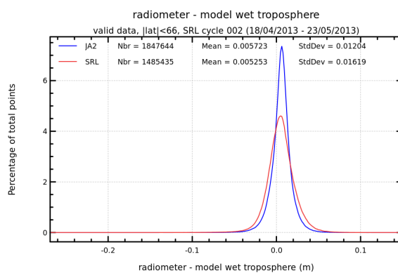
FIGURE 13 – Histogram of wet troposphere differences between radiometer and ECMWF model for cycle 002.
