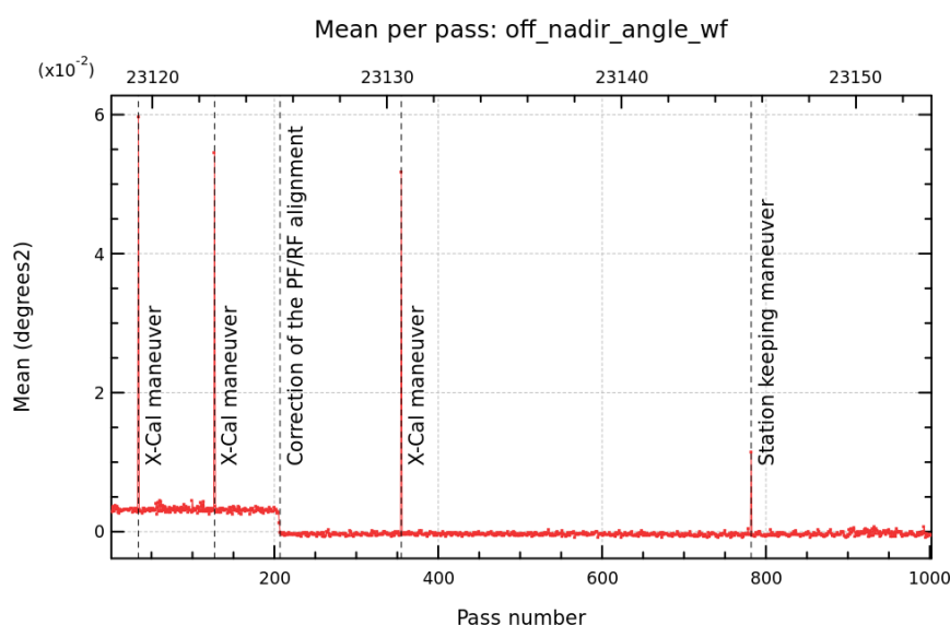
FIGURE 1 – Monitoring of mean of off-nadir angle from waveform per pass.
