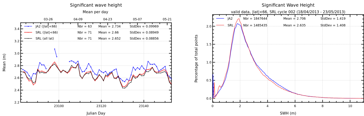
FIGURE 7 – Daily monitoring of significant wave height for AltiKa (Ka-band) and Jason-2 (Ku-band) on the left and histogram for cycle 002 on the right (limited to 66° latitude).
