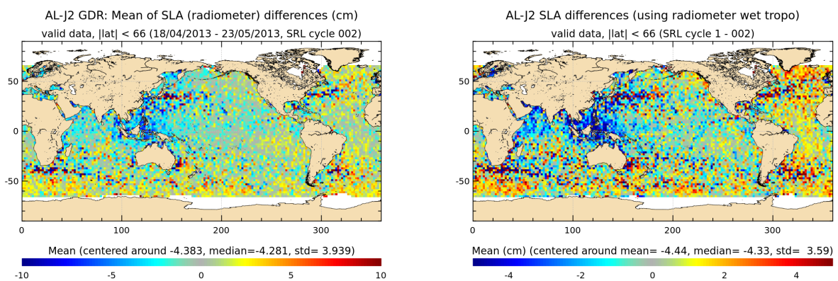
FIGURE 21 – Saral/AltiKa – Jason-2 SLA differences for cycle 002 (left) and averaged over the whole Saral/AltiKa period (right)
