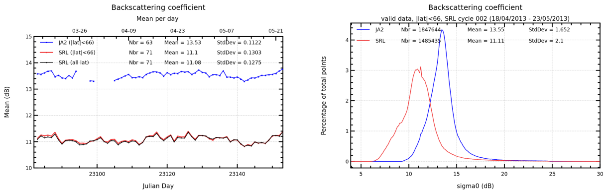
FIGURE 8 – Daily monitoring of backscattering coefficient for Saral/AltiKa and Jason-2 on the left and histogram for cycle 002 on the right (limited to 66° latitude).
