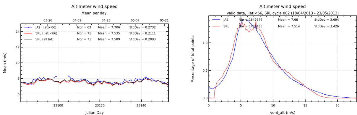
FIGURE 11 – Daily monitoring of altimeter wind speed for Saral/AltiKa and Jason-2 on the left and histogram for cycle 002 on the right (limited to 66° latitude).
