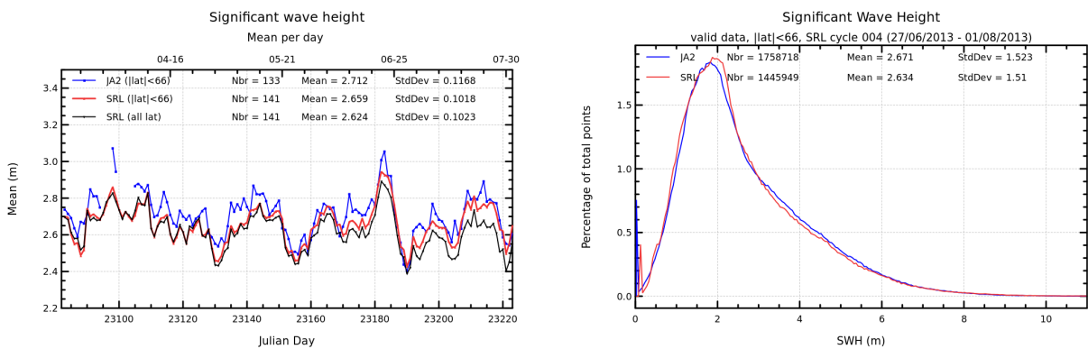
FIGURE 6 – Daily monitoring of significant wave height for AltiKa (Ka-band) and Jason-2 (Ku-band) on the left and histogram for cycle 004 on the right (limited to 66° latitude).
