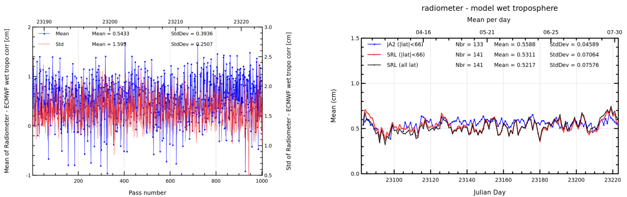
FIGURE 11 – Pass monitoring of wet troposphere differences between radiometer and ECMWF model for Saral/AltiKa cycle 004 (left) and daily monitoring of wet troposphere differences between radiometer and ECMWF model (right).
