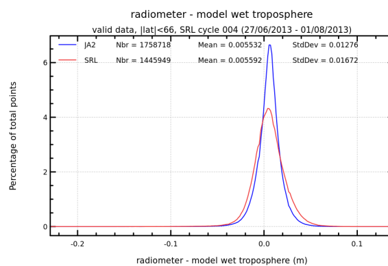
FIGURE 12 – Histogram of wet troposphere differences between radiometer and ECMWF model for cycle 004.
