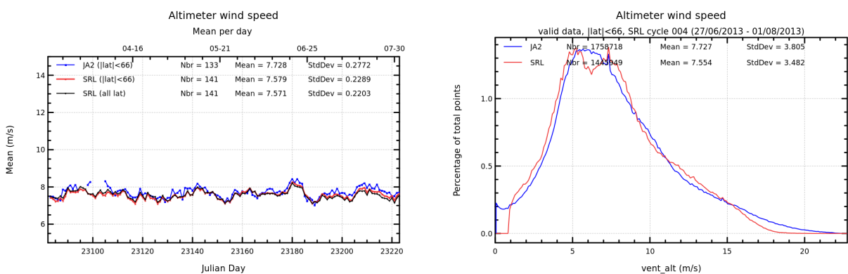
FIGURE 10 – Daily monitoring of altimeter wind speed for Saral/AltiKa and Jason-2 on the left and histogram for cycle 004 on the right (limited to 66° latitude).
