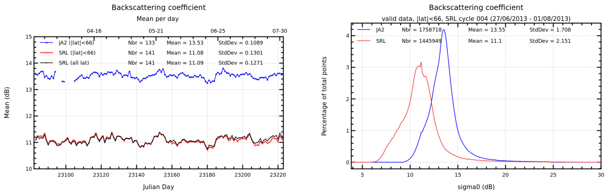
FIGURE 7 – Daily monitoring of backscattering coefficient for Saral/AltiKa and Jason-2 on the left and histogram for cycle 004 on the right (limited to 66° latitude).
