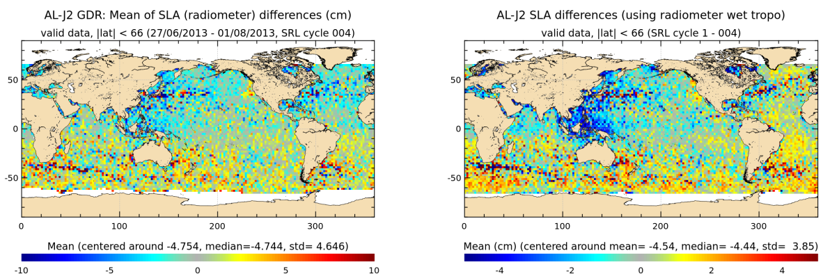
FIGURE 20 – Saral/AltiKa – Jason-2 SLA differences for cycle 004 (left) and averaged over the whole Saral/AltiKa period (right)
