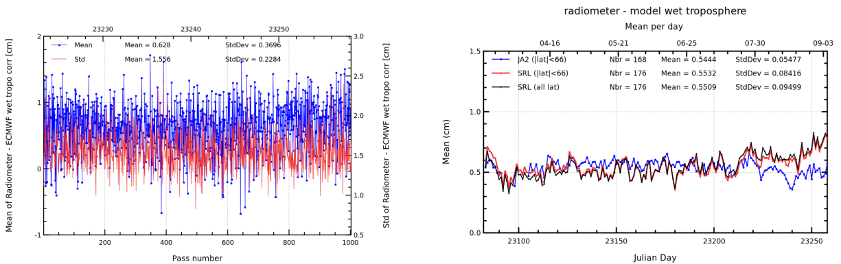
FIGURE 11 – Pass monitoring of wet troposphere differences between radiometer and ECMWF model for Saral/AltiKa cycle 005 (left) and daily monitoring of wet troposphere differences between radiometer and ECMWF model (right).
