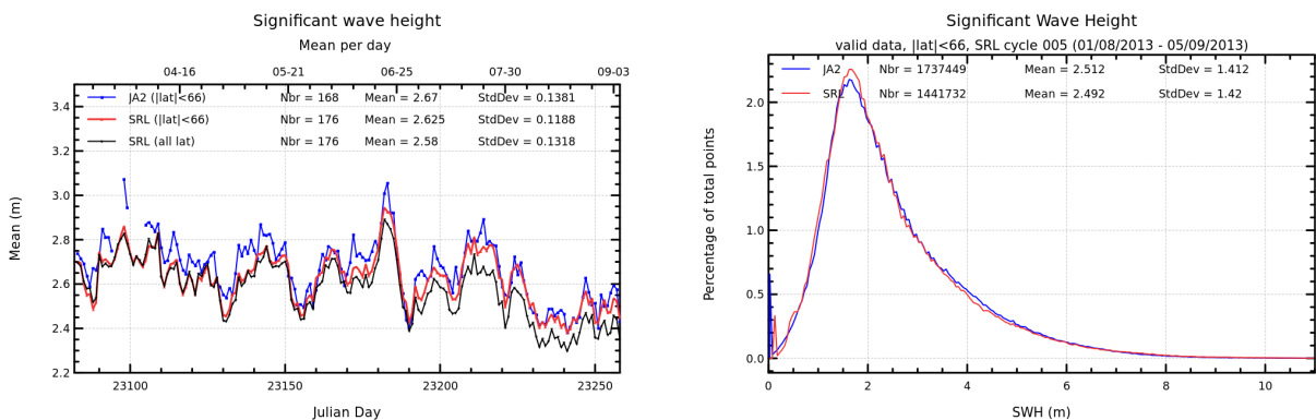
FIGURE 6 – Daily monitoring of significant wave height for AltiKa (Ka-band) and Jason-2 (Ku-band) on the left and histogram for cycle 005 on the right (limited to 66° latitude).
