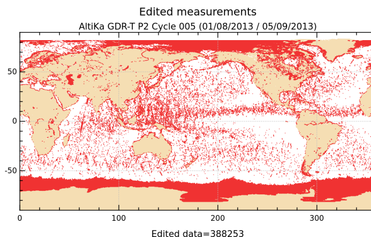
FIGURE 2 – Edited measurements for cycle 005.
