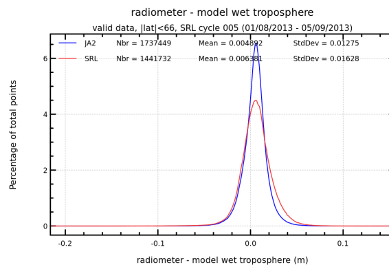
FIGURE 12 – Histogram of wet troposphere differences between radiometer and ECMWF model for cycle 005.
