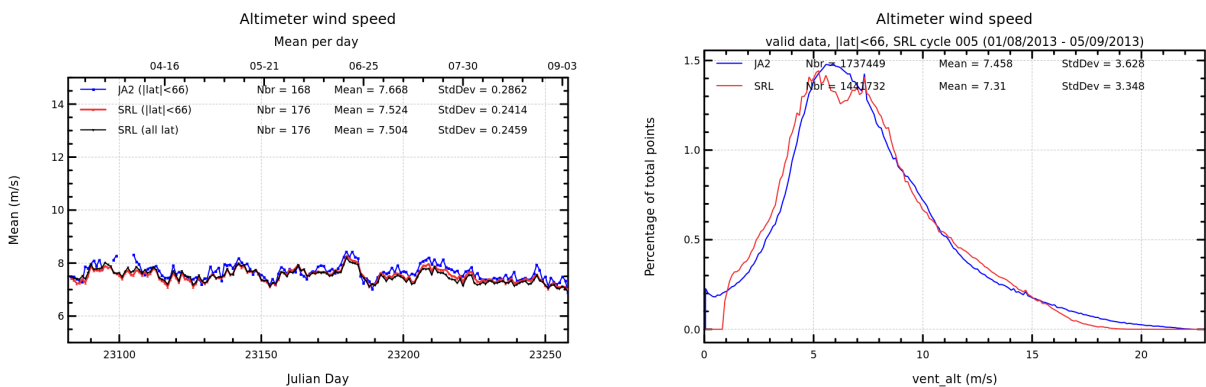
FIGURE 10 – Daily monitoring of altimeter wind speed for Saral/AltiKa and Jason-2 on the left and histogram for cycle 005 on the right (limited to 66° latitude).
