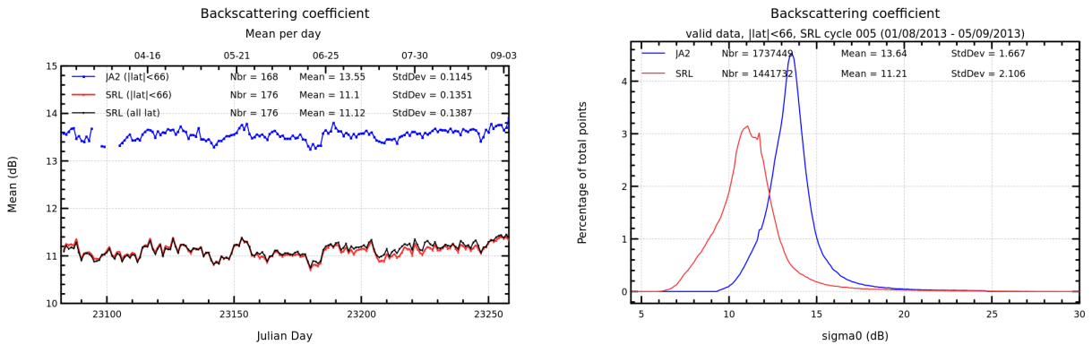
FIGURE 7 – Daily monitoring of backscattering coefficient for Saral/AltiKa and Jason-2 on the left and histogram for cycle 005 on the right (limited to 66° latitude).
