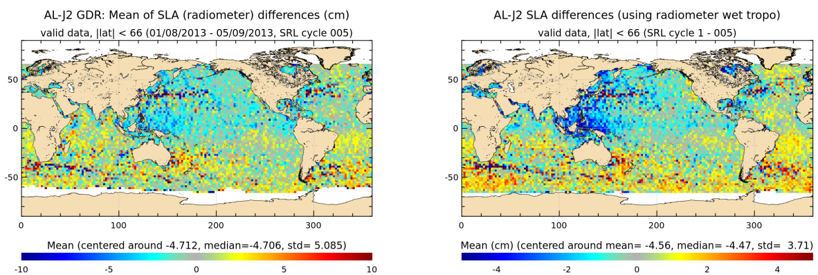
FIGURE 20 – Saral/AltiKa – Jason-2 SLA differences for cycle 005 (left) and averaged over the whole Saral/AltiKa period (right)
