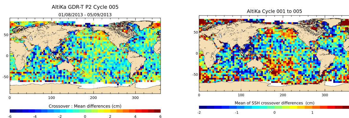
FIGURE 13 – Mean SSH at crossovers for cycle 005 (left) and over the whole Saral/AltiKa period (right).
