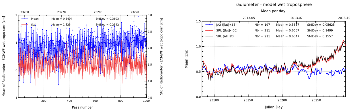
FIGURE 11 – Pass monitoring of wet troposphere differences between radiometer and ECMWF model for Saral/AltiKa cycle 006 (left) and daily monitoring of wet troposphere differences between radiometer and ECMWF model (right).
