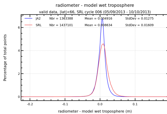
FIGURE 13 – Histogram of wet troposphere differences between radiometer and ECMWF model for cycle 006.
