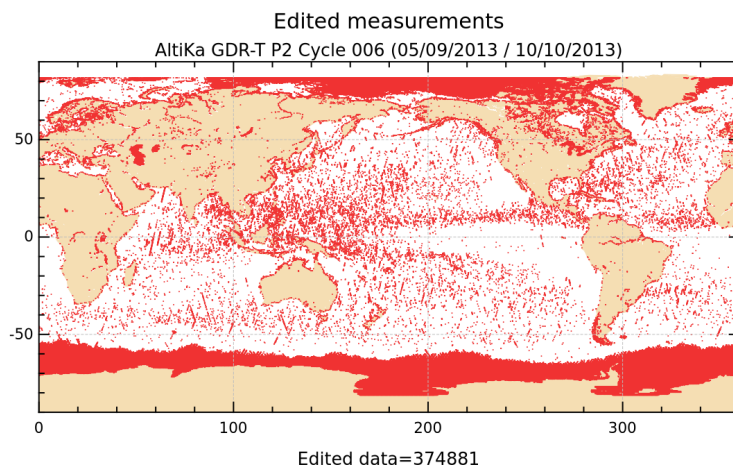
FIGURE 2 – Edited measurements for cycle 006.
