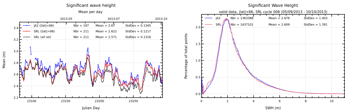
FIGURE 6 – Daily monitoring of significant wave height for AltiKa (Ka-band) and Jason-2 (Ku-band) on the left and histogram for cycle 006 on the right (limited to 66° latitude).
