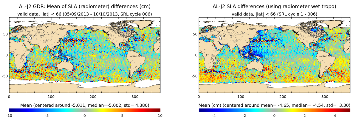
FIGURE 21 – Saral/AltiKa – Jason-2 SLA differences for cycle 006 (left) and averaged over the whole Saral/AltiKa period (right)
