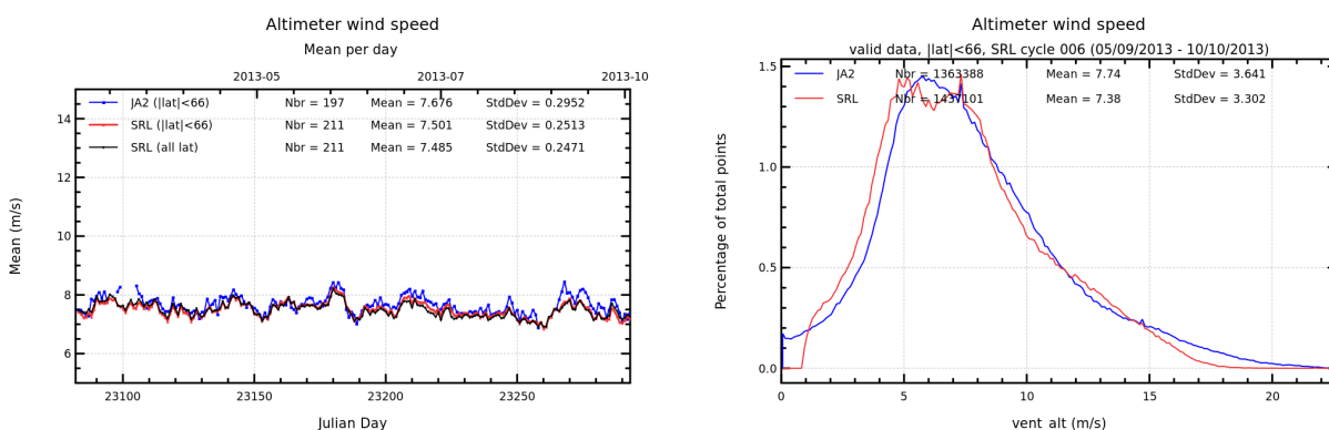
FIGURE 10 – Daily monitoring of altimeter wind speed for Saral/AltiKa and Jason-2 on the left and histogram for cycle 006 on the right (limited to 66° latitude).
