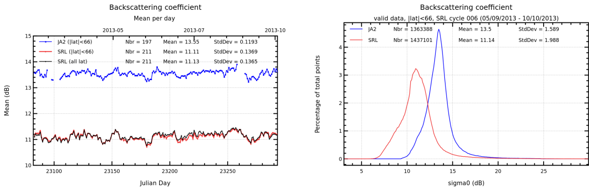
FIGURE 7 – Daily monitoring of backscattering coefficient for Saral/AltiKa and Jason-2 on the left and histogram for cycle 006 on the right (limited to 66° latitude).
