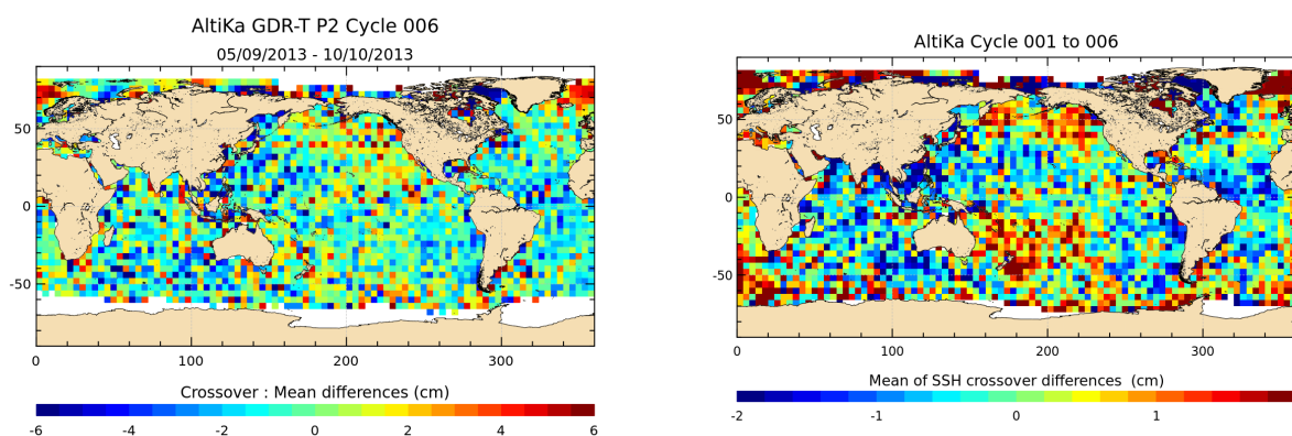
FIGURE 14 – Mean SSH at crossovers for cycle 006 (left) and over the whole Saral/AltiKa period (right).
