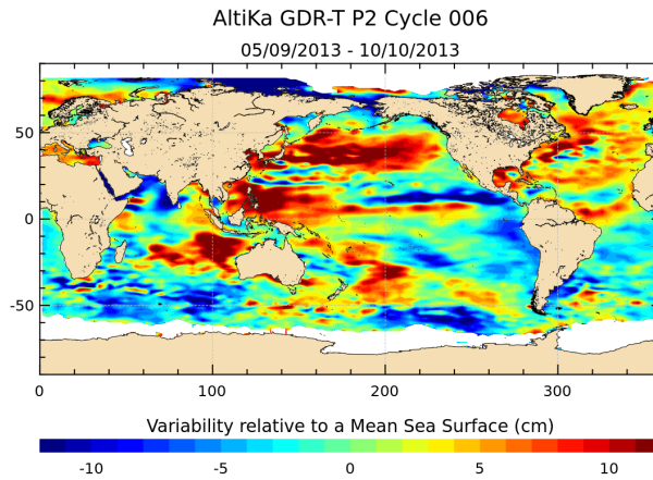
FIGURE 19 – Sea level anomaly relative to MSS for cycle 006.
