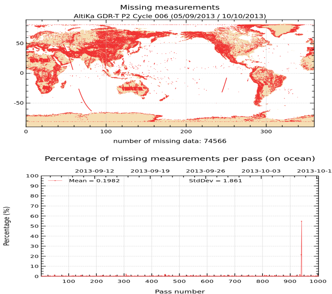
FIGURE 1 – Map of missing measurements for cycle 006 on top. Monitoring of percentage of missing ocean measurements per pass on bottom
