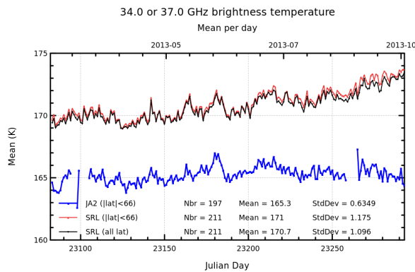
FIGURE 12 – Daily monitoring of 34 GHz (Jason-2) and 37 GHz (Saral/AltiKa) brightness temperature for Saral/AltiKa and Jason-2.
