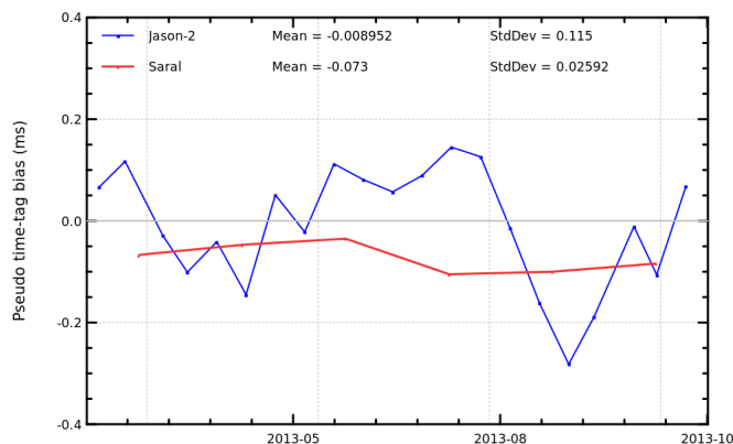
FIGURE 17 – Cyclic monitoring of pseudo time tag bias for Saral/AltiKa.
