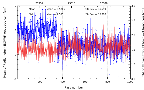
FIGURE 11 – Pass monitoring of wet troposphere differences between radiometer and ECMWF model for Saral/AltiKa cycle 007.
