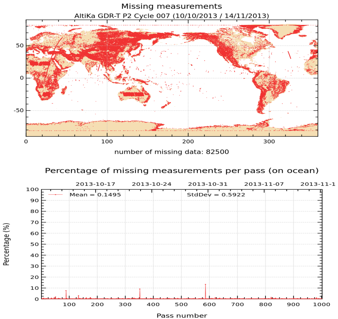
FIGURE 1 – Map of missing measurements for cycle 007 on top. Monitoring of percentage of missing ocean measurements per pass on bottom
