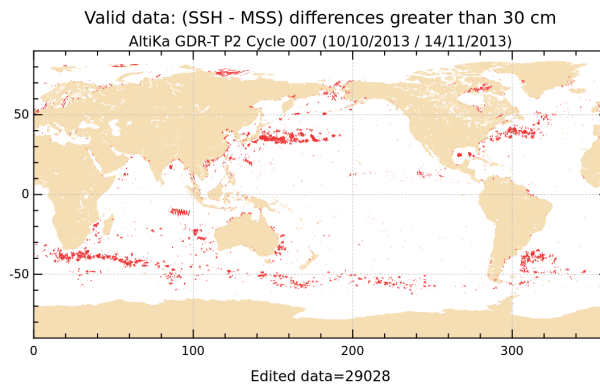
FIGURE 20 – Differences higher than a 30 cm threshold for cycle 007.
