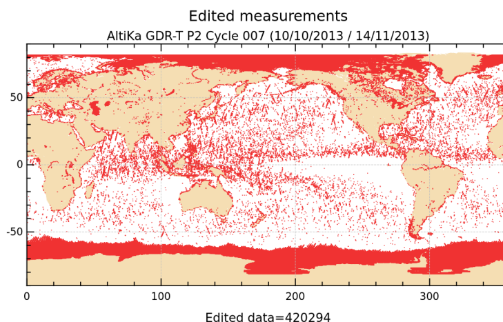
FIGURE 2 – Edited measurements for cycle 007.
