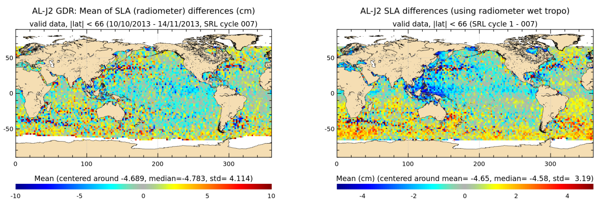
FIGURE 21 – Saral/AltiKa – Jason-2 SLA differences for cycle 007 (left) and averaged over the whole Saral/AltiKa period (right)
