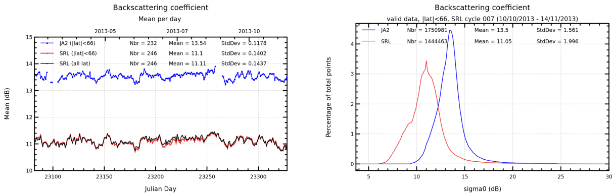
FIGURE 7 – Daily monitoring of backscattering coefficient for Saral/AltiKa and Jason-2 on the left and histogram for cycle 007 on the right (limited to 66° latitude).
