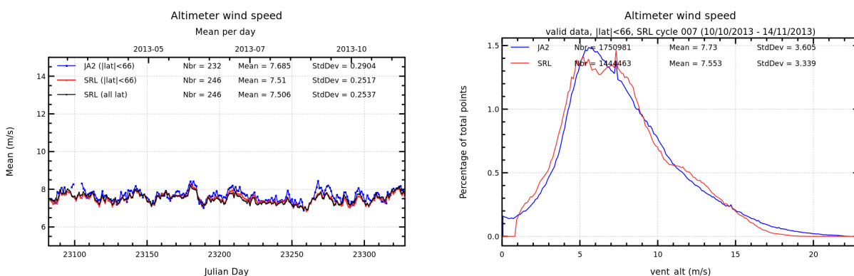
FIGURE 10 – Daily monitoring of altimeter wind speed for Saral/AltiKa and Jason-2 on the left and histogram for cycle 007 on the right (limited to 66° latitude).
