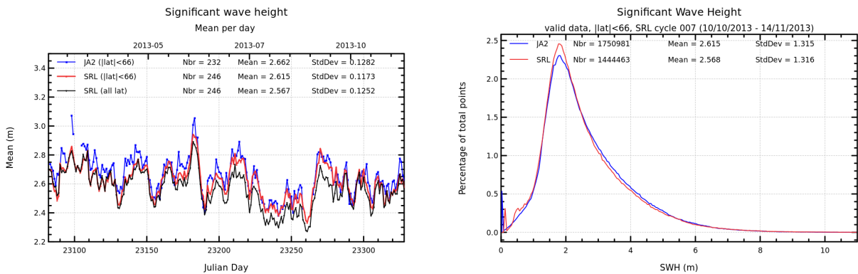
FIGURE 6 – Daily monitoring of significant wave height for AltiKa (Ka-band) and Jason-2 (Ku-band) on the left and histogram for cycle 007 on the right (limited to 66° latitude).
