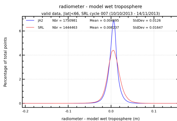
FIGURE 13 – Histogram of wet troposphere differences between radiometer and ECMWF model for cycle 007.
