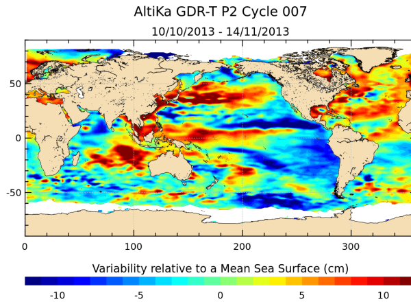
FIGURE 19 – Sea level anomaly relative to MSS for cycle 007.
