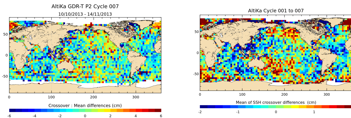
FIGURE 14 – Mean SSH at crossovers for cycle 007 (left) and over the whole Saral/AltiKa period (right).
