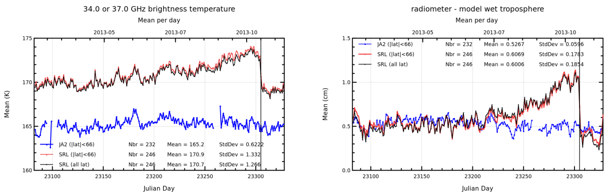
FIGURE 12 – Daily monitoring of 34 GHz (Jason-2) and 37 GHz (Saral/AltiKa) brightness temperature (left) and daily monitoring of wet troposphere differences between radiometer and ECMWF model (right) for Saral/AltiKa and Jason-2. Black vertical line : modification of the onboard radiometer database value.
