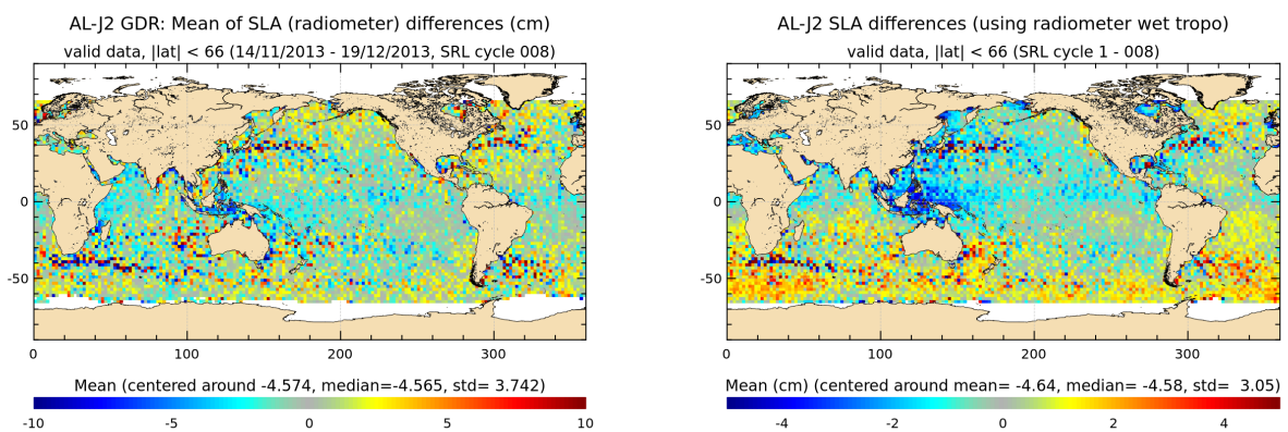
FIGURE 20 – Saral/AltiKa – Jason-2 SLA differences for cycle 008 (left) and averaged over the whole Saral/AltiKa period (right)
