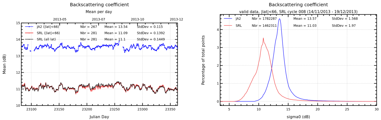
FIGURE 7 – Daily monitoring of backscattering coefficient for Saral/AltiKa and Jason-2 on the left and histogram for cycle 008 on the right (limited to 66° latitude).
