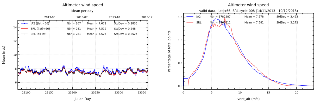
FIGURE 10 – Daily monitoring of altimeter wind speed for Saral/AltiKa and Jason-2 on the left and histogram for cycle 008 on the right (limited to 66° latitude).
