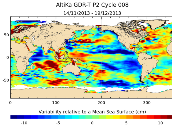
FIGURE 18 – Sea level anomaly relative to MSS for cycle 008.
