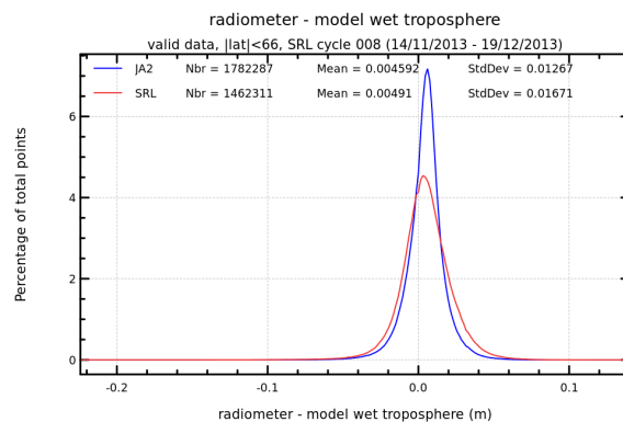
FIGURE 12 – Histogram of wet troposphere differences between radiometer and ECMWF model for cycle 008.
