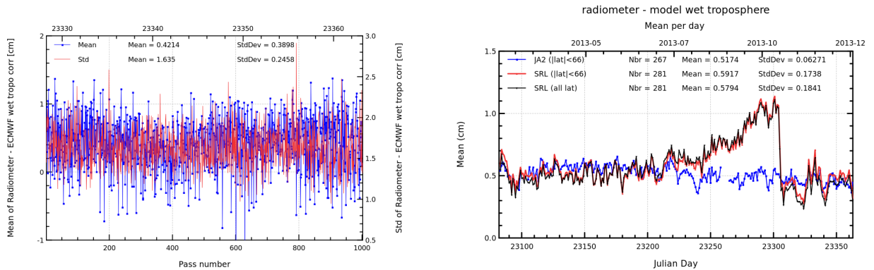
FIGURE 11 – Pass monitoring of wet troposphere differences between radiometer and ECMWF model for Saral/AltiKa cycle 008 (left) and daily monitoring of wet troposphere differences between radiometer and ECMWF model (right).
