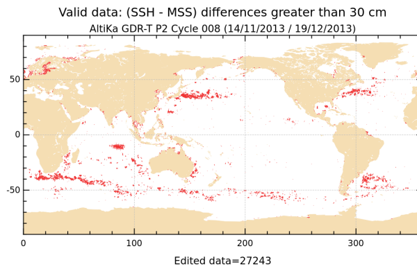
FIGURE 19 – Differences higher than a 30 cm threshold for cycle 008.
