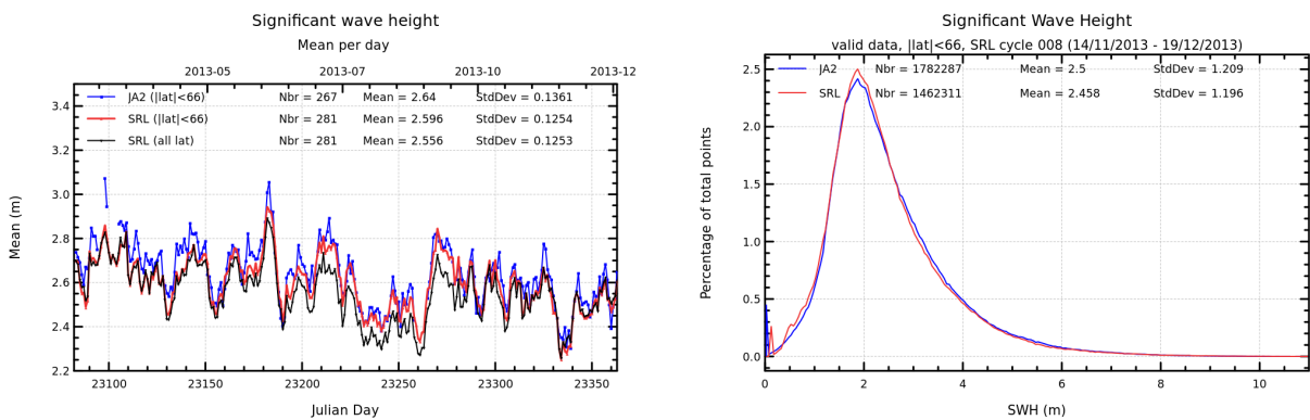
FIGURE 6 – Daily monitoring of significant wave height for AltiKa (Ka-band) and Jason-2 (Ku-band) on the left and histogram for cycle 008 on the right (limited to 66° latitude).
