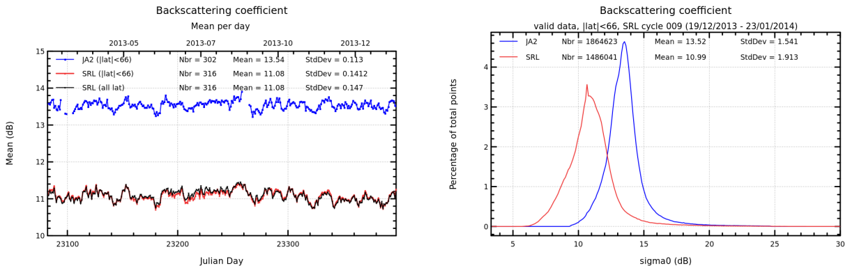
FIGURE 7 – Daily monitoring of backscattering coefficient for Saral/AltiKa and Jason-2 on the left and histogram for cycle 009 on the right (limited to 66° latitude).
