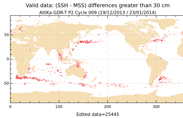
FIGURE 19 – Differences higher than a 30 cm threshold for cycle 009.
