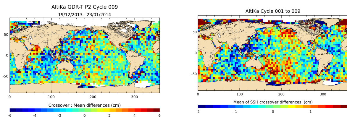
FIGURE 13 – Mean SSH at crossovers for cycle 009 (left) and over the whole Saral/AltiKa period (right).
