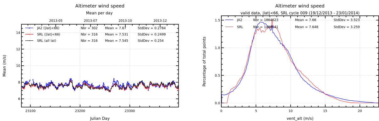
FIGURE 10 – Daily monitoring of altimeter wind speed for Saral/AltiKa and Jason-2 on the left and histogram for cycle 009 on the right (limited to 66° latitude).
