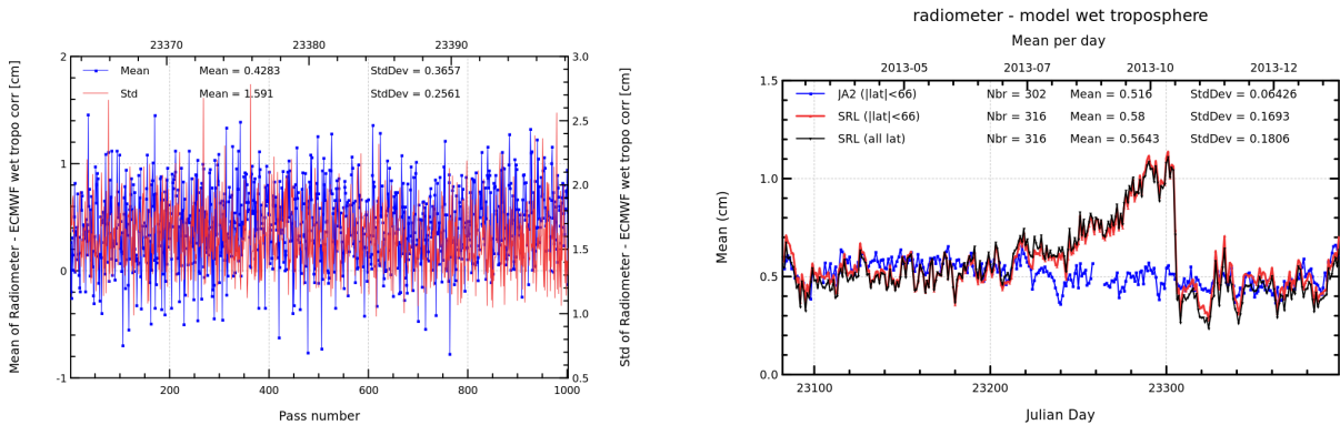
FIGURE 11 – Pass monitoring of wet troposphere differences between radiometer and ECMWF model for Saral/AltiKa cycle 009 (left) and daily monitoring of wet troposphere differences between radiometer and ECMWF model (right).
