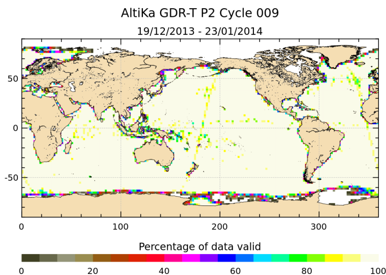
FIGURE 3 – Percentage of valid measurements for cycle 009. Note that zones, which do not have any valid data (e.g. completely covered by sea ice) are not shown (=white).
