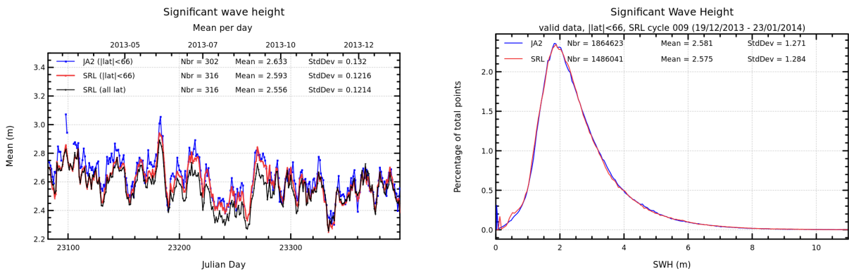
FIGURE 6 – Daily monitoring of significant wave height for AltiKa (Ka-band) and Jason-2 (Ku-band) on the left and histogram for cycle 009 on the right (limited to 66° latitude).
