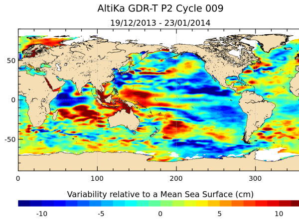
FIGURE 18 – Sea level anomaly relative to MSS for cycle 009.
