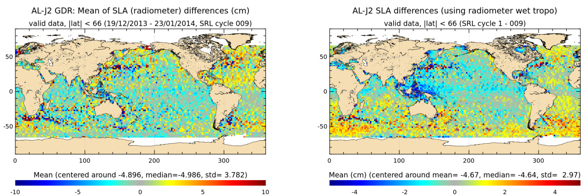
FIGURE 20 – Saral/AltiKa – Jason-2 SLA differences for cycle 009 (left) and averaged over the whole Saral/AltiKa period (right)
