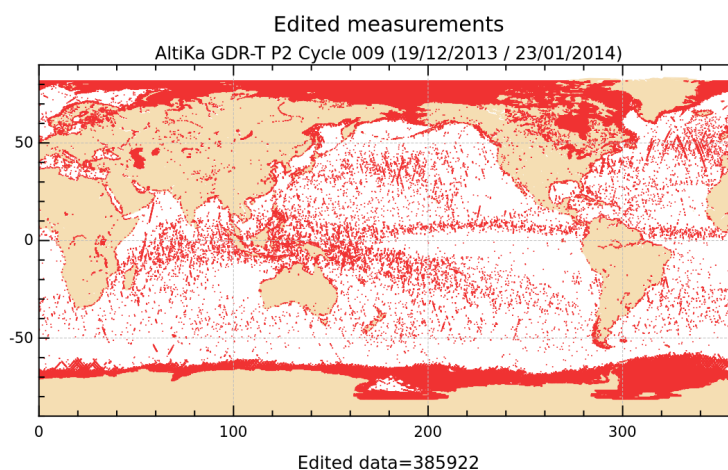
FIGURE 2 – Edited measurements for cycle 009.
