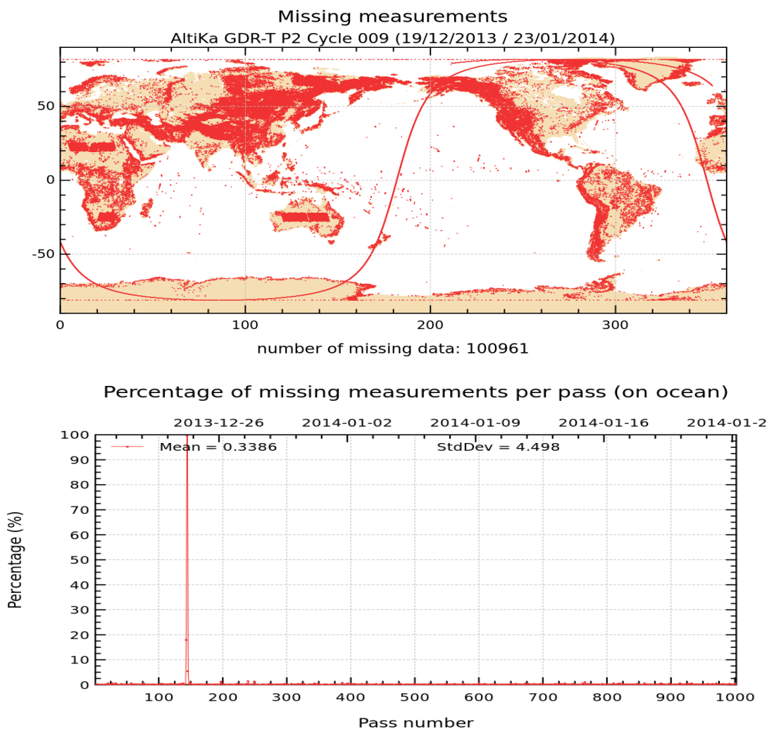
FIGURE 1 – Map of missing measurements for cycle 009 on top. Monitoring of percentage of missing ocean measurements per pass on bottom
