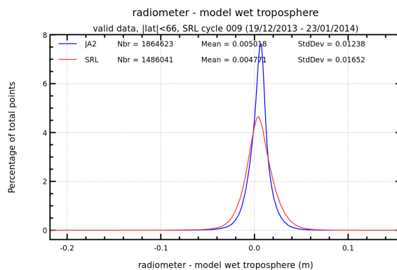
FIGURE 12 – Histogram of wet troposphere differences between radiometer and ECMWF model for cycle 009.
