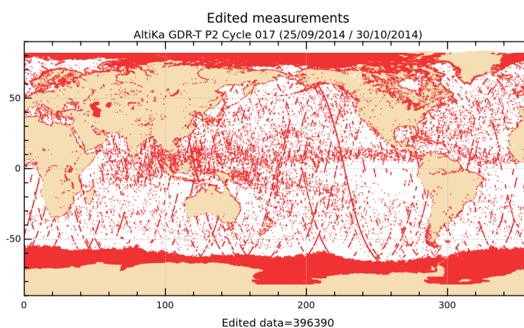
FIGURE 2 – Edited measurements for cycle 017.
