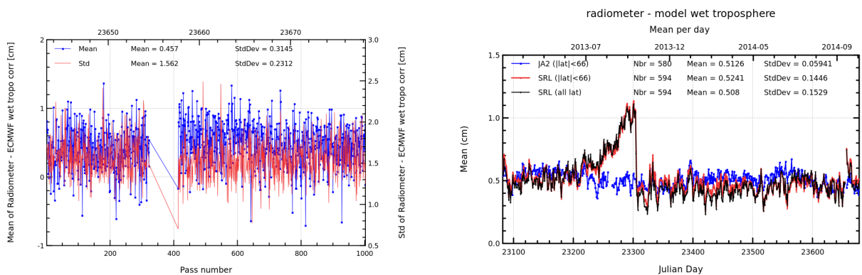
FIGURE 11 – Pass monitoring of wet troposphere differences between radiometer and ECMWF model for Saral/AltiKa cycle 017 (left) and daily monitoring of wet troposphere differences between radiometer and ECMWF model (right).
