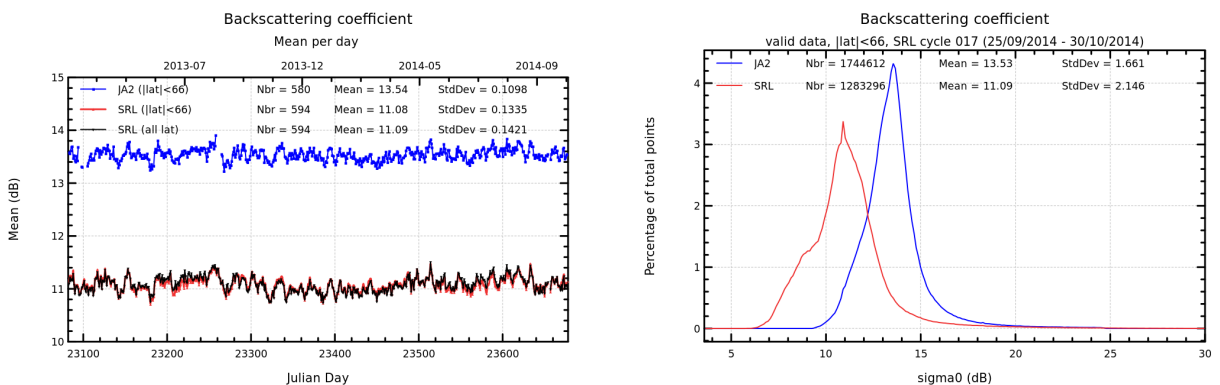
FIGURE 7 – Daily monitoring of backscattering coefficient for Saral/AltiKa and Jason-2 on the left and histogram for cycle 017 on the right (limited to 66° latitude).
