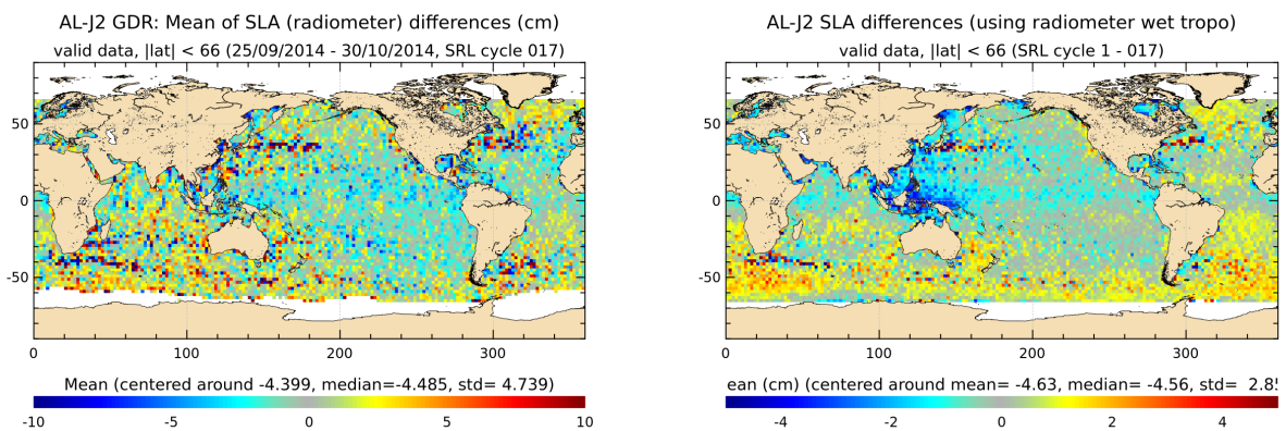
FIGURE 20 – Saral/AltiKa – Jason-2 SLA differences for cycle 017 (left) and averaged over the whole Saral/AltiKa period (right)
