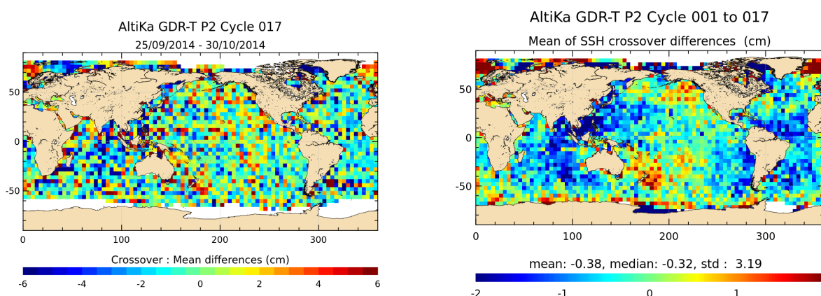
FIGURE 13 – Mean SSH at crossovers for cycle 017 (left) and over the whole Saral/AltiKa period (right).
