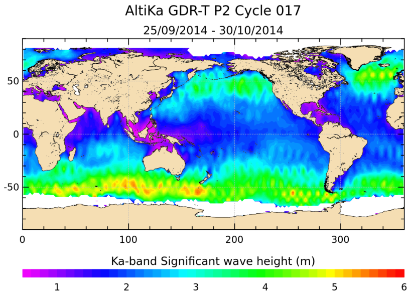
FIGURE 5 – Significant wave height for cycle 017.
