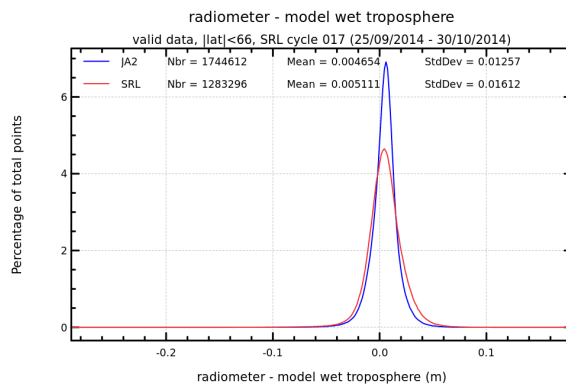
FIGURE 12 – Histogram of wet troposphere differences between radiometer and ECMWF model for cycle 017.
