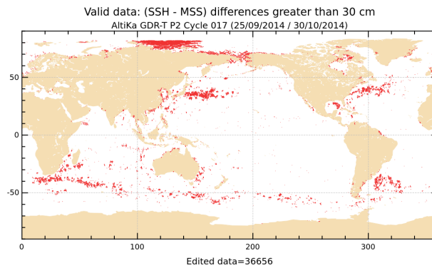
FIGURE 19 – Differences higher than a 30 cm threshold for cycle 017.
