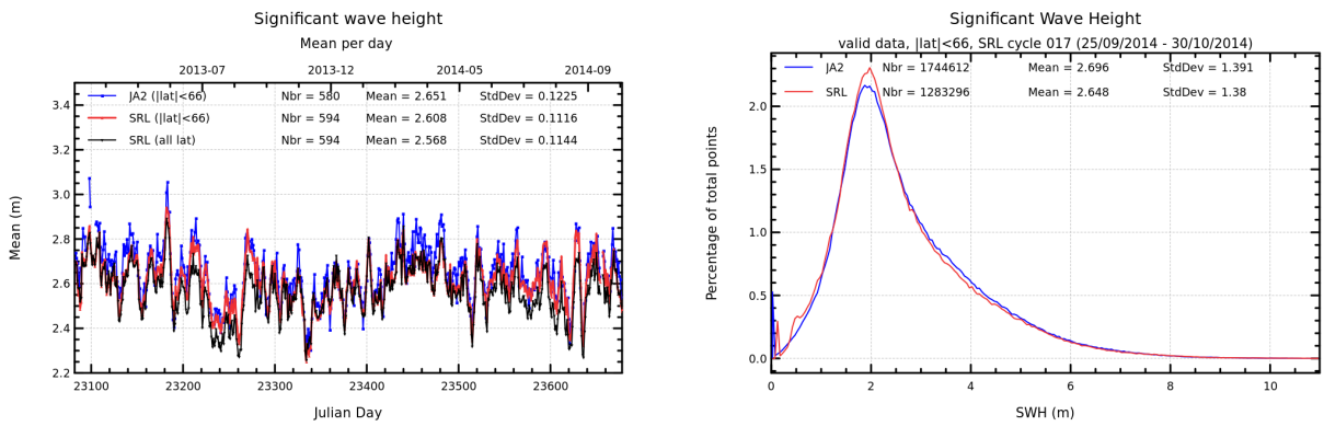
FIGURE 6 – Daily monitoring of significant wave height for AltiKa (Ka-band) and Jason-2 (Ku-band) on the left and histogram for cycle 017 on the right (limited to 66° latitude).
