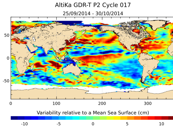
FIGURE 18 – Sea level anomaly relative to MSS for cycle 017.
