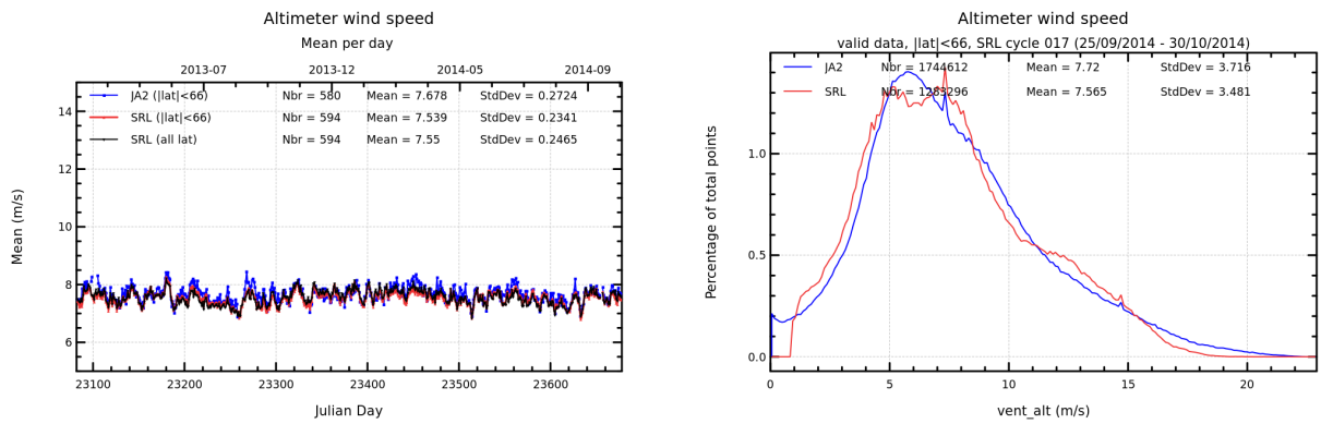
FIGURE 10 – Daily monitoring of altimeter wind speed for Saral/AltiKa and Jason-2 on the left and histogram for cycle 017 on the right (limited to 66° latitude).
