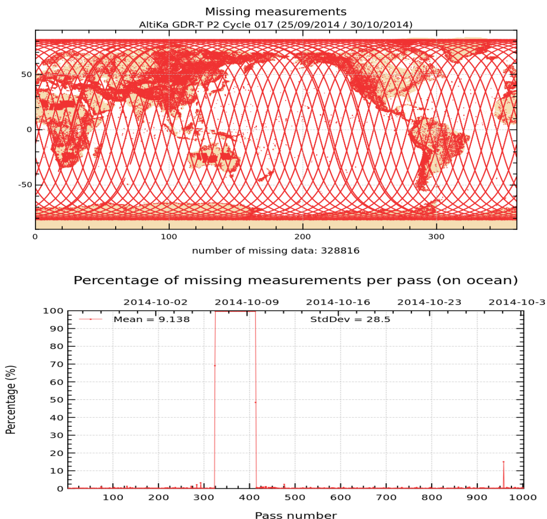
FIGURE 1 – Map of missing measurements for cycle 017 on top. Monitoring of percentage of missing ocean measurements per pass on bottom
