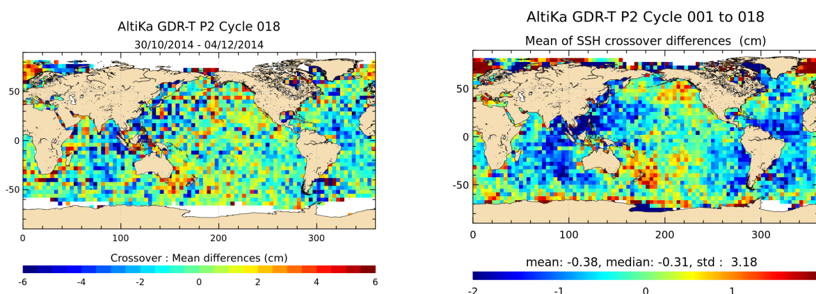
FIGURE 13 – Mean SSH at crossovers for cycle 018 (left) and over the whole Saral/AltiKa period (right).
