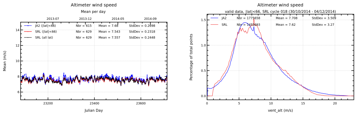
FIGURE 10 – Daily monitoring of altimeter wind speed for Saral/AltiKa and Jason-2 on the left and histogram for cycle 018 on the right (limited to 66° latitude).
