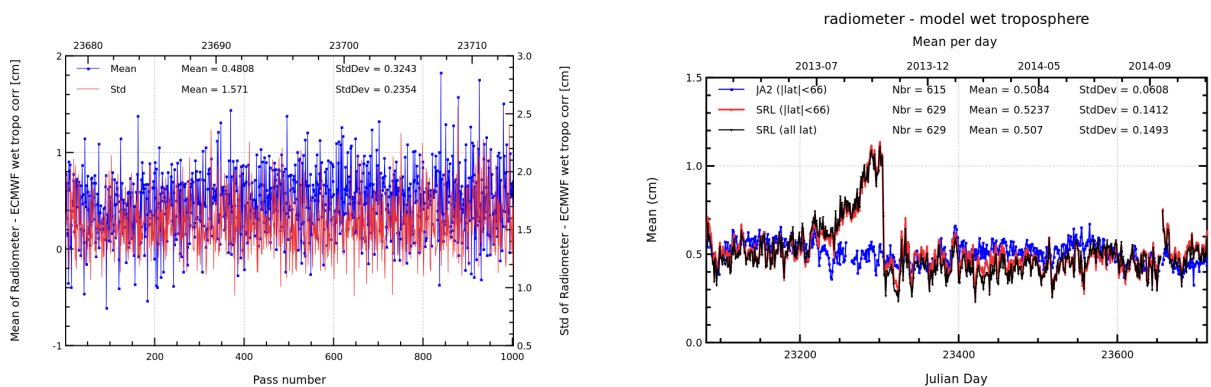
FIGURE 11 – Pass monitoring of wet troposphere differences between radiometer and ECMWF model for Saral/AltiKa cycle 018 (left) and daily monitoring of wet troposphere differences between radiometer and ECMWF model (right).
