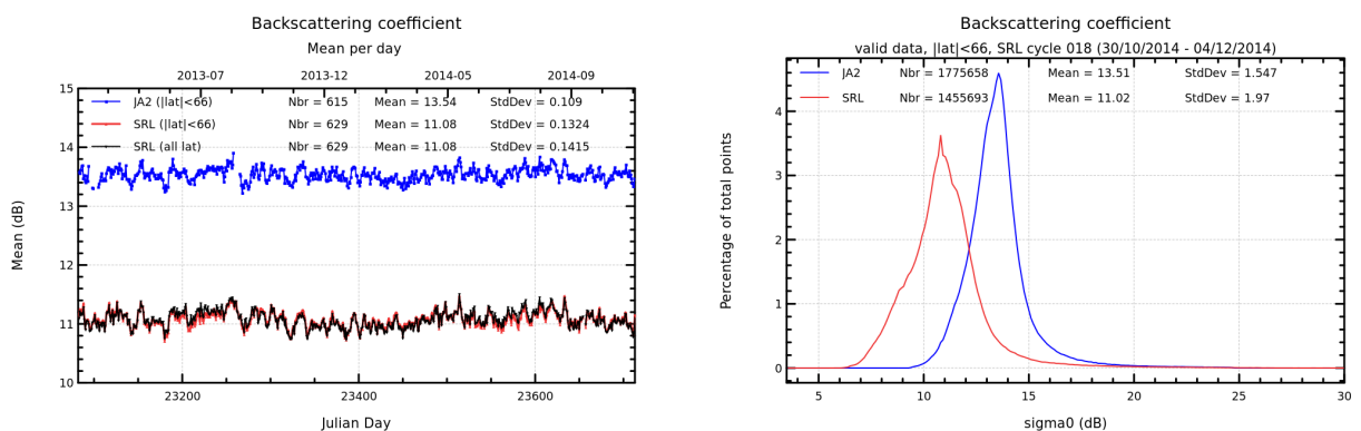
FIGURE 7 – Daily monitoring of backscattering coefficient for Saral/AltiKa and Jason-2 on the left and histogram for cycle 018 on the right (limited to 66° latitude).
