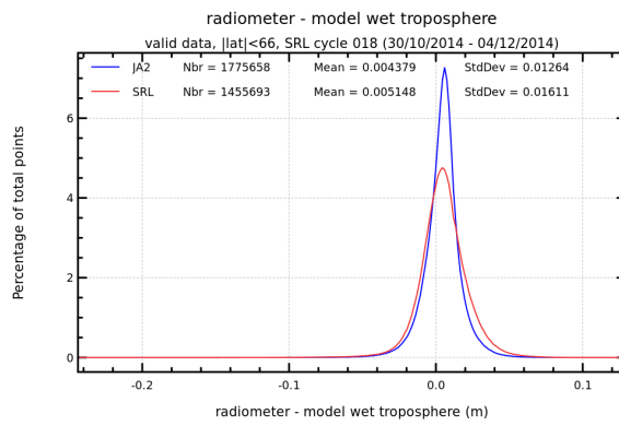
FIGURE 12 – Histogram of wet troposphere differences between radiometer and ECMWF model for cycle 018.
