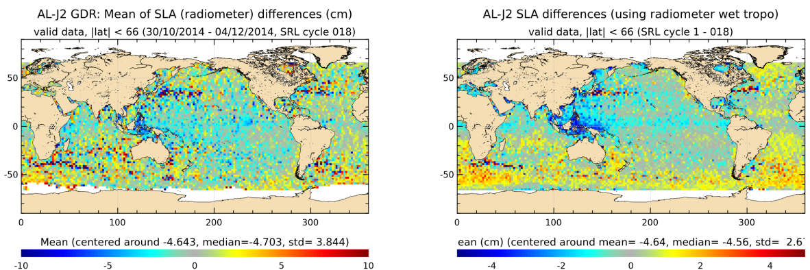
FIGURE 20 – Saral/AltiKa – Jason-2 SLA differences for cycle 018 (left) and averaged over the whole Saral/AltiKa period (right)
