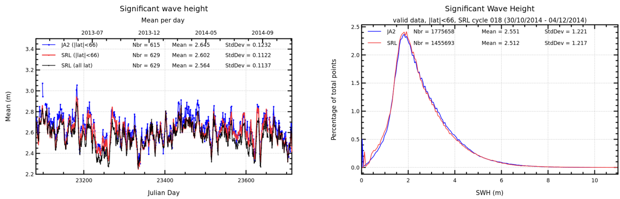
FIGURE 6 – Daily monitoring of significant wave height for AltiKa (Ka-band) and Jason-2 (Ku-band) on the left and histogram for cycle 018 on the right (limited to 66° latitude).
