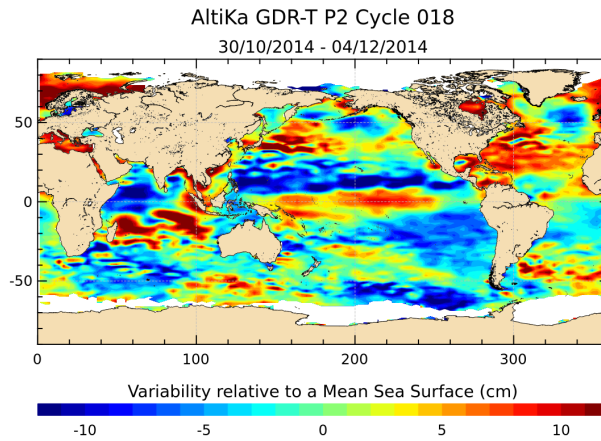
FIGURE 18 – Sea level anomaly relative to MSS for cycle 018.
