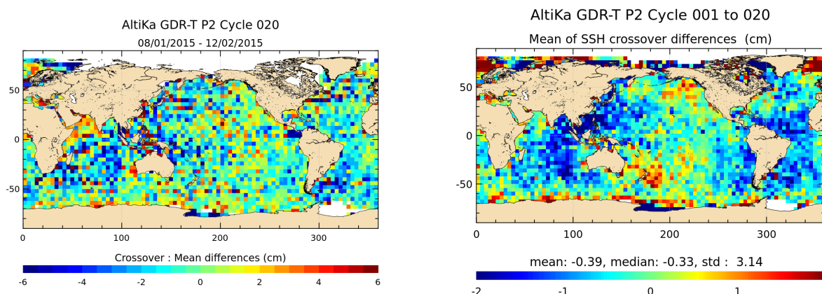
FIGURE 13 – Mean SSH at crossovers for cycle 020 (left) and over the whole Saral/AltiKa period (right).
