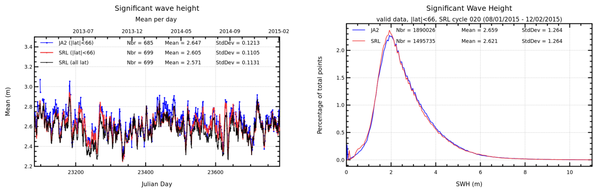
FIGURE 6 – Daily monitoring of significant wave height for AltiKa (Ka-band) and Jason-2 (Ku-band) on the left and histogram for cycle 020 on the right (limited to 66° latitude).
