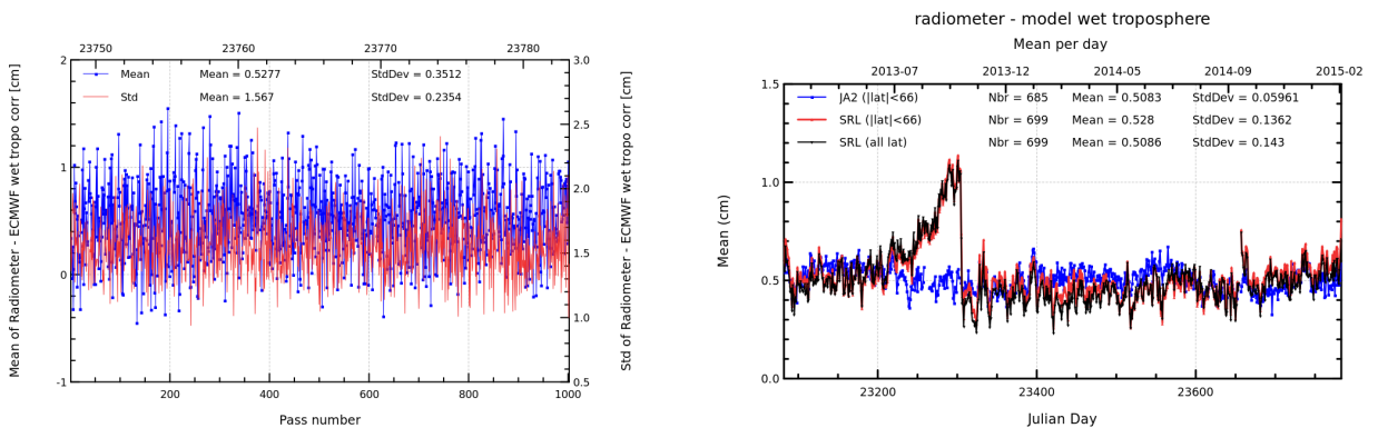
FIGURE 11 – Pass monitoring of wet troposphere differences between radiometer and ECMWF model for Saral/AltiKa cycle 020 (left) and daily monitoring of wet troposphere differences between radiometer and ECMWF model (right).
