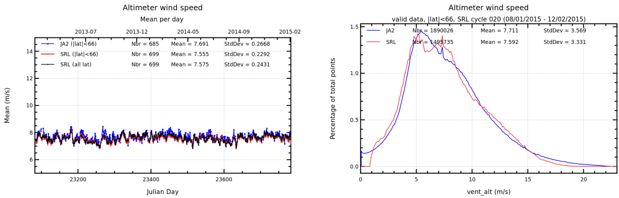
FIGURE 10 – Daily monitoring of altimeter wind speed for Saral/AltiKa and Jason-2 on the left and histogram for cycle 020 on the right (limited to 66° latitude).
