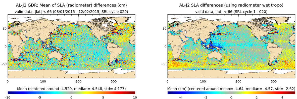
FIGURE 20 – Saral/AltiKa – Jason-2 SLA differences for cycle 020 (left) and averaged over the whole Saral/AltiKa period (right)
