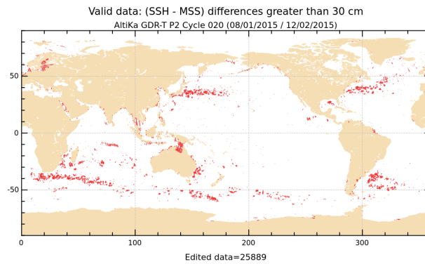
FIGURE 19 – Differences higher than a 30 cm threshold for cycle 020.
