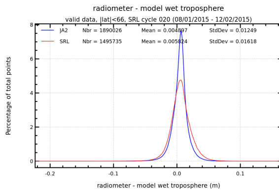
FIGURE 12 – Histogram of wet troposphere differences between radiometer and ECMWF model for cycle 020.
