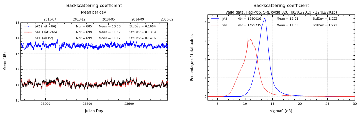
FIGURE 7 – Daily monitoring of backscattering coefficient for Saral/AltiKa and Jason-2 on the left and histogram for cycle 020 on the right (limited to 66° latitude).
