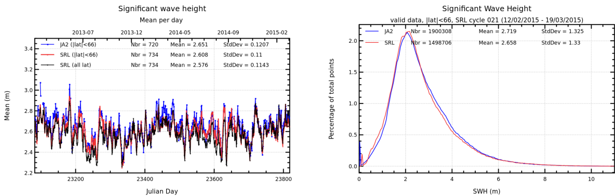
FIGURE 6 – Daily monitoring of significant wave height for AltiKa (Ka-band) and Jason-2 (Ku-band) on the left and histogram for cycle 021 on the right (limited to 66° latitude).
