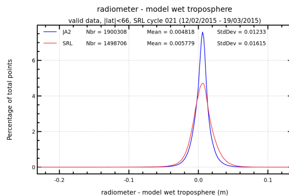
FIGURE 12 – Histogram of wet troposphere differences between radiometer and ECMWF model for cycle 021.
