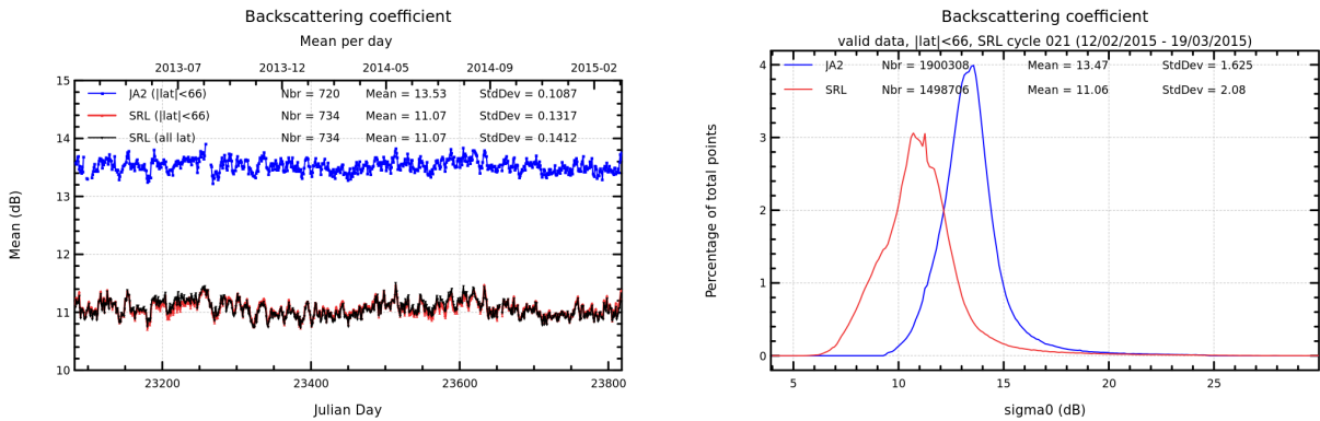
FIGURE 7 – Daily monitoring of backscattering coefficient for Saral/AltiKa and Jason-2 on the left and histogram for cycle 021 on the right (limited to 66° latitude).
