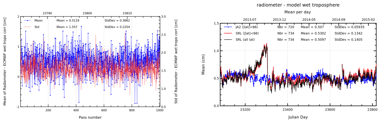
FIGURE 11 – Pass monitoring of wet troposphere differences between radiometer and ECMWF model for Saral/AltiKa cycle 021 (left) and daily monitoring of wet troposphere differences between radiometer and ECMWF model (right).
