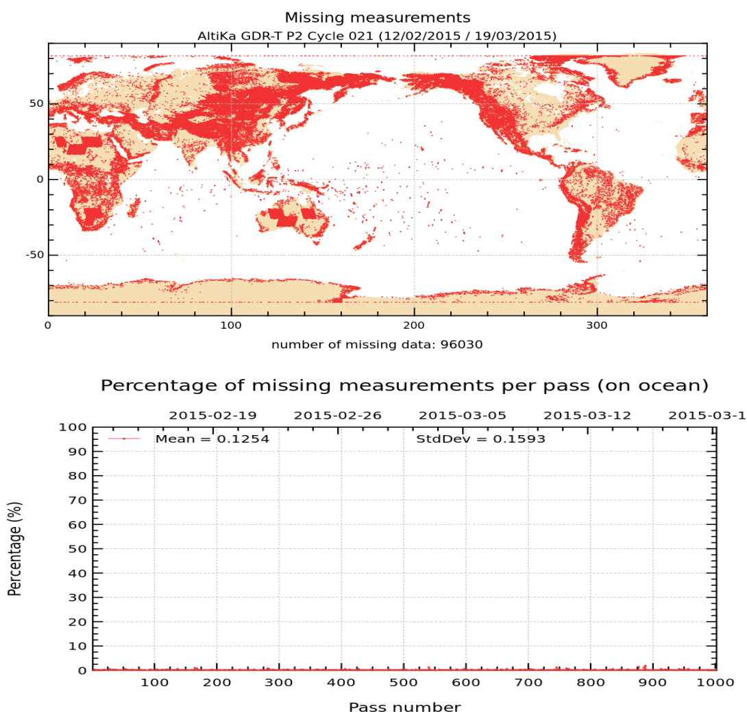
FIGURE 1 – Map of missing measurements for cycle 021 on top. Monitoring of percentage of missing ocean measurements per pass on bottom
