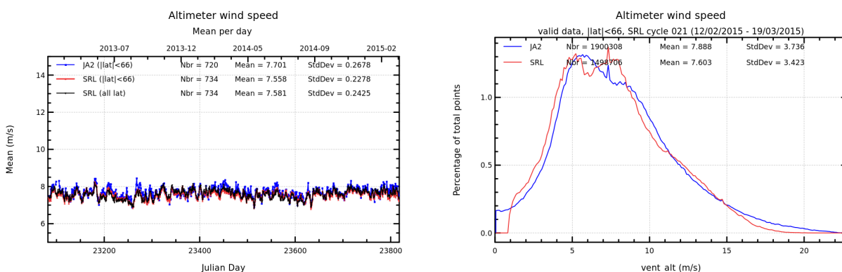
FIGURE 10 – Daily monitoring of altimeter wind speed for Saral/AltiKa and Jason-2 on the left and histogram for cycle 021 on the right (limited to 66° latitude).
