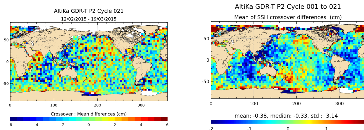
FIGURE 13 – Mean SSH at crossovers for cycle 021 (left) and over the whole Saral/AltiKa period (right).
