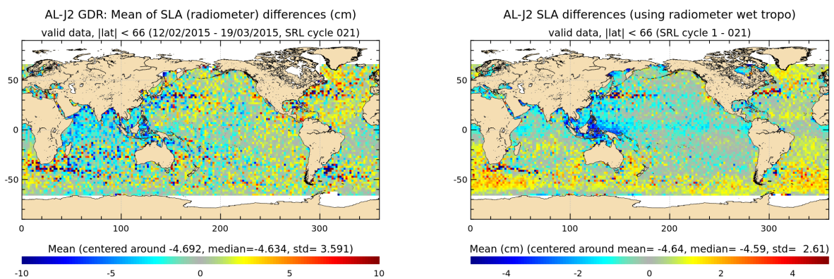
FIGURE 20 – Saral/AltiKa – Jason-2 SLA differences for cycle 021 (left) and averaged over the whole Saral/AltiKa period (right)
