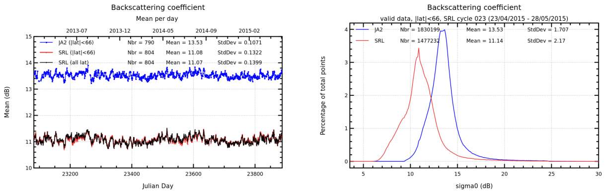
FIGURE 7 – Daily monitoring of backscattering coefficient for Saral/AltiKa and Jason-2 on the left and histogram for cycle 023 on the right (limited to 66° latitude).
