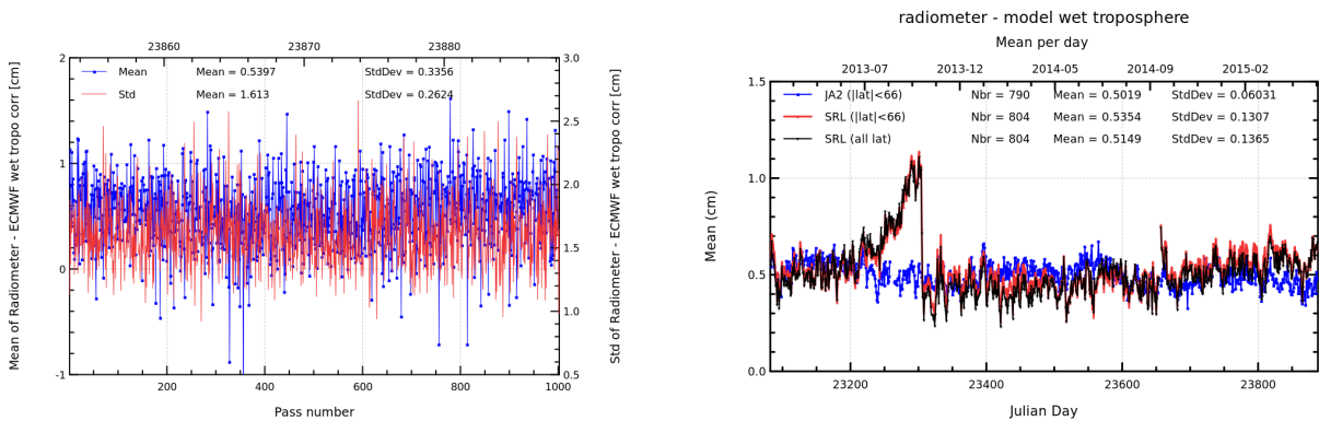
FIGURE 11 – Pass monitoring of wet troposphere differences between radiometer and ECMWF model for Saral/AltiKa cycle 023 (left) and daily monitoring of wet troposphere differences between radiometer and ECMWF model (right).
