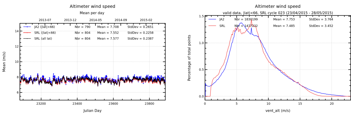
FIGURE 10 – Daily monitoring of altimeter wind speed for Saral/AltiKa and Jason-2 on the left and histogram for cycle 023 on the right (limited to 66° latitude).
