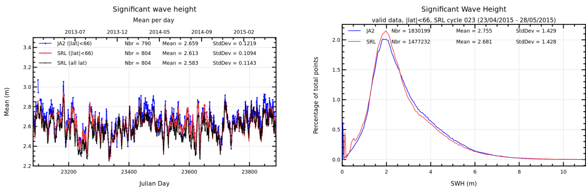
FIGURE 6 – Daily monitoring of significant wave height for AltiKa (Ka-band) and Jason-2 (Ku-band) on the left and histogram for cycle 023 on the right (limited to 66° latitude).
