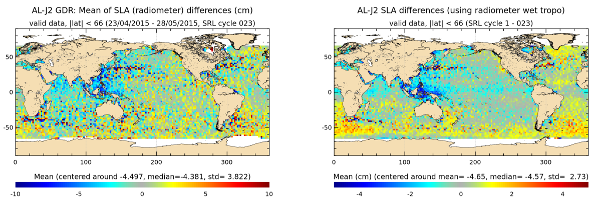
FIGURE 20 – Saral/AltiKa – Jason-2 SLA differences for cycle 023 (left) and averaged over the whole Saral/AltiKa period (right)
