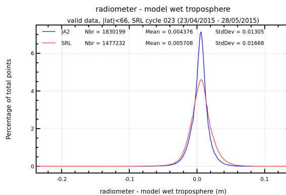
FIGURE 12 – Histogram of wet troposphere differences between radiometer and ECMWF model for cycle 023.
