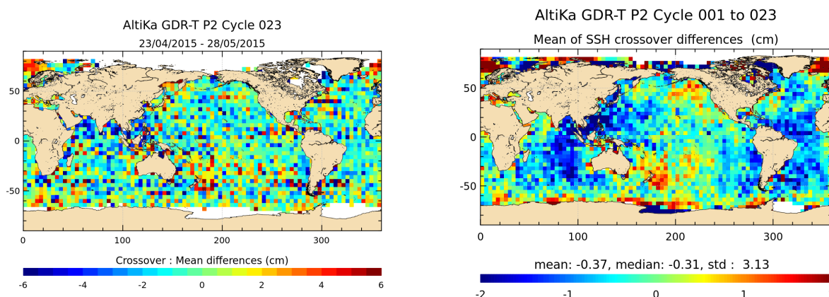
FIGURE 13 – Mean SSH at crossovers for cycle 023 (left) and over the whole Saral/AltiKa period (right).
