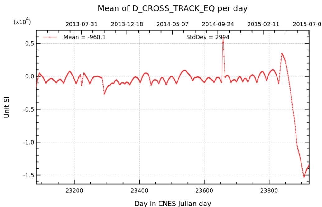
FIGURE 22 – Daily monitoring of SARAL/AltiKa's cross-track deviation from the nominal ground track until the end of cycle 24.
