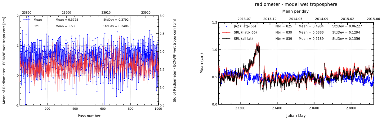
FIGURE 11 – Pass monitoring of wet troposphere differences between radiometer and ECMWF model for Saral/AltiKa cycle 024 (left) and daily monitoring of wet troposphere differences between radiometer and ECMWF model (right).
