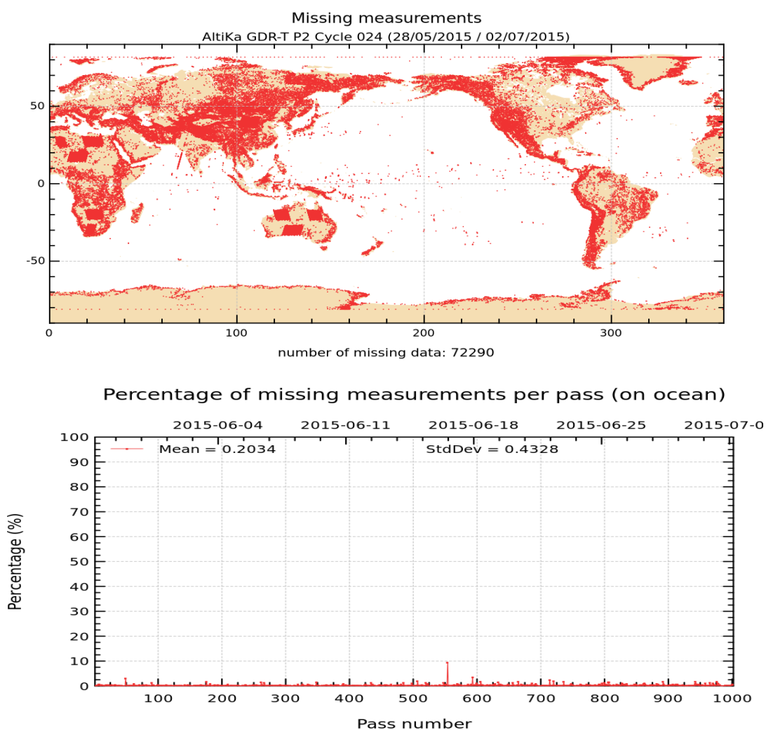
FIGURE 1 – Map of missing measurements for cycle 024 on top. Monitoring of percentage of missing ocean measurements per pass on bottom
