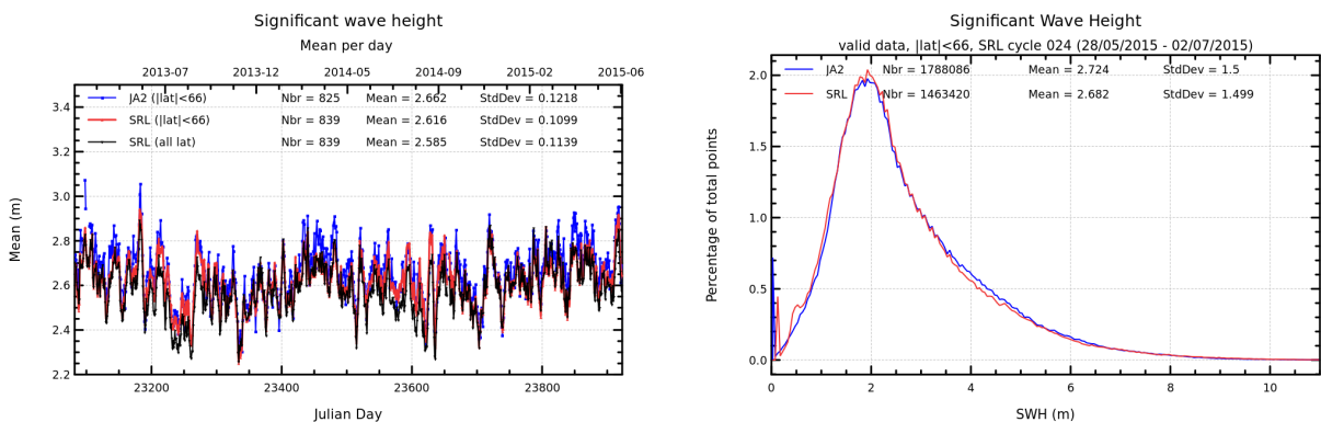
FIGURE 6 – Daily monitoring of significant wave height for AltiKa (Ka-band) and Jason-2 (Ku-band) on the left and histogram for cycle 024 on the right (limited to 66° latitude).
