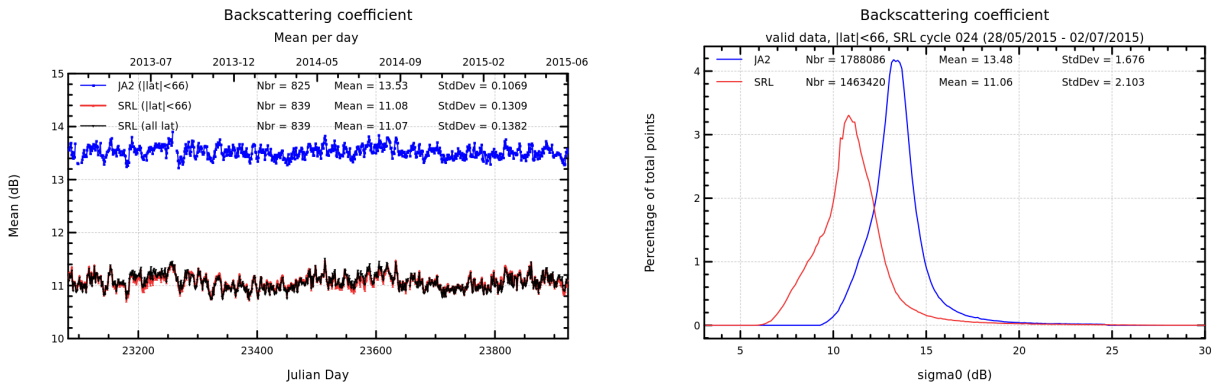
FIGURE 7 – Daily monitoring of backscattering coefficient for Saral/AltiKa and Jason-2 on the left and histogram for cycle 024 on the right (limited to 66° latitude).
