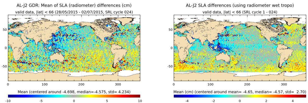
FIGURE 20 – Saral/AltiKa – Jason-2 SLA differences for cycle 024 (left) and averaged over the whole Saral/AltiKa period (right)
