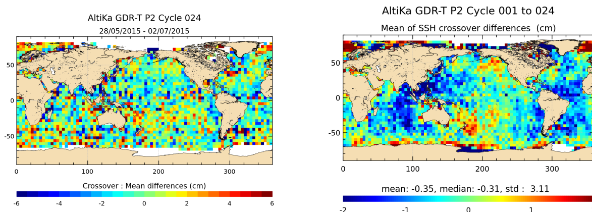
FIGURE 13 – Mean SSH at crossovers for cycle 024 (left) and over the whole Saral/AltiKa period (right).
