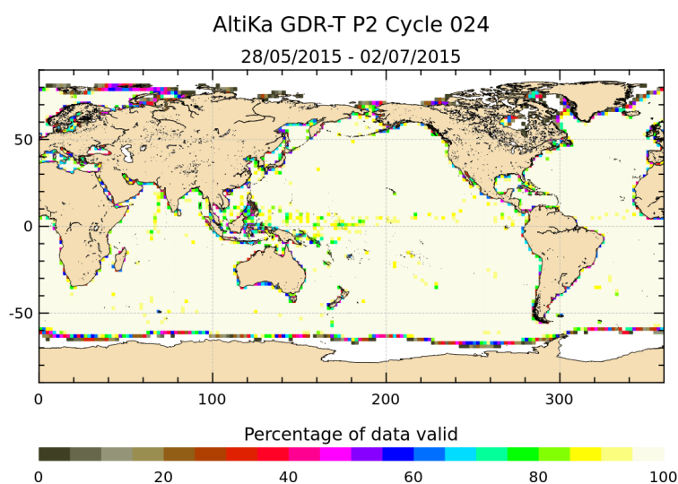
FIGURE 3 – Percentage of valid measurements for cycle 024. Note that zones, which do not have any valid data (e.g. completely covered by sea ice) are not shown (=white).
