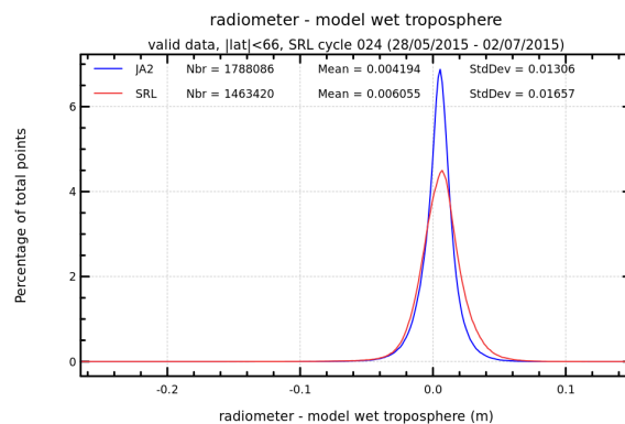
FIGURE 12 – Histogram of wet troposphere differences between radiometer and ECMWF model for cycle 024.
