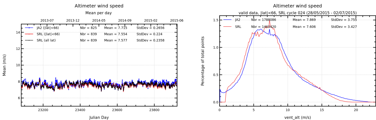
FIGURE 10 – Daily monitoring of altimeter wind speed for Saral/AltiKa and Jason-2 on the left and histogram for cycle 024 on the right (limited to 66° latitude).
