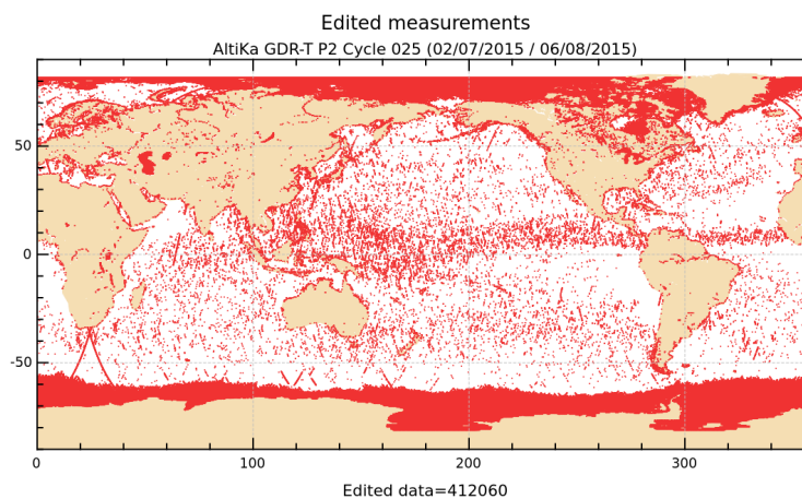
FIGURE 2 – Edited measurements for cycle 025.
