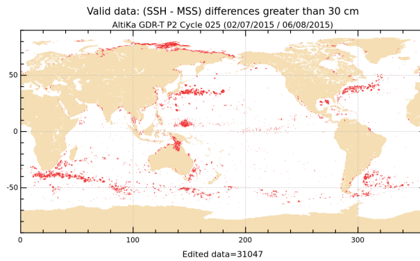
FIGURE 20 – Differences higher than a 30 cm threshold for cycle 025.
