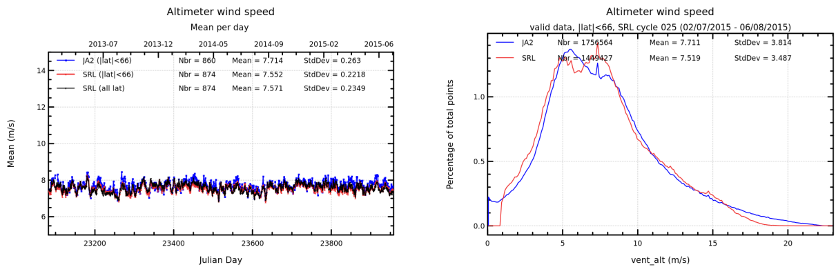
FIGURE 11 – Daily monitoring of altimeter wind speed for Saral/AltiKa and Jason-2 on the left and histogram for cycle 025 on the right (limited to 66° latitude).
