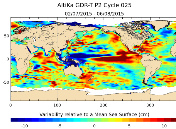
FIGURE 19 – Sea level anomaly relative to MSS for cycle 025.
