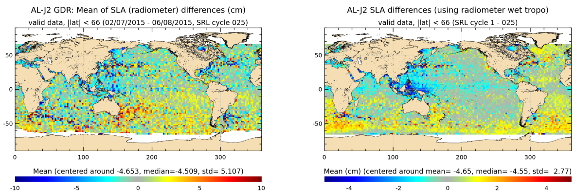
FIGURE 21 – Saral/AltiKa – Jason-2 SLA differences for cycle 025 (left) and averaged over the whole Saral/AltiKa period (right)
