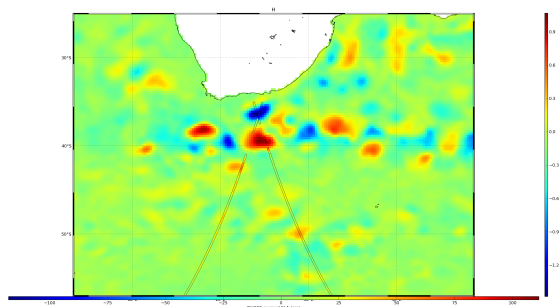
FIGURE 3 – Overlaying SARAL/AltiKa SLA along passes 528 and 601 with DUACS map.
