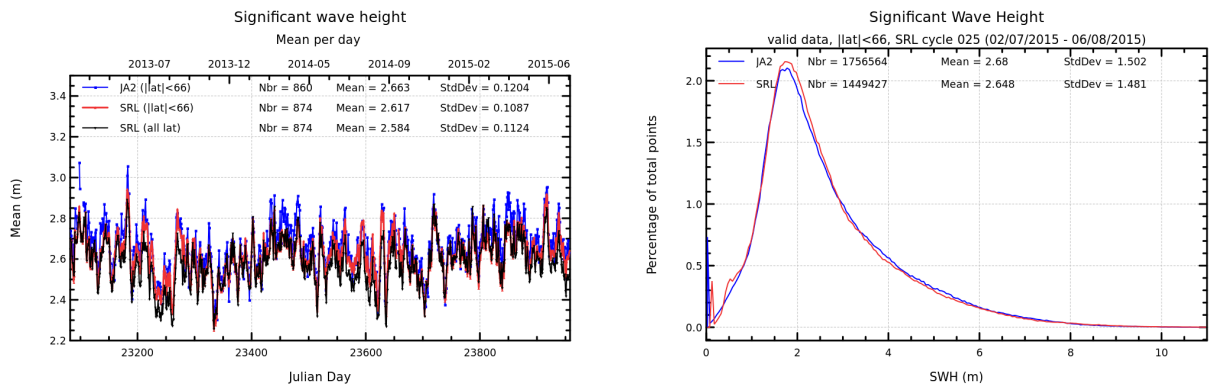
FIGURE 7 – Daily monitoring of significant wave height for AltiKa (Ka-band) and Jason-2 (Ku-band) on the left and histogram for cycle 025 on the right (limited to 66° latitude).
