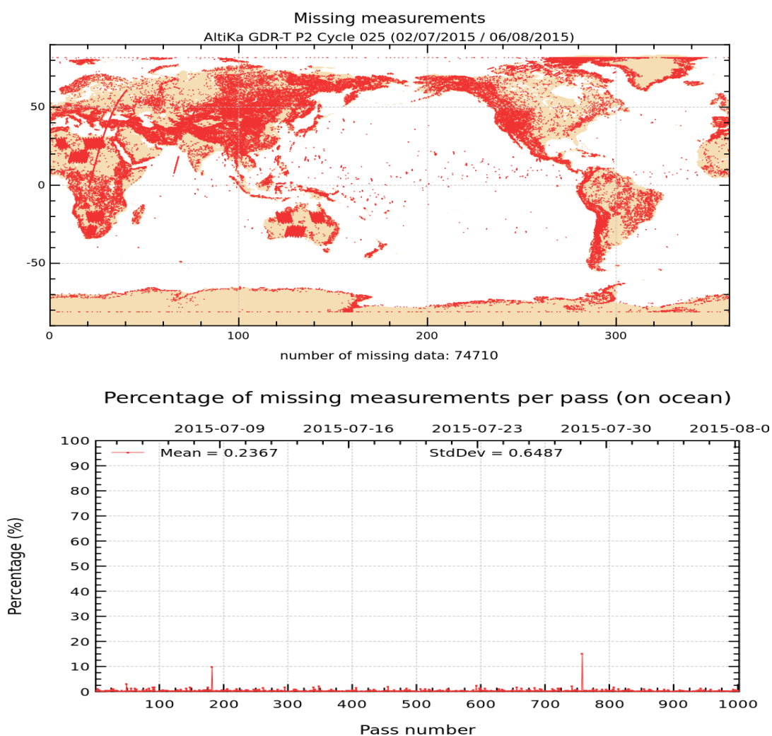
FIGURE 1 – Map of missing measurements for cycle 025 on top. Monitoring of percentage of missing ocean measurements per pass on bottom
