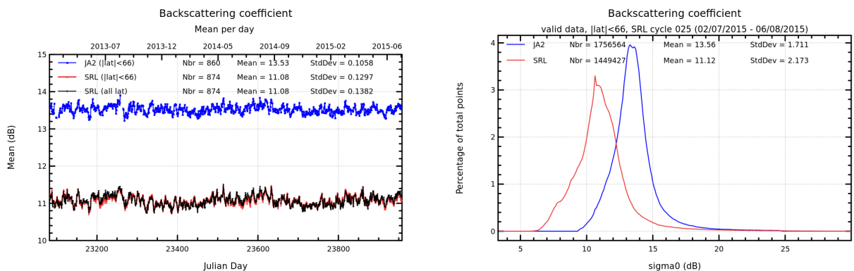
FIGURE 8 – Daily monitoring of backscattering coefficient for Saral/AltiKa and Jason-2 on the left and histogram for cycle 025 on the right (limited to 66° latitude).
