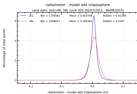
FIGURE 13 – Histogram of wet troposphere differences between radiometer and ECMWF model for cycle 025.
