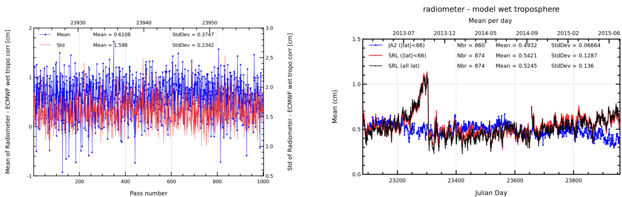
FIGURE 12 – Pass monitoring of wet troposphere differences between radiometer and ECMWF model for Saral/AltiKa cycle 025 (left) and daily monitoring of wet troposphere differences between radiometer and ECMWF model (right).
