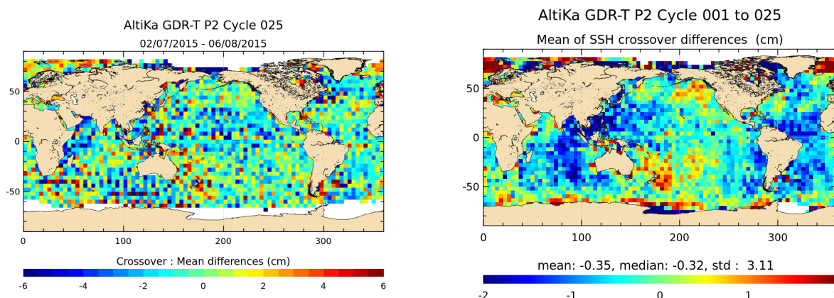
FIGURE 14 – Mean SSH at crossovers for cycle 025 (left) and over the whole Saral/AltiKa period (right).
