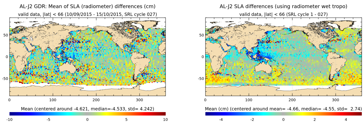
FIGURE 20 – Saral/AltiKa – Jason-2 SLA differences for cycle 027 (left) and averaged over the whole Saral/AltiKa period (right)
