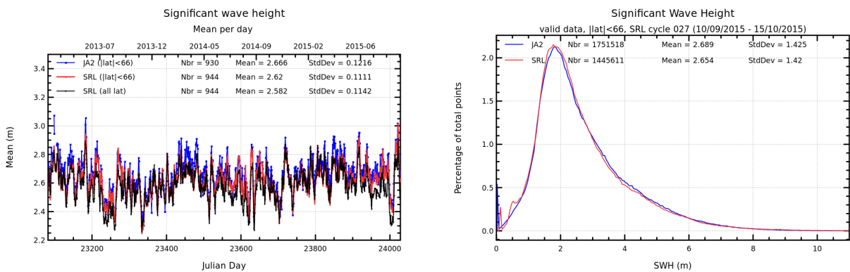
FIGURE 6 – Daily monitoring of significant wave height for AltiKa (Ka-band) and Jason-2 (Ku-band) on the left and histogram for cycle 027 on the right (limited to 66° latitude).
