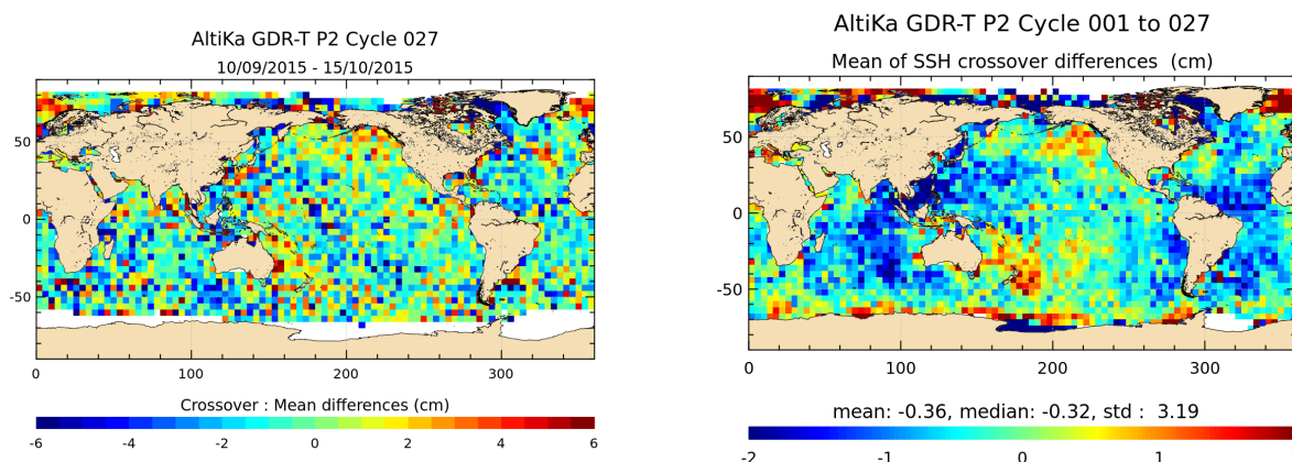
FIGURE 13 – Mean SSH at crossovers for cycle 027 (left) and over the whole Saral/AltiKa period (right).
