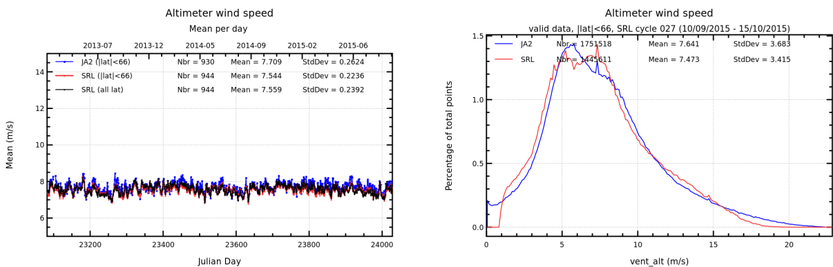
FIGURE 10 – Daily monitoring of altimeter wind speed for Saral/AltiKa and Jason-2 on the left and histogram for cycle 027 on the right (limited to 66° latitude).
