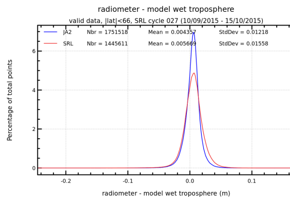
FIGURE 12 – Histogram of wet troposphere differences between radiometer and ECMWF model for cycle 027.
