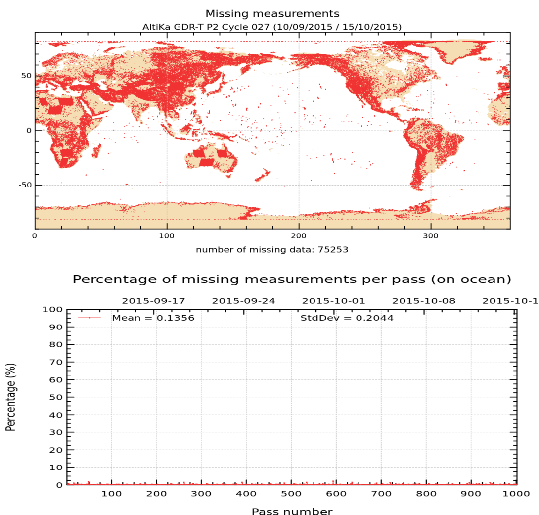
FIGURE 1 – Map of missing measurements for cycle 027 on top. Monitoring of percentage of missing ocean measurements per pass on bottom
