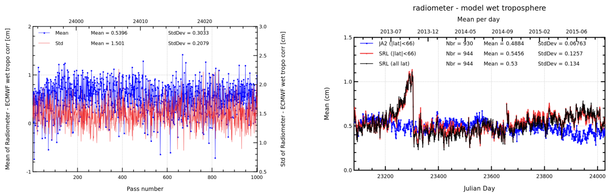
FIGURE 11 – Pass monitoring of wet troposphere differences between radiometer and ECMWF model for Saral/AltiKa cycle 027 (left) and daily monitoring of wet troposphere differences between radiometer and ECMWF model (right).
