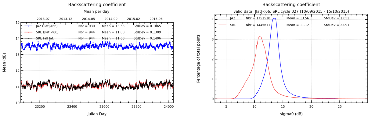
FIGURE 7 – Daily monitoring of backscattering coefficient for Saral/AltiKa and Jason-2 on the left and histogram for cycle 027 on the right (limited to 66° latitude).
