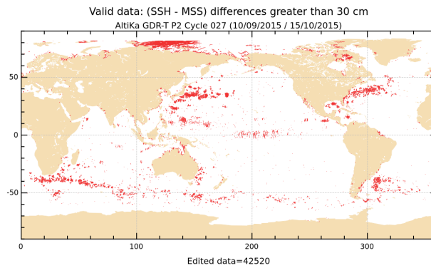
FIGURE 19 – Differences higher than a 30 cm threshold for cycle 027.
