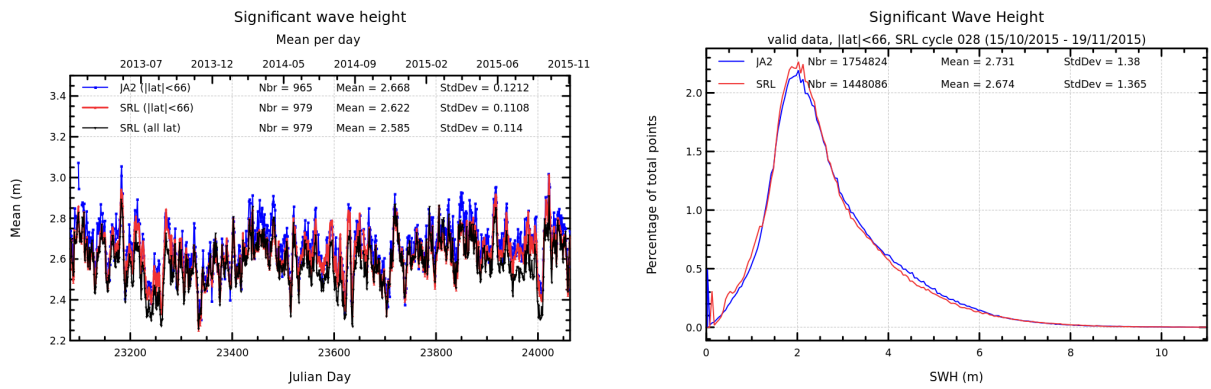
FIGURE 7 – Daily monitoring of significant wave height for AltiKa (Ka-band) and Jason-2 (Ku-band) on the left and histogram for cycle 028 on the right (limited to 66° latitude).
