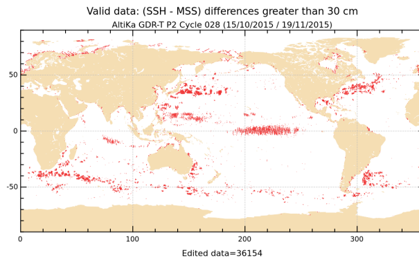
FIGURE 20 – Differences higher than a 30 cm threshold for cycle 028.
