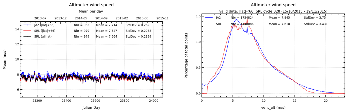
FIGURE 11 – Daily monitoring of altimeter wind speed for Saral/AltiKa and Jason-2 on the left and histogram for cycle 028 on the right (limited to 66° latitude).
