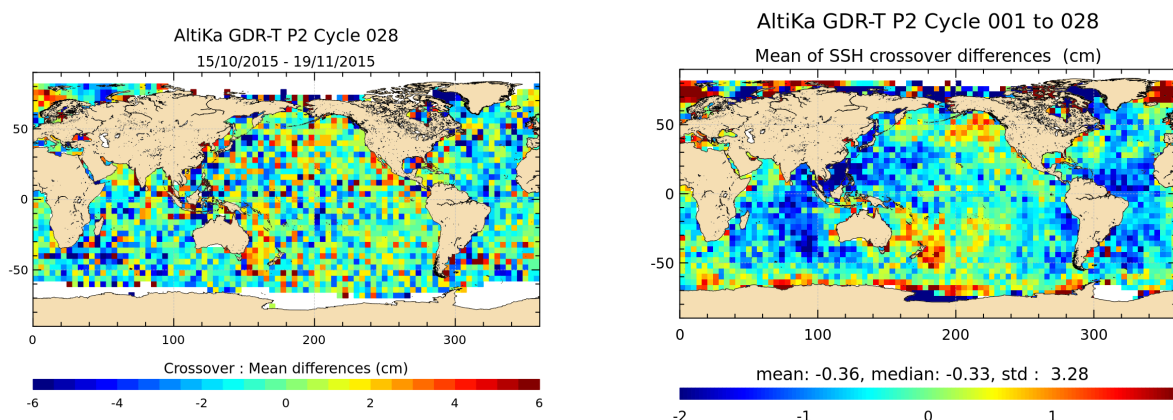
FIGURE 14 – Mean SSH at crossovers for cycle 028 (left) and over the whole Saral/AltiKa period (right).
