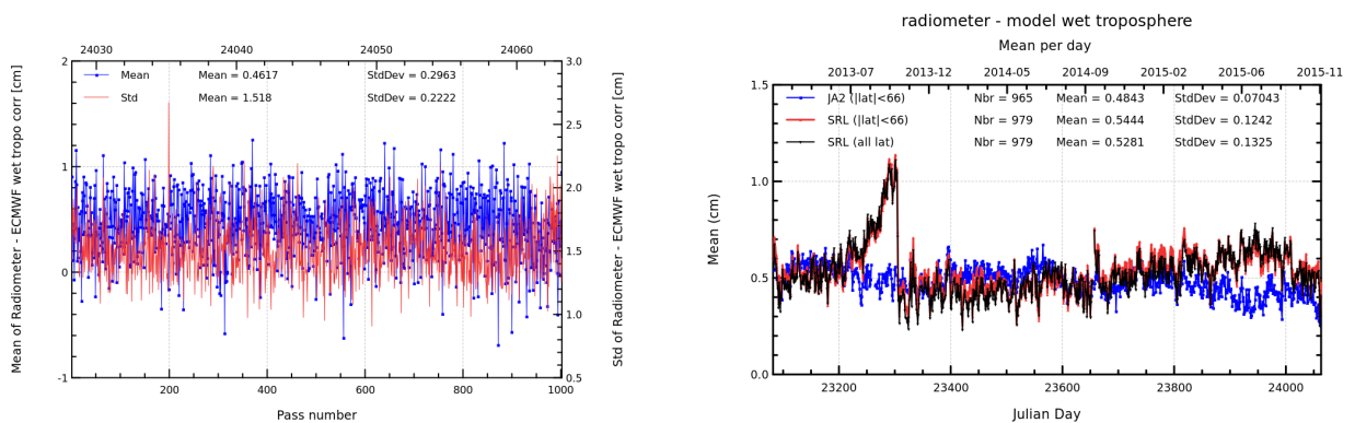
FIGURE 12 – Pass monitoring of wet troposphere differences between radiometer and ECMWF model for Saral/AltiKa cycle 028 (left) and daily monitoring of wet troposphere differences between radiometer and ECMWF model (right).
