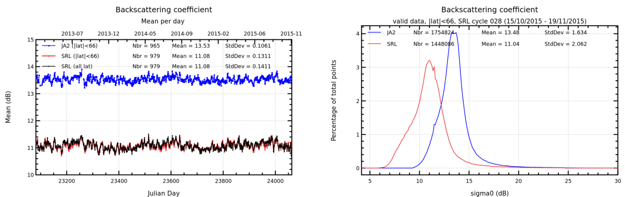
FIGURE 8 – Daily monitoring of backscattering coefficient for Saral/AltiKa and Jason-2 on the left and histogram for cycle 028 on the right (limited to 66° latitude).
