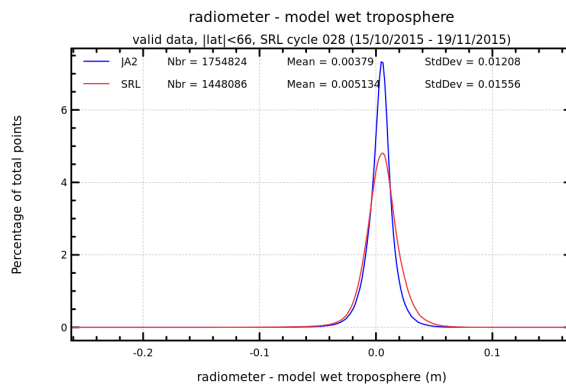
FIGURE 13 – Histogram of wet troposphere differences between radiometer and ECMWF model for cycle 028.
