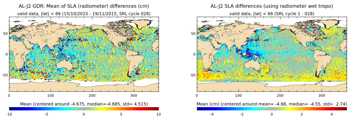
FIGURE 21 – Saral/AltiKa – Jason-2 SLA differences for cycle 028 (left) and averaged over the whole Saral/AltiKa period (right)
