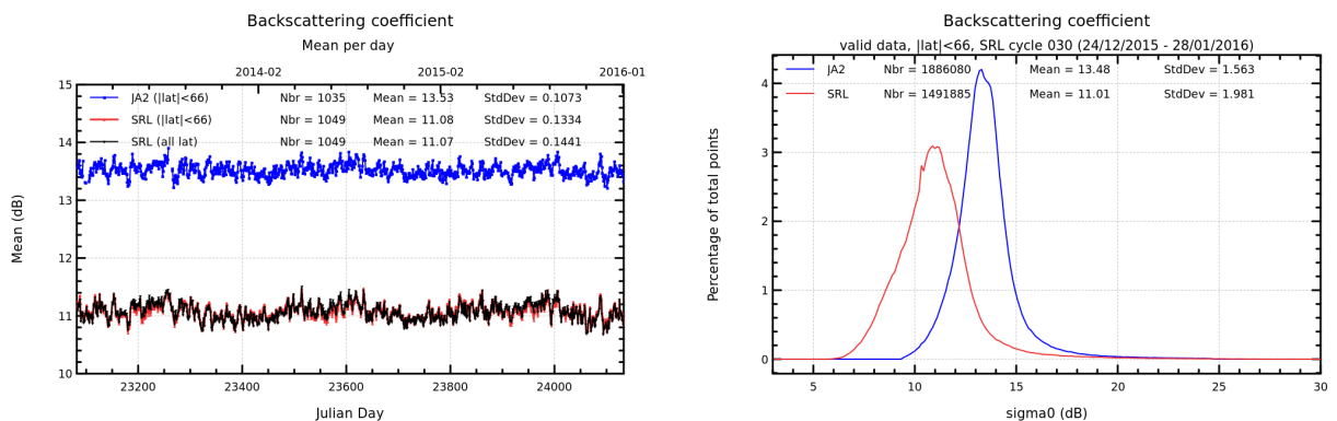
FIGURE 8 – Daily monitoring of backscattering coefficient for Saral/AltiKa and Jason-2 on the left and histogram for cycle 030 on the right (limited to 66° latitude).
