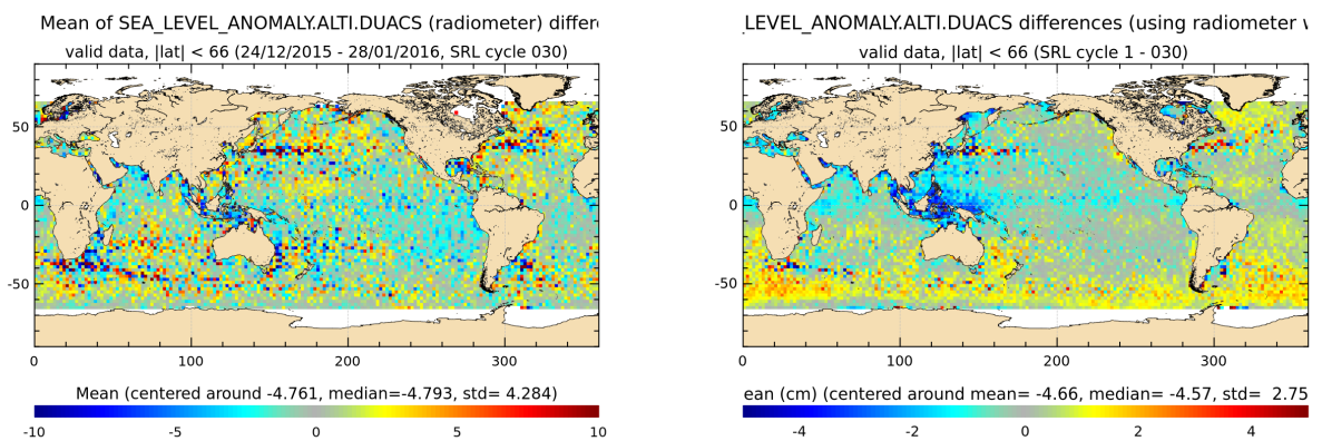
FIGURE 21 – Saral/AltiKa – Jason-2 SLA differences for cycle 030 (left) and averaged over the whole Saral/AltiKa period (right)
