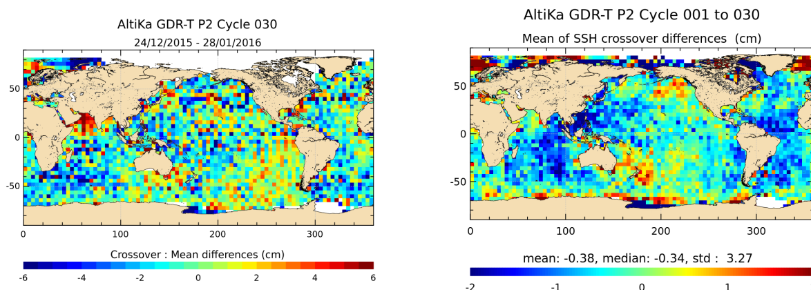
FIGURE 14 – Mean SSH at crossovers for cycle 030 (left) and over the whole Saral/AltiKa period (right).
