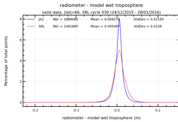
FIGURE 13 – Histogram of wet troposphere differences between radiometer and ECMWF model for cycle 030.
