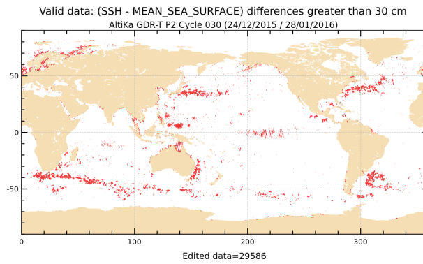
FIGURE 20 – Differences higher than a 30 cm threshold for cycle 030.
