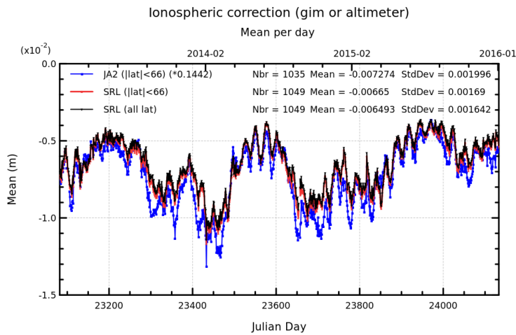
FIGURE 9 – Daily monitoring of dual-frequency ionosphere correction for Jason-2 and GIM ionosphere correction for Saral/AltiKa.
