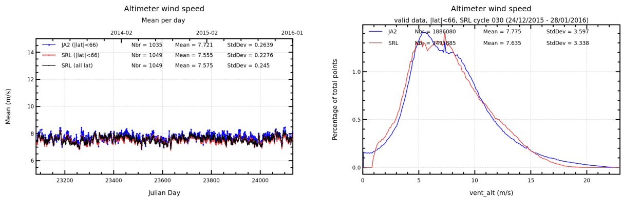
FIGURE 11 – Daily monitoring of altimeter wind speed for Saral/AltiKa and Jason-2 on the left and histogram for cycle 030 on the right (limited to 66° latitude).
