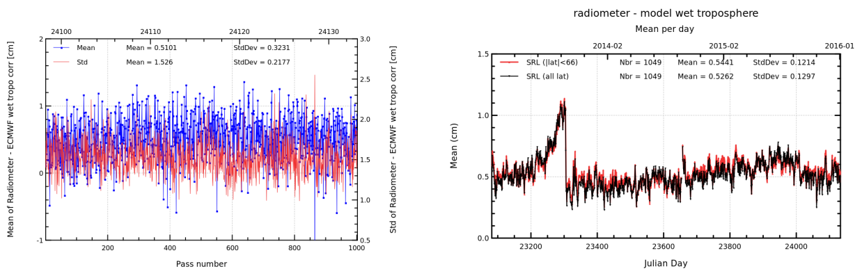
FIGURE 12 – Pass monitoring of wet troposphere differences between radiometer and ECMWF model for Saral/AltiKa cycle 030 (left) and daily monitoring of wet troposphere differences between radiometer and ECMWF model (right).
