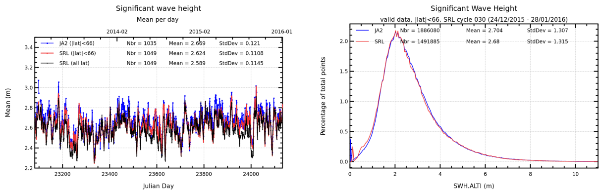
FIGURE 7 – Daily monitoring of significant wave height for AltiKa (Ka-band) and Jason-2 (Ku-band) on the left and histogram for cycle 030 on the right (limited to 66° latitude).
