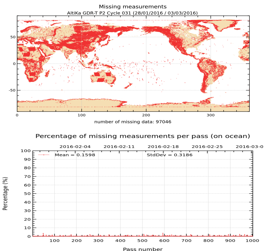
FIGURE 1 – Map of missing measurements for cycle 031 on top. Monitoring of percentage of missing ocean measurements per pass on bottom
