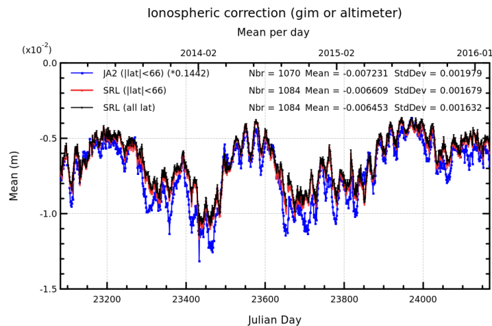
FIGURE 10 – Daily monitoring of dual-frequency ionosphere correction for Jason-2 and GIM ionosphere correction for Saral/AltiKa.
