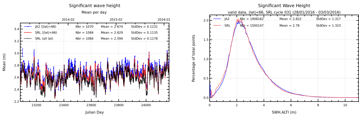
FIGURE 8 – Daily monitoring of significant wave height for AltiKa (Ka-band) and Jason-2 (Ku-band) on the left and histogram for cycle 031 on the right (limited to 66° latitude).
