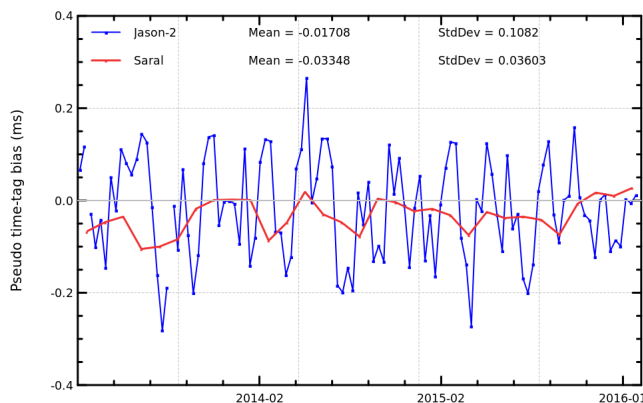
FIGURE 18 – Cyclic monitoring of pseudo time tag bias for Saral/AltiKa.
