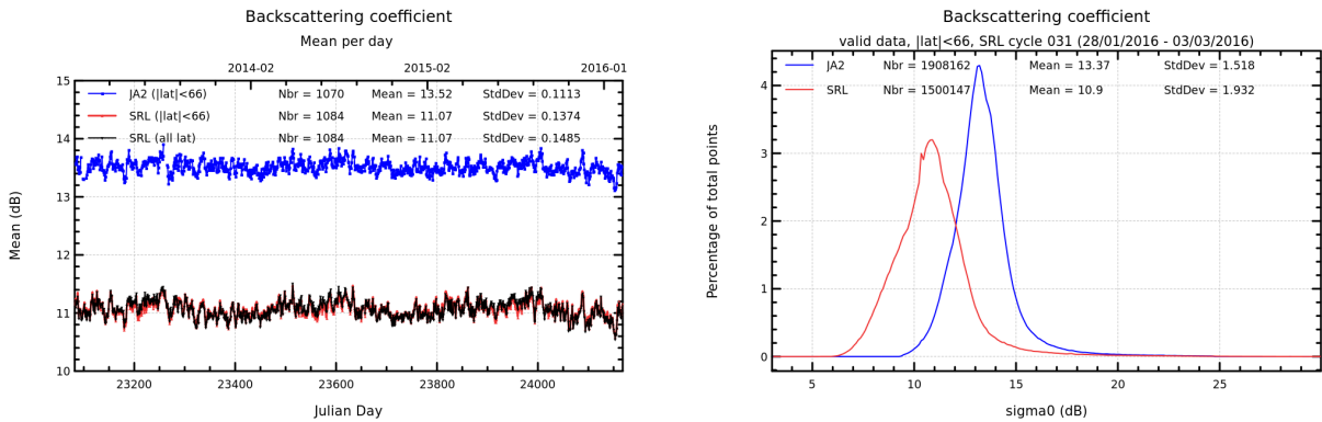
FIGURE 9 – Daily monitoring of backscattering coefficient for Saral/AltiKa and Jason-2 on the left and histogram for cycle 031 on the right (limited to 66° latitude).
