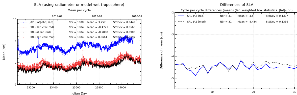
FIGURE 19 – Daily monitoring of mean SLA for Saral/AltiKa and Jason-2 (left) and cycle per cycle monitoring of differences of (Saral/AltiKa – Jason-2) mean SLA (right).
