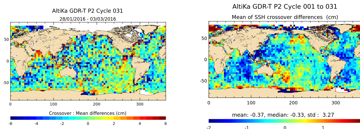
FIGURE 15 – Mean SSH at crossovers for cycle 031 (left) and over the whole Saral/AltiKa period (right).
