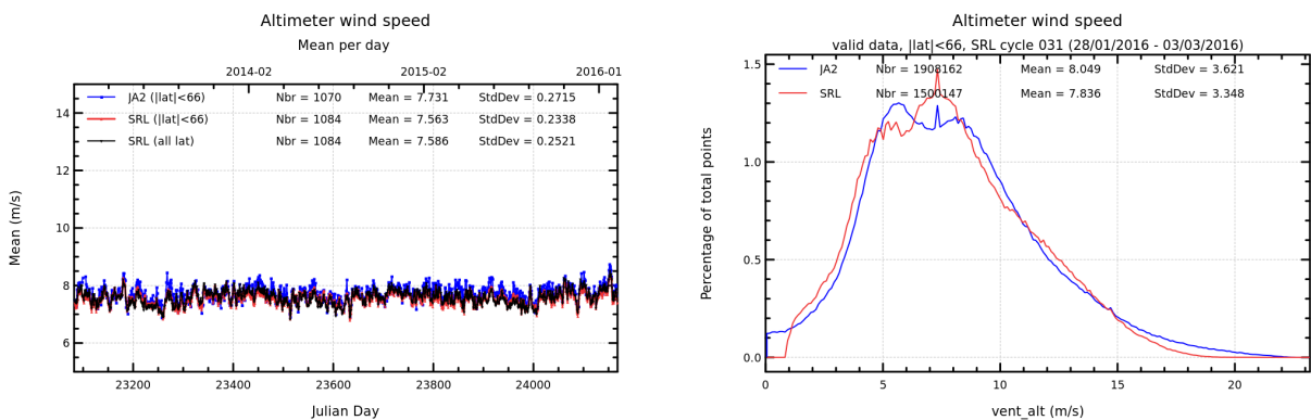
FIGURE 12 – Daily monitoring of altimeter wind speed for Saral/AltiKa and Jason-2 on the left and histogram for cycle 031 on the right (limited to 66° latitude).
