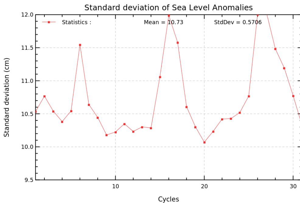
FIGURE 23 – Cyclic monitoring of standard deviation of along track SLA for Saral/AltiKa and Jason-2 (respectively 35 day and almost 10 day cycles).
