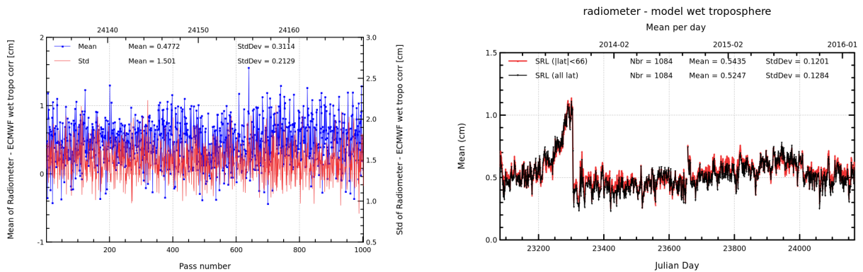
FIGURE 13 – Pass monitoring of wet troposphere differences between radiometer and ECMWF model for Saral/AltiKa cycle 031 (left) and daily monitoring of wet troposphere differences between radiometer and ECMWF model (right).
