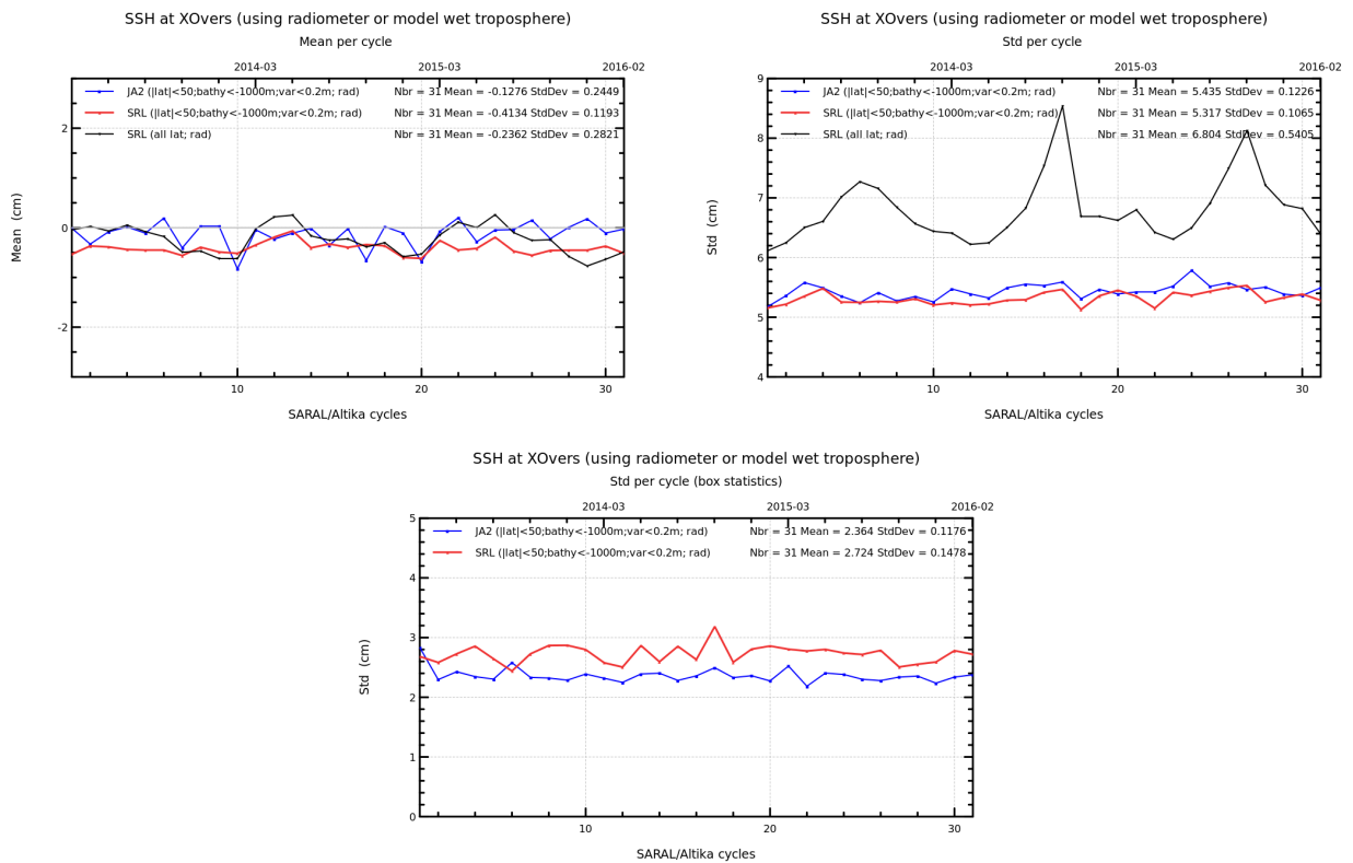
FIGURE 16 – Cyclic monitoring of mean (left) and standard deviation (right) of SSH differences at crossovers for Saral/AltiKa and Jason-2. Standard deviation of SSH differences at crossover using box averages.
