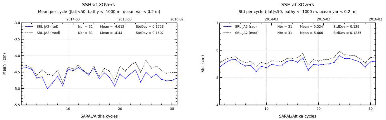
FIGURE 17 – Cyclic monitoring of mean (left) and standard deviation (right) of (Saral/AltiKa – Jason-2) SSH differences at crossovers using geographical selections.
