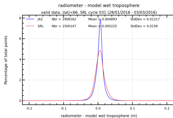
FIGURE 14 – Histogram of wet troposphere differences between radiometer and ECMWF model for cycle 031.
