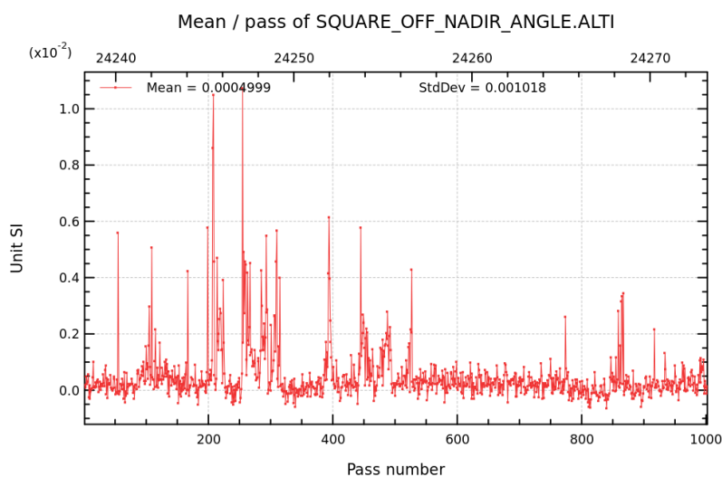
Figure 3: Mispointing cycle 34.
