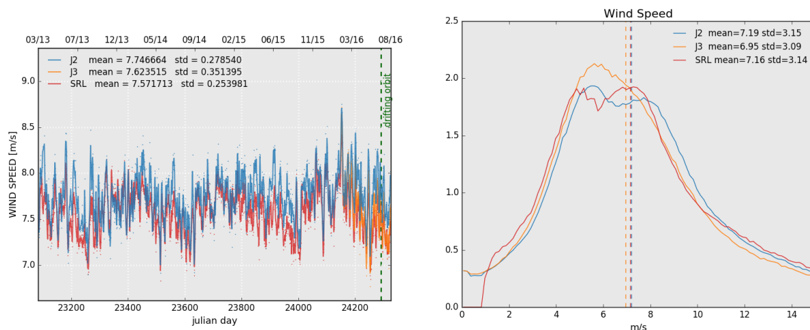
Figure 10: Daily monitoring of altimeter wind speed for Saral/AltiKa, Jason-2 and Jason-3 on the left and histogram for cycle 100 on the right (limited to 66° latitude).
