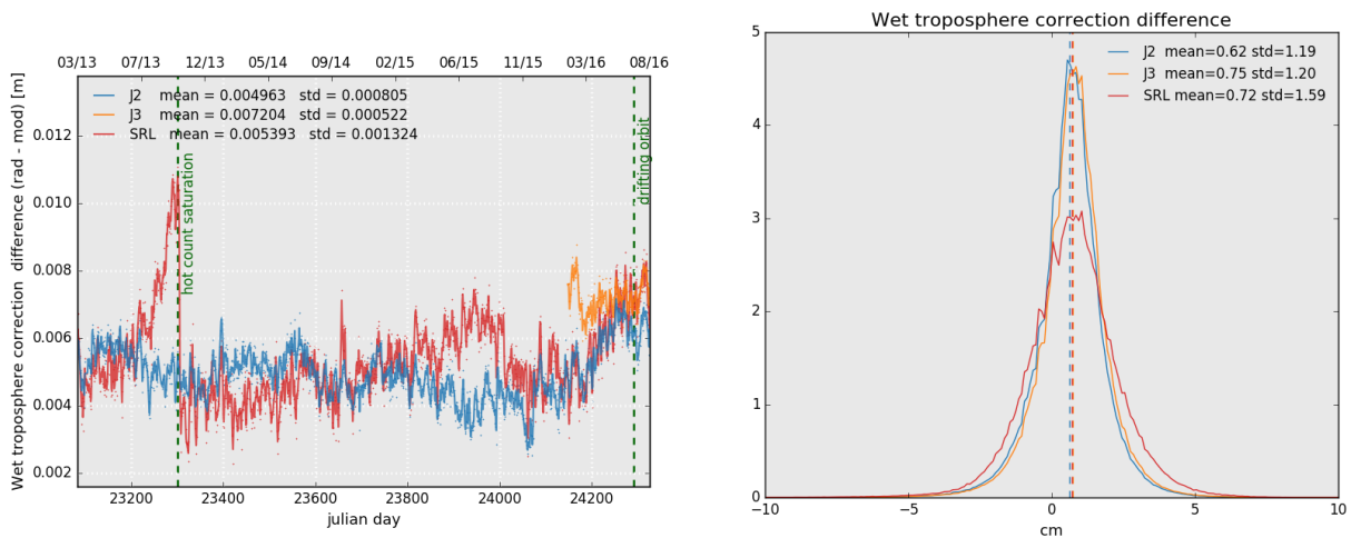
Figure 12: Daily monitoring of wet troposphere differences (Radiometer-ECMWF model) for Saral/AltiKa Jason-2 and Jason-3 (left) and histogram on the right (limited to 66° latitude) for cycle 100 .
