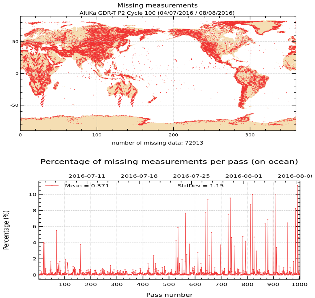
Figure 1: Map of missing measurements for cycle 100 on top. Monitoring of percentage of missing ocean measurements per pass on bottom.
