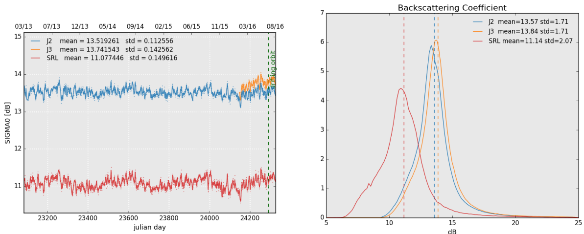
Figure 7: Daily monitoring of backscattering coefficient for Saral/AltiKa, Jason-2 and Jason-3 on the left and histogram for cycle 100 on the right (limited to 66° latitude).
