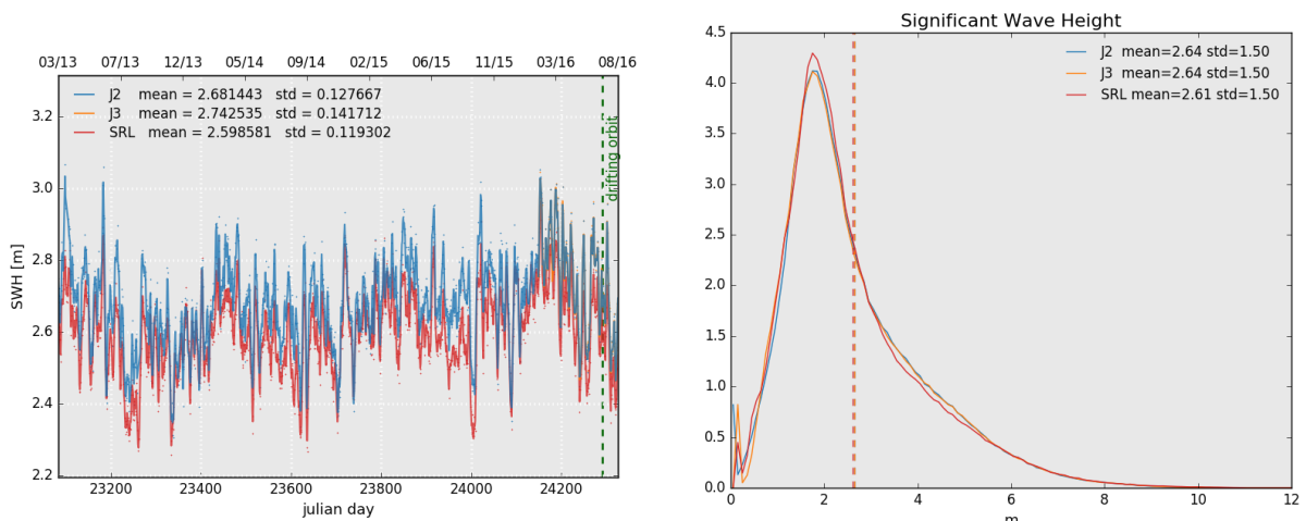
Figure 6: Daily monitoring of significant wave height for AltiKa (Ka-band) Jason-2 and Jason-3 (Ku-band) on the left and histogram for cycle 100 on the right (limited to 66^\circ latitude).
