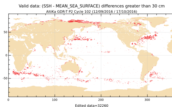
Figure 20: SLA higher than 30 cm for cycle 102.
