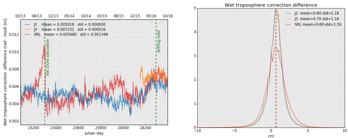
Figure 12: Daily monitoring of wet troposphere differences (Radiometer-ECMWF model) for Saral/AltiKa Jason-2 and Jason-3 (left) and histogram on the right (limited to 66° latitude) for cycle 102 .
