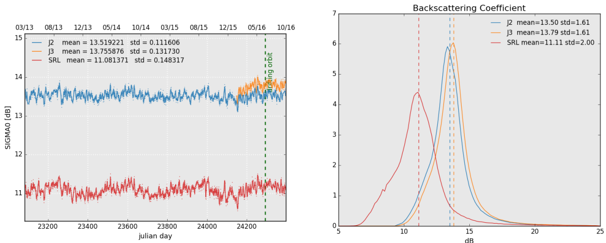
Figure 7: Daily monitoring of backscattering coefficient for Saral/AltiKa, Jason-2 and Jason-3 on the left and histogram for cycle 102 on the right (limited to 66° latitude).
