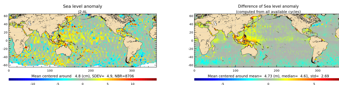
Figure 21: Jason-2 – Saral/AltiKa SLA differences for cycle 102 (left) and averaged over the whole Saral/AltiKa period (right).
