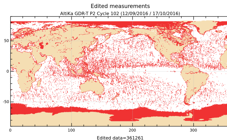
Figure 2: Edited measurements for cycle 102.
