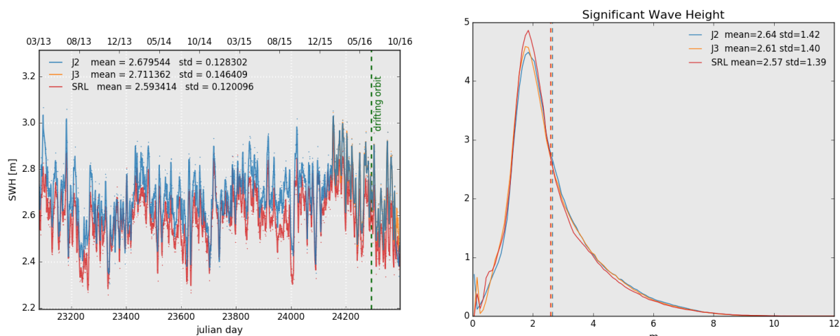
Figure 6: Daily monitoring of significant wave height for AltiKa (Ka-band) Jason-2 and Jason-3 (Ku-band) on the left and histogram for cycle 102 on the right (limited to 66^\circ latitude).
