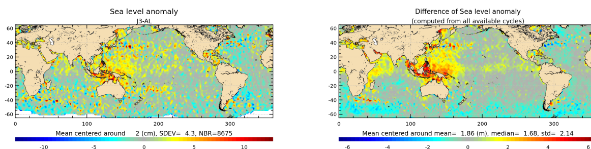
Figure 22: Jason-3 – Saral/AltiKa SLA differences for cycle 102 (left) and averaged over the whole Saral/AltiKa period (right).
