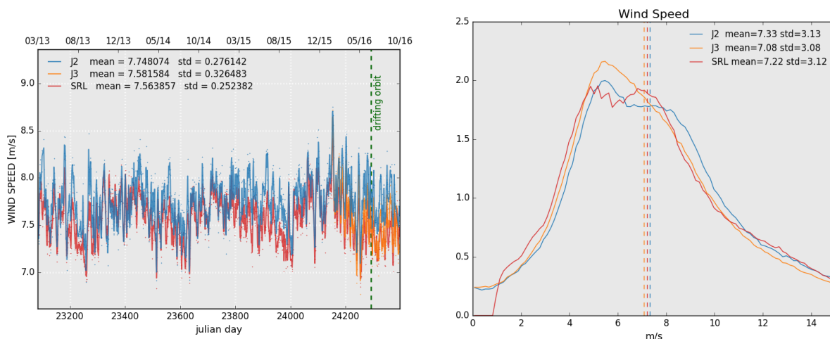
Figure 10: Daily monitoring of altimeter wind speed for Saral/AltiKa, Jason-2 and Jason-3 on the left and histogram for cycle 102 on the right (limited to 66° latitude).
