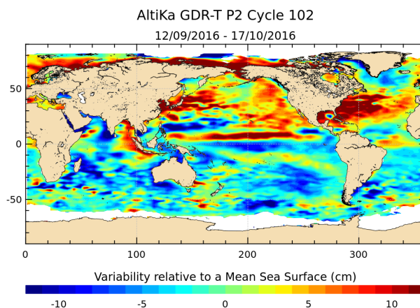
Figure 19: Sea level anomaly relative to MSS for cycle 102.
