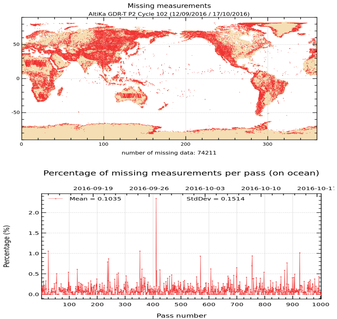
Figure 1: Map of missing measurements for cycle 102 on top. Monitoring of percentage of missing ocean measurements per pass on bottom.
