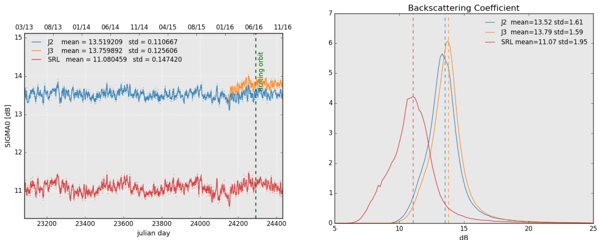
Figure 7: Daily monitoring of backscattering coefficient for Saral/AltiKa, Jason-2 and Jason-3 on the left and histogram for cycle 103 on the right (limited to 66° latitude).
