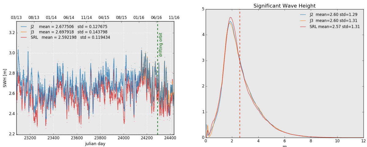
Figure 6: Daily monitoring of significant wave height for AltiKa (Ka-band) Jason-2 and Jason-3 (Ku-band) on the left and histogram for cycle 103 on the right (limited to 66^\circ latitude).
