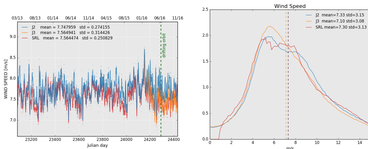
Figure 10: Daily monitoring of altimeter wind speed for Saral/AltiKa, Jason-2 and Jason-3 on the left and histogram for cycle 103 on the right (limited to 66° latitude).
