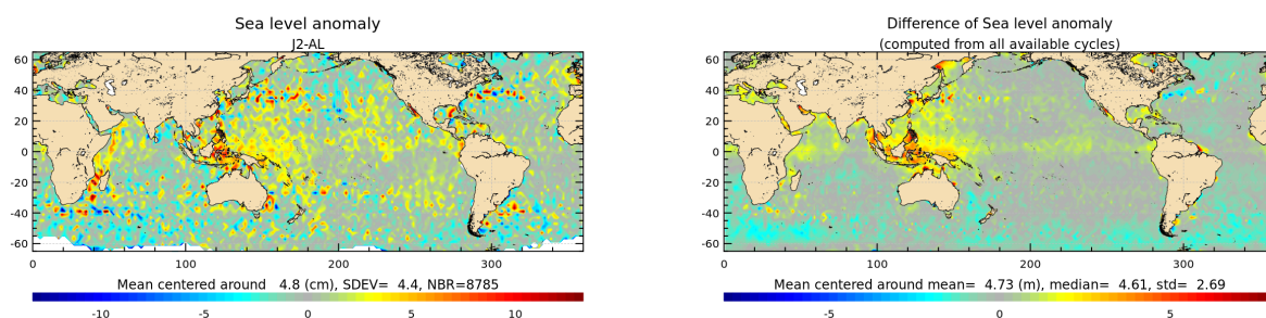
Figure 21: Jason-2 – Saral/AltiKa SLA differences for cycle 103 (left) and averaged over the whole Saral/AltiKa period (right).
