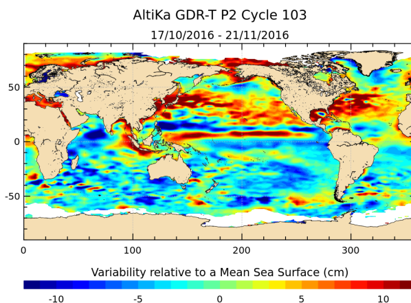
Figure 19: Sea level anomaly relative to MSS for cycle 103.
