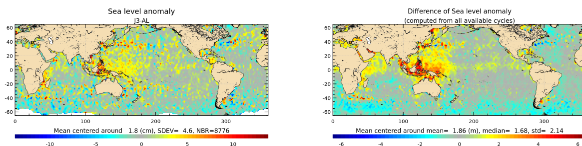
Figure 22: Jason-3 – Saral/AltiKa SLA differences for cycle 103 (left) and averaged over the whole Saral/AltiKa period (right).
