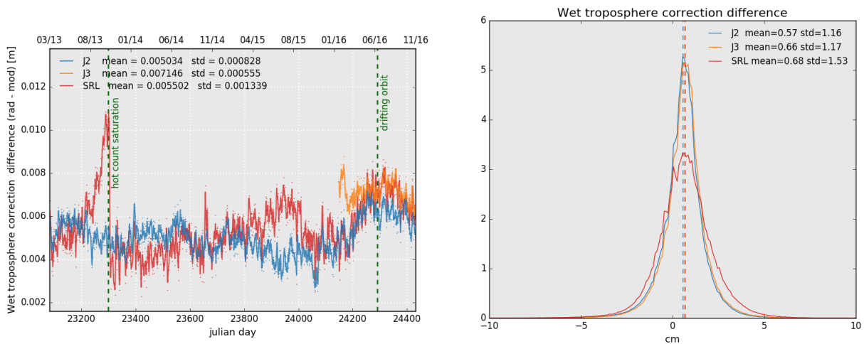
Figure 12: Daily monitoring of wet troposphere differences (Radiometer-ECMWF model) for Saral/AltiKa Jason-2 and Jason-3 (left) and histogram on the right (limited to 66° latitude) for cycle 103 .
