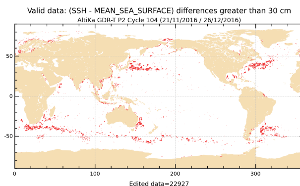
Figure 20: SLA higher than 30 cm for cycle 104.
