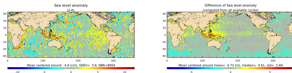
Figure 21: Jason-2 – Saral/AltiKa SLA differences for cycle 104 (left) and averaged over the whole Saral/AltiKa period (right).
