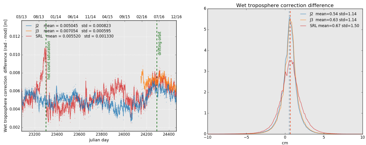
Figure 12: Daily monitoring of wet troposphere differences (Radiometer-ECMWF model) for Saral/AltiKa Jason-2 and Jason-3 (left) and histogram on the right (limited to 66° latitude) for cycle 104 .
