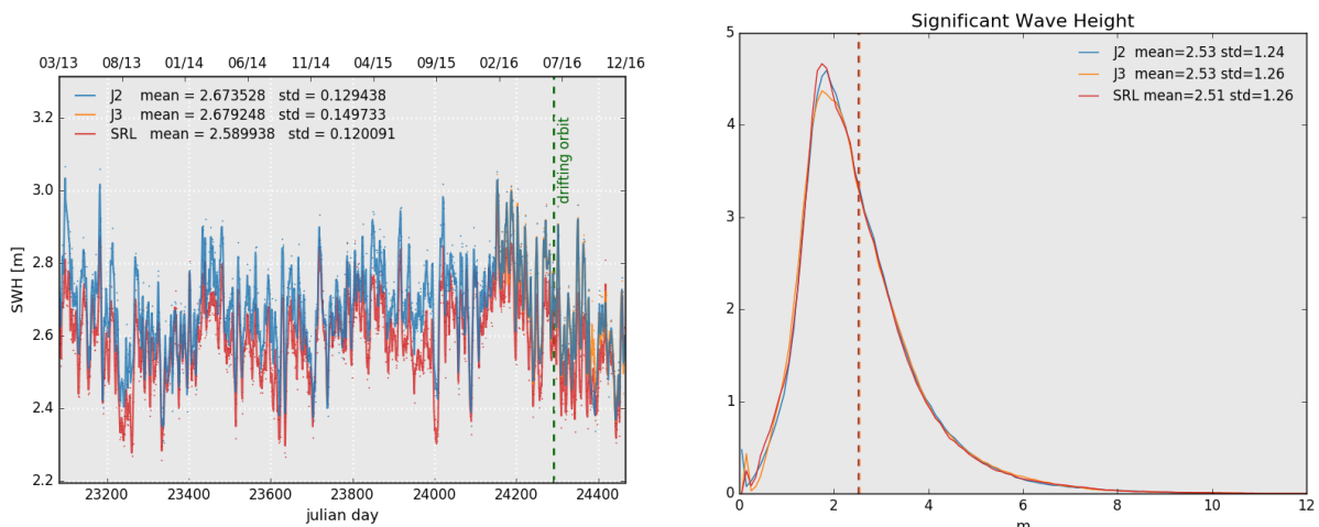
Figure 6: Daily monitoring of significant wave height for AltiKa (Ka-band) Jason-2 and Jason-3 (Ku-band) on the left and histogram for cycle 104 on the right (limited to 66^\circ latitude).
