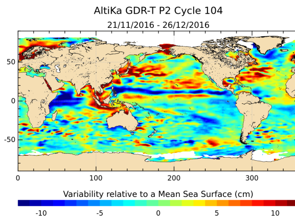
Figure 19: Sea level anomaly relative to MSS for cycle 104.
