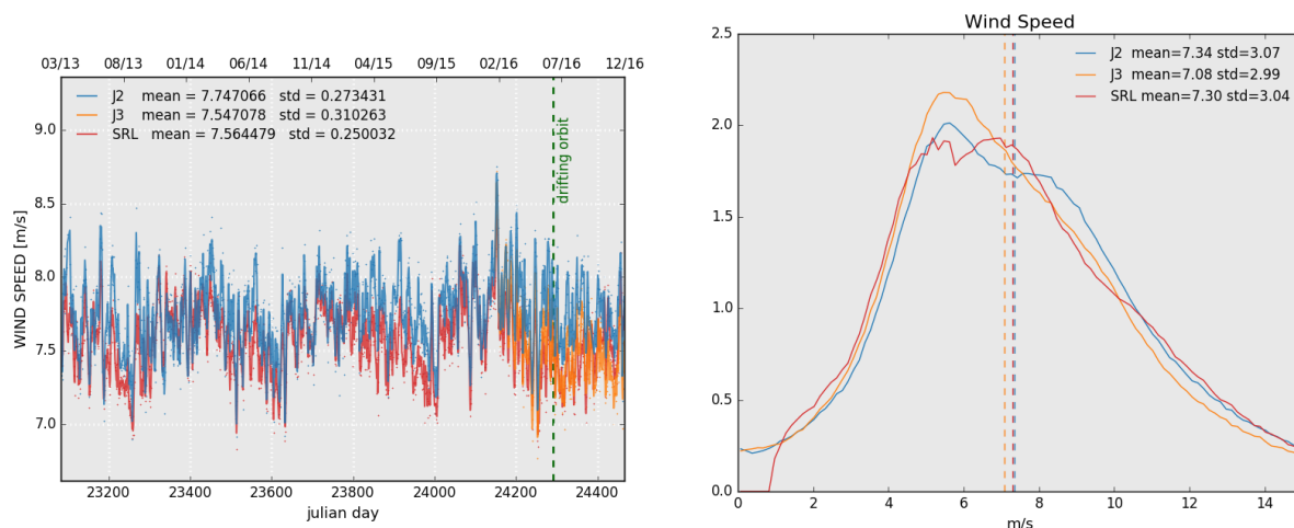
Figure 10: Daily monitoring of altimeter wind speed for Saral/AltiKa, Jason-2 and Jason-3 on the left and histogram for cycle 104 on the right (limited to 66° latitude).
