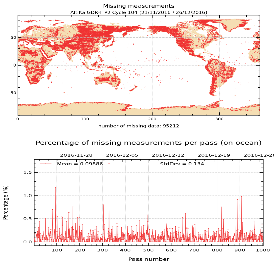
Figure 1: Map of missing measurements for cycle 104 on top. Monitoring of percentage of missing ocean measurements per pass on bottom.
