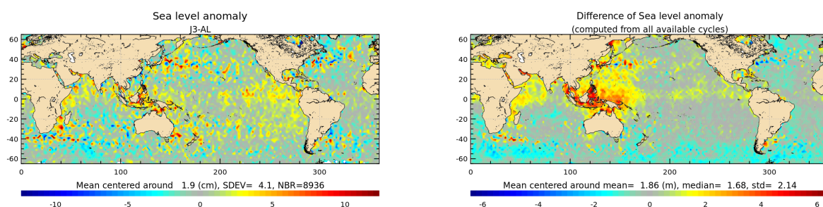
Figure 22: Jason-3 – Saral/AltiKa SLA differences for cycle 104 (left) and averaged over the whole Saral/AltiKa period (right).
