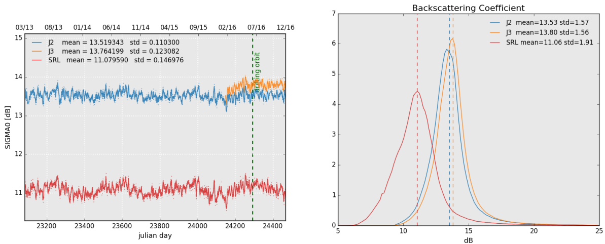
Figure 7: Daily monitoring of backscattering coefficient for Saral/AltiKa, Jason-2 and Jason-3 on the left and histogram for cycle 104 on the right (limited to 66° latitude).
