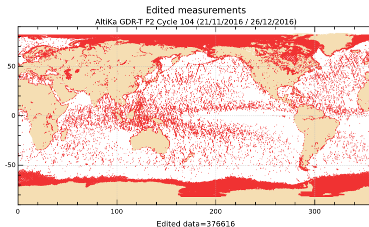
Figure 2: Edited measurements for cycle 104.
