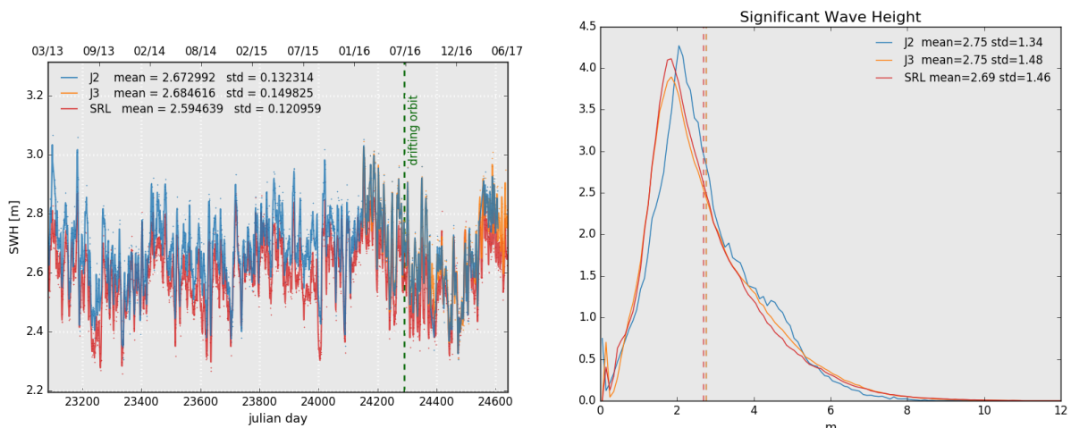
Figure 6: Daily monitoring of significant wave height for AltiKa (Ka-band) Jason-2 and Jason-3 (Ku-band) on the left and histogram for cycle 109 on the right (limited to 66^\circ latitude).
