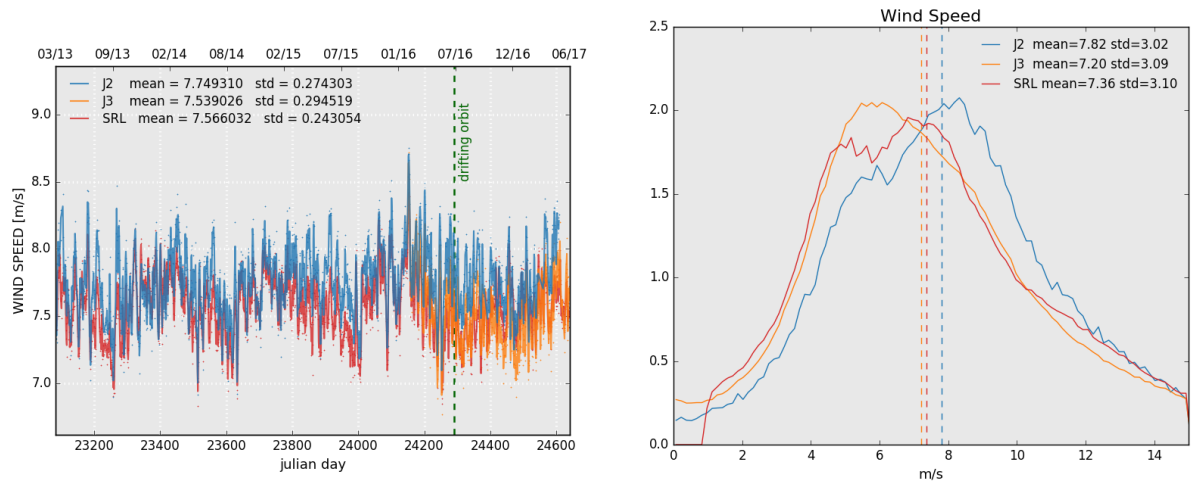
Figure 10: Daily monitoring of altimeter wind speed for Saral/AltiKa, Jason-2 and Jason-3 on the left and histogram for cycle 109 on the right (limited to 66° latitude).
