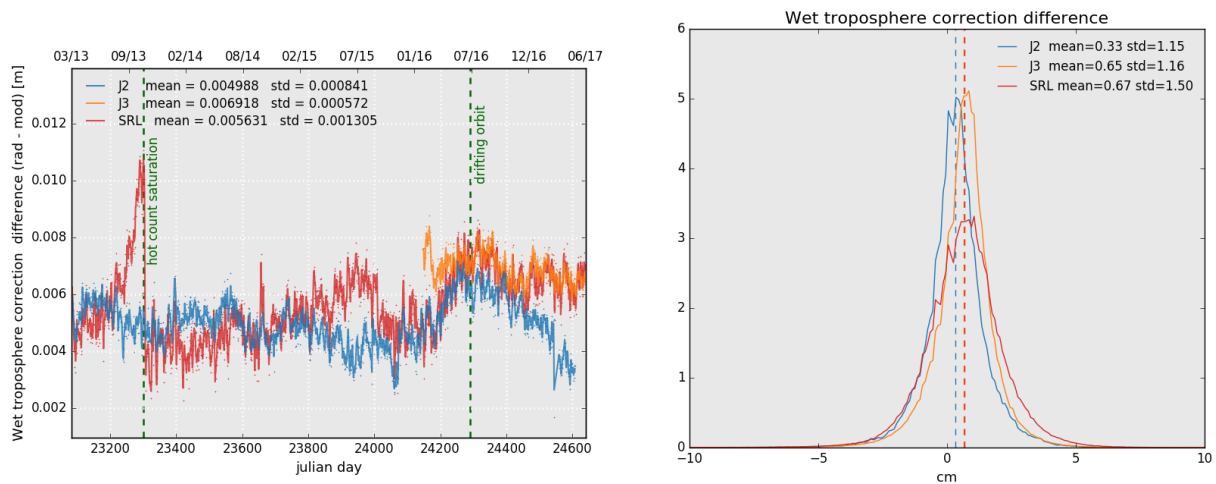
Figure 12: Daily monitoring of wet troposphere differences (Radiometer-ECMWF model) for Saral/AltiKa Jason-2 and Jason-3 (left) and histogram on the right (limited to 66° latitude) for cycle 109 .
