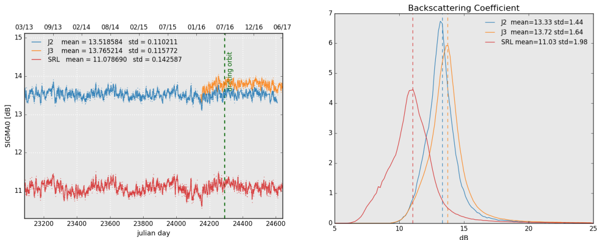
Figure 7: Daily monitoring of backscattering coefficient for Saral/AltiKa, Jason-2 and Jason-3 on the left and histogram for cycle 109 on the right (limited to 66° latitude).
