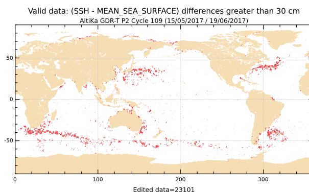
Figure 20: SLA higher than 30 cm for cycle 109.
