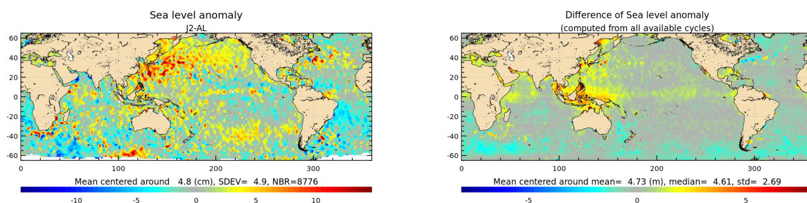
Figure 21: Jason-2 – Saral/AltiKa SLA differences for cycle 110 (left) and averaged over the whole Saral/AltiKa period (right).
