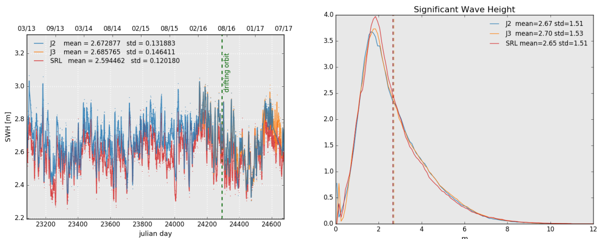
Figure 6: Daily monitoring of significant wave height for AltiKa (Ka-band) Jason-2 and Jason-3 (Ku-band) on the left and histogram for cycle 110 on the right (limited to 66^\circ latitude).
