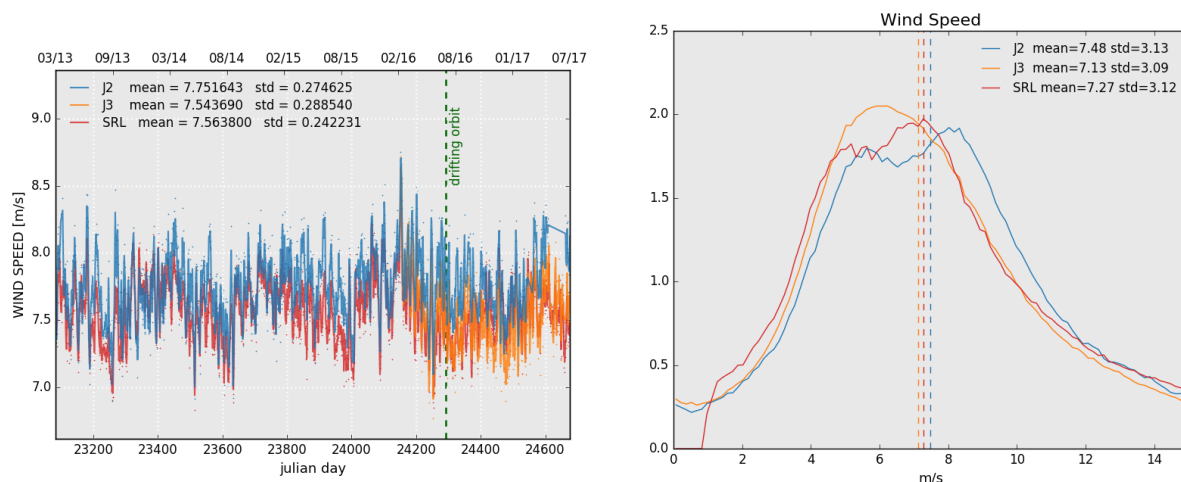
Figure 10: Daily monitoring of altimeter wind speed for Saral/AltiKa, Jason-2 and Jason-3 on the left and histogram for cycle 110 on the right (limited to 66° latitude).
