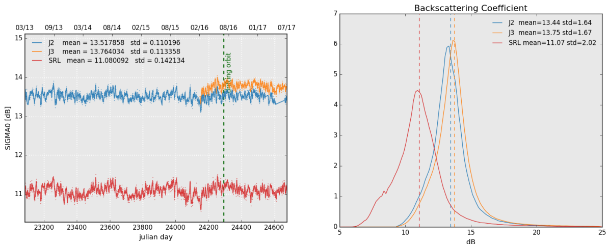
Figure 7: Daily monitoring of backscattering coefficient for Saral/AltiKa, Jason-2 and Jason-3 on the left and histogram for cycle 110 on the right (limited to 66° latitude).
