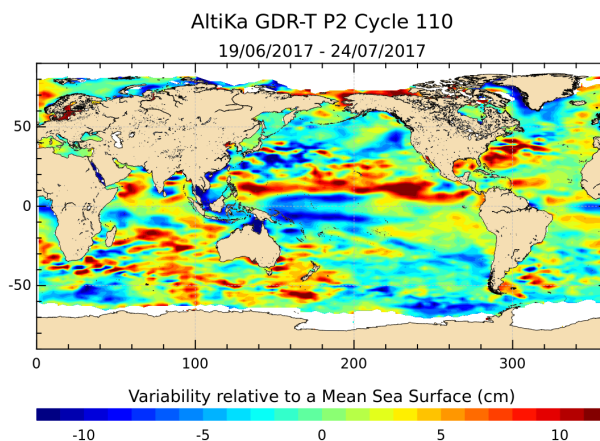
Figure 19: Sea level anomaly relative to MSS for cycle 110.
