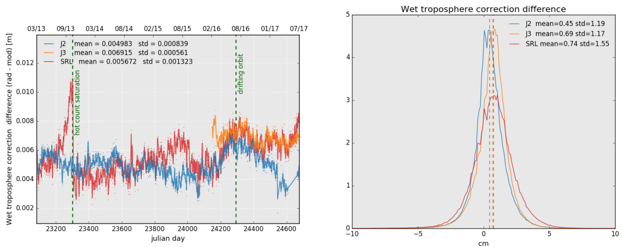
Figure 12: Daily monitoring of wet troposphere differences (Radiometer-ECMWF model) for Saral/AltiKa Jason-2 and Jason-3 (left) and histogram on the right (limited to 66° latitude) for cycle 110 .
