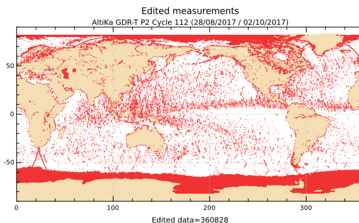
Figure 2: Edited measurements for cycle 112.
