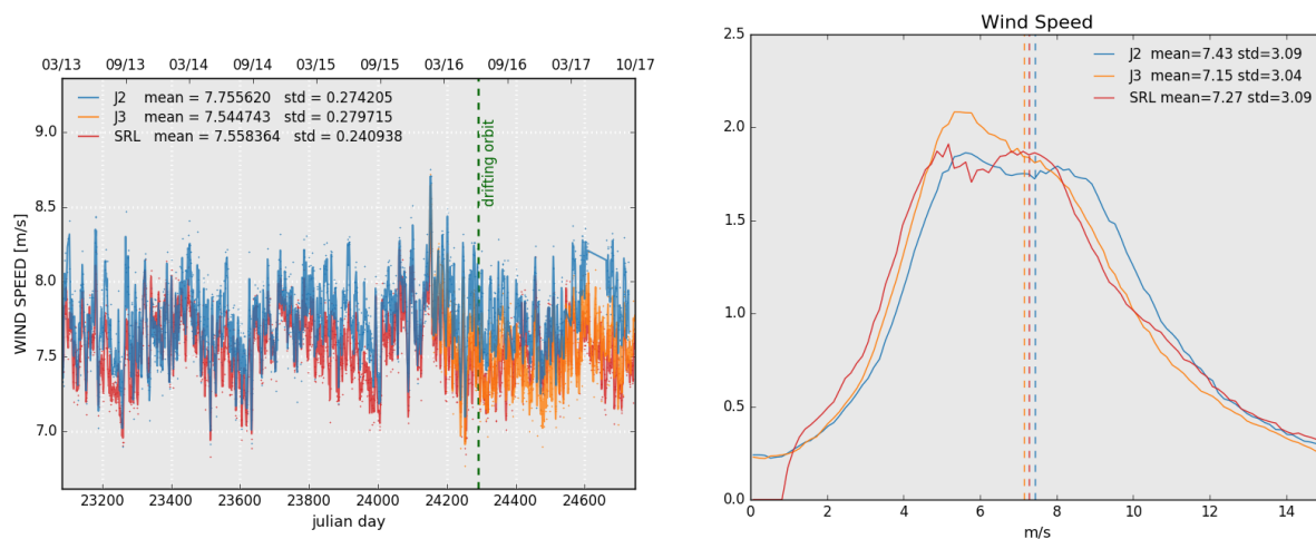
Figure 11: Daily monitoring of altimeter wind speed for Saral/AltiKa, Jason-2 and Jason-3 on the left and histogram for cycle 112 on the right (limited to 66° latitude).
