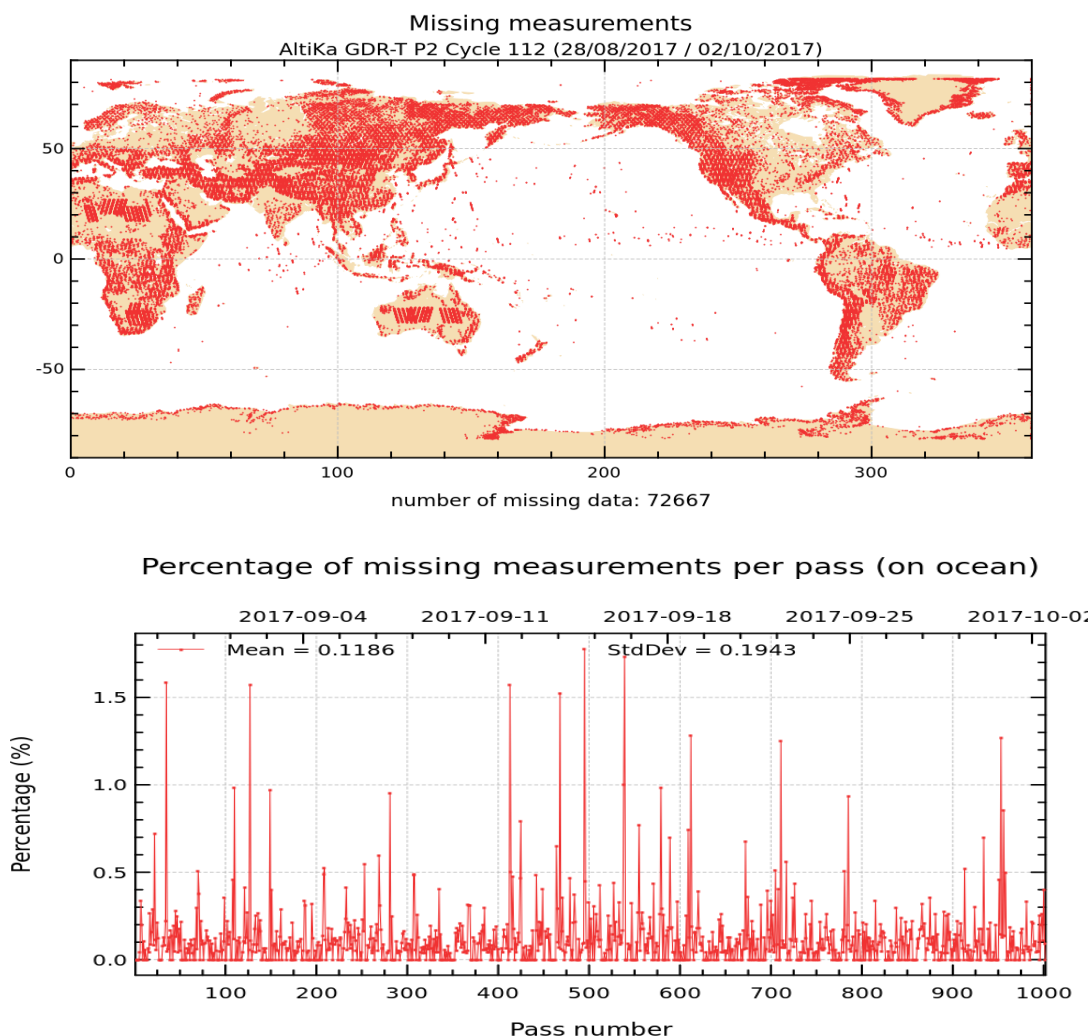
Figure 1: Map of missing measurements for cycle 112 on top. Monitoring of percentage of missing ocean measurements per pass on bottom.
