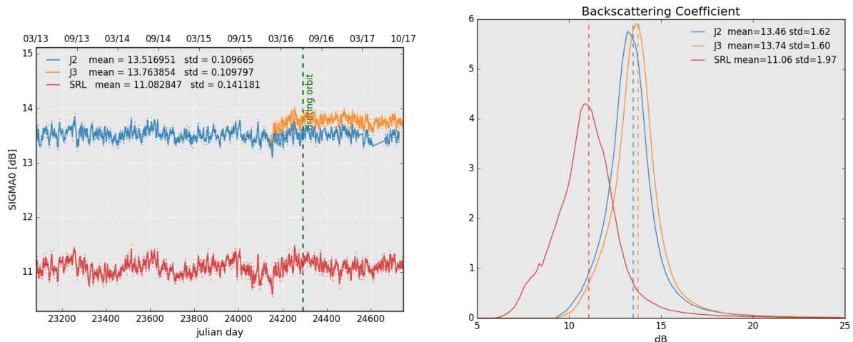
Figure 8: Daily monitoring of backscattering coefficient for Saral/AltiKa, Jason-2 and Jason-3 on the left and histogram for cycle 112 on the right (limited to 66° latitude).
