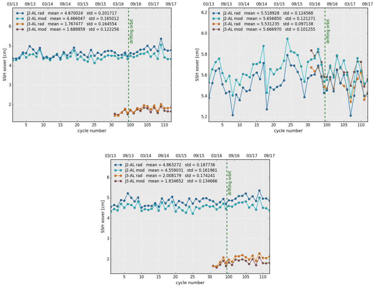
Figure 17: Cyclic monitoring of mean (left) and standard deviation (right) of Jason-2 / AltiKa Jason-3 / AltiKa SSH differences at crossovers using geographical selections. Box-averaged differences (bottom).
