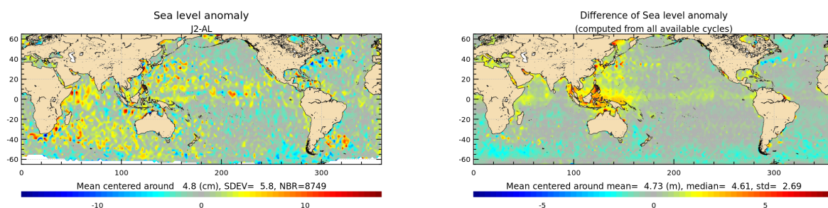
Figure 22: Jason-2 – Saral/AltiKa SLA differences for cycle 112 (left) and averaged over the whole Saral/AltiKa period (right).
