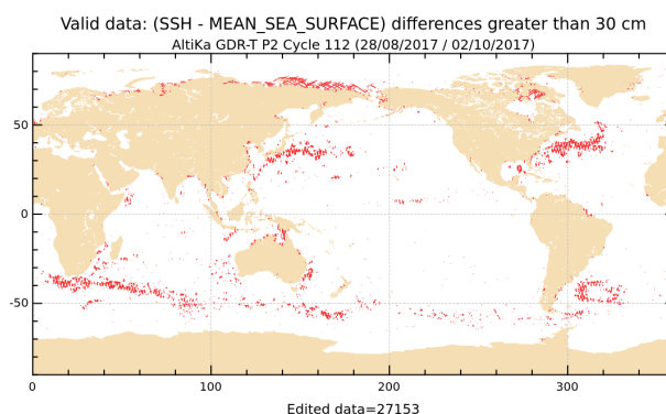
Figure 21: SLA higher than 30 cm for cycle 112.
