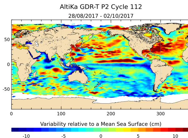
Figure 20: Sea level anomaly relative to MSS for cycle 112.
