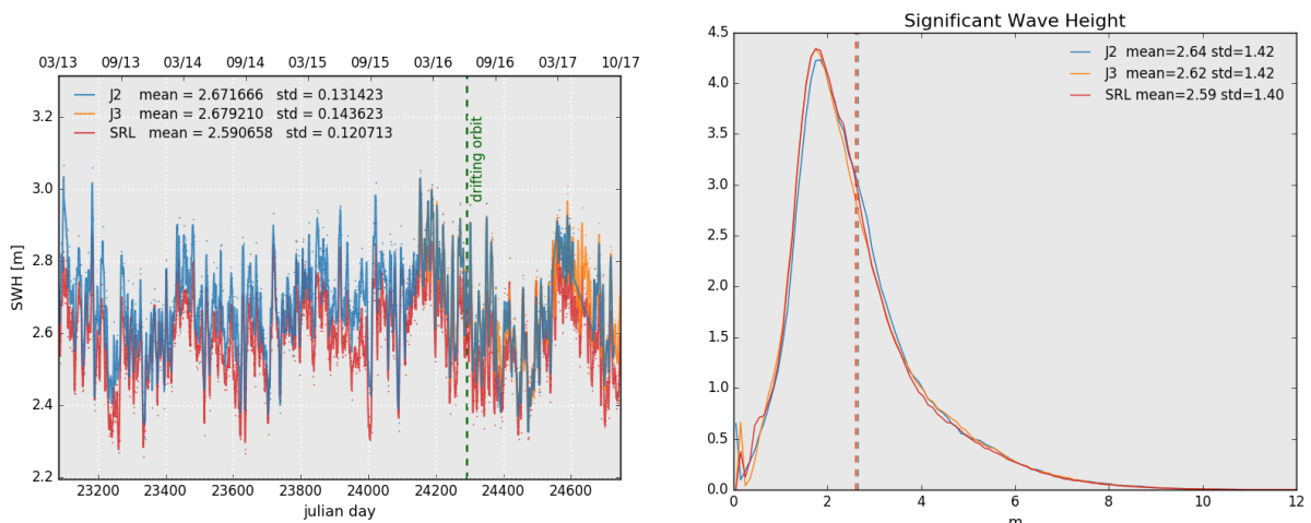
Figure 7: Daily monitoring of significant wave height for AltiKa (Ka-band) Jason-2 and Jason-3 (Ku-band) on the left and histogram for cycle 112 on the right (limited to 66^\circ latitude).
