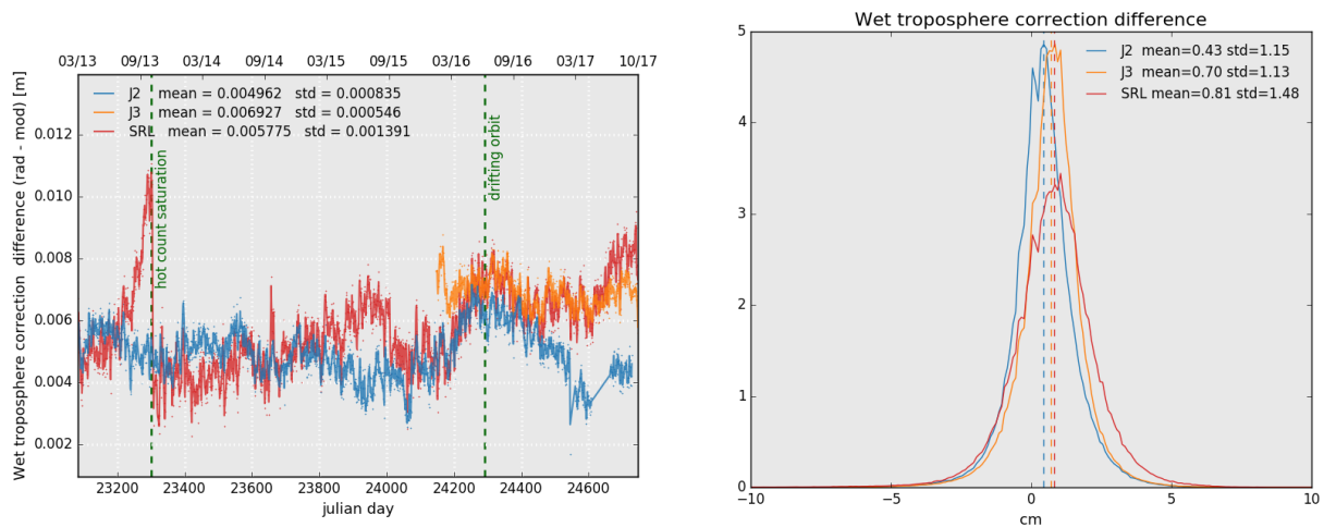
Figure 13: Daily monitoring of wet troposphere differences (Radiometer-ECMWF model) for Saral/AltiKa Jason-2 and Jason-3 (left) and histogram on the right (limited to 66° latitude) for cycle 112 .
