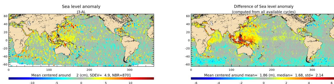
Figure 23: Jason-3 – Saral/AltiKa SLA differences for cycle 112 (left) and averaged over the whole Saral/AltiKa period (right).
