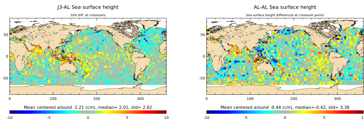
Figure 15: Mean of multi-mission SSH and mono-mission SSH differences at crossovers for cycle 117.
