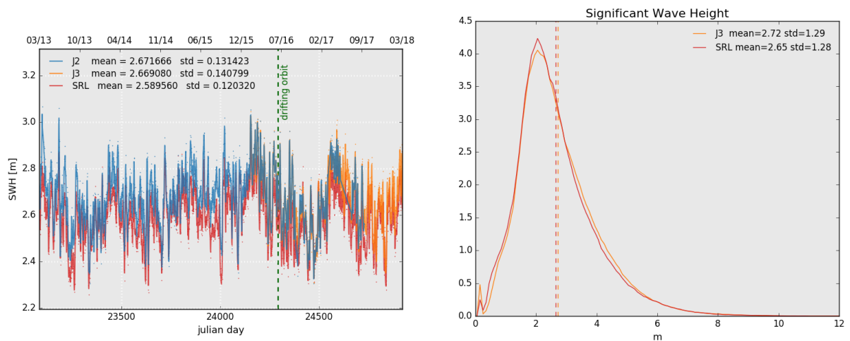
Figure 7: Daily monitoring of significant wave height for AltiKa (Ka-band) Jason-2 and Jason-3 (Ku-band) on the left and histogram for cycle 117 on the right (limited to 66° latitude).
