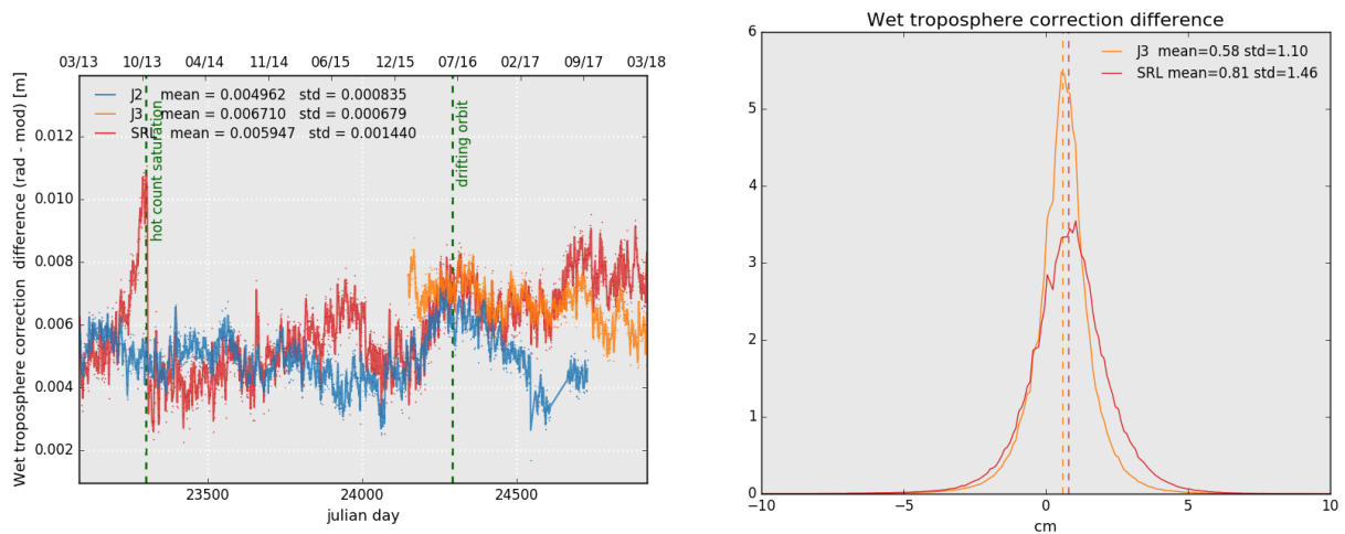
Figure 13: Daily monitoring of wet troposphere differences (Radiometer-ECMWF model) for Saral/AltiKa Jason-2 and Jason-3 (left) and histogram on the right (limited to 66° latitude) for cycle 117 .
