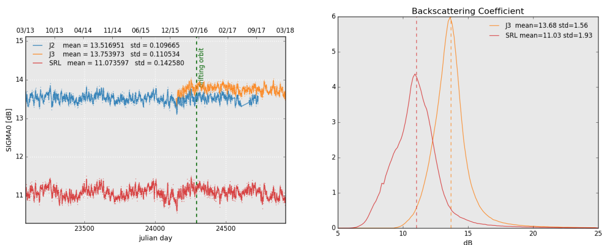
Figure 8: Daily monitoring of backscattering coefficient for Saral/AltiKa, Jason-2 and Jason-3 on the left and histogram for cycle 117 on the right (limited to 66° latitude).
