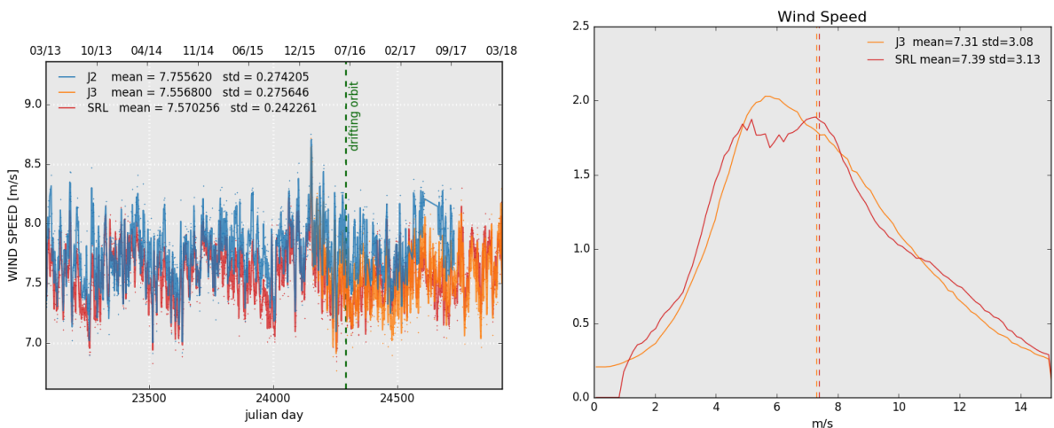
Figure 11: Daily monitoring of altimeter wind speed for Saral/AltiKa, Jason-2 and Jason-3 on the left and histogram for cycle 117 on the right (limited to 66^\circ latitude).
