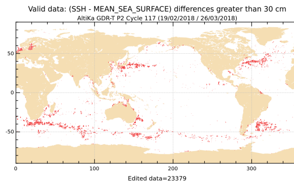
Figure 21: SLA higher than 30 cm for cycle 117.
