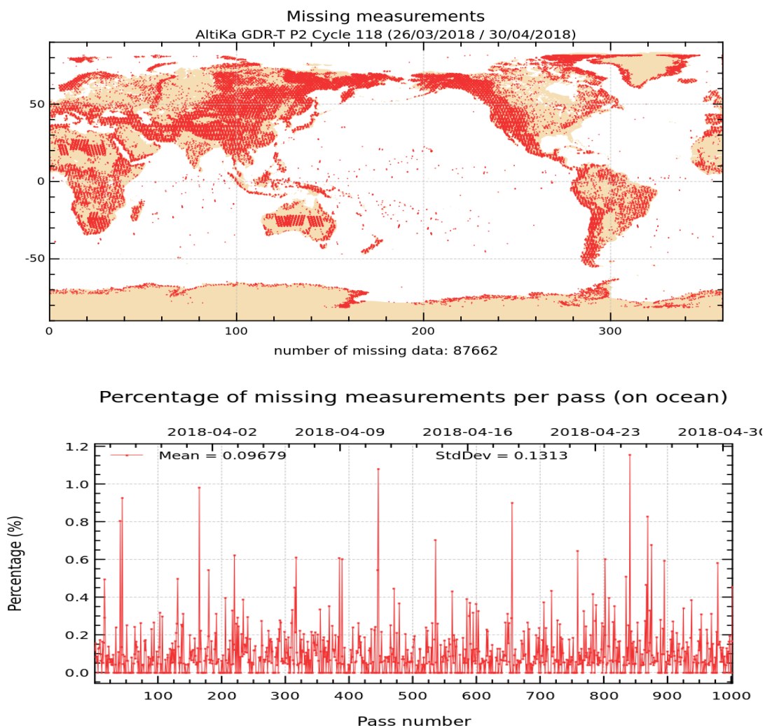
Figure 1: Map of missing measurements for cycle 118 on top. Monitoring of percentage of missing ocean measurements per pass on bottom.
