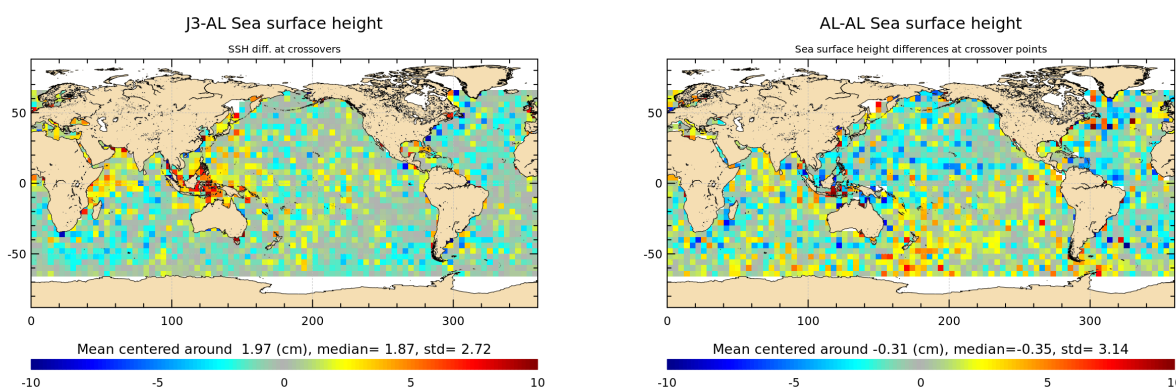
Figure 15: Mean of multi-mission SSH and mono-mission SSH differences at crossovers for cycle 118.
