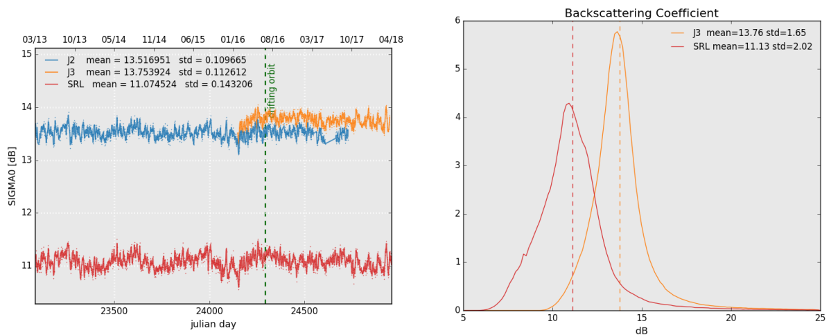
Figure 8: Daily monitoring of backscattering coefficient for Saral/AltiKa, Jason-2 and Jason-3 on the left and histogram for cycle 118 on the right (limited to 66° latitude).
