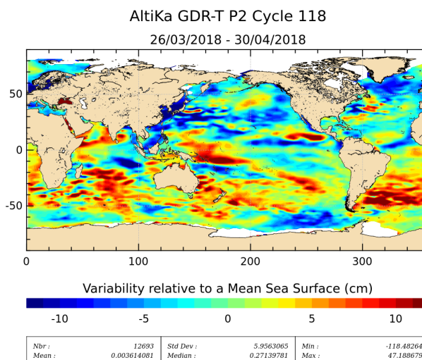
Figure 20: Sea level anomaly relative to MSS for cycle 118.
