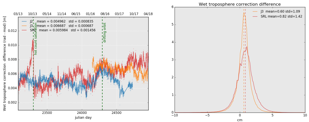
Figure 13: Daily monitoring of wet troposphere differences (Radiometer-ECMWF model) for Saral/AltiKa Jason-2 and Jason-3 (left) and histogram on the right (limited to 66° latitude) for cycle 118 .
