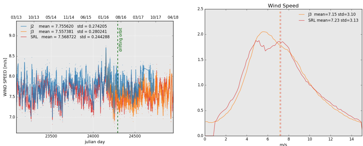
Figure 11: Daily monitoring of altimeter wind speed for Saral/AltiKa, Jason-2 and Jason-3 on the left and histogram for cycle 118 on the right (limited to 66° latitude).
