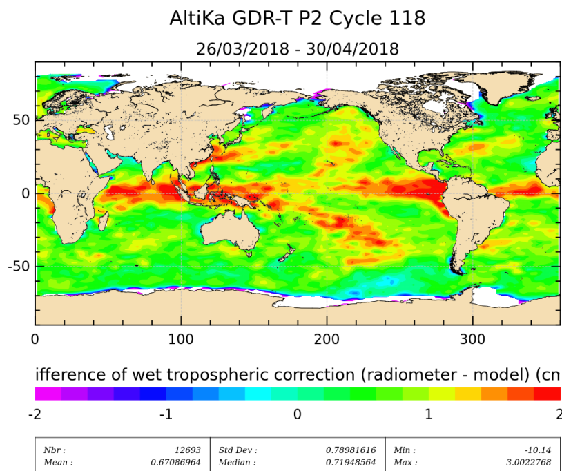
Figure 12: Mean of wet troposphere correction difference (Radiometer-ECMWF model) for cycle 118.
