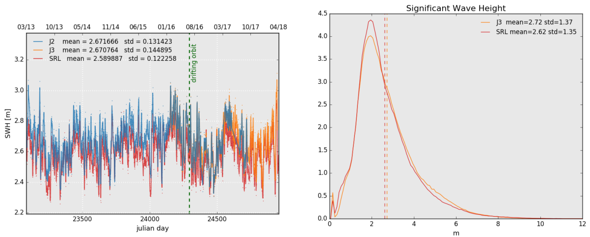
Figure 7: Daily monitoring of significant wave height for AltiKa (Ka-band) Jason-2 and Jason-3 (Ku-band) on the left and histogram for cycle 118 on the right (limited to 66° latitude).
