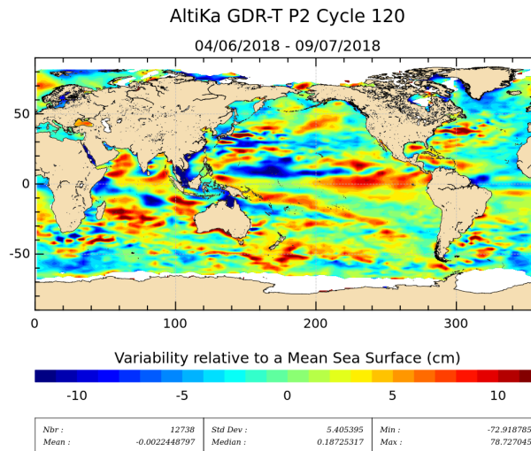
Figure 20: Sea level anomaly relative to MSS for cycle 120.
