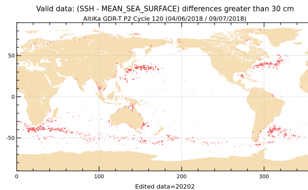
Figure 21: SLA higher than 30 cm for cycle 120.
