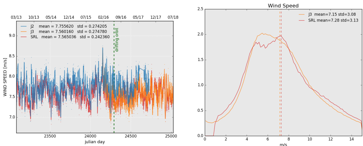
Figure 11: Daily monitoring of altimeter wind speed for Saral/AltiKa, Jason-2 and Jason-3 on the left and histogram for cycle 120 on the right (limited to 66° latitude).
