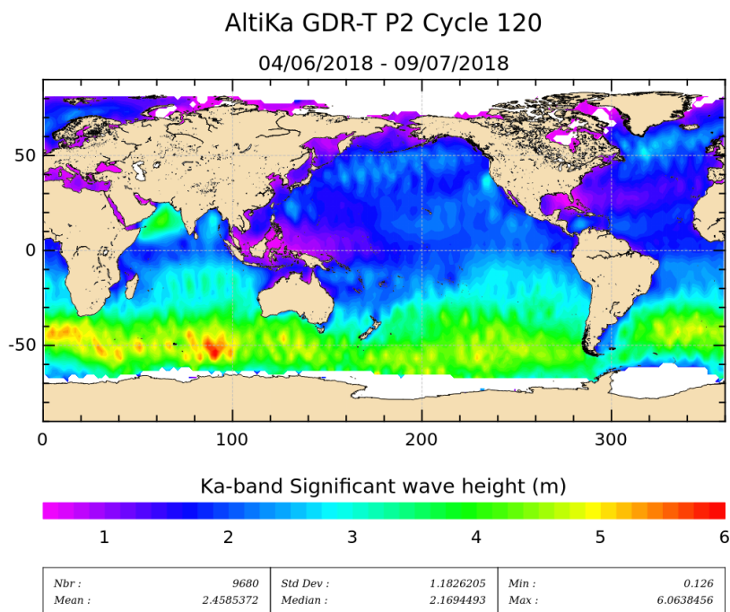
Figure 6: Significant wave height for cycle 120.
