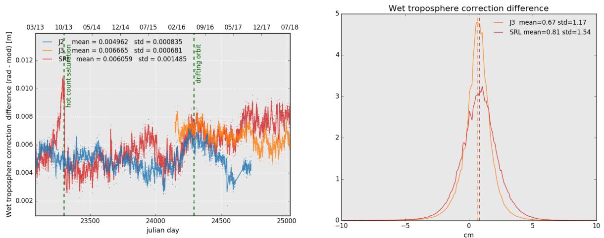
Figure 13: Daily monitoring of wet troposphere differences (Radiometer-ECMWF model) for Saral/AltiKa Jason-2 and Jason-3 (left) and histogram on the right (limited to 66° latitude) for cycle 120 .
