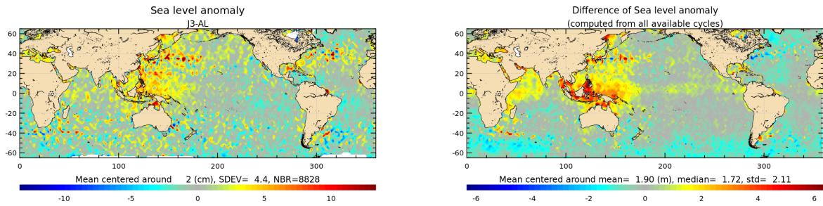
Figure 22: Jason-3 – Saral/AltiKa SLA differences for cycle 120 (left) and averaged over the whole Saral/AltiKa period (right).
