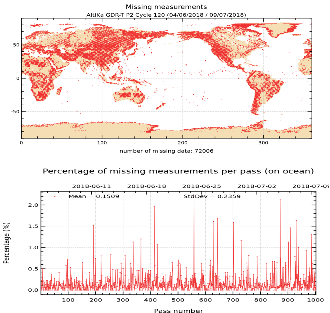
Figure 1: Map of missing measurements for cycle 120 on top. Monitoring of percentage of missing ocean measurements per pass on bottom.
