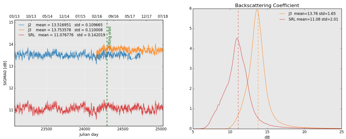
Figure 8: Daily monitoring of backscattering coefficient for Saral/AltiKa, Jason-2 and Jason-3 on the left and histogram for cycle 120 on the right (limited to 66° latitude).
