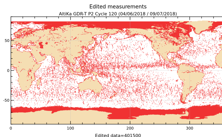
Figure 2: Edited measurements for cycle 120.
