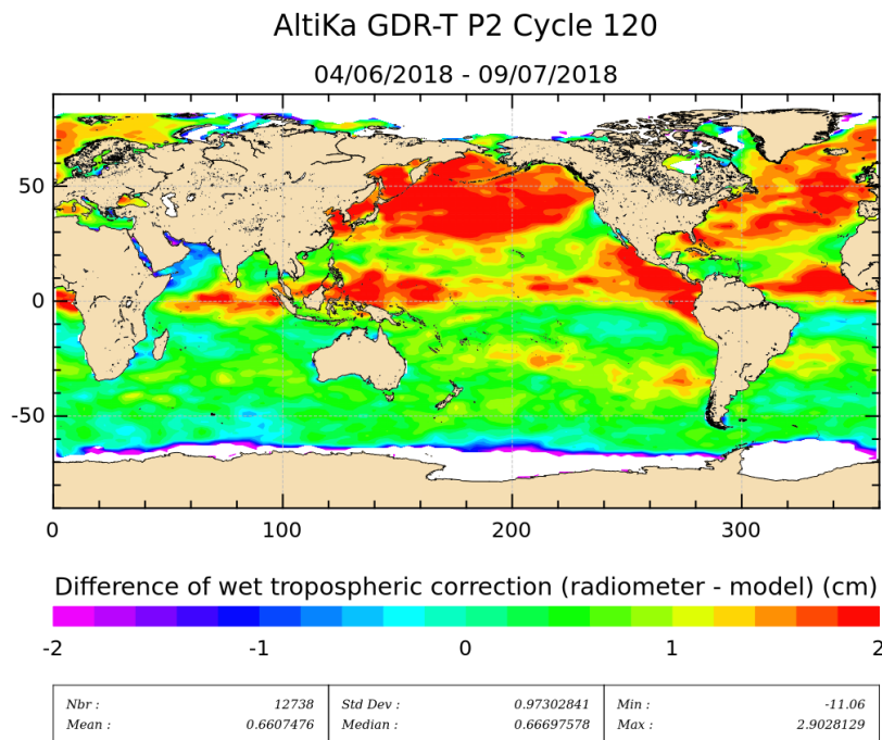
Figure 12: Mean of wet troposphere correction difference (Radiometer-ECMWF model) for cycle 120.
