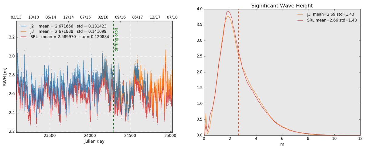
Figure 7: Daily monitoring of significant wave height for AltiKa (Ka-band) Jason-2 and Jason-3 (Ku-band) on the left and histogram for cycle 120 on the right (limited to 66° latitude).
