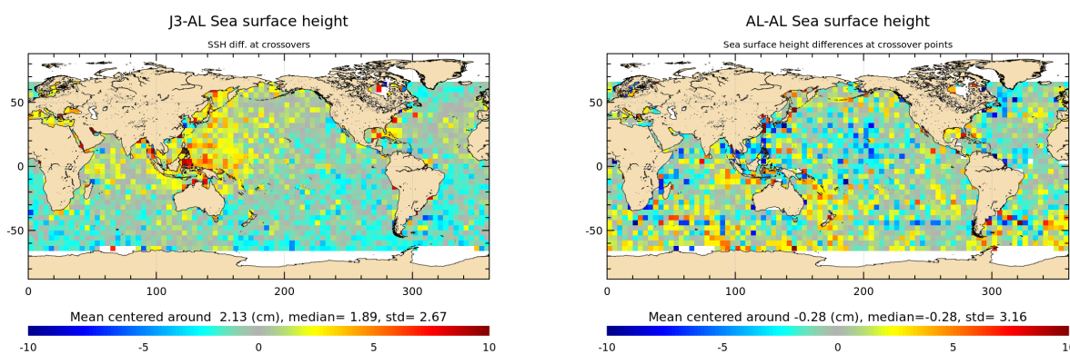
Figure 15: Mean of multi-mission SSH and mono-mission SSH differences at crossovers for cycle 120.
