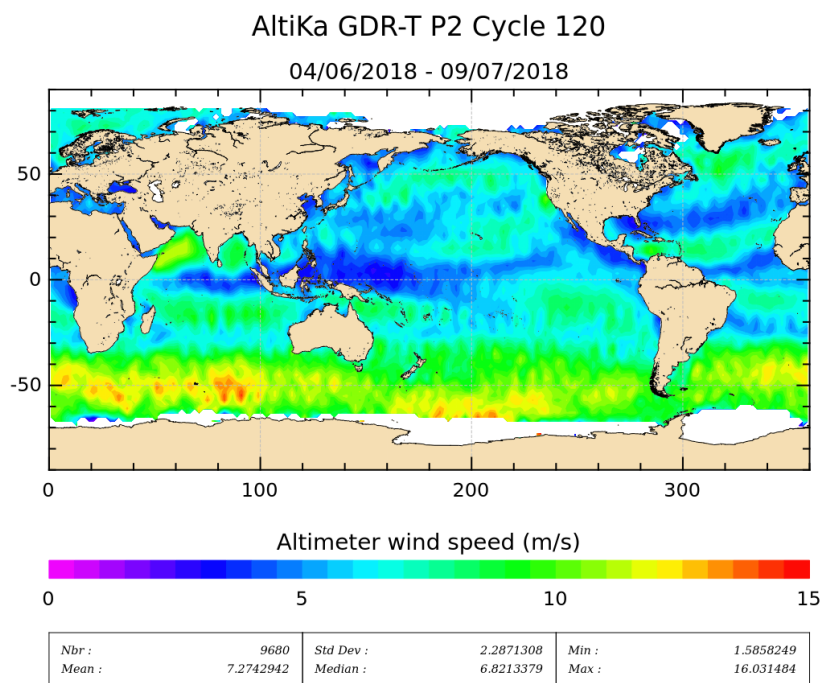
Figure 10: Altimeter wind speed for cycle 120.
