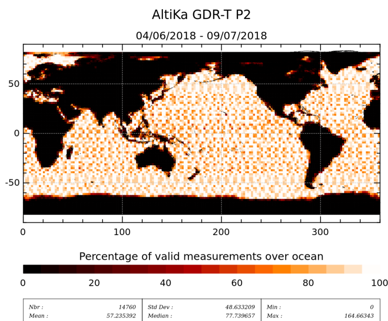
Figure 3: Percentage of valid measurements for cycle 120.
