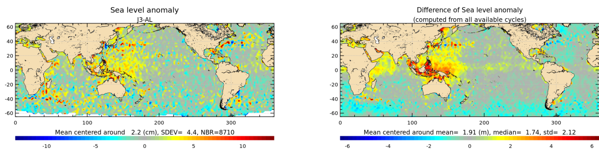
Figure 23: Jason-3 – Saral/AltiKa SLA differences for cycle 122 (left) and averaged over the whole Saral/AltiKa period (right).
