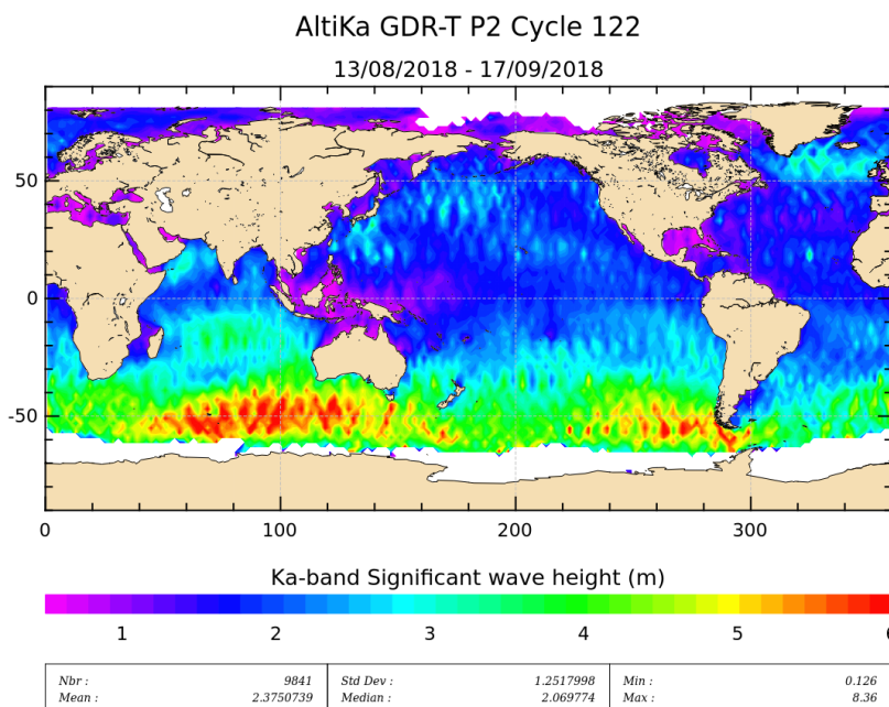
Figure 7: Significant wave height for cycle 122.
