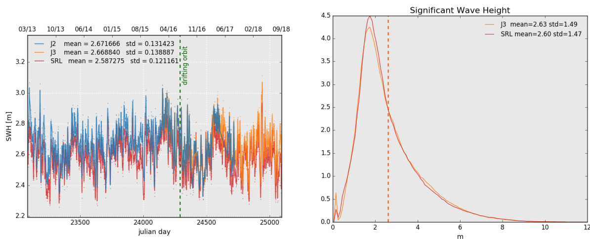
Figure 8: Daily monitoring of significant wave height for AltiKa (Ka-band) Jason-2 and Jason-3 (Ku-band) on the left and histogram for cycle 122 on the right (limited to 66^\circ latitude).
