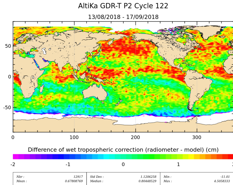
Figure 13: Mean of wet troposphere correction difference (Radiometer-ECMWF model) for cycle 122.
