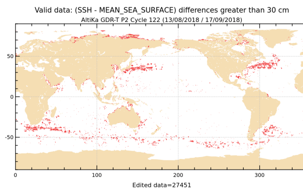
Figure 22: SLA higher than 30 cm for cycle 122.
