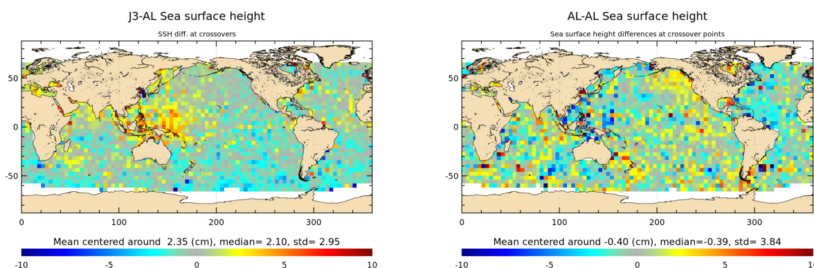
Figure 16: Mean of multi-mission SSH and mono-mission SSH differences at crossovers for cycle 122.
