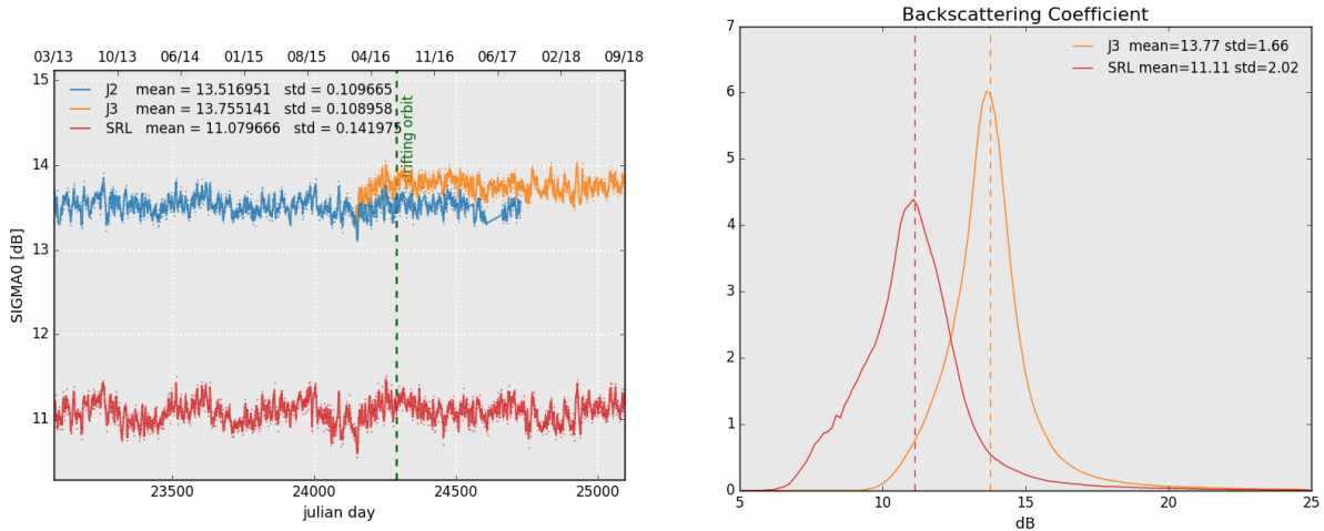
Figure 9: Daily monitoring of backscattering coefficient for Saral/AltiKa, Jason-2 and Jason-3 on the left and histogram for cycle 122 on the right (limited to 66° latitude).
