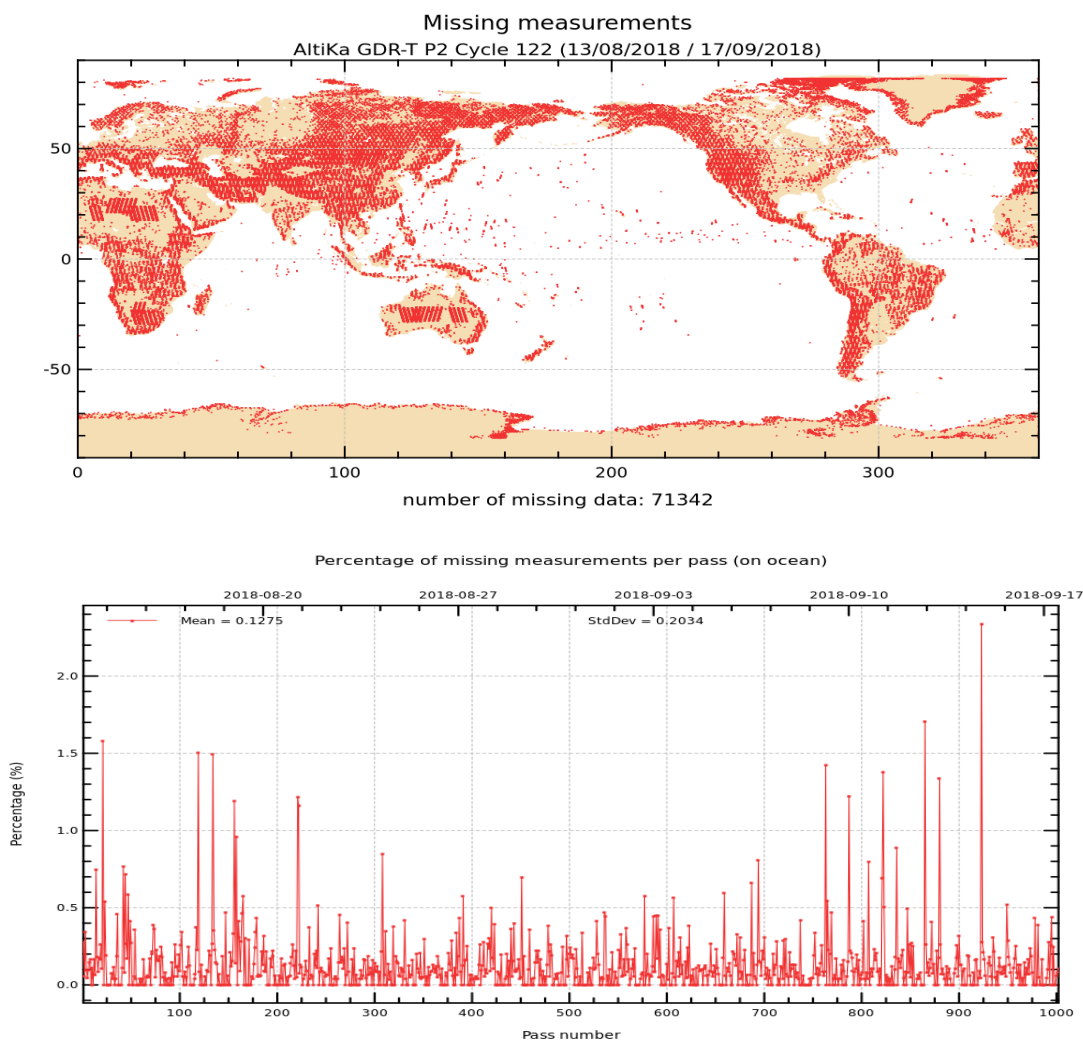
Figure 1: Map of missing measurements for cycle 122 on top. Monitoring of percentage of missing ocean measurements per pass on bottom.
