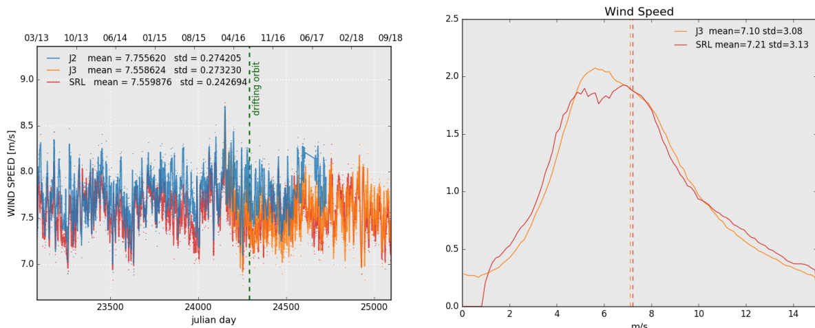
Figure 12: Daily monitoring of altimeter wind speed for Saral/AltiKa, Jason-2 and Jason-3 on the left and histogram for cycle 122 on the right (limited to 66° latitude).
