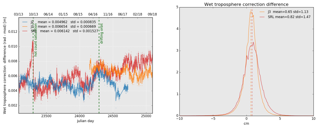
Figure 14: Daily monitoring of wet troposphere differences (Radiometer-ECMWF model) for Saral/AltiKa Jason-2 and Jason-3 (left) and histogram on the right (limited to 66° latitude) for cycle 122 .
