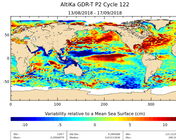
Figure 21: Sea level anomaly relative to MSS for cycle 122.
