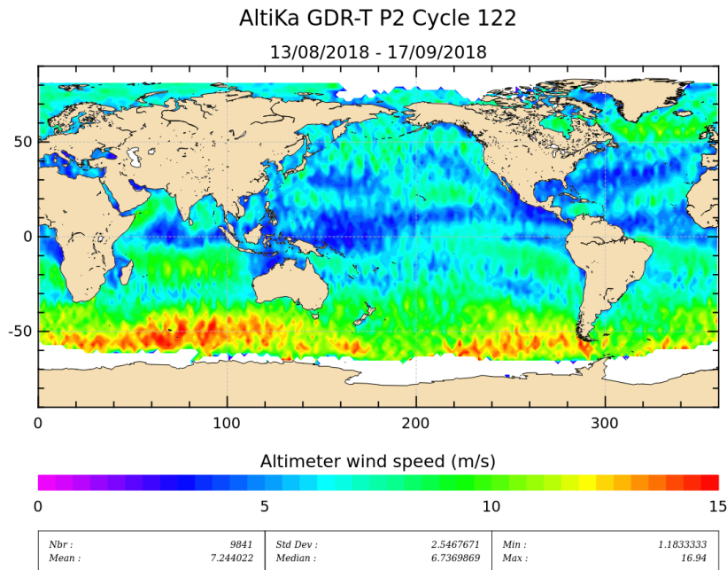
Figure 11: Altimeter wind speed for cycle 122.
