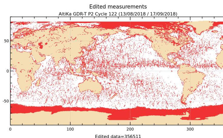
Figure 2: Edited measurements for cycle 122.
