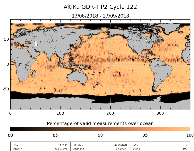
Figure 3: Percentage of valid measurements for cycle 122.
