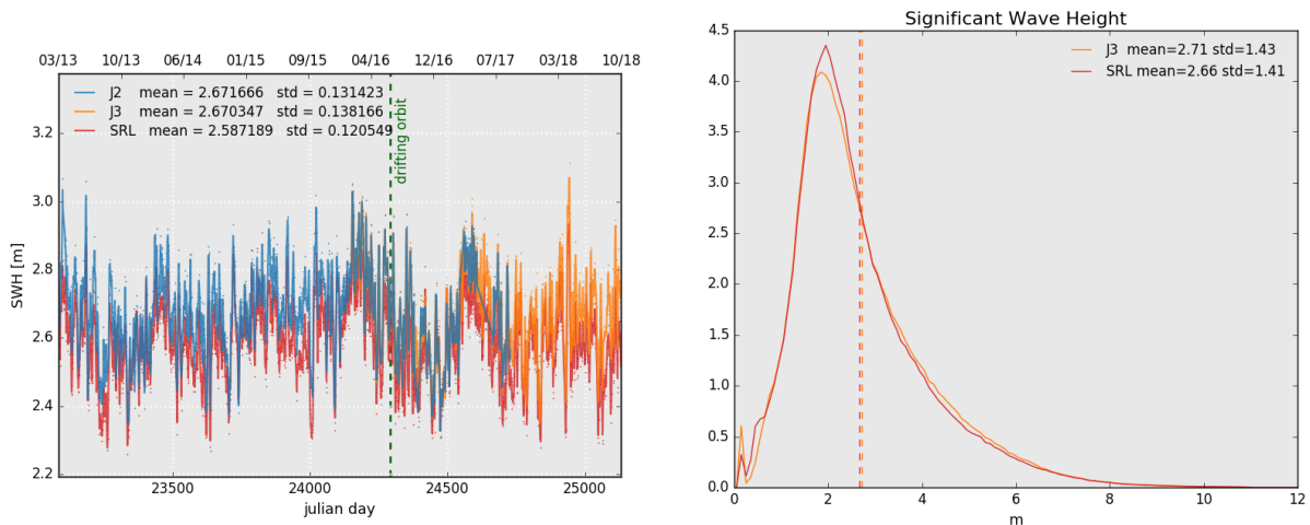
Figure 8: Daily monitoring of significant wave height for AltiKa (Ka-band) Jason-2 and Jason-3 (Ku-band) on the left and histogram for cycle 123 on the right (limited to 66^\circ latitude).
