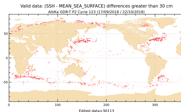
Figure 22: SLA higher than 30 cm for cycle 123.
