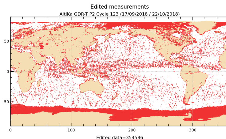
Figure 2: Edited measurements for cycle 123.
