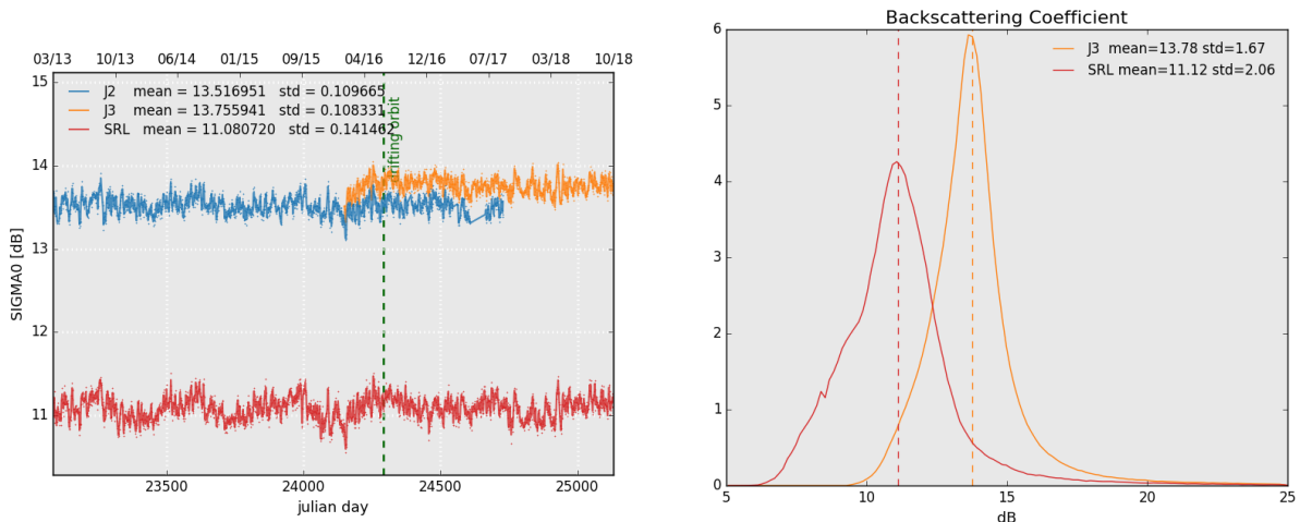
Figure 9: Daily monitoring of backscattering coefficient for Saral/AltiKa, Jason-2 and Jason-3 on the left and histogram for cycle 123 on the right (limited to 66° latitude).
