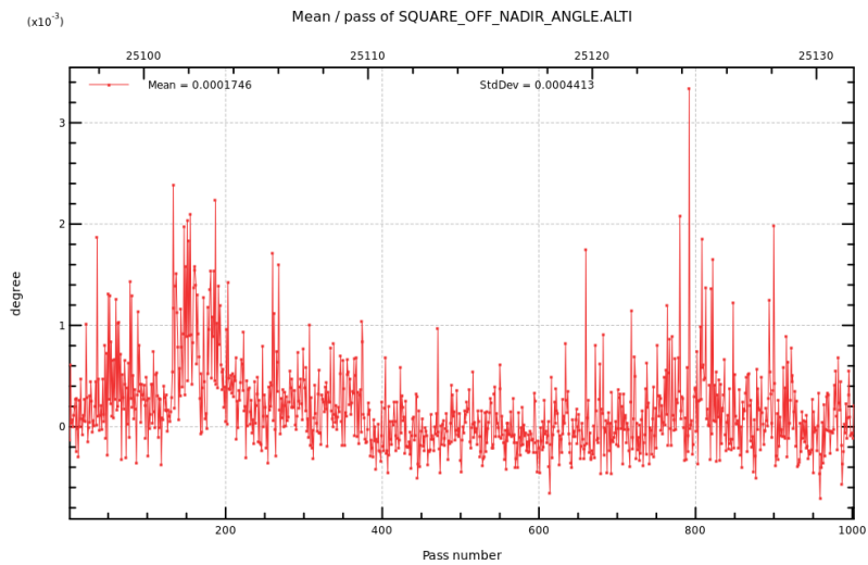
Figure 4: Mispointing cycle 123.
