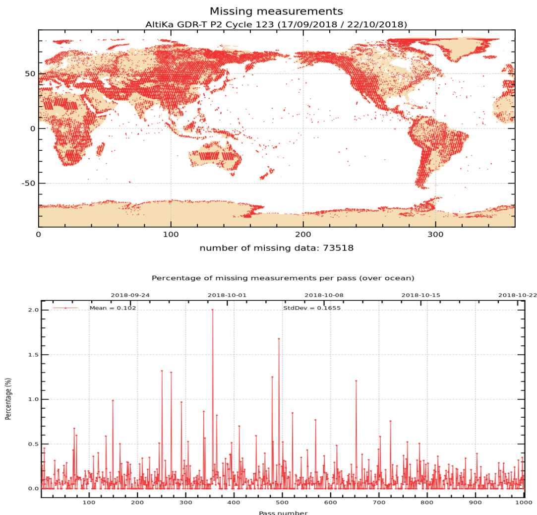
Figure 1: Map of missing measurements for cycle 123 on top. Monitoring of percentage of missing ocean measurements per pass on bottom.
