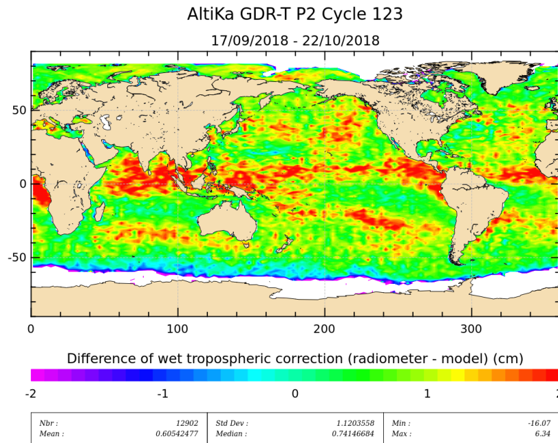
Figure 13: Mean of wet troposphere correction difference (Radiometer-ECMWF model) for cycle 123.
