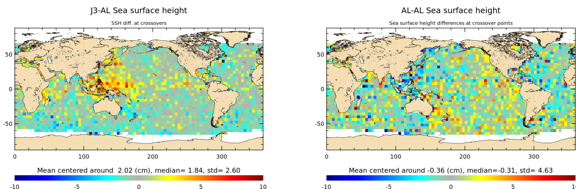
Figure 16: Mean of multi-mission SSH and mono-mission SSH differences at crossovers for cycle 123.
