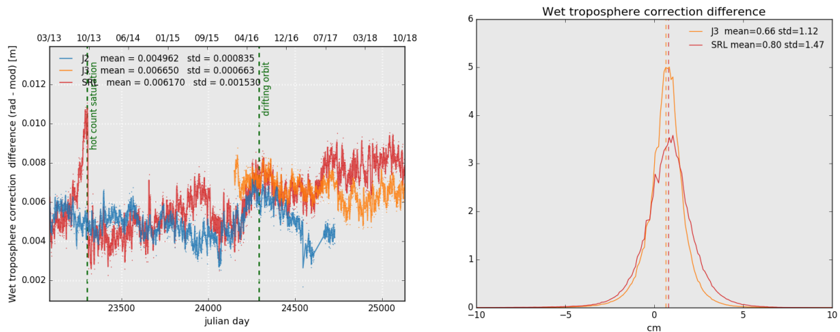
Figure 14: Daily monitoring of wet troposphere differences (Radiometer-ECMWF model) for Saral/AltiKa Jason-2 and Jason-3 (left) and histogram on the right (limited to 66° latitude) for cycle 123 .
