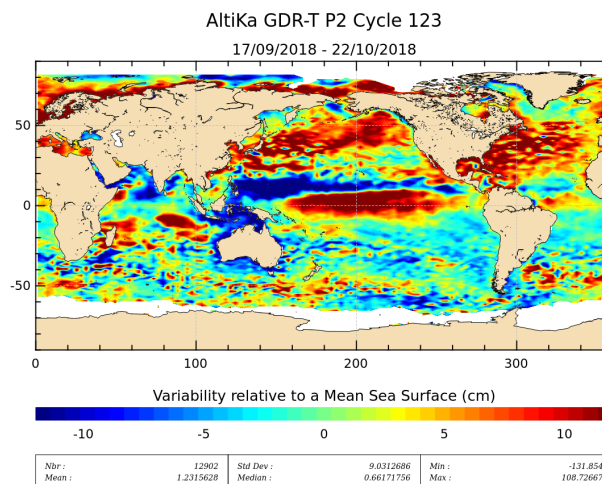
Figure 21: Sea level anomaly relative to MSS for cycle 123.
