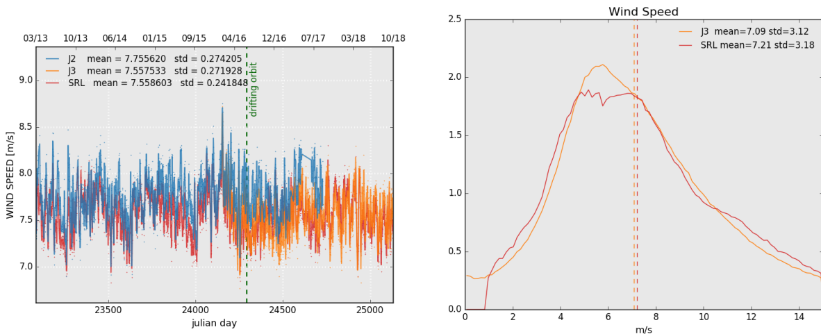
Figure 12: Daily monitoring of altimeter wind speed for Saral/AltiKa, Jason-2 and Jason-3 on the left and histogram for cycle 123 on the right (limited to 66° latitude).
