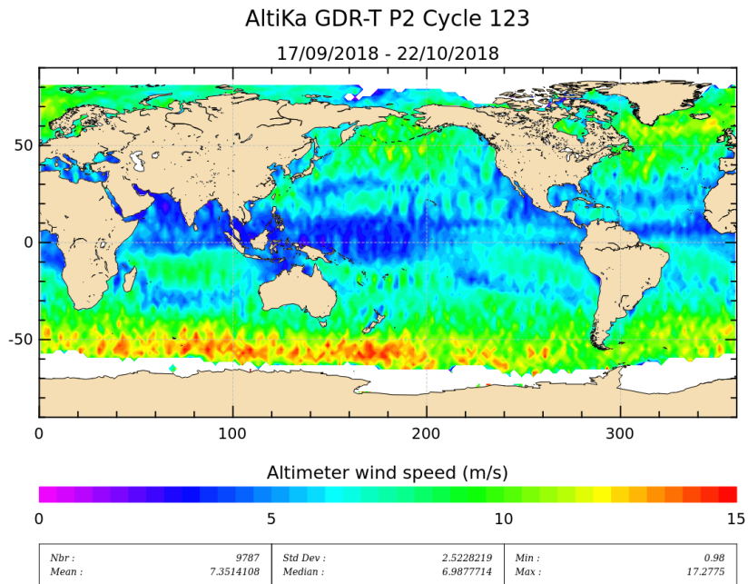
Figure 11: Altimeter wind speed for cycle 123.
