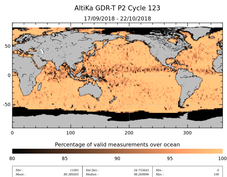
Figure 3: Percentage of valid measurements for cycle 123.
