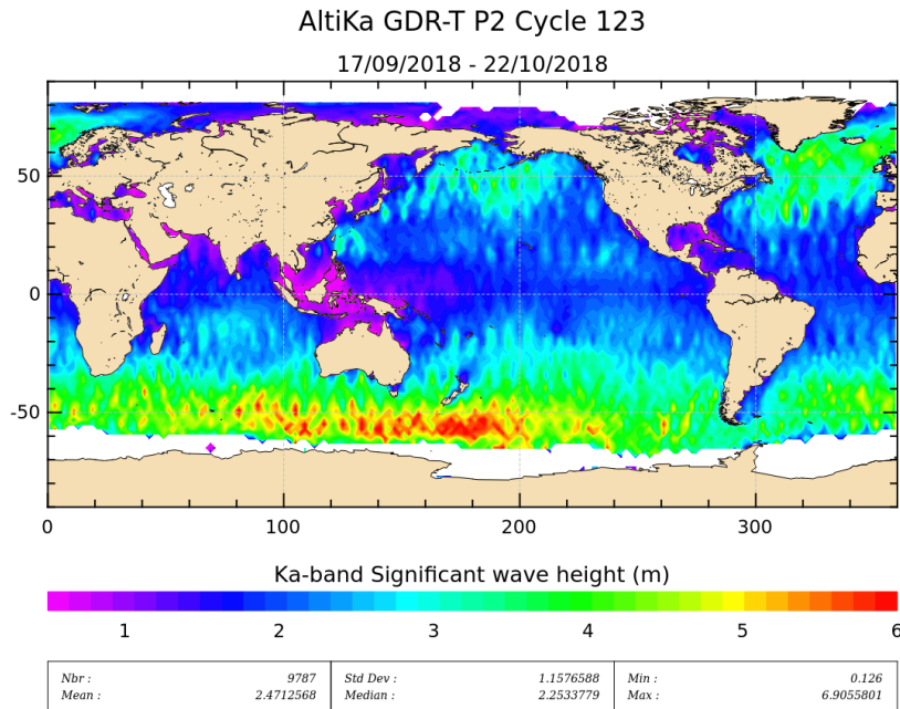
Figure 7: Significant wave height for cycle 123.
