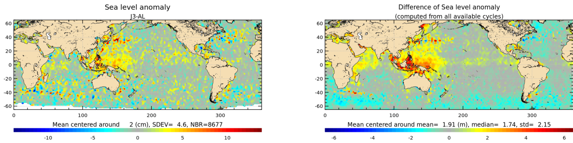
Figure 23: Jason-3 – Saral/AltiKa SLA differences for cycle 123 (left) and averaged over the whole Saral/AltiKa period (right).
