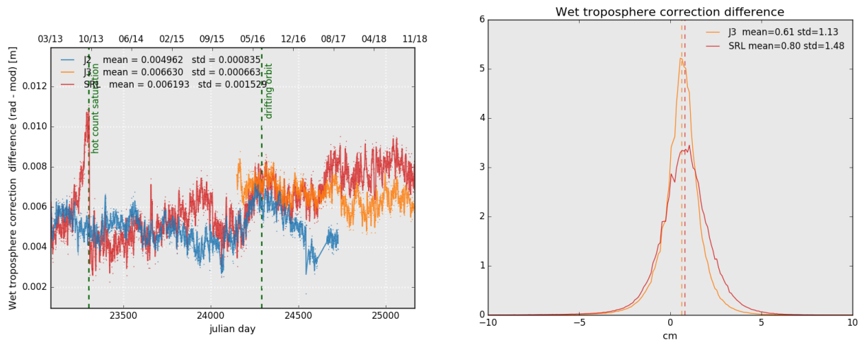
Figure 14: Daily monitoring of wet troposphere differences (Radiometer-ECMWF model) for Saral/AltiKa Jason-2 and Jason-3 (left) and histogram on the right (limited to 66° latitude) for cycle 124 .
