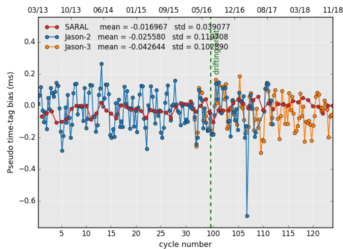
Figure 19: Cyclic monitoring of pseudo time tag bias for Saral/AltiKa.
