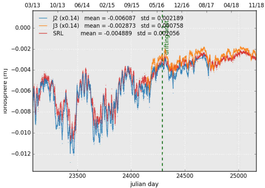
Figure 10: Daily monitoring of dual-frequency ionosphere correction for Jason-2 Jason-3 and GIM ionosphere correction for Saral/AltiKa.
