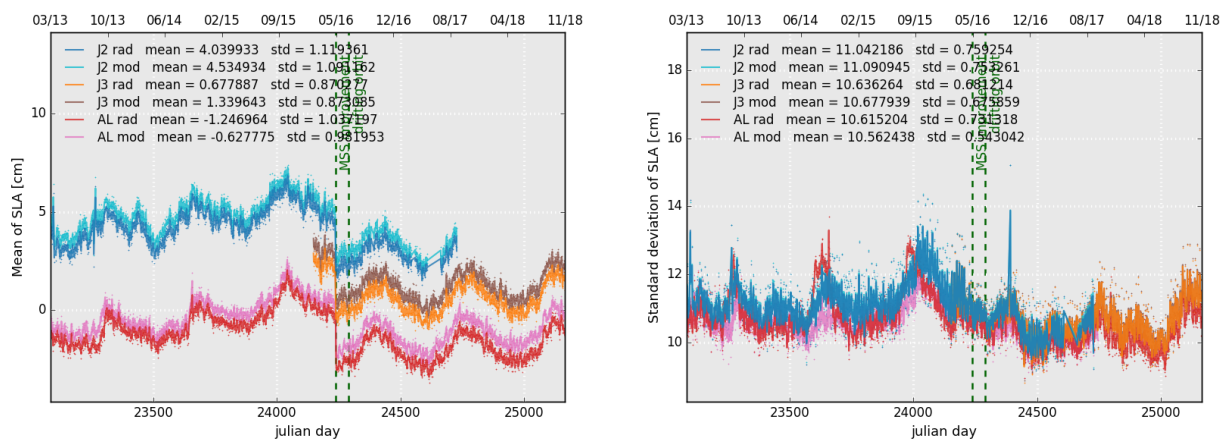
Figure 20: Daily monitoring of the mean (right) and standard deviation (left) of SLA for Saral/AltiKa, Jason-2 and Jason-3.
