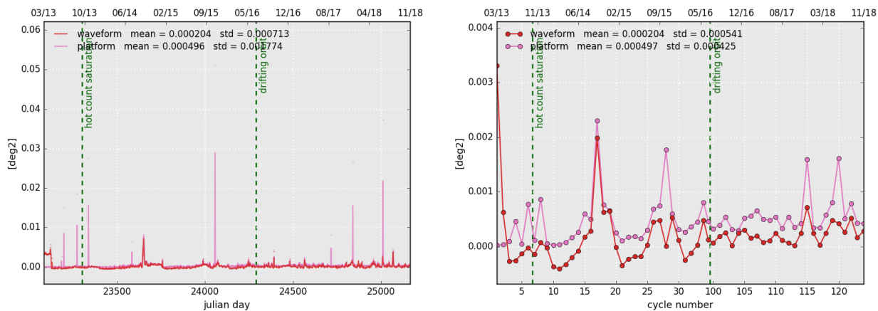
Figure 15: Daily (left) and cyclic (right) monitoring of SARAL/AltiKa's mispointing angle SARAL/AltiKa : comparison between the one derived from waveform retracking and the one measured by platform star-trackers.
