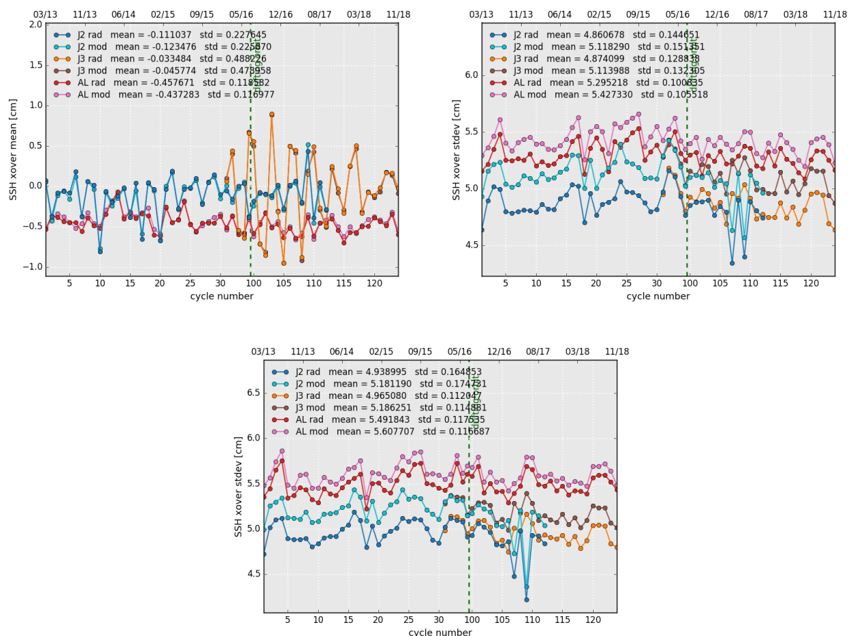
Figure 17: Cyclic monitoring of mean (left) and standard deviation of SSH differences at crossovers using only the geographical selection criteria (right) and both geographical selection and latitude weighting (bottom).
