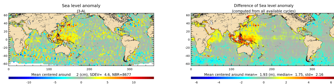
Figure 23: Jason-3 – Saral/AltiKa SLA differences for cycle 124 (left) and averaged over the whole Saral/AltiKa period (right).
