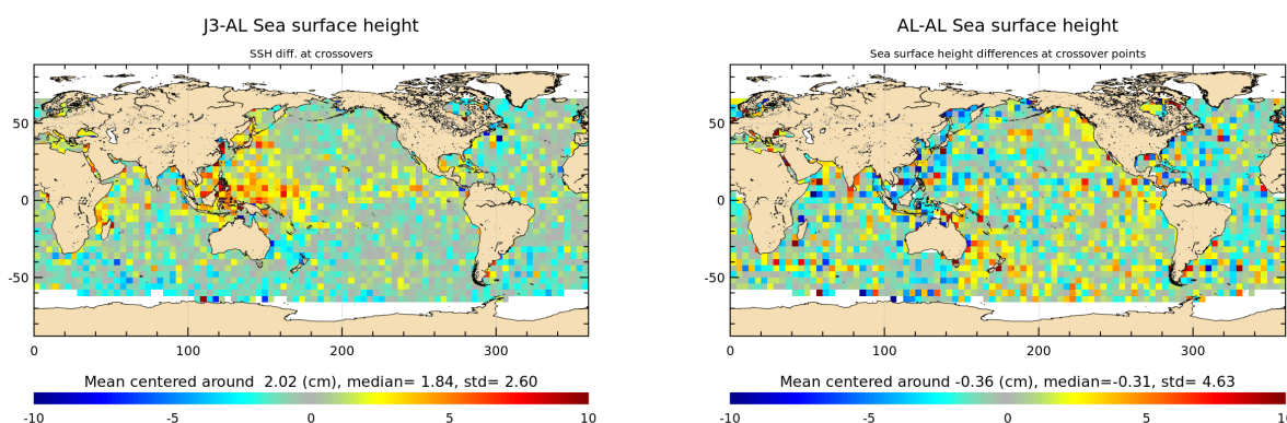
Figure 16: Mean of multi-mission SSH and mono-mission SSH differences at crossovers for cycle 124.
