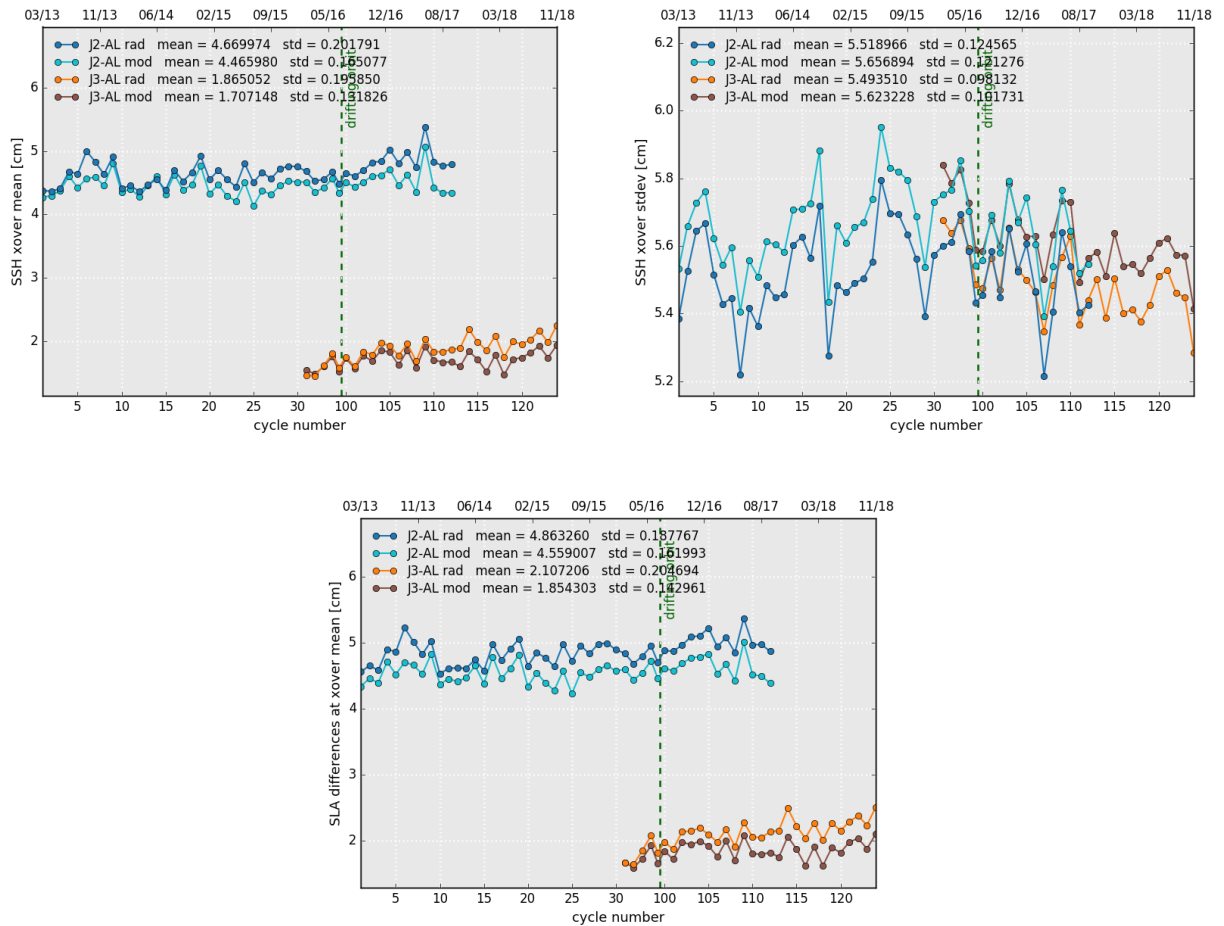
Figure 18: Cyclic monitoring of mean (left) and standard deviation (right) of Jason-2 / ALtiKa & Jason-3 / ALtiKa SSH differences at crossovers using geographical selections. Box-averaged SLA differences at crossovers (bottom).
