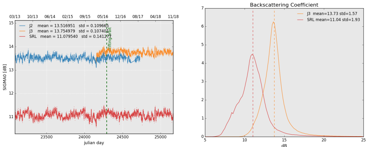
Figure 9: Daily monitoring of backscattering coefficient for Saral/AltiKa, Jason-2 and Jason-3 on the left and histogram for cycle 124 on the right (limited to 66° latitude).
