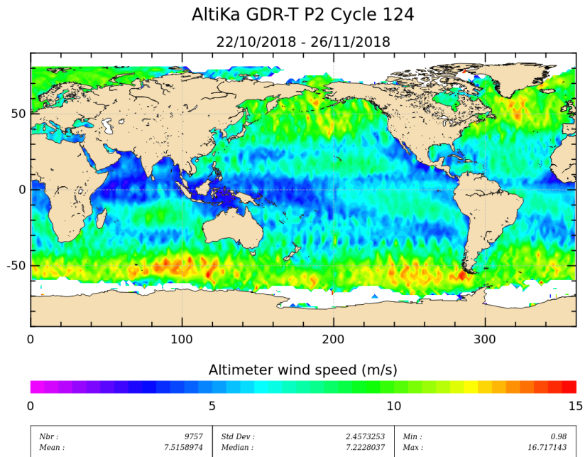
Figure 11: Altimeter wind speed for cycle 124.
