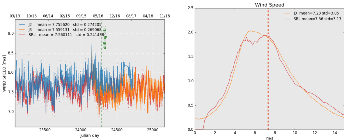
Figure 12: Daily monitoring of altimeter wind speed for Saral/AltiKa, Jason-2 and Jason-3 on the left and histogram for cycle 124 on the right (limited to 66° latitude).
