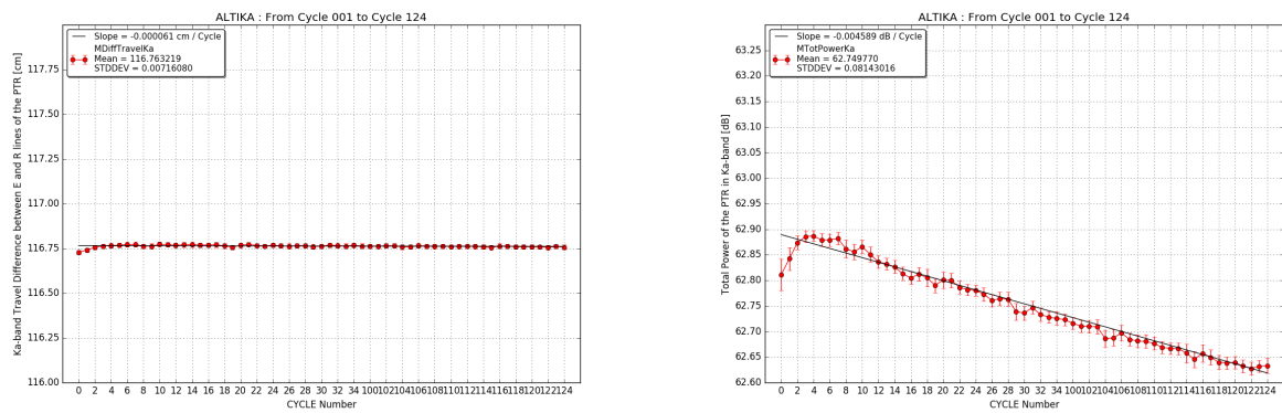
Figure 6: Internal path delay (left) and total power of the PTR (right) for Ka-band.
