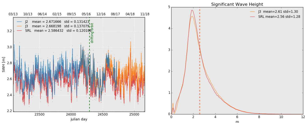
Figure 8: Daily monitoring of significant wave height for AltiKa (Ka-band) Jason-2 and Jason-3 (Ku-band) on the left and histogram for cycle 124 on the right (limited to 66^\circ latitude).
