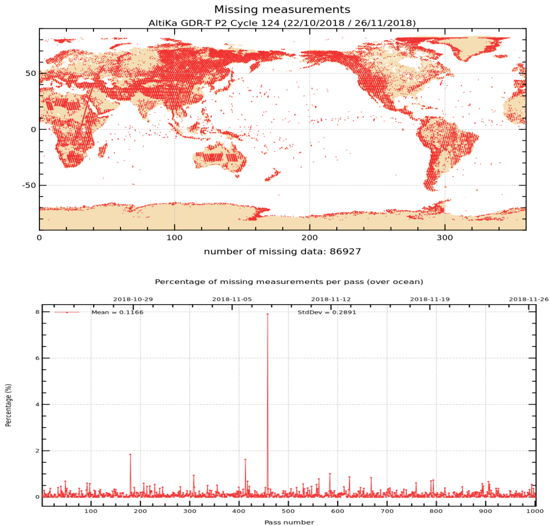
Figure 1: Map of missing measurements for cycle 124 on top. Monitoring of percentage of missing ocean measurements per pass on bottom.
