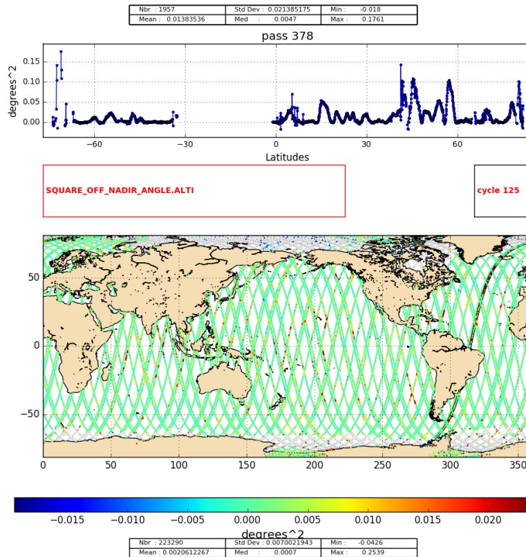
Figure 6: Mispointing Cycle 125: along track 362 to 496.
