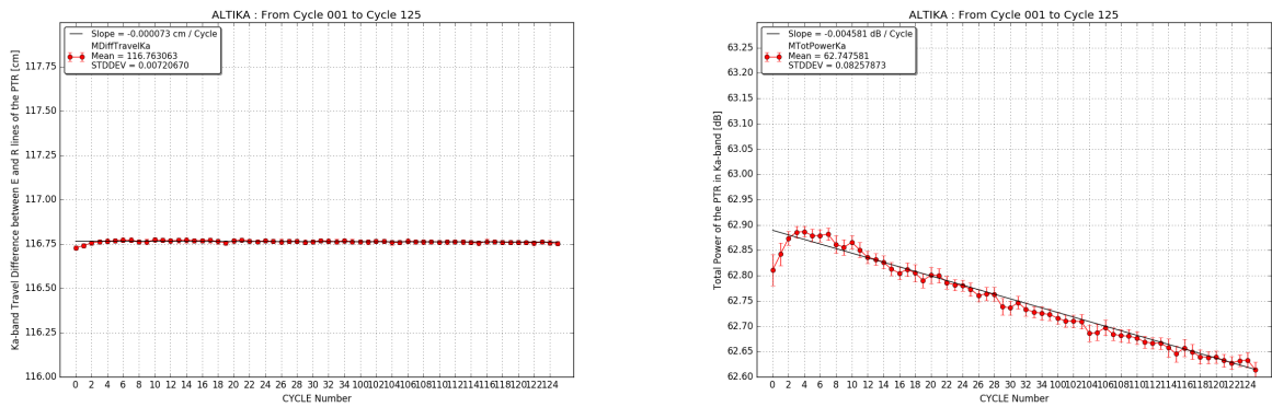
Figure 7: Internal path delay (left) and total power of the PTR (right) for Ka-band.
