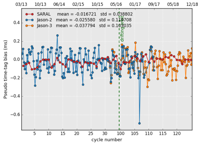
Figure 20: Cyclic monitoring of pseudo time tag bias for Saral/AltiKa.
