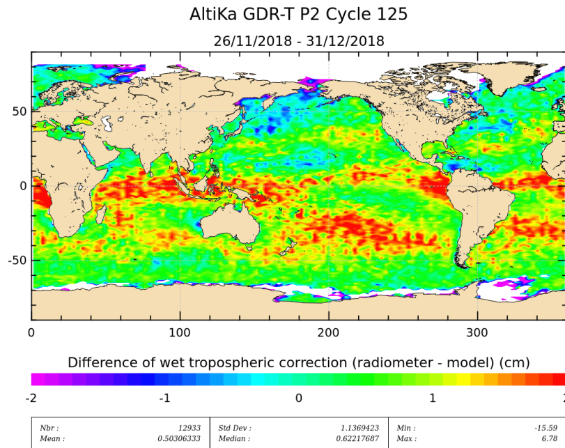
Figure 14: Mean of wet troposphere correction difference (Radiometer-ECMWF model) for cycle 125.
