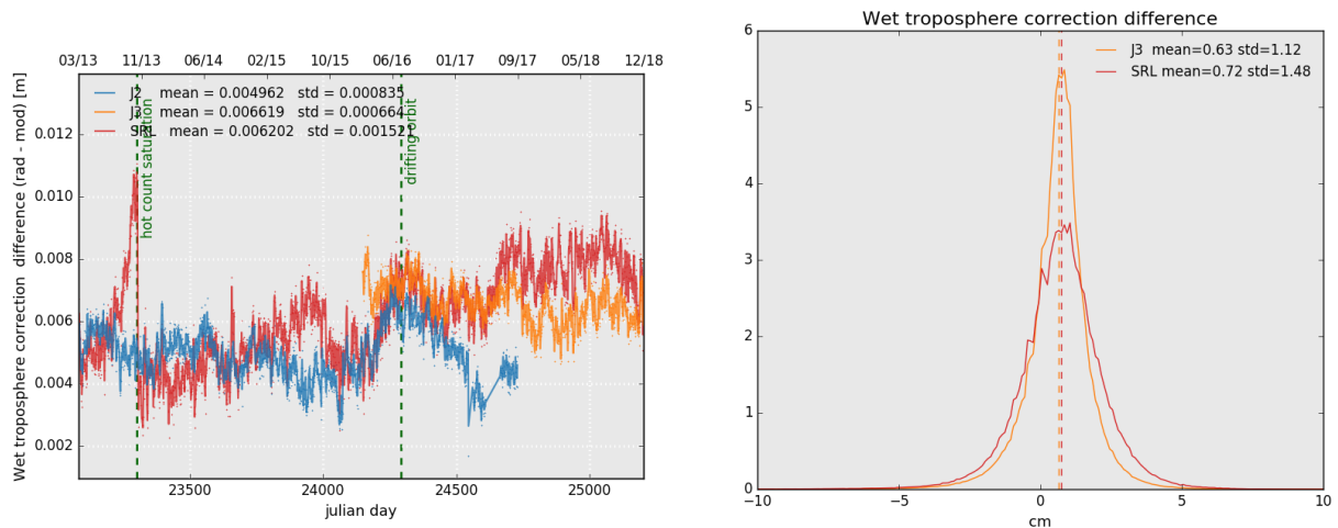
Figure 15: Daily monitoring of wet troposphere differences (Radiometer-ECMWF model) for Saral/AltiKa Jason-2 and Jason-3 (left) and histogram on the right (limited to 66° latitude) for cycle 125 .
