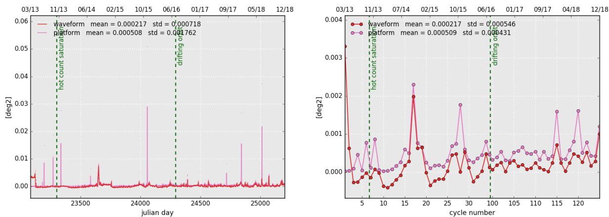
Figure 16: Daily (left) and cyclic (right) monitoring of SARAL/AltiKa's mispointing angle SARAL/AltiKa : comparison between the one derived from waveform tracking and the one measured by platform startrackers.
