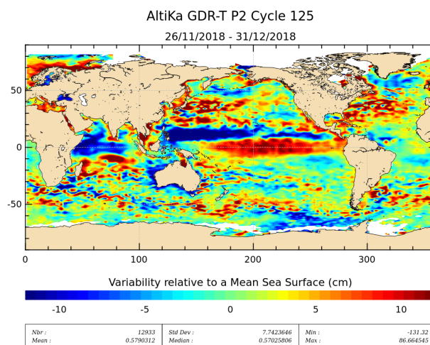
Figure 22: Sea level anomaly relative to MSS for cycle 125.
