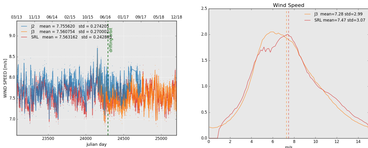
Figure 13: Daily monitoring of altimeter wind speed for Saral/AltiKa, Jason-2 and Jason-3 on the left and histogram for cycle 125 on the right (limited to 66° latitude).
