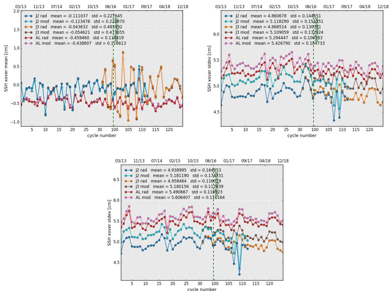
Figure 18: Cyclic monitoring of mean (left) and standard deviation of SSH differences at crossovers using only the geographical selection criteria (right) and both geographical selection and latitude weighting (bottom).
