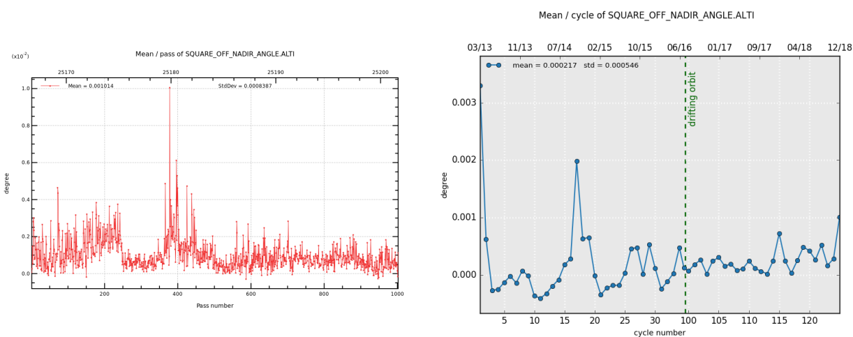
Figure 4: Mispointing: Cycle 125 / per track (left), whole time serie / per cycle (right).
