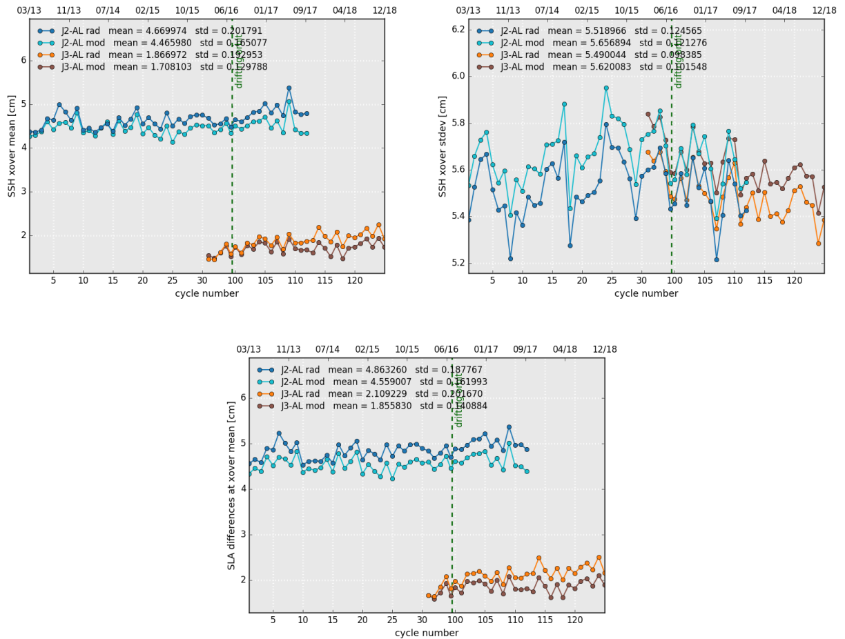
Figure 19: Cyclic monitoring of mean (left) and standard deviation (right) of Jason-2 / ALtiKa & Jason-3 / ALtiKa SSH differences at crossovers using geographical selections. Box-averaged SLA differences at crossovers (bottom).
