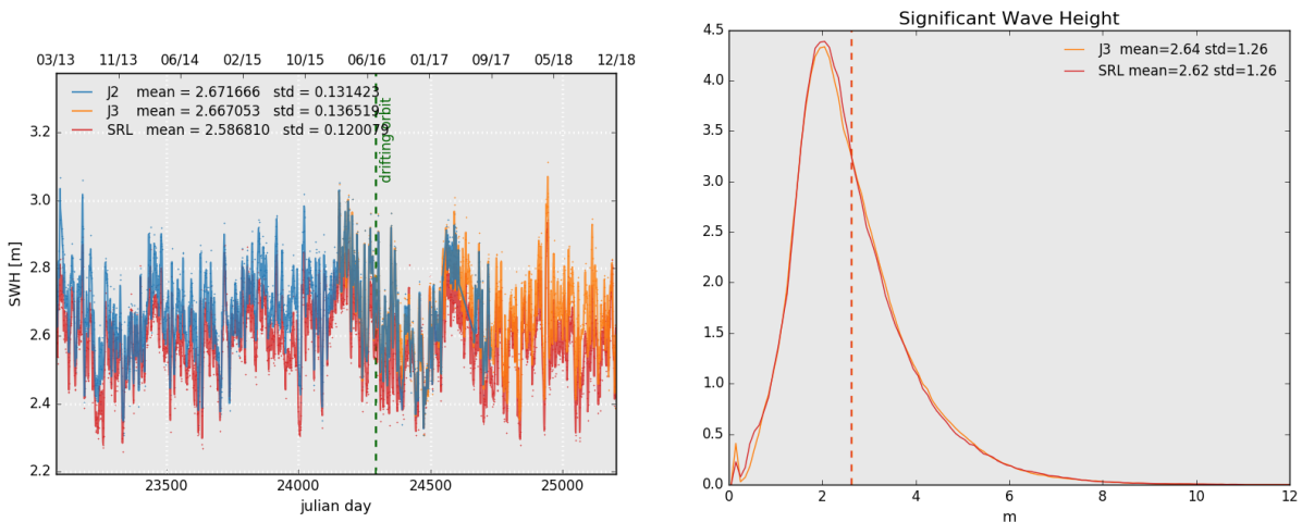
Figure 9: Daily monitoring of significant wave height for AltiKa (Ka-band) Jason-2 and Jason-3 (Ku-band) on the left and histogram for cycle 125 on the right (limited to 66^\circ latitude).
