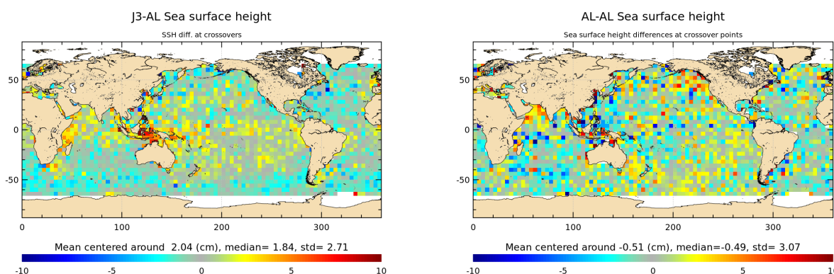
Figure 17: Mean of multi-mission SSH and mono-mission SSH differences at crossovers for cycle 125.
