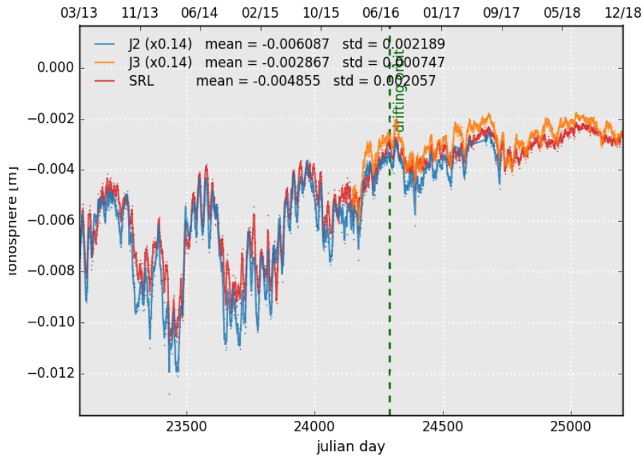
Figure 11: Daily monitoring of dual-frequency ionosphere correction for Jason-2 Jason-3 and GIM ionosphere correction for Saral/AltiKa.
