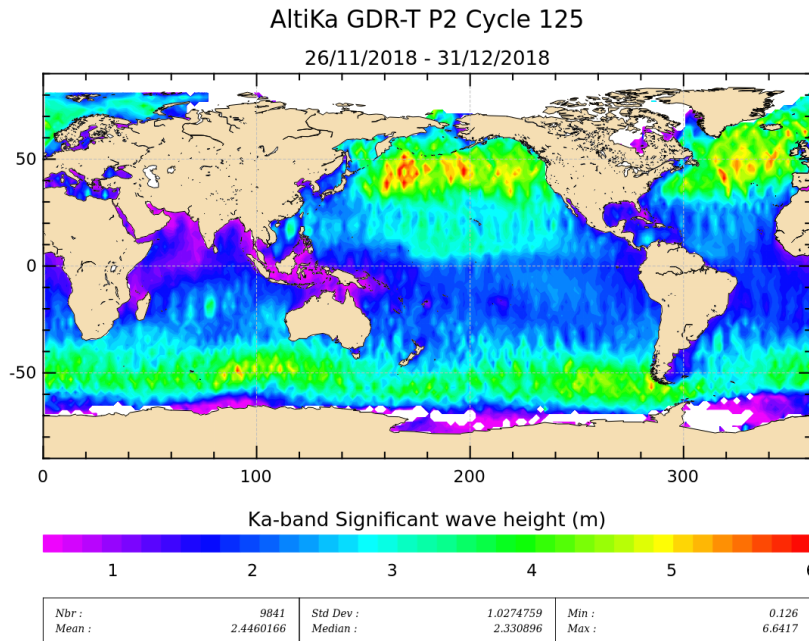
Figure 8: Significant wave height for cycle 125.
