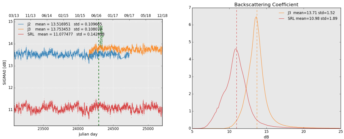
Figure 10: Daily monitoring of backscattering coefficient for Saral/AltiKa, Jason-2 and Jason-3 on the left and histogram for cycle 125 on the right (limited to 66° latitude).
