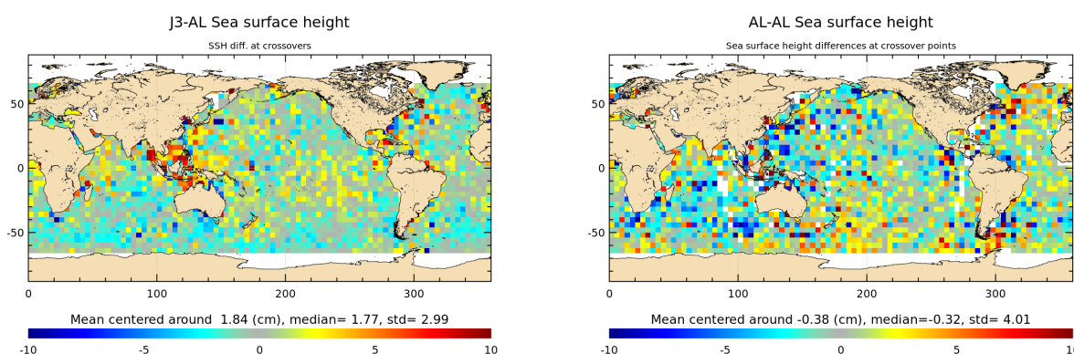
Figure 15: Mean of multi-mission SSH and mono-mission SSH differences at crossovers for cycle 128.
