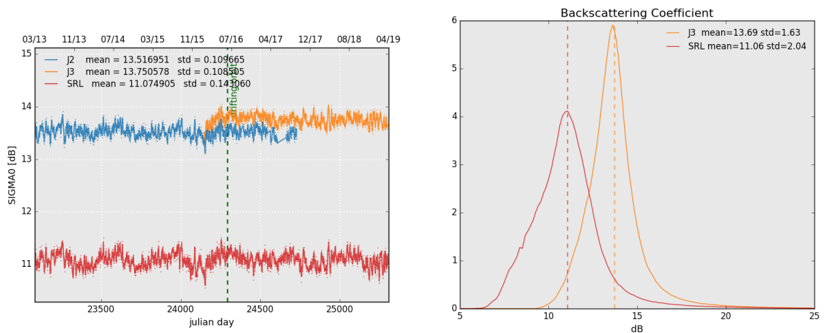
Figure 7: Daily monitoring of backscattering coefficient for Saral/AltiKa, Jason-2 and Jason-3 on the left and histogram for cycle 128 on the right (limited to 66° latitude).
