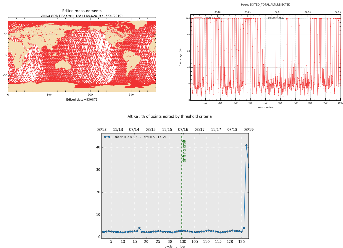
Figure 2: Rejected measurements on thresholds criteria : Cycle 128, map and monitoring of % of rejected measurements per track (top), whole time serie / % of rejected measurements per cycle (bottom).
