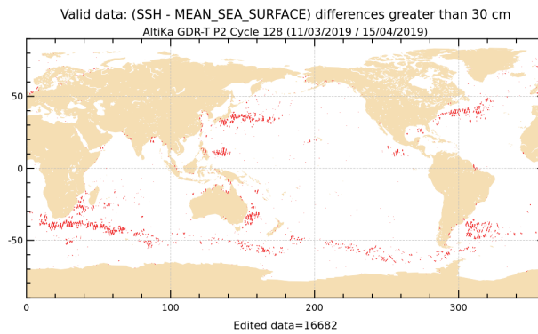
Figure 20: Sea level anomaly relative to MSS for cycle 128.
