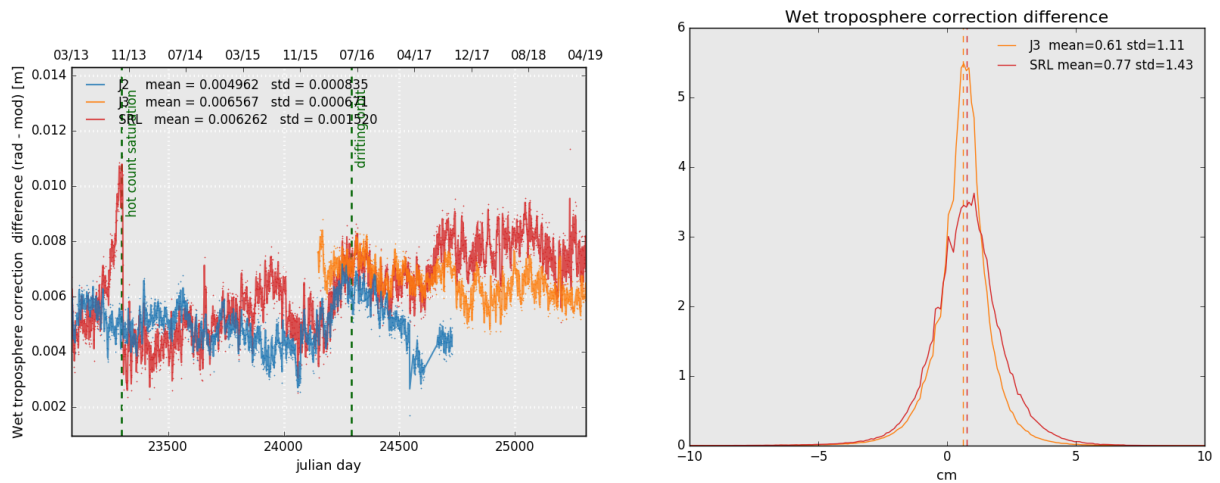
Figure 12: Daily monitoring of wet troposphere differences (Radiometer-ECMWF model) for Saral/AltiKa Jason-2 and Jason-3 (left) and histogram on the right (limited to 66° latitude) for cycle 128 .
