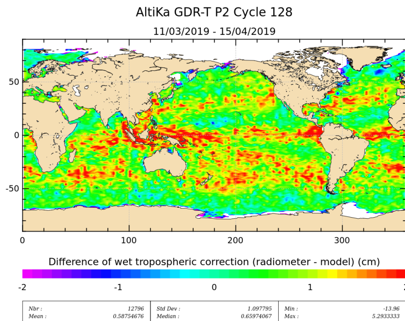
Figure 11: Mean of wet troposphere correction difference (Radiometer-ECMWF model) for cycle 128.
