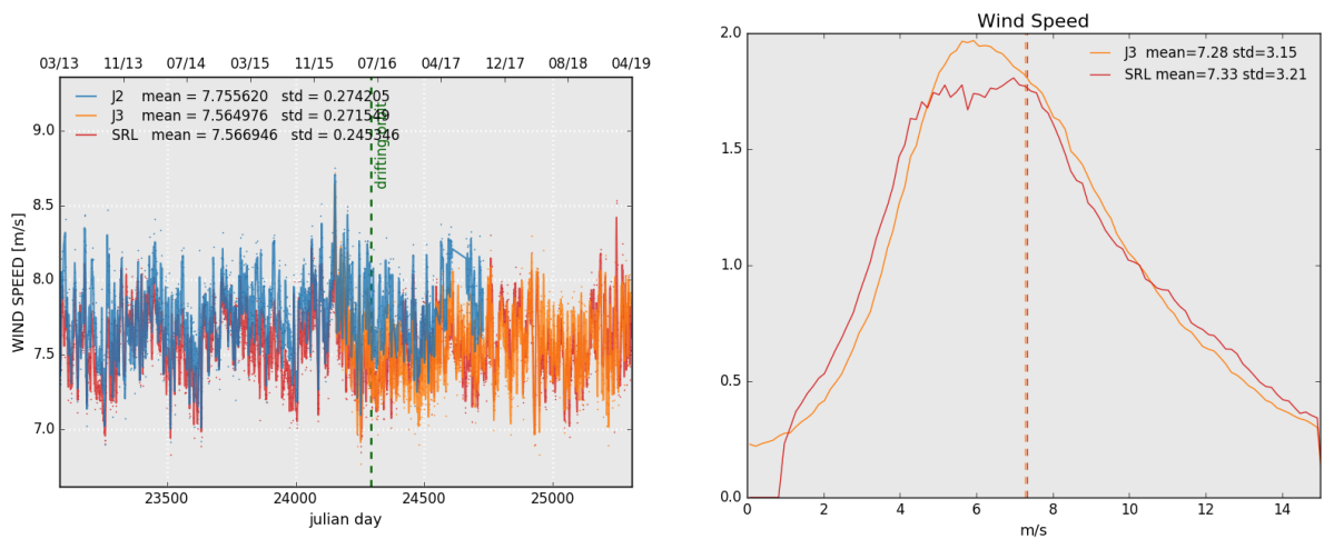
Figure 10: Daily monitoring of altimeter wind speed for Saral/AltiKa, Jason-2 and Jason-3 on the left and histogram for cycle 128 on the right (limited to 66° latitude).
