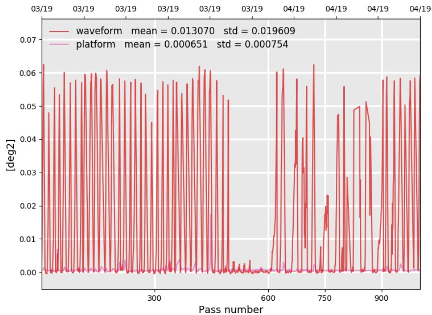
Figure 14: Monitoring per pass for cycle 128 of SARAL/AltiKa's mispointing angle: comparison between the one derived from waveform retracking and the one measured by platform startrackers.
