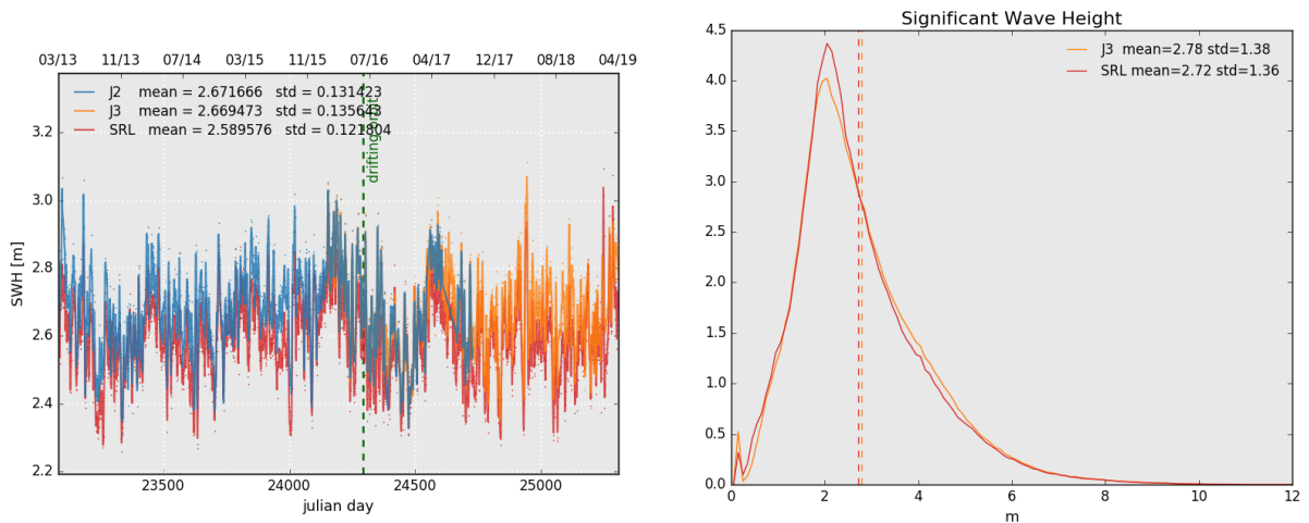
Figure 6: Daily monitoring of significant wave height for AltiKa (Ka-band) Jason-2 and Jason-3 (Ku-band) on the left and histogram for cycle 128 on the right (limited to 66° latitude).
