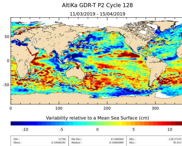
Figure 20: Sea level anomaly relative to MSS for cycle 128.
