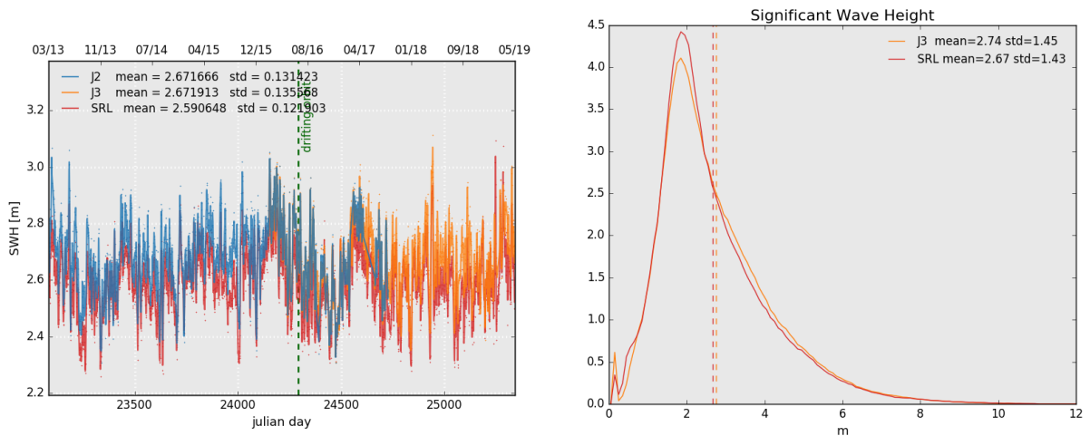
Figure 6: Daily monitoring of significant wave height for AltiKa (Ka-band) Jason-2 and Jason-3 (Ku-band) on the left and histogram for cycle 129 on the right (limited to 66° latitude).
