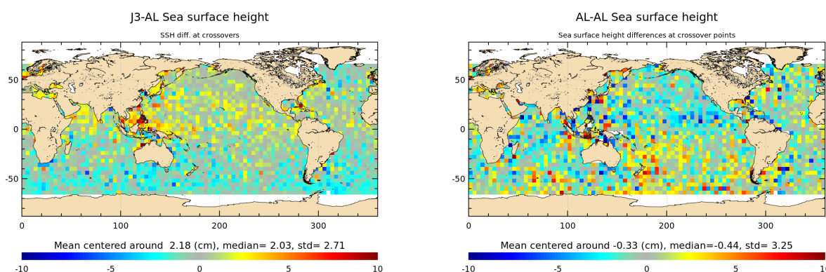
Figure 15: Mean of multi-mission SSH and mono-mission SSH differences at crossovers for cycle 129.
