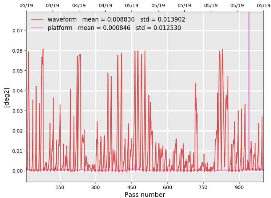
Figure 14: Monitoring per pass for cycle 129 of SARAL/AltiKa's mispointing angle: comparison between the one derived from waveform retracking and the one measured by platform startrackers.
