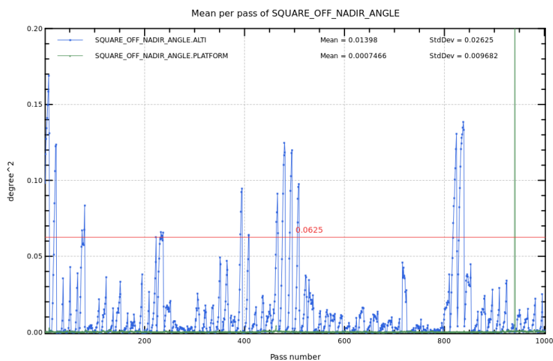
Figure 3: Mispointing cycle 129.
