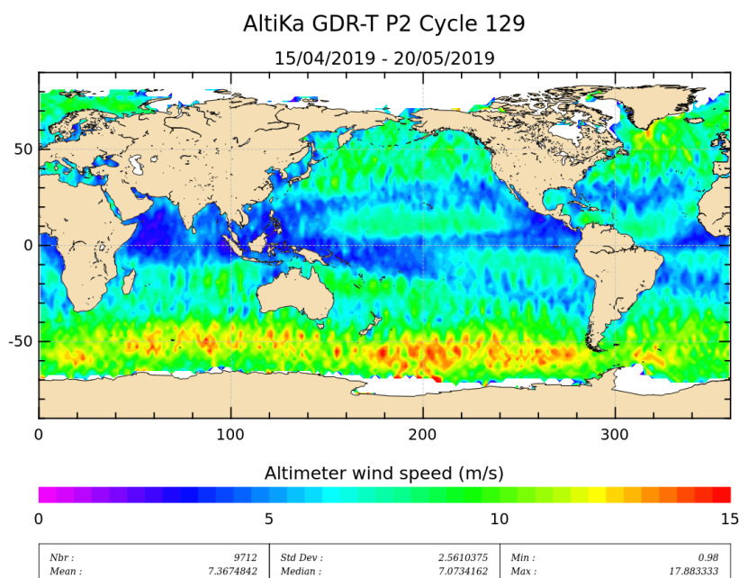
Figure 9: Altimeter wind speed for cycle 129.
