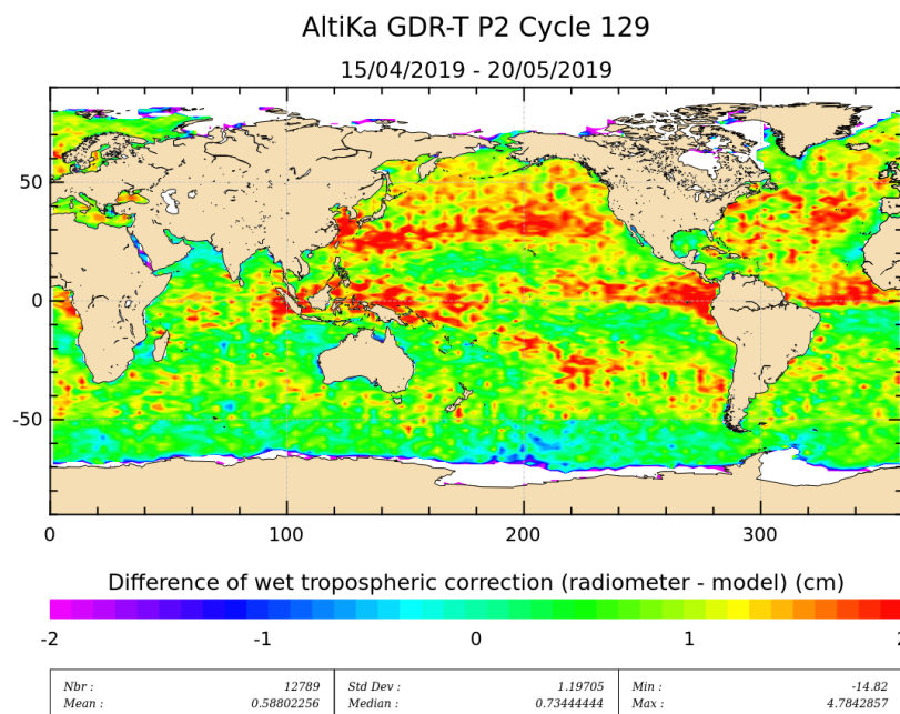
Figure 11: Mean of wet troposphere correction difference (Radiometer-ECMWF model) for cycle 129.
