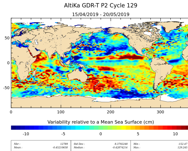
Figure 20: Sea level anomaly relative to MSS for cycle 129.
