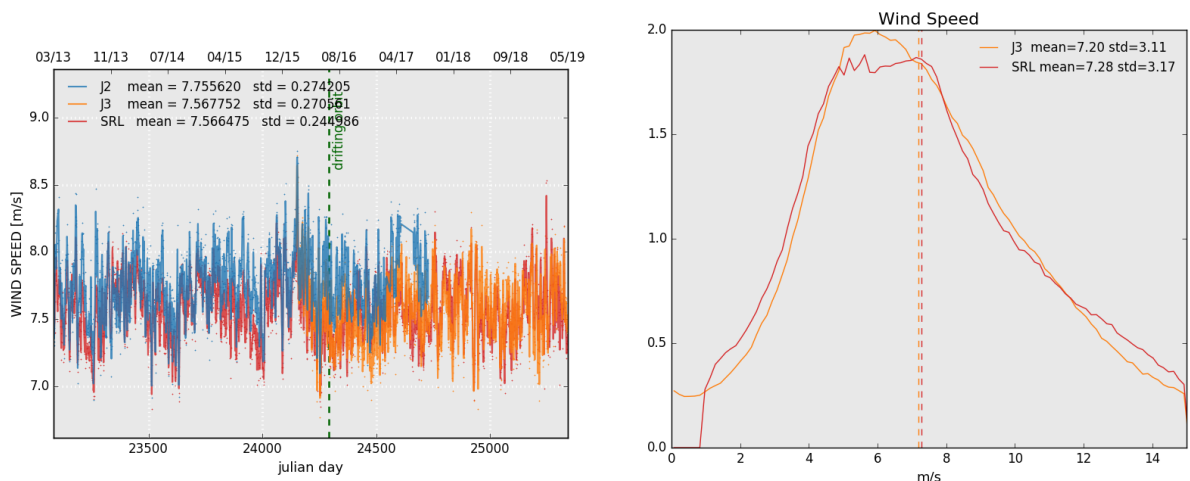
Figure 10: Daily monitoring of altimeter wind speed for Saral/AltiKa, Jason-2 and Jason-3 on the left and histogram for cycle 129 on the right (limited to 66° latitude).
