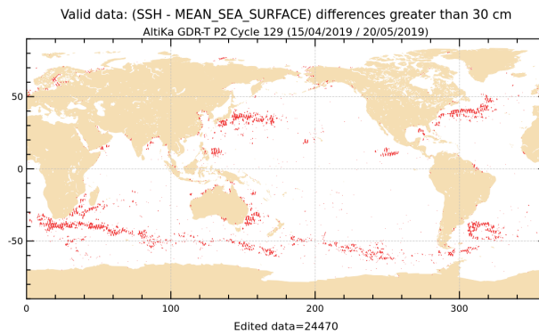
Figure 20: Sea level anomaly relative to MSS for cycle 129.
