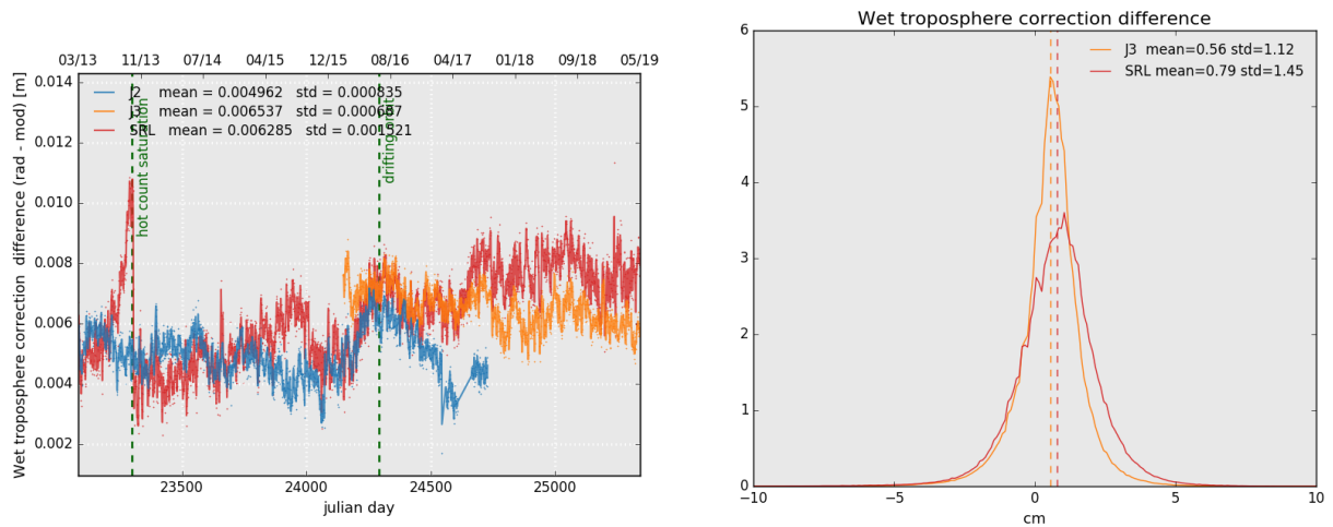
Figure 12: Daily monitoring of wet troposphere differences (Radiometer-ECMWF model) for Saral/AltiKa Jason-2 and Jason-3 (left) and histogram on the right (limited to 66° latitude) for cycle 129 .
