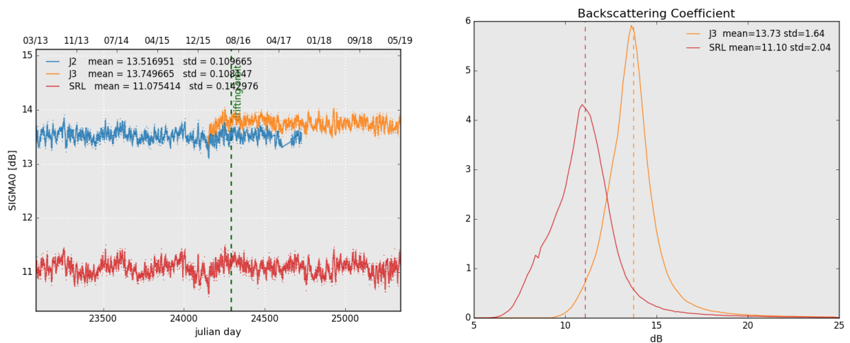
Figure 7: Daily monitoring of backscattering coefficient for Saral/AltiKa, Jason-2 and Jason-3 on the left and histogram for cycle 129 on the right (limited to 66° latitude).
