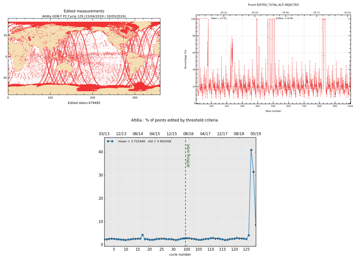
Figure 2: Rejected measurements on thresholds criteria : Cycle 129, map and monitoring of % of rejected measurements per track (top), whole time serie / % of rejected measurements per cycle (bottom).
