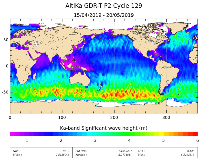
Figure 5: Significant wave height for cycle 129.
