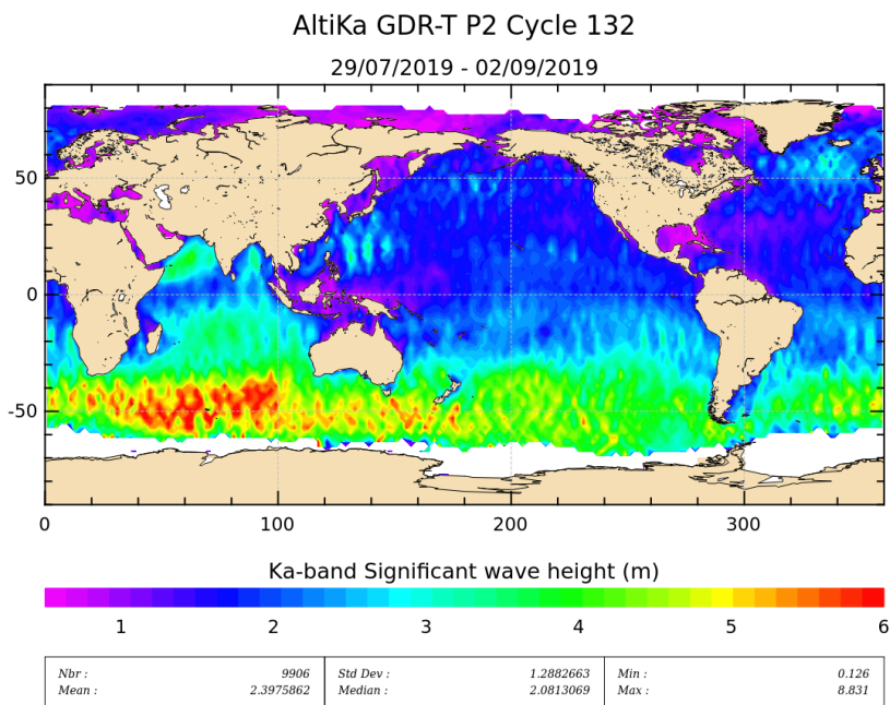
Figure 5: Significant wave height for cycle 132.
