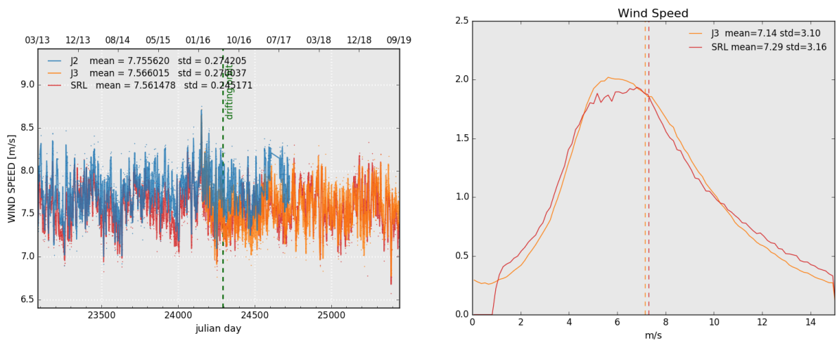
Figure 10: Daily monitoring of altimeter wind speed for Saral/AltiKa, Jason-2 and Jason-3 on the left and histogram for cycle 132 on the right (limited to 66° latitude).
