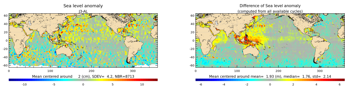
Figure 20: SLA higher than 30 cm for cycle 132.
