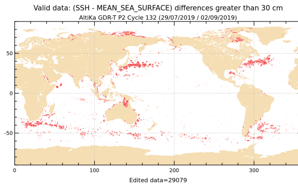
Figure 19: Sea level anomaly relative to MSS for cycle 132.
