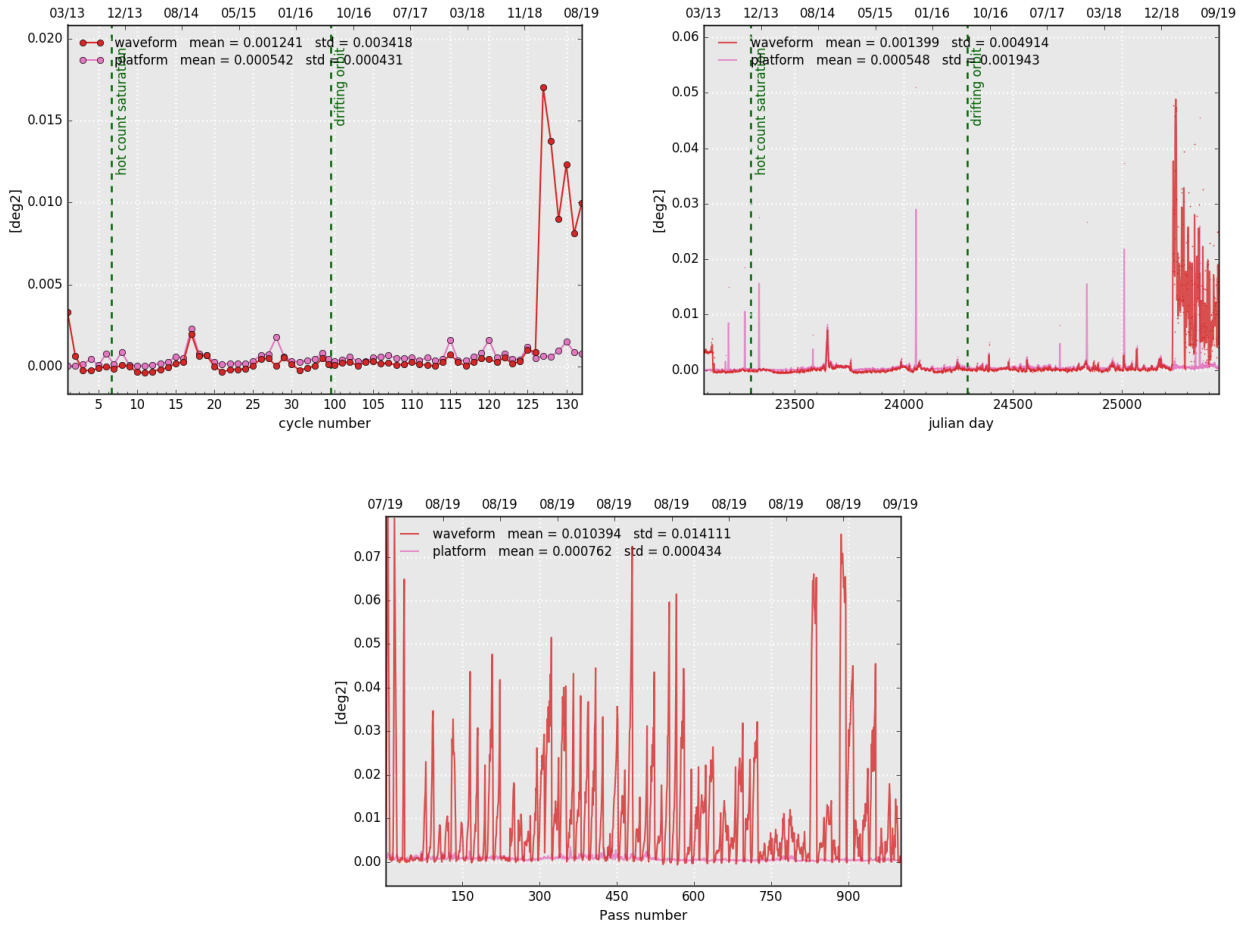
Figure 13: Cyclic monitoring(left), daily monitoring(right) and monitoring per pass for cycle 132 (bottom) of SARAL/AltiKa’s mispointing angle: comparison between the one derived from waveform retracking and the one measured by platform startrackers.
