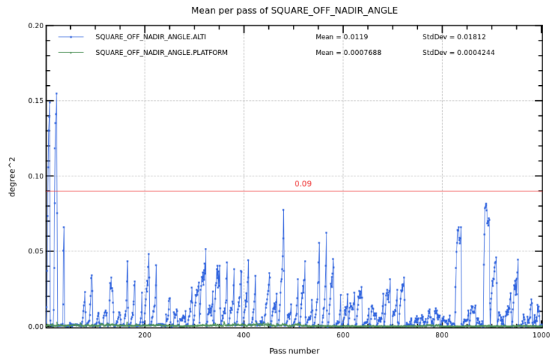
Figure 3: Mispointing cycle 132. Users are advised to use data with off\_nadir\_angle < 0.09deg^2
