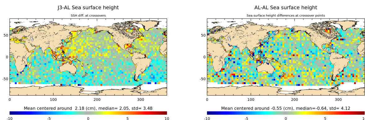
Figure 14: Mean of multi-mission SSH and mono-mission SSH differences at crossovers for cycle 132.
