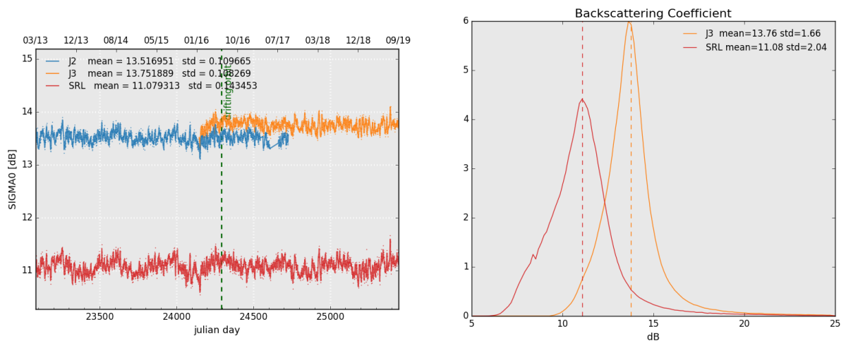
Figure 7: Daily monitoring of backscattering coefficient for Saral/AltiKa, Jason-2 and Jason-3 on the left and histogram for cycle 132 on the right (limited to 66° latitude).
