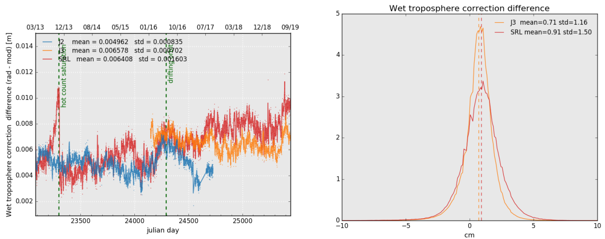
Figure 12: Daily monitoring of wet troposphere differences (Radiometer-ECMWF model) for Saral/AltiKa Jason-2 and Jason-3 (left) and histogram on the right (limited to 66° latitude) for cycle 132 .
