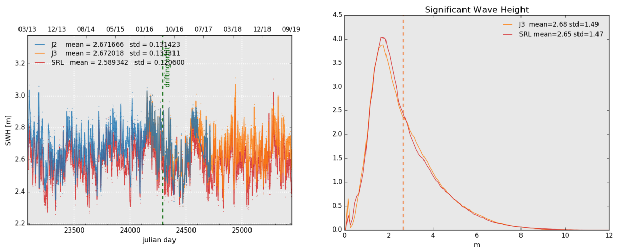
Figure 6: Daily monitoring of significant wave height for AltiKa (Ka-band) Jason-2 and Jason-3 (Ku-band) on the left and histogram for cycle 132 on the right (limited to 66° latitude).
