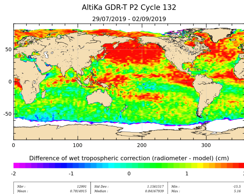
Figure 11: Mean of wet troposphere correction difference (Radiometer-ECMWF model) for cycle 132.
