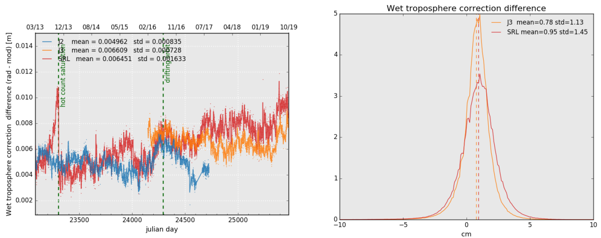
Figure 12: Daily monitoring of wet troposphere differences (Radiometer-ECMWF model) for Saral/AltiKa Jason-2 and Jason-3 (left) and histogram on the right (limited to 66° latitude) for cycle 133 .
