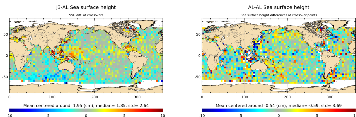
Figure 14: Mean of multi-mission SSH and mono-mission SSH differences at crossovers for cycle 133.
