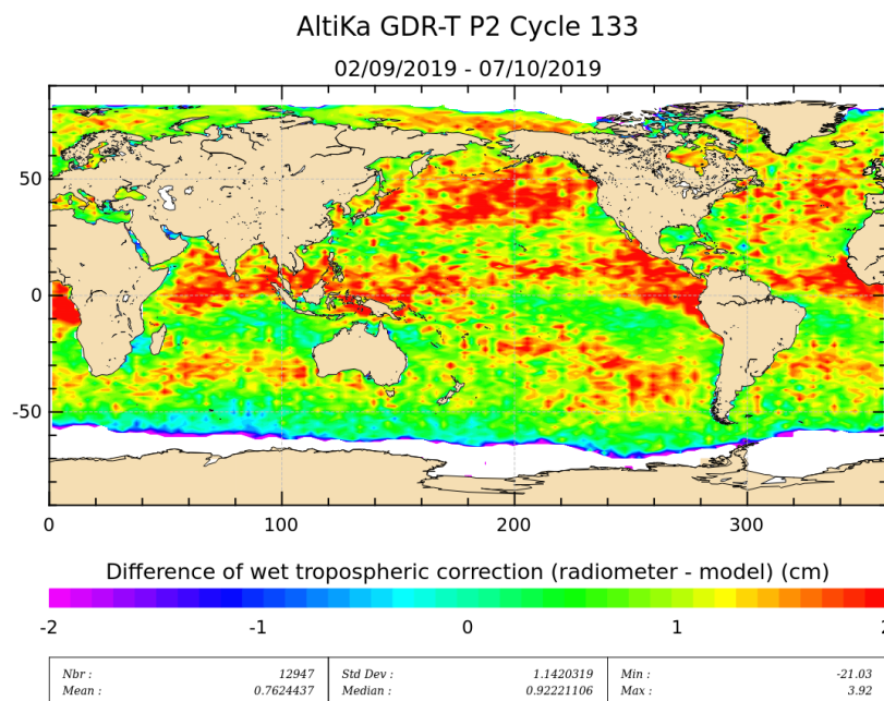
Figure 11: Mean of wet troposphere correction difference (Radiometer-ECMWF model) for cycle 133.
