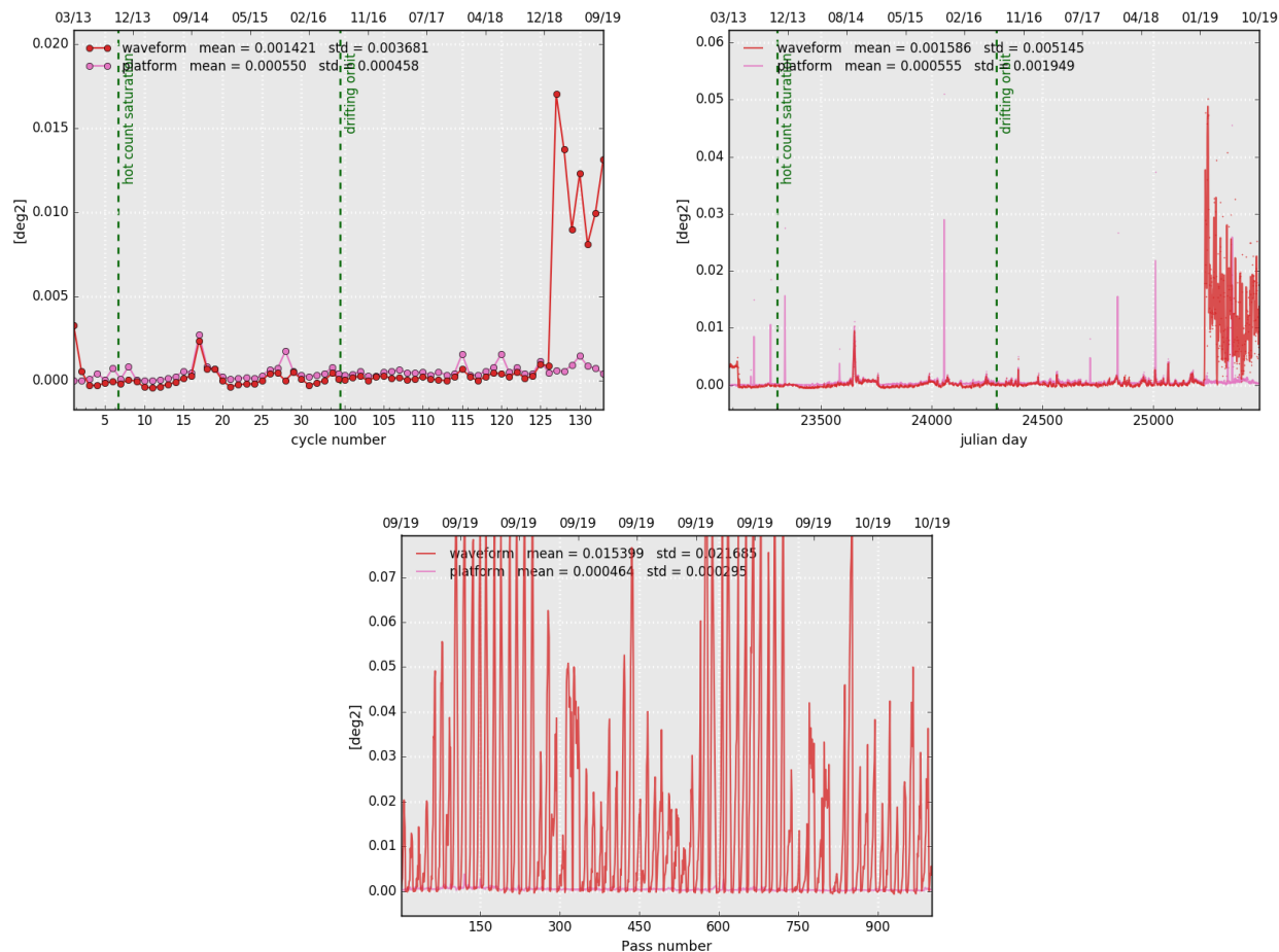
Figure 13: Cyclic monitoring(left), daily monitoring(right) and monitoring per pass for cycle 133 (bottom) of SARAL/AltiKa's mispointing angle: comparison between the one derived from waveform retracking and the one measured by platform startrackers.
