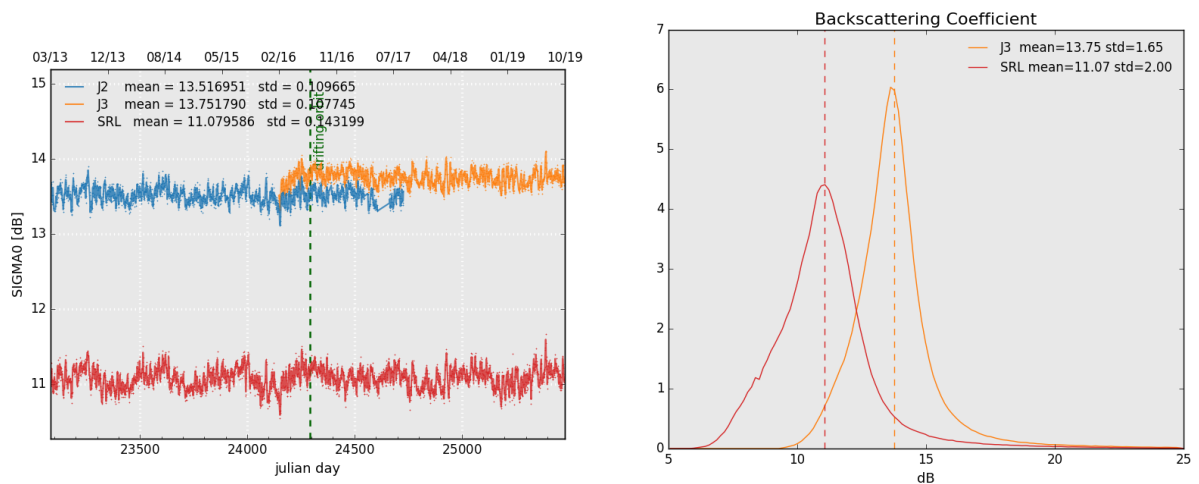
Figure 7: Daily monitoring of backscattering coefficient for Saral/AltiKa, Jason-2 and Jason-3 on the left and histogram for cycle 133 on the right (limited to 66° latitude).
