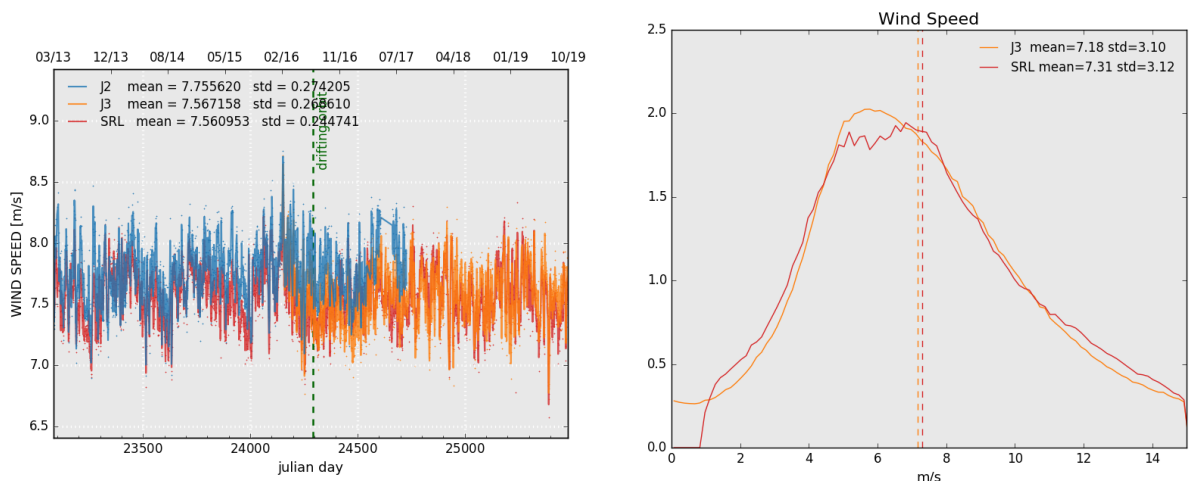
Figure 10: Daily monitoring of altimeter wind speed for Saral/AltiKa, Jason-2 and Jason-3 on the left and histogram for cycle 133 on the right (limited to 66° latitude).
