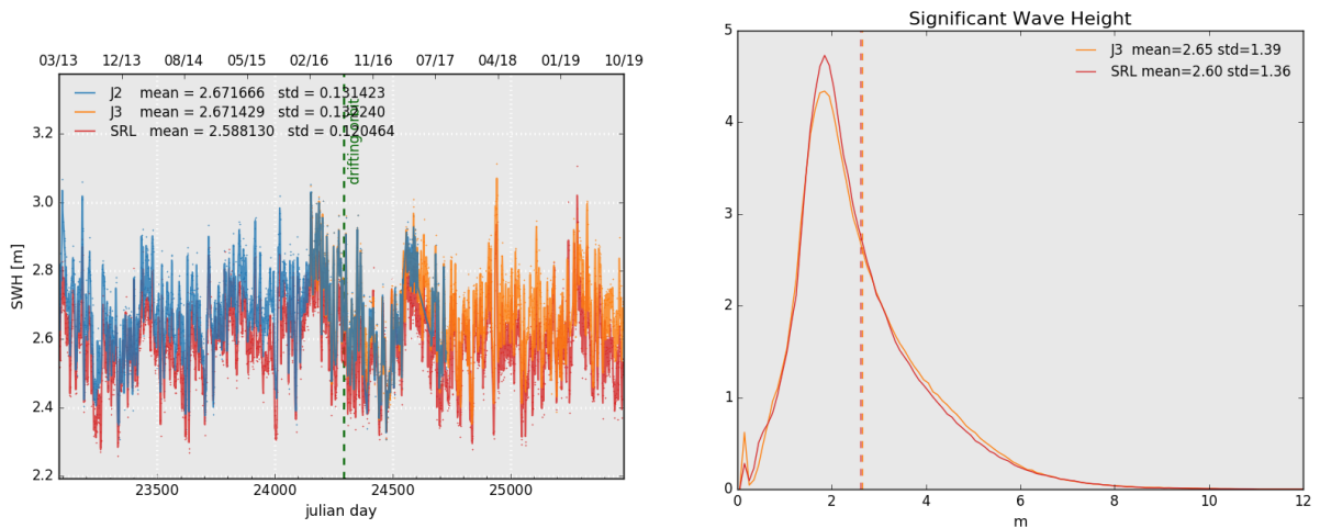
Figure 6: Daily monitoring of significant wave height for AltiKa (Ka-band) Jason-2 and Jason-3 (Ku-band) on the left and histogram for cycle 133 on the right (limited to 66° latitude).
