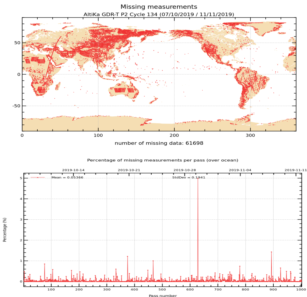
Figure 1: Map of missing measurements for cycle 134 on top. Monitoring of percentage of missing ocean measurements per pass on bottom.
