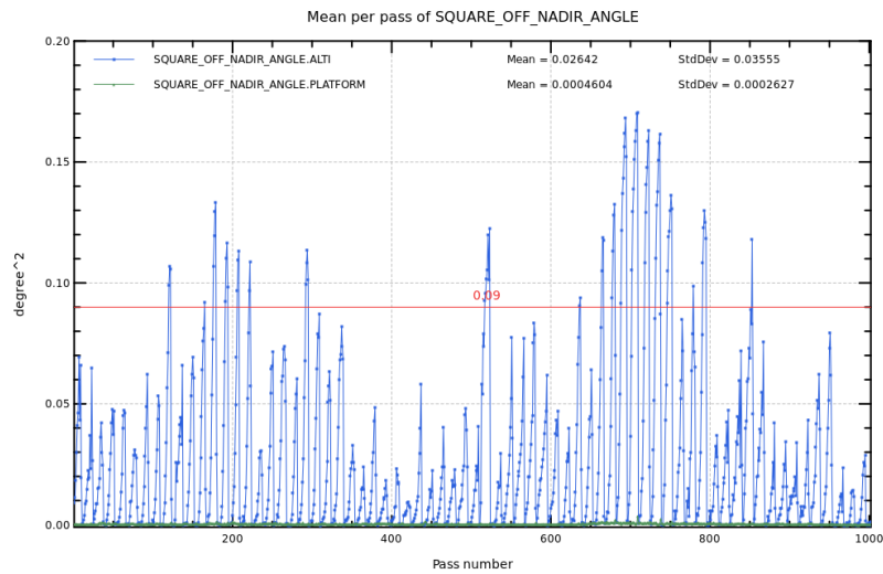
Figure 3: Mispointing cycle 134.
