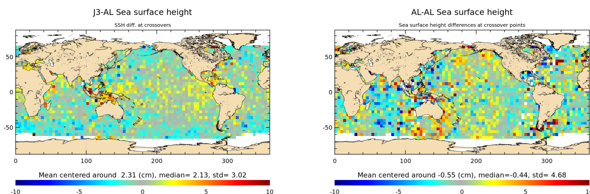
Figure 14: Mean of multi-mission SSH and mono-mission SSH differences at crossovers for cycle 134.
