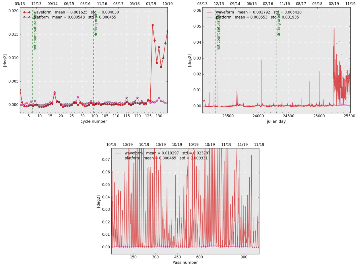
Figure 13: Cyclic monitoring(left), daily monitoring(right) and monitoring per pass for cycle 134 (bottom) of SARAL/AltiKa's mispointing angle: comparison between the one derived from waveform retracking and the one measured by platform startrackers.
