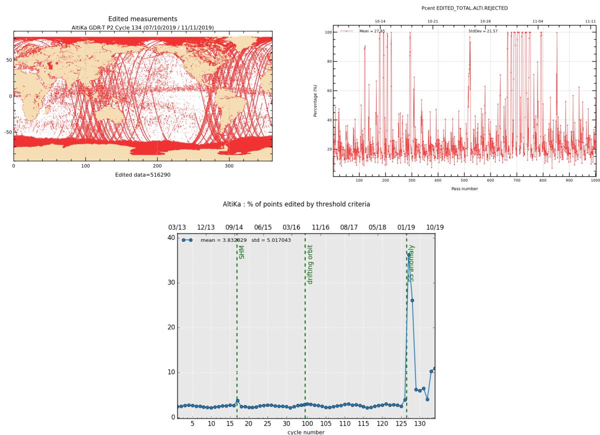
Figure 2: Rejected measurements on thresholds criteria : Cycle 134, map and monitoring of % of rejected measurements per track (top), whole time serie / % of rejected measurements per cycle (bottom).
