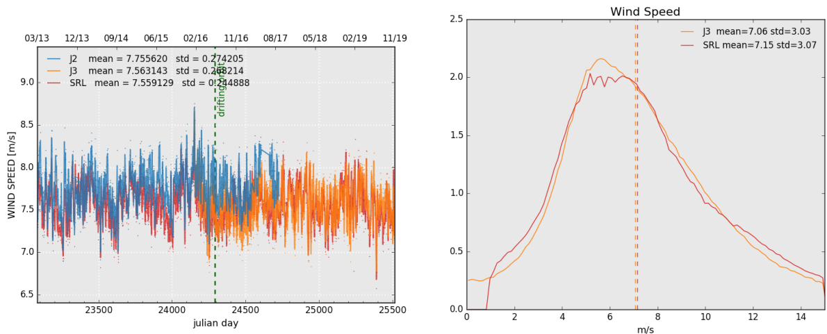
Figure 10: Daily monitoring of altimeter wind speed for Saral/AltiKa, Jason-2 and Jason-3 on the left and histogram for cycle 134 on the right (limited to 66° latitude).
