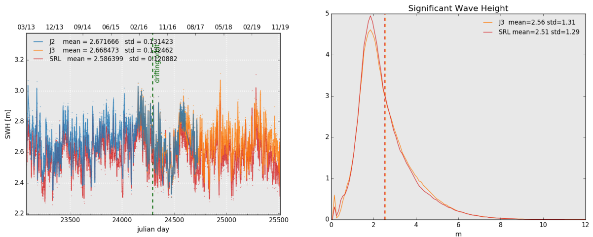
Figure 6: Daily monitoring of significant wave height for AltiKa (Ka-band) Jason-2 and Jason-3 (Ku-band) on the left and histogram for cycle 134 on the right (limited to 66° latitude).
