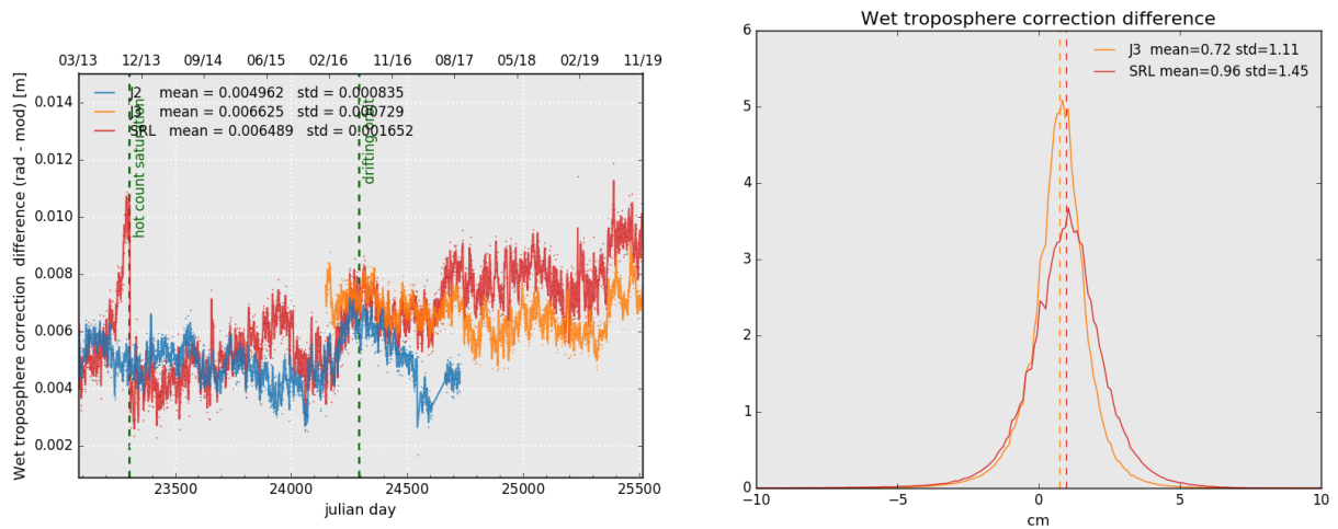
Figure 12: Daily monitoring of wet troposphere differences (Radiometer-ECMWF model) for Saral/AltiKa Jason-2 and Jason-3 (left) and histogram on the right (limited to 66° latitude) for cycle 134 .
