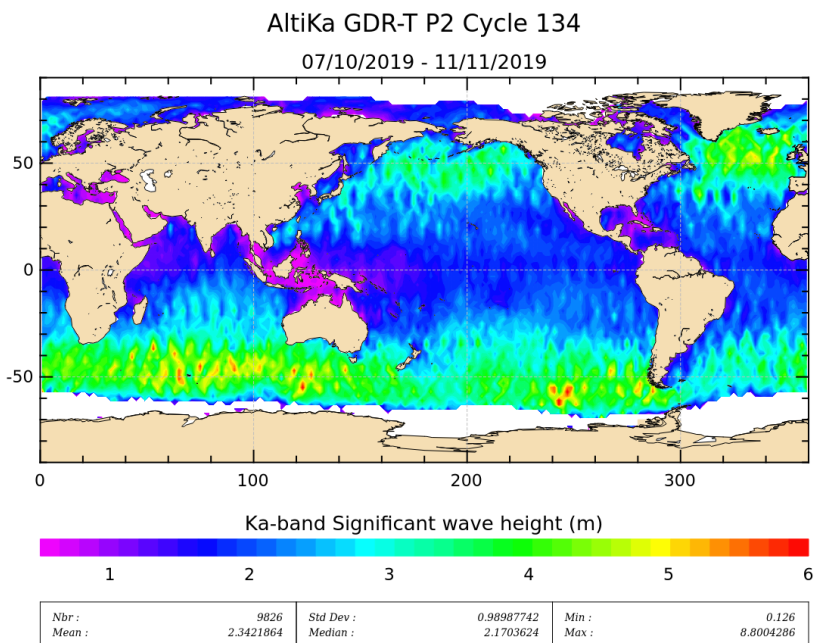
Figure 5: Significant wave height for cycle 134.
