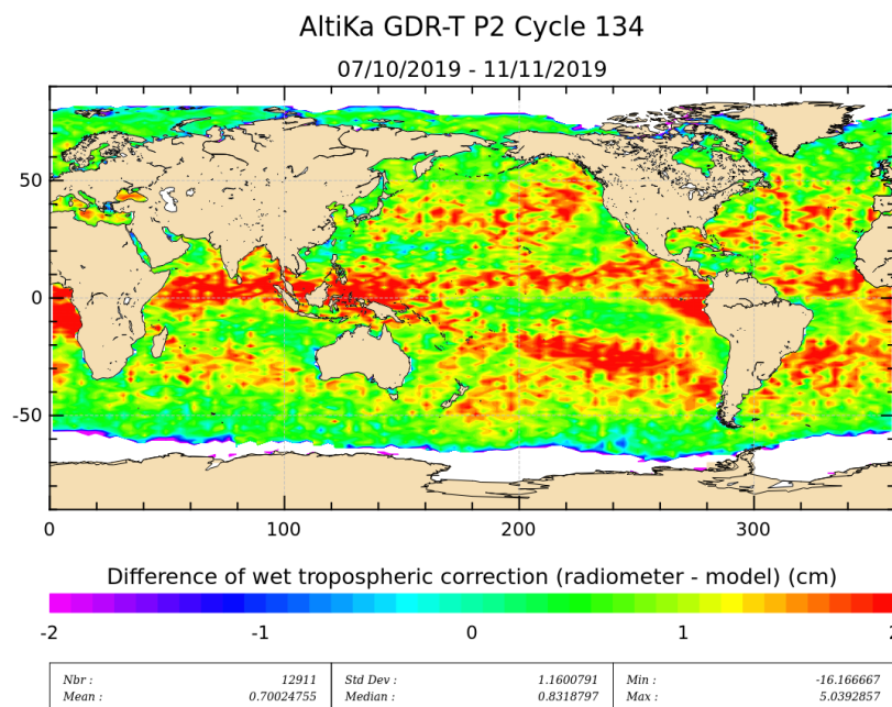
Figure 11: Mean of wet troposphere correction difference (Radiometer-ECMWF model) for cycle 134.
