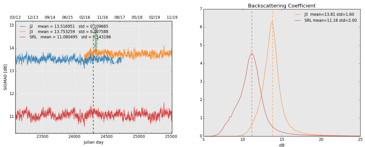
Figure 7: Daily monitoring of backscattering coefficient for Saral/AltiKa, Jason-2 and Jason-3 on the left and histogram for cycle 134 on the right (limited to 66° latitude).
