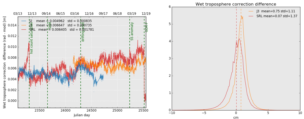
Figure 13: Daily monitoring of wet troposphere differences (Radiometer-ECMWF model) for Saral/AltiKa Jason-2 and Jason-3 (left) and histogram on the right (limited to 66° latitude) for cycle 135 .
