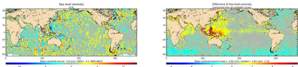
Figure 22: Jason-3 – Saral/AltiKa SLA differences for cycle 135 (left) and averaged over the whole Saral/AltiKa period (right).
