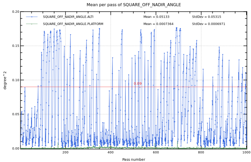
Figure 3: Mispointing cycle 135.
