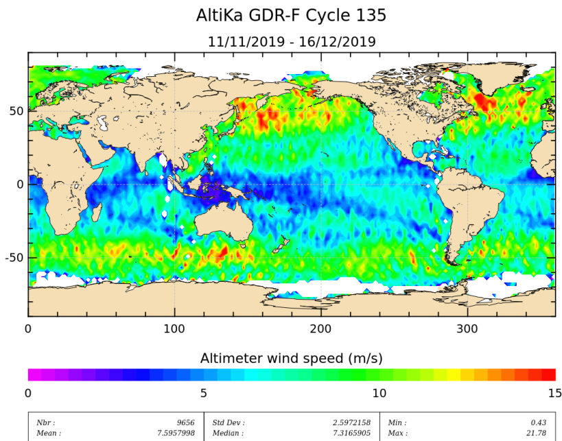
Figure 10: Altimeter wind speed for cycle 135.
