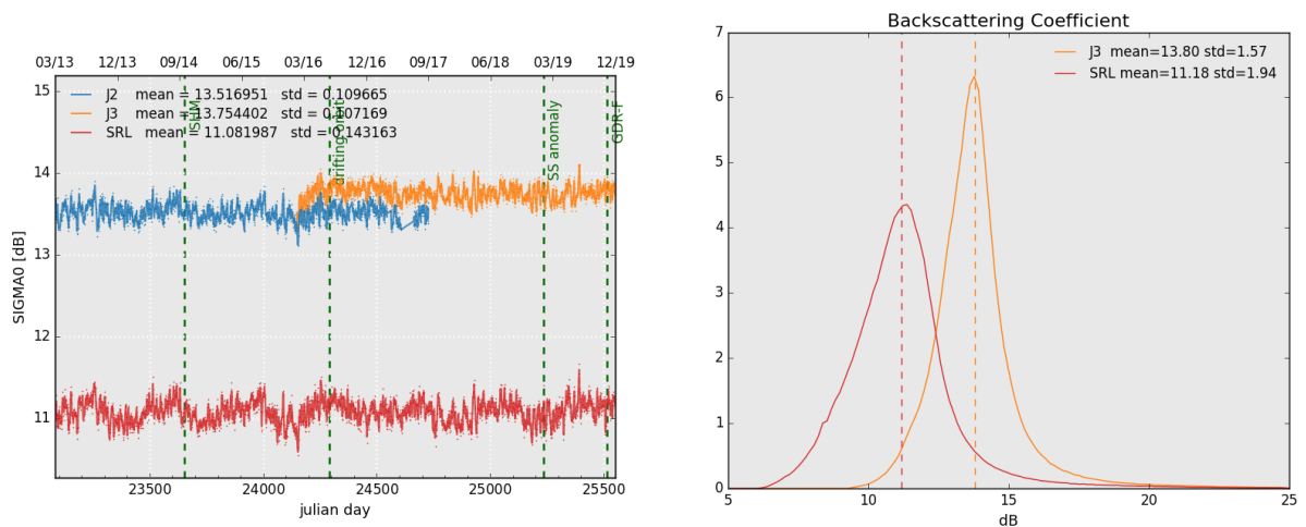
Figure 8: Daily monitoring of backscattering coefficient for Saral/AltiKa, Jason-2 and Jason-3 on the left and histogram for cycle 135 on the right (limited to 66° latitude).
