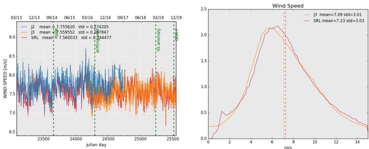
Figure 11: Daily monitoring of altimeter wind speed for Saral/AltiKa, Jason-2 and Jason-3 on the left and histogram for cycle 135 on the right (limited to 66° latitude).
