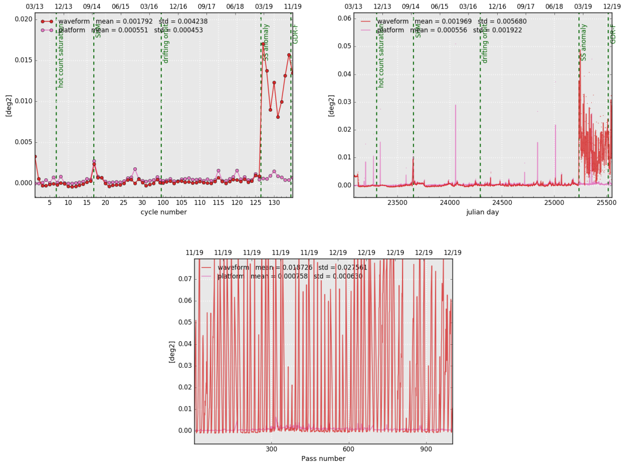
Figure 14: Cyclic monitoring(left), daily monitoring(right) and monitoring per pass for cycle 135 (bottom) of SARAL/AltiKa’s mispointing angle: comparison between the one derived from waveform retracking and the one measured by platform startrackers.
