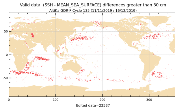
Figure 20: Sea level anomaly relative to MSS for cycle 135.
