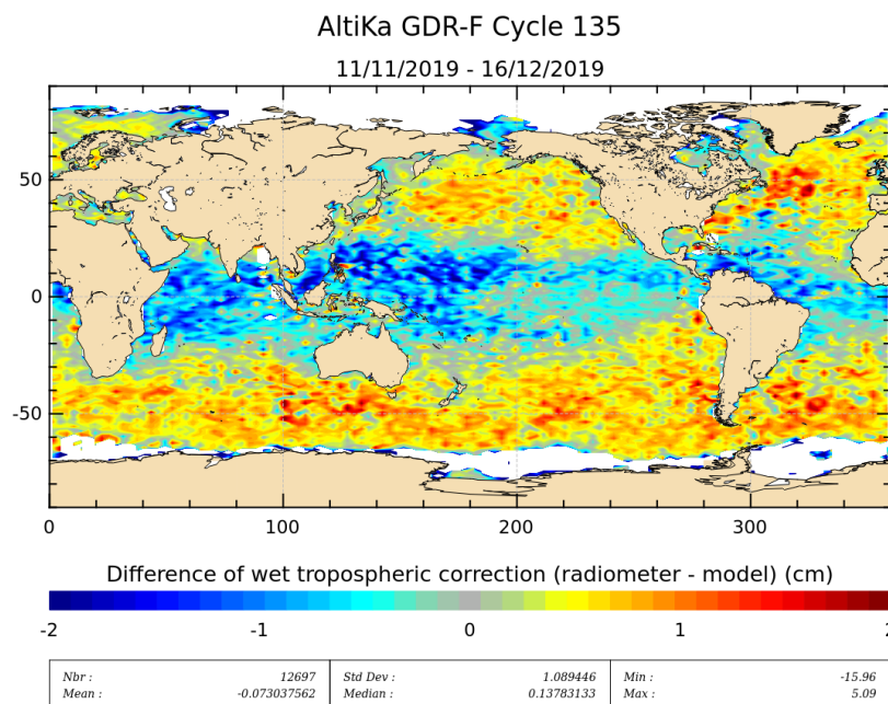
Figure 12: Mean of wet troposphere correction difference (Radiometer-ECMWF model) for cycle 135.
