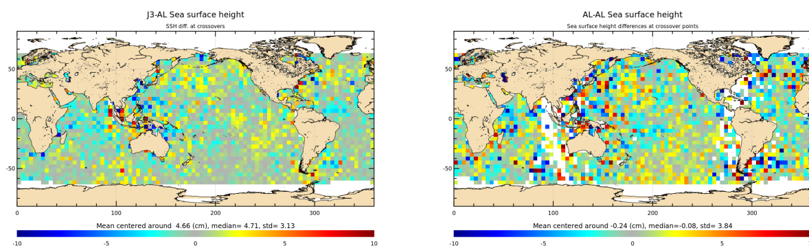
Figure 15: Mean of multi-mission SSH and mono-mission SSH differences at crossovers for cycle 135.
