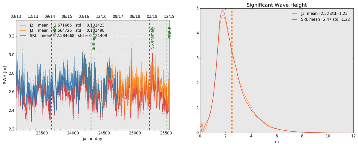
Figure 7: Daily monitoring of significant wave height for AltiKa (Ka-band) Jason-2 and Jason-3 (Ku-band) on the left and histogram for cycle 135 on the right (limited to 66° latitude).
