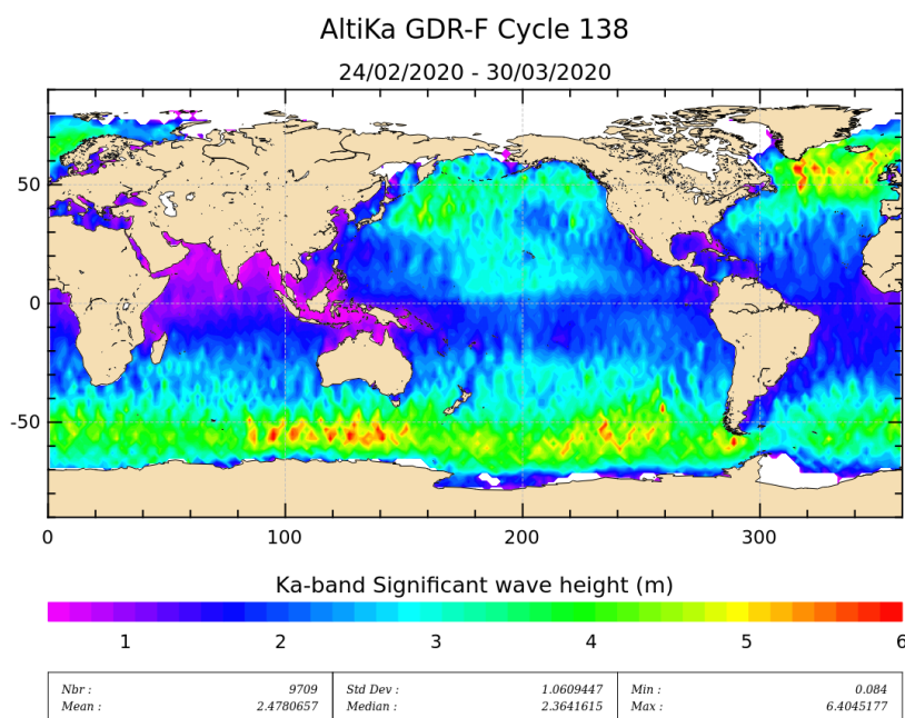
Figure 5: Significant wave height for cycle 138.
