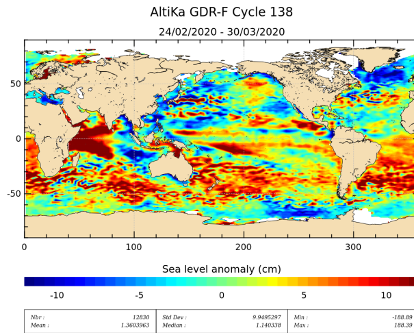
Figure 19: Sea level anomaly relative to MSS for cycle 138.
