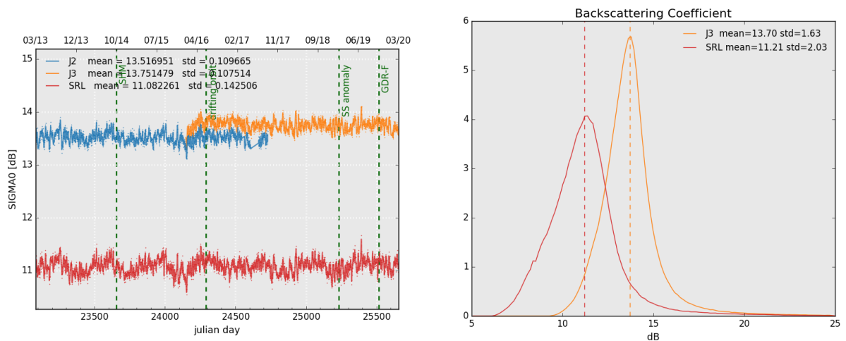
Figure 7: Daily monitoring of backscattering coefficient for Saral/AltiKa, Jason-2 and Jason-3 on the left and histogram for cycle 138 on the right (limited to 66° latitude).
