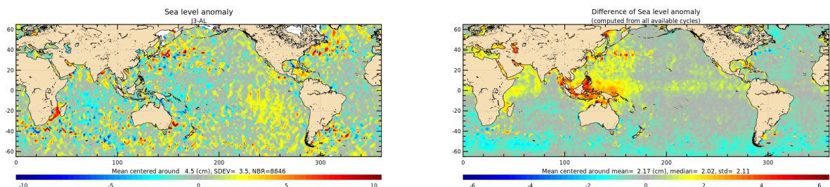
Figure 21: Jason-3 – Saral/AltiKa SLA differences for cycle 138 (left) and averaged over the whole Saral/AltiKa period (right).
