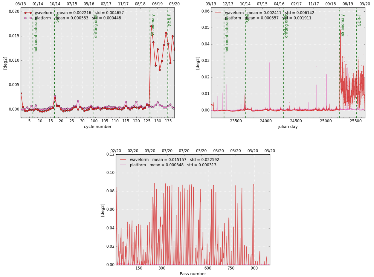
Figure 13: Cyclic monitoring(left), daily monitoring(right) and monitoring per pass for cycle 138 (bottom) of SARAL/AltiKa’s mispointing angle: comparison between the one derived from waveform retracking and the one measured by platform startrackers.
