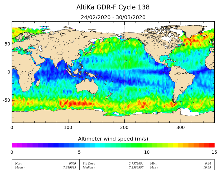
Figure 9: Altimeter wind speed for cycle 138.
