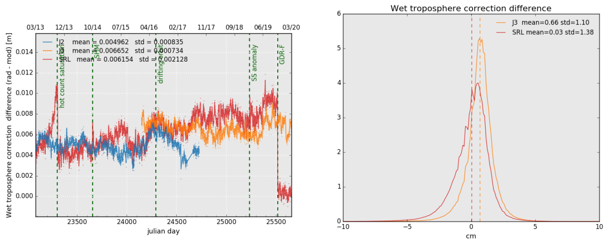
Figure 12: Daily monitoring of wet troposphere differences (Radiometer-ECMWF model) for Saral/AltiKa Jason-2 and Jason-3 (left) and histogram on the right (limited to 66° latitude) for cycle 138 .
