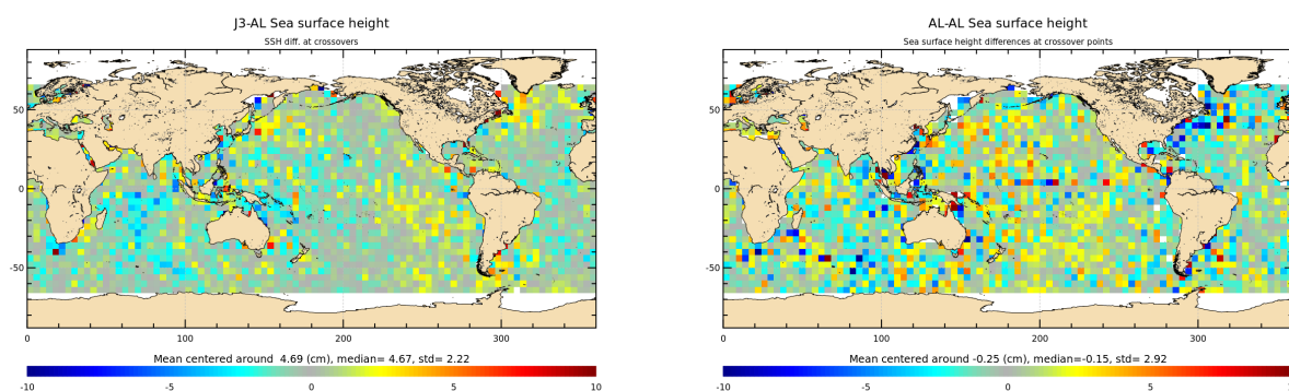
Figure 14: Mean of multi-mission SSH and mono-mission SSH differences at crossovers for cycle 138.
