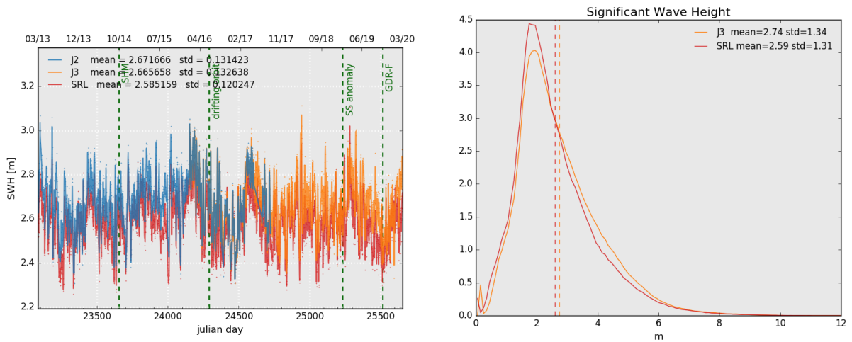
Figure 6: Daily monitoring of significant wave height for AltiKa (Ka-band) Jason-2 and Jason-3 (Ku-band) on the left and histogram for cycle 138 on the right (limited to 66° latitude).
