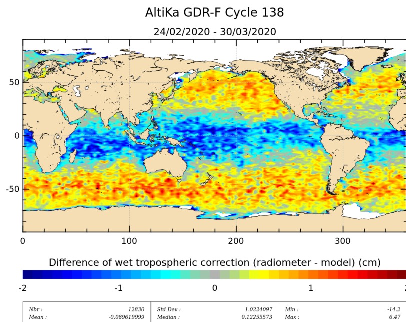
Figure 11: Mean of wet troposphere correction difference (Radiometer-ECMWF model) for cycle 138.
