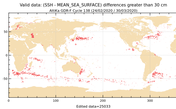
Figure 19: Sea level anomaly relative to MSS for cycle 138.
