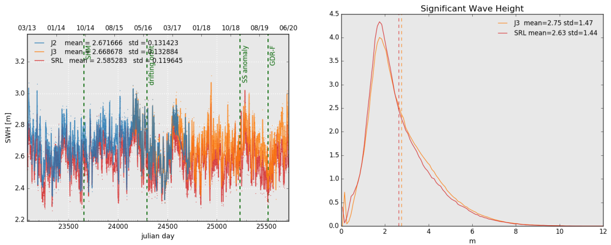
Figure 6: Daily monitoring of significant wave height for AltiKa (Ka-band) Jason-2 and Jason-3 (Ku-band) on the left and histogram for cycle 140 on the right (limited to 66° latitude).
