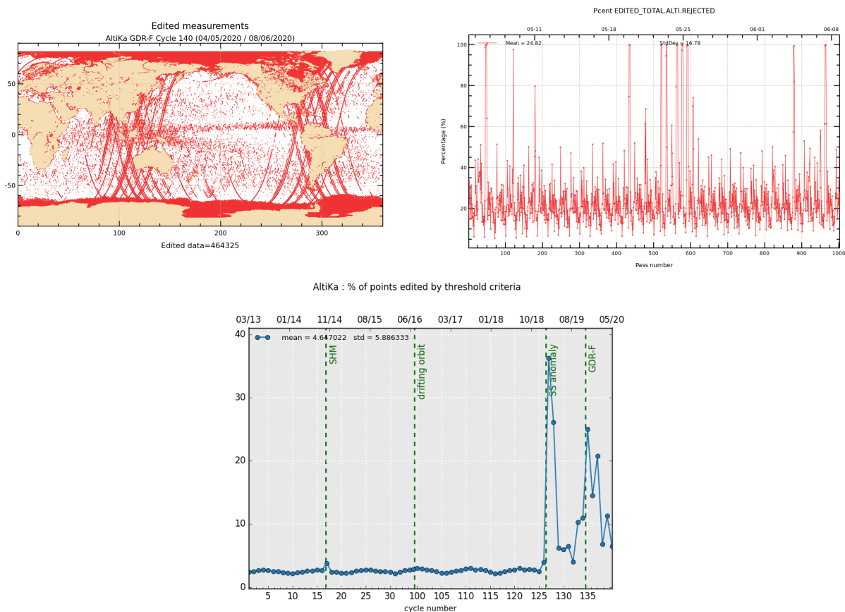
Figure 2: Rejected measurements on thresholds criteria : Cycle 140, map and monitoring of % of rejected measurements per track (top), whole time serie / % of rejected measurements per cycle (bottom).
