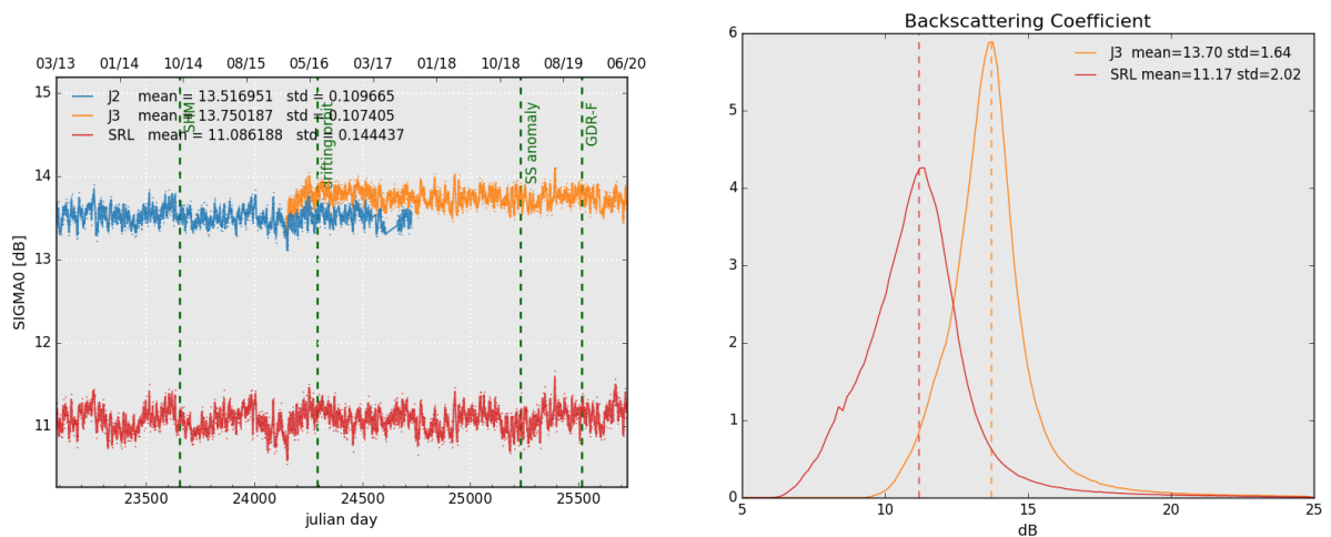
Figure 7: Daily monitoring of backscattering coefficient for Saral/AltiKa, Jason-2 and Jason-3 on the left and histogram for cycle 140 on the right (limited to 66° latitude).
