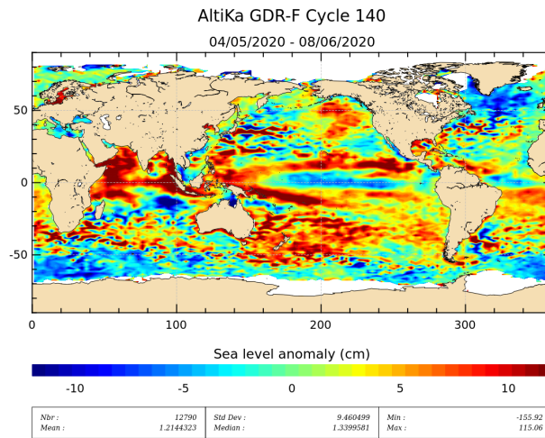
Figure 19: Sea level anomaly relative to MSS for cycle 140.
