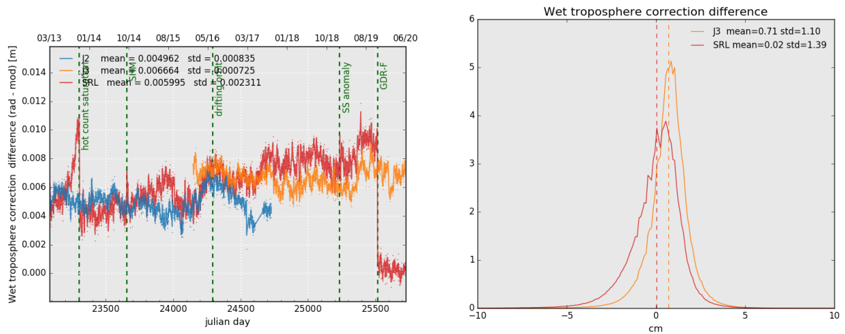
Figure 12: Daily monitoring of wet troposphere differences (Radiometer-ECMWF model) for Saral/AltiKa Jason-2 and Jason-3 (left) and histogram on the right (limited to 66° latitude) for cycle 140 .
