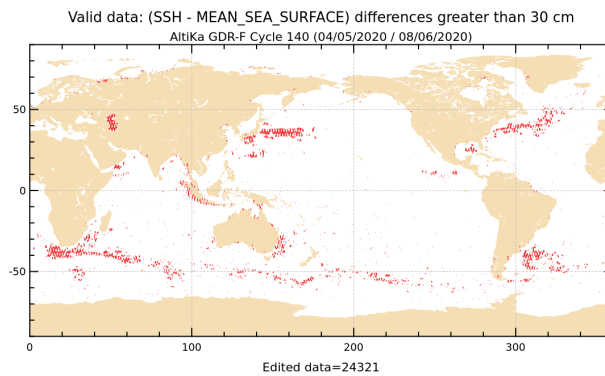
Figure 19: Sea level anomaly relative to MSS for cycle 140.
