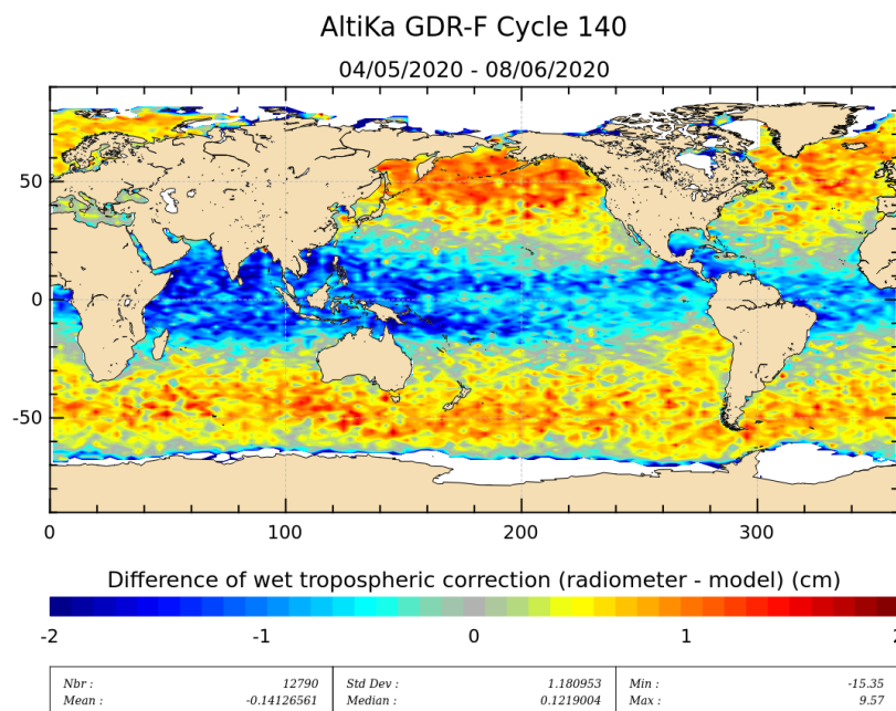
Figure 11: Mean of wet troposphere correction difference (Radiometer-ECMWF model) for cycle 140.
