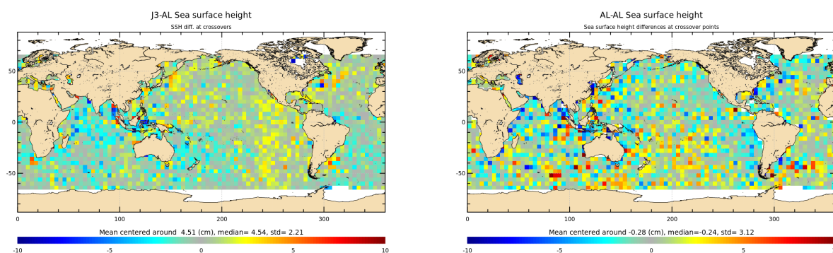
Figure 14: Mean of multi-mission SSH and mono-mission SSH differences at crossovers for cycle 140.
