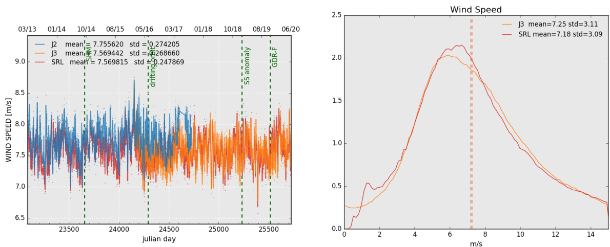
Figure 10: Daily monitoring of altimeter wind speed for Saral/AltiKa, Jason-2 and Jason-3 on the left and histogram for cycle 140 on the right (limited to 66° latitude).
