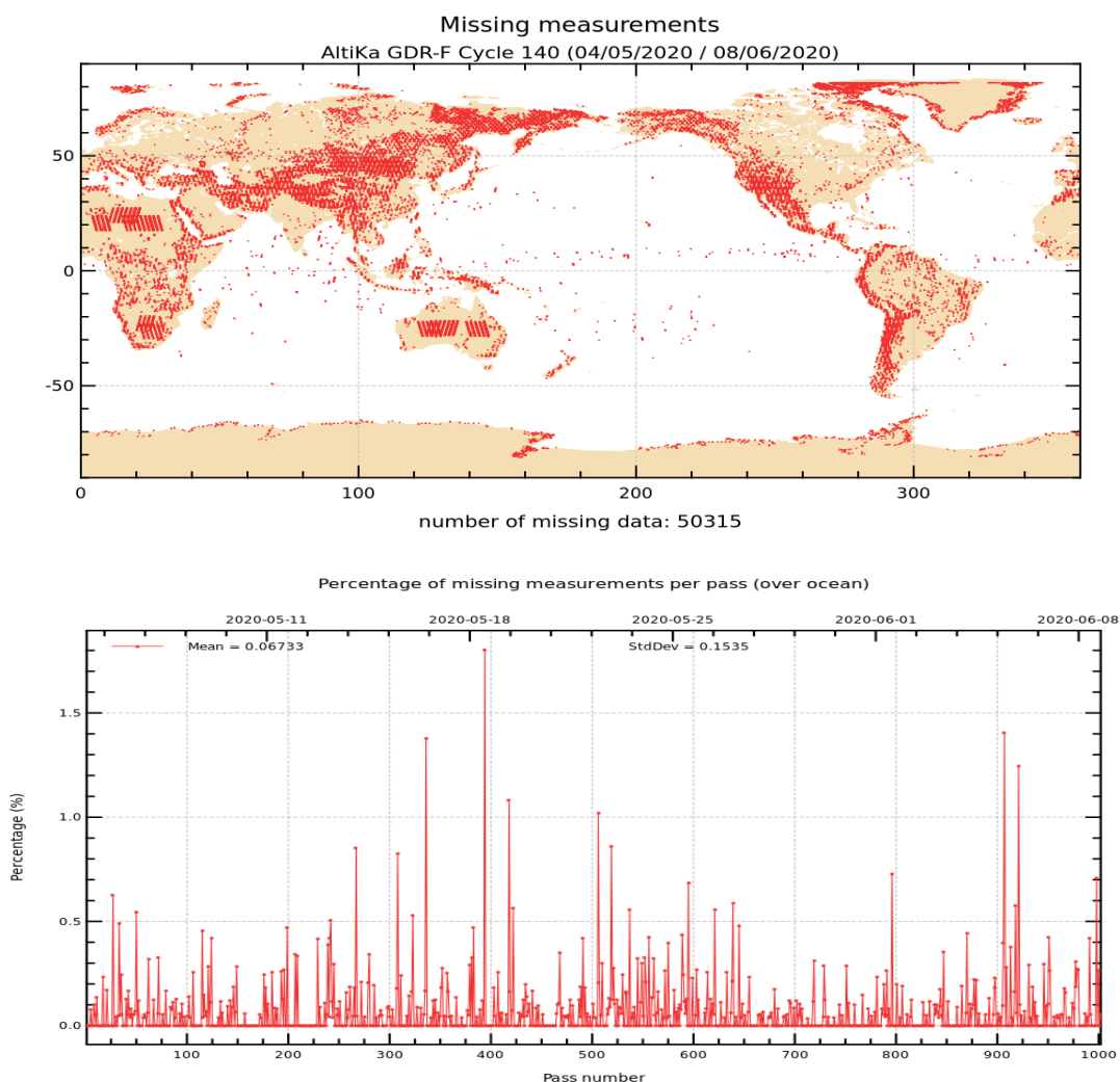
Figure 1: Map of missing measurements for cycle 140 on top. Monitoring of percentage of missing ocean measurements per pass on bottom.
