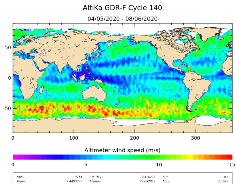
Figure 9: Altimeter wind speed for cycle 140.
