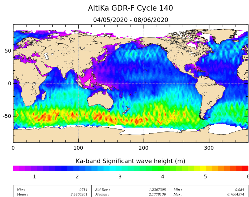
Figure 5: Significant wave height for cycle 140.
