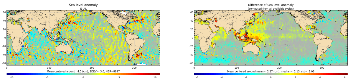
Figure 21: Jason-3 – Saral/AltiKa SLA differences for cycle 140 (left) and averaged over the whole Saral/AltiKa period (right).
