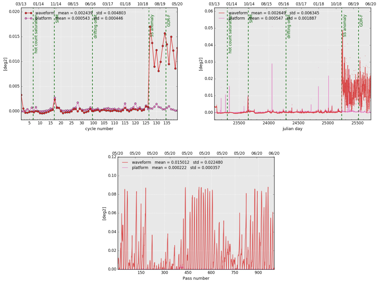
Figure 13: Cyclic monitoring(left), daily monitoring(right) and monitoring per pass for cycle 140 (bottom) of SARAL/AltiKa's mispointing angle: comparison between the one derived from waveform retracking and the one measured by platform startrackers.
