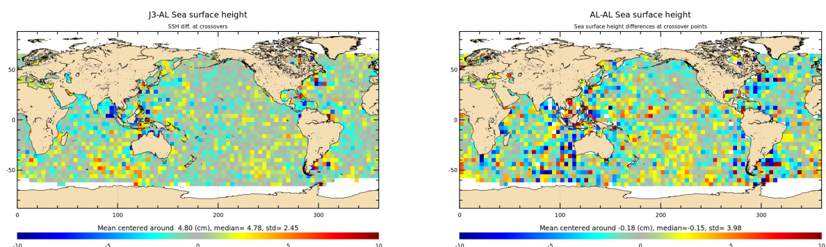
Figure 14: Mean of multi-mission SSH and mono-mission SSH differences at crossovers for cycle 142.
