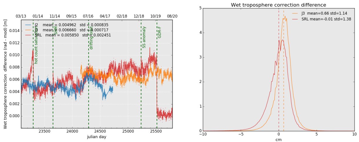
Figure 12: Daily monitoring of wet troposphere differences (Radiometer-ECMWF model) for Saral/AltiKa Jason-2 and Jason-3 (left) and histogram on the right (limited to 66° latitude) for cycle 142 .
