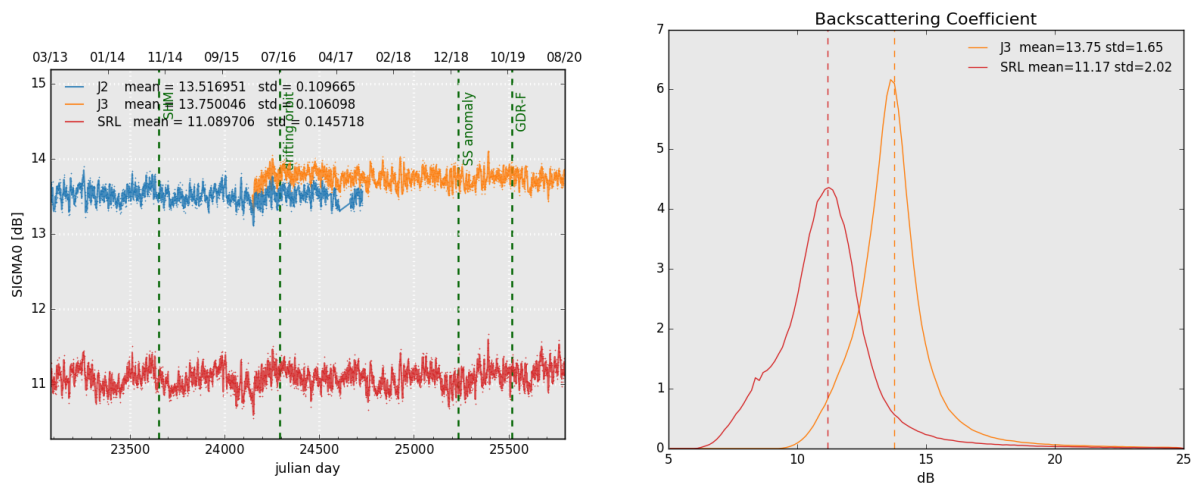
Figure 7: Daily monitoring of backscattering coefficient for Saral/AltiKa, Jason-2 and Jason-3 on the left and histogram for cycle 142 on the right (limited to 66° latitude).
