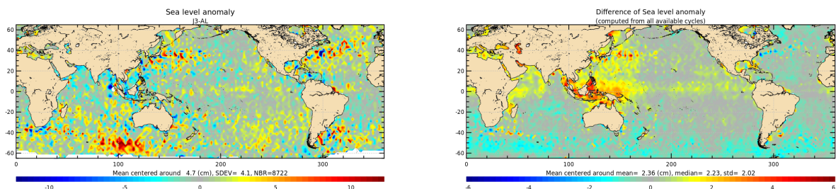
Figure 21: Jason-3 – Saral/AltiKa SLA differences for cycle 142 (left) and averaged over the whole Saral/AltiKa period (right).
