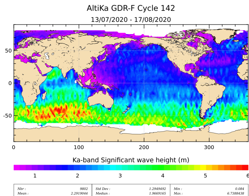
Figure 5: Significant wave height for cycle 142.
