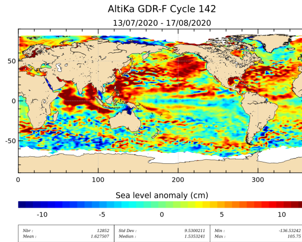
Figure 19: Sea level anomaly relative to MSS for cycle 142.
