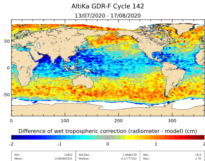
Figure 11: Mean of wet troposphere correction difference (Radiometer-ECMWF model) for cycle 142.
