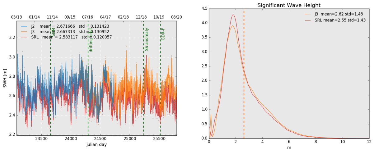
Figure 6: Daily monitoring of significant wave height for AltiKa (Ka-band) Jason-2 and Jason-3 (Ku-band) on the left and histogram for cycle 142 on the right (limited to 66° latitude).
