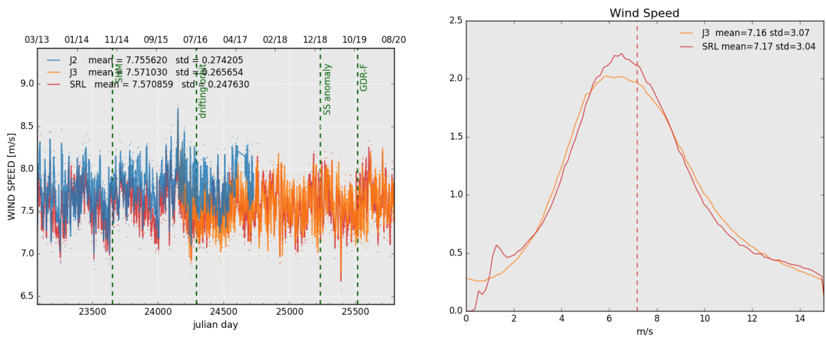
Figure 10: Daily monitoring of altimeter wind speed for Saral/AltiKa, Jason-2 and Jason-3 on the left and histogram for cycle 142 on the right (limited to 66° latitude).
