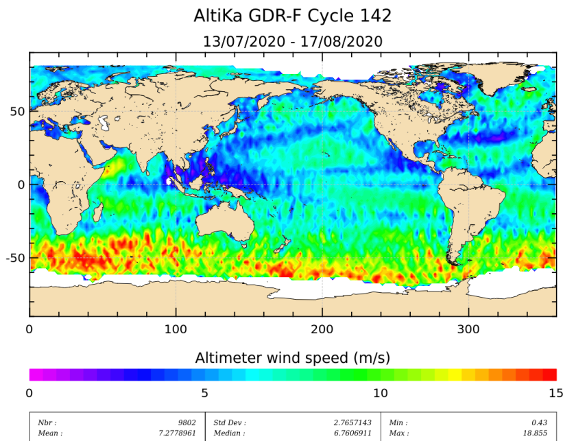
Figure 9: Altimeter wind speed for cycle 142.
