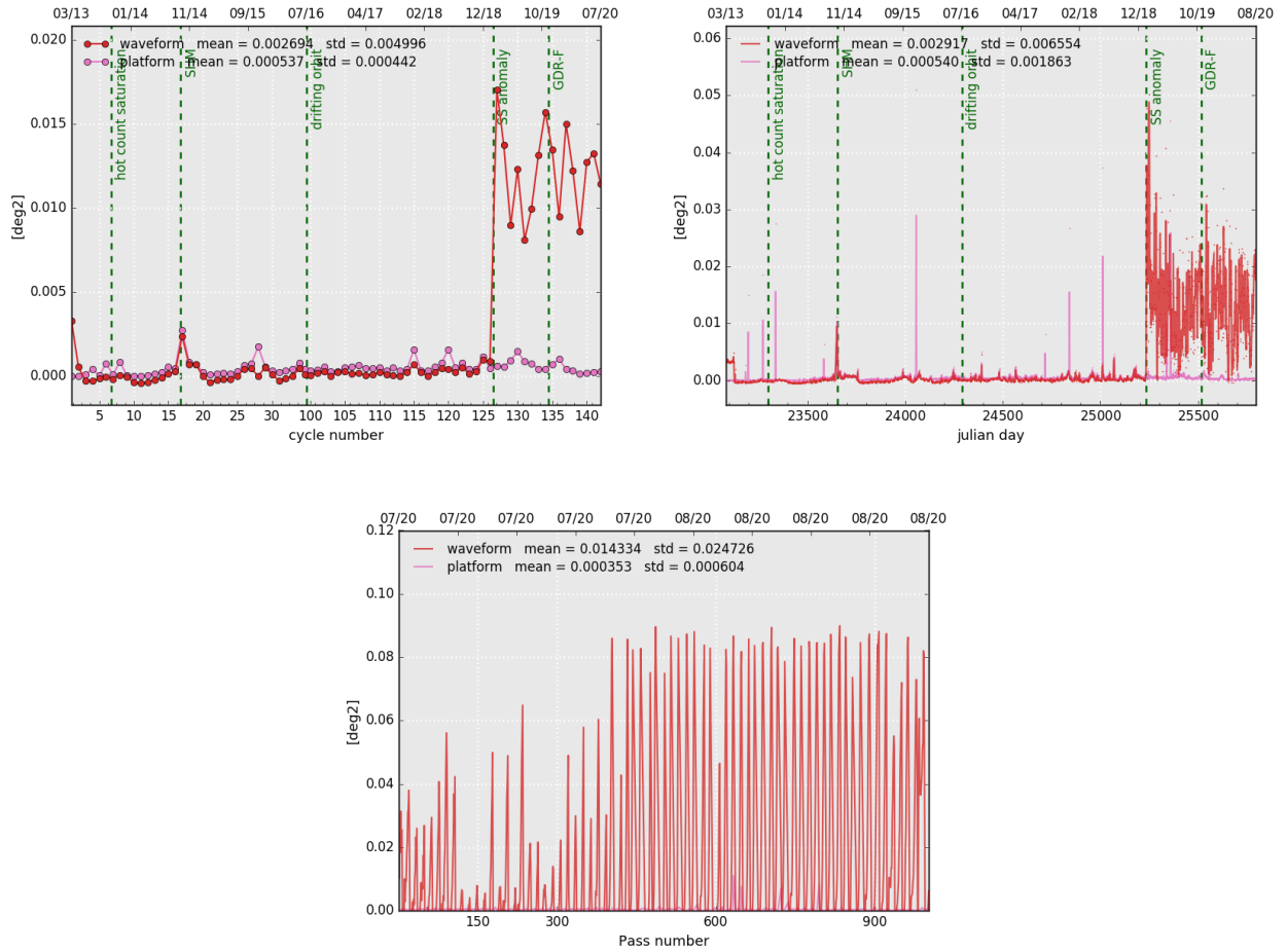
Figure 13: Cyclic monitoring(left), daily monitoring(right) and monitoring per pass for cycle 142 (bottom) of SARAL/AltiKa's mispointing angle: comparison between the one derived from waveform retracking and the one measured by platform startrackers.
