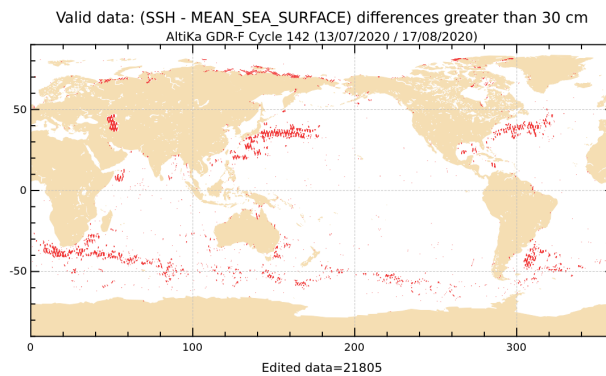
Figure 19: Sea level anomaly relative to MSS for cycle 142.
