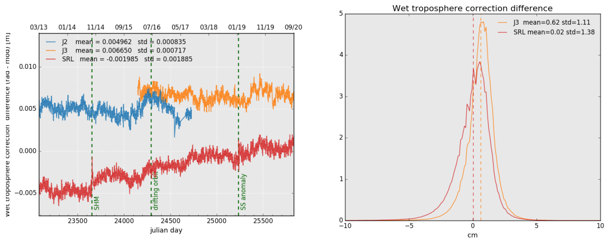
Figure 12: Daily monitoring of wet troposphere differences (Radiometer-ECMWF model) for Saral/AltiKa Jason-2 and Jason-3 (left) and histogram on the right (limited to 66° latitude) for cycle 143 .
