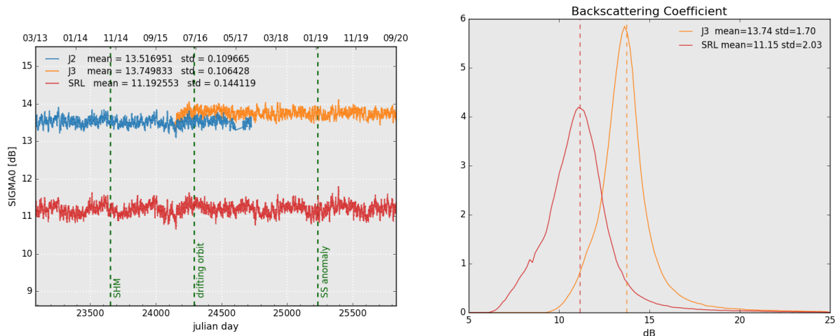
Figure 7: Daily monitoring of backscattering coefficient for Saral/AltiKa, Jason-2 and Jason-3 on the left and histogram for cycle 143 on the right (limited to 66° latitude).
