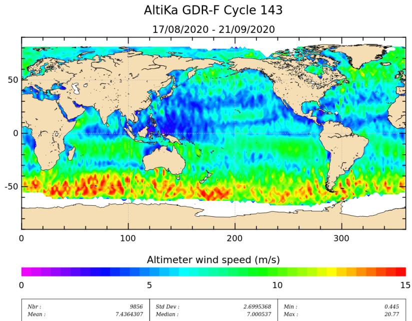
Figure 9: Altimeter wind speed for cycle 143.
