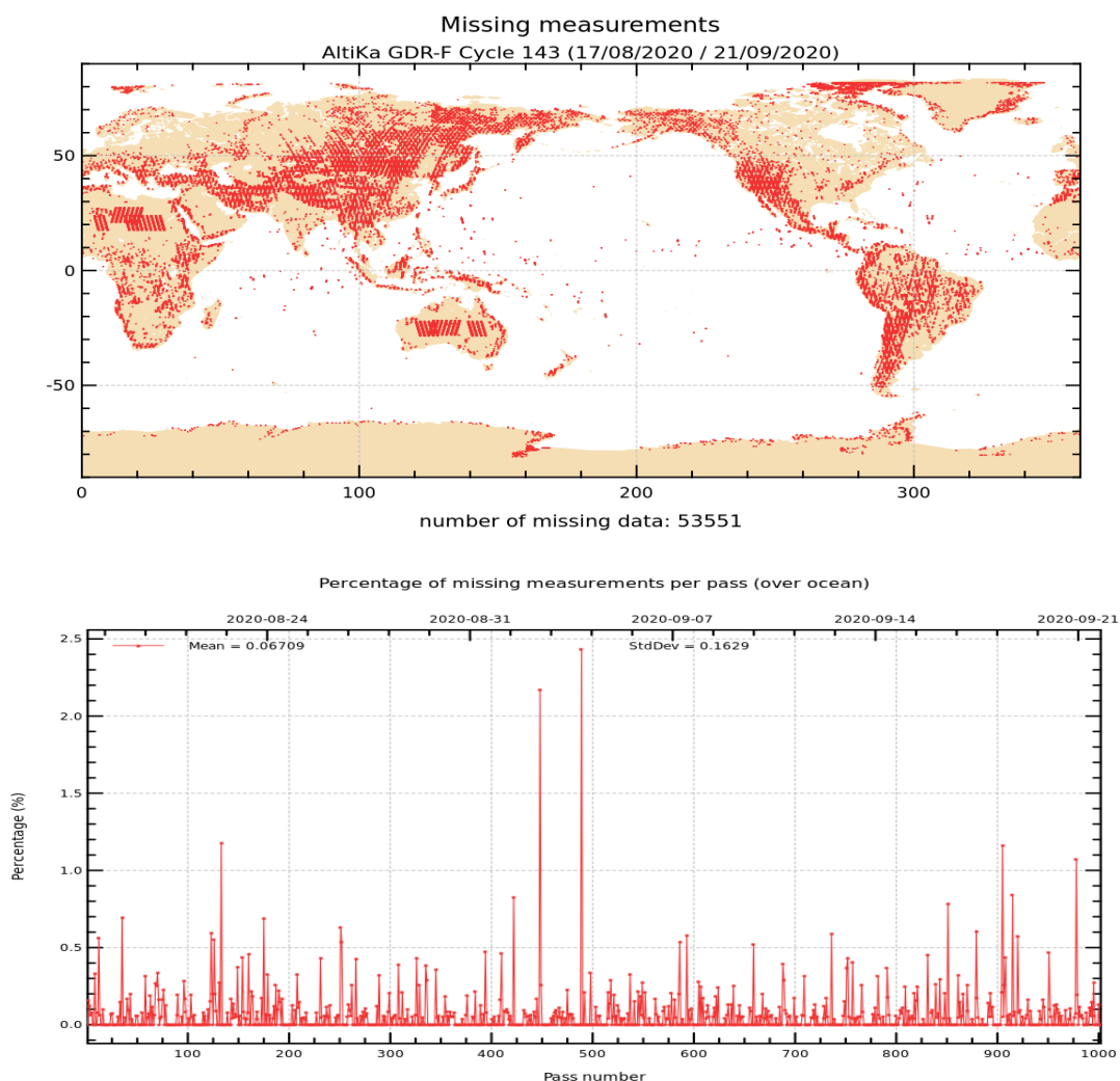
Figure 1: Map of missing measurements for cycle 143 on top. Monitoring of percentage of missing ocean measurements per pass on bottom.
