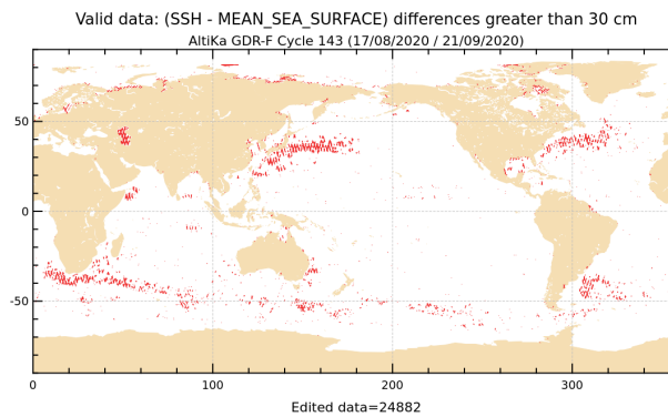
Figure 19: Sea level anomaly relative to MSS for cycle 143.
