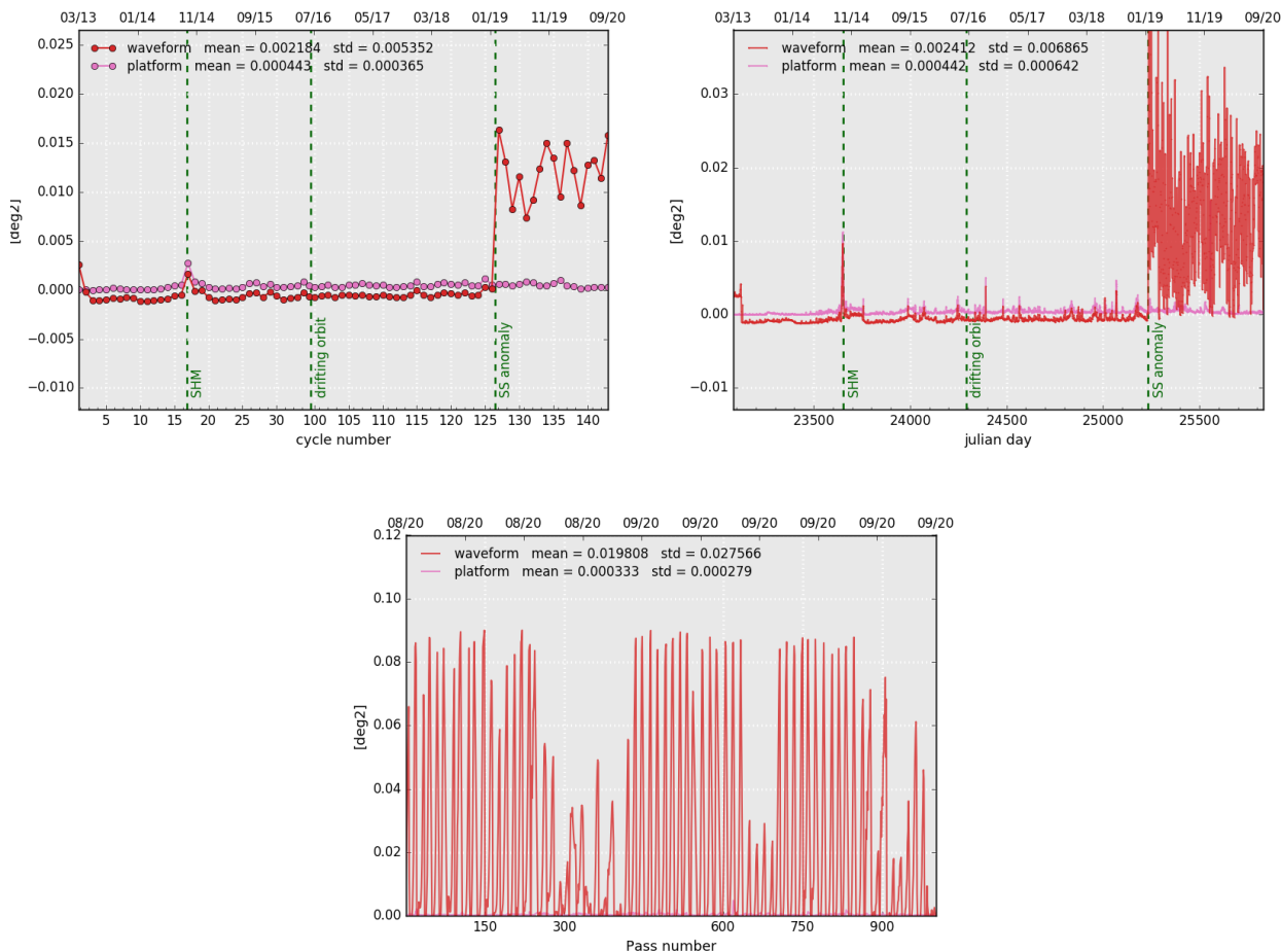
Figure 13: Cyclic monitoring(left), daily monitoring(right) and monitoring per pass for cycle 143 (bottom) of SARAL/AltiKa's mispointing angle: comparison between the one derived from waveform retracking and the one measured by platform startrackers.
