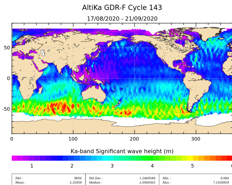
Figure 5: Significant wave height for cycle 143.
