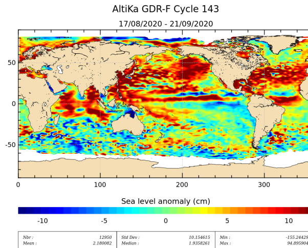
Figure 19: Sea level anomaly relative to MSS for cycle 143.
