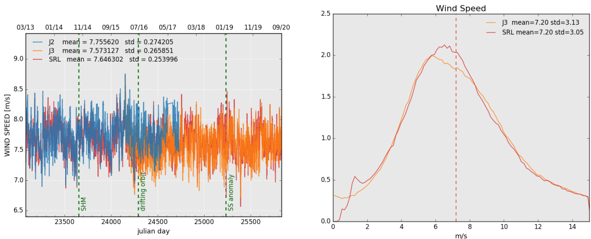
Figure 10: Daily monitoring of altimeter wind speed for Saral/AltiKa, Jason-2 and Jason-3 on the left and histogram for cycle 143 on the right (limited to 66° latitude).
