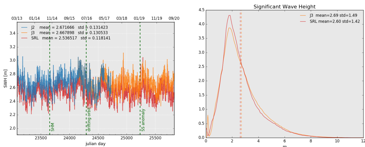
Figure 6: Daily monitoring of significant wave height for AltiKa (Ka-band) Jason-2 and Jason-3 (Ku-band) on the left and histogram for cycle 143 on the right (limited to 66^\circ latitude).
