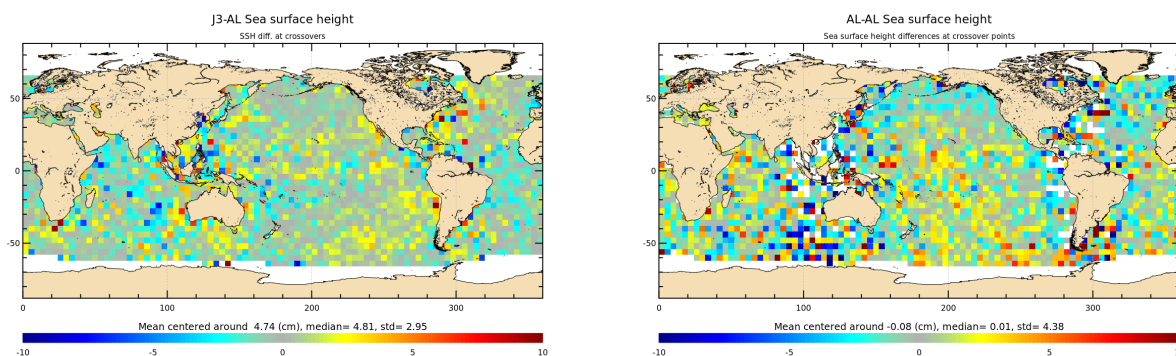
Figure 14: Mean of multi-mission SSH and mono-mission SSH differences at crossovers for cycle 143.
