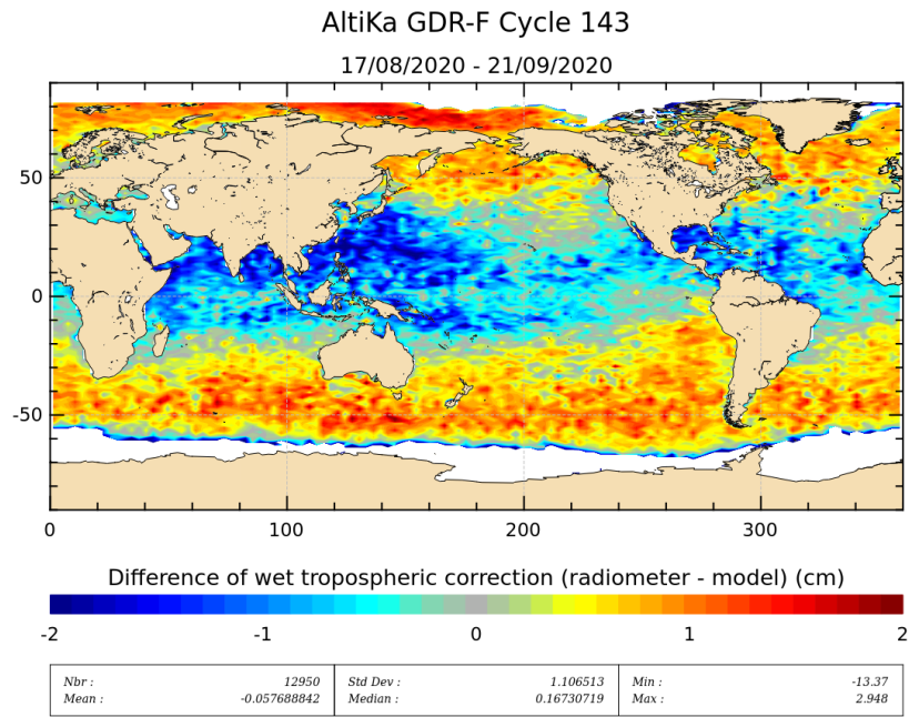
Figure 11: Mean of wet troposphere correction difference (Radiometer-ECMWF model) for cycle 143.
