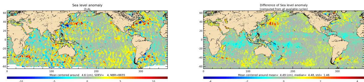
Figure 21: Jason-3 – Saral/AltiKa SLA differences for cycle 143 (left) and averaged over the whole Saral/AltiKa period (right).
