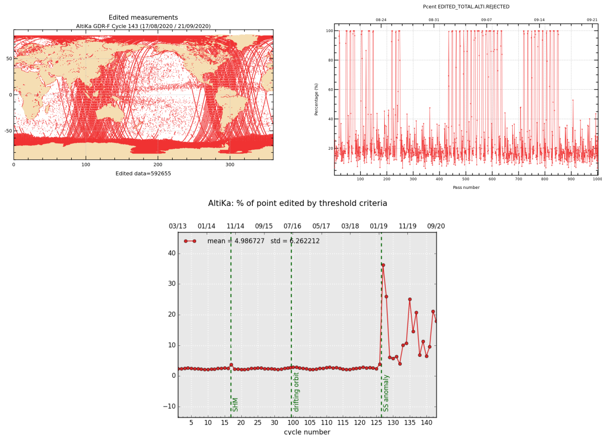
Figure 2: Rejected measurements on thresholds criteria : Cycle 143, map and monitoring of % of rejected measurements per track (top), whole time serie / % of rejected measurements per cycle (bottom).
