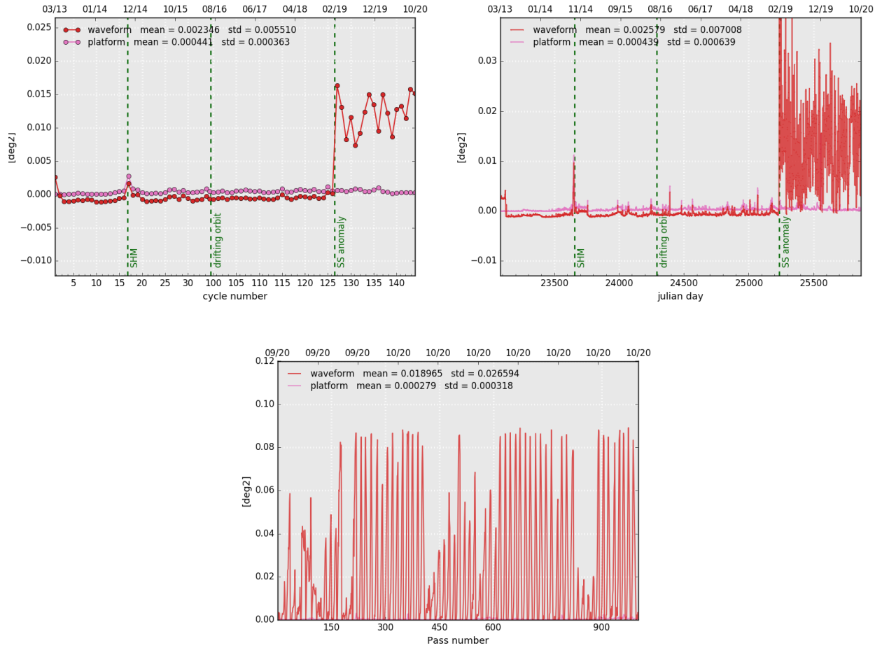
Figure 13: Cyclic monitoring(left), daily monitoring(right) and monitoring per pass for cycle 144 (bottom) of SARAL/AltiKa's mispointing angle: comparison between the one derived from waveform retracking and the one measured by platform startrackers.
