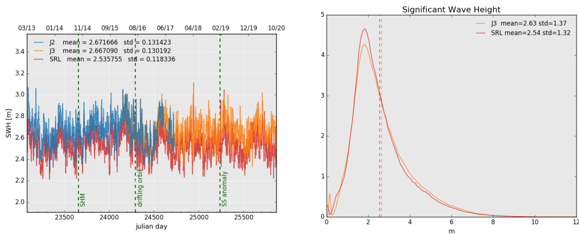
Figure 6: Daily monitoring of significant wave height for AltiKa (Ka-band) Jason-2 and Jason-3 (Ku-band) on the left and histogram for cycle 144 on the right (limited to 66^\circ latitude).
