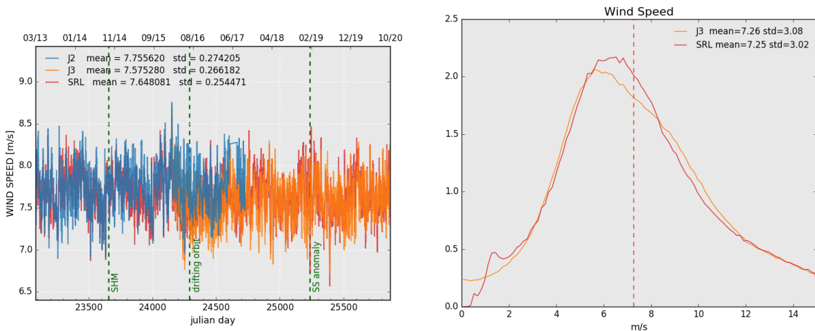
Figure 10: Daily monitoring of altimeter wind speed for Saral/AltiKa, Jason-2 and Jason-3 on the left and histogram for cycle 144 on the right (limited to 66° latitude).
