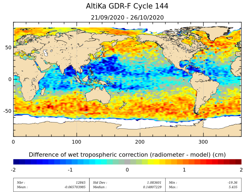
Figure 11: Mean of wet troposphere correction difference (Radiometer-ECMWF model) for cycle 144.
