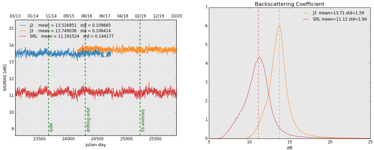
Figure 7: Daily monitoring of backscattering coefficient for Saral/AltiKa, Jason-2 and Jason-3 on the left and histogram for cycle 144 on the right (limited to 66° latitude).
