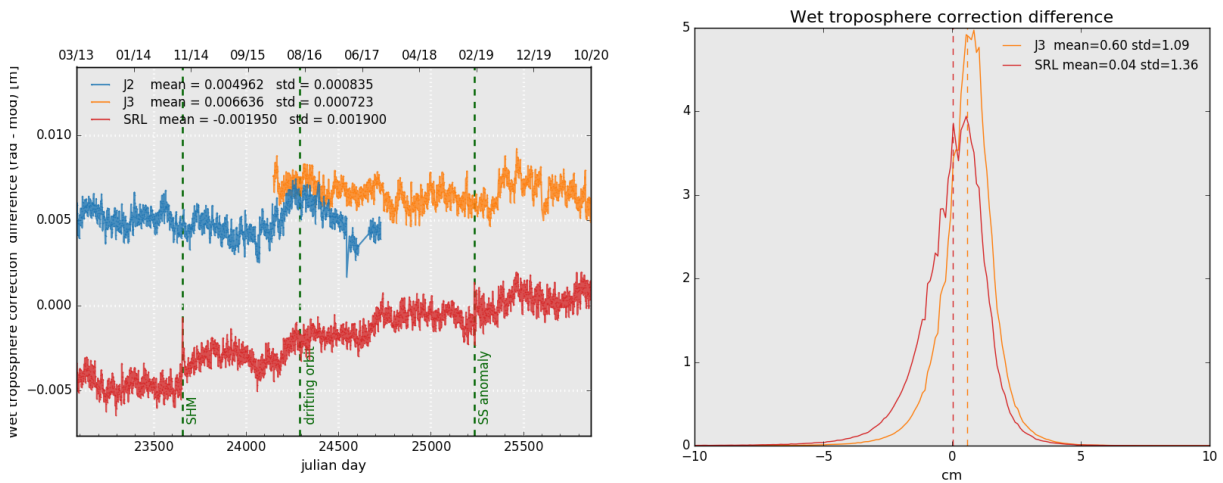
Figure 12: Daily monitoring of wet troposphere differences (Radiometer-ECMWF model) for Saral/AltiKa Jason-2 and Jason-3 (left) and histogram on the right (limited to 66° latitude) for cycle 144 .
