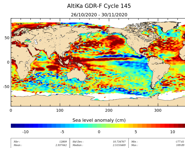
Figure 20: Sea level anomaly relative to MSS for cycle 145.
