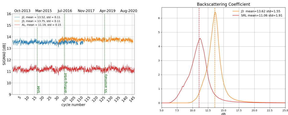
Figure 8: Daily monitoring of backscattering coefficient for Saral/AltiKa, Jason-2 and Jason-3 on the left and histogram for cycle 145 on the right (limited to 66° latitude).
