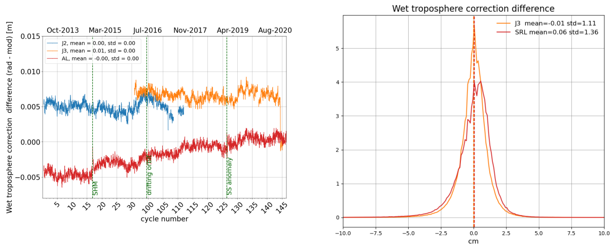
Figure 13: Daily monitoring of wet troposphere differences (Radiometer-ECMWF model) for Saral/AltiKa Jason-2 and Jason-3 (left) and histogram on the right (limited to 66° latitude) for cycle 145 .
