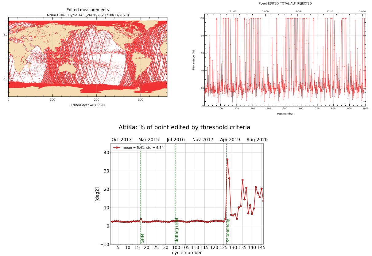
Figure 2: Rejected measurements on thresholds criteria : Cycle 145, map and monitoring of % of rejected measurements per track (top), whole time serie / % of rejected measurements per cycle (bottom).
