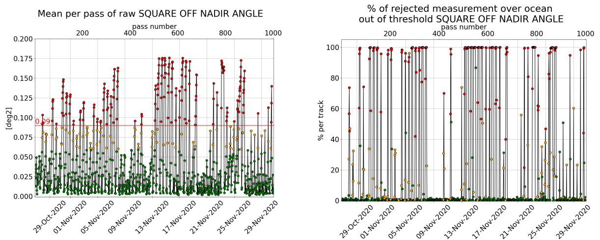
Figure 3: [left] Mispointing cycle 145, [right] Percentage of rejected measurement by threshold on square off-nadir angle.
