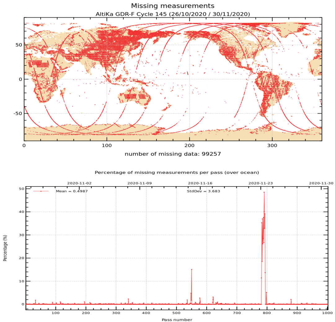
Figure 1: Map of missing measurements for cycle 145 on top. Monitoring of percentage of missing ocean measurements per pass on bottom.
