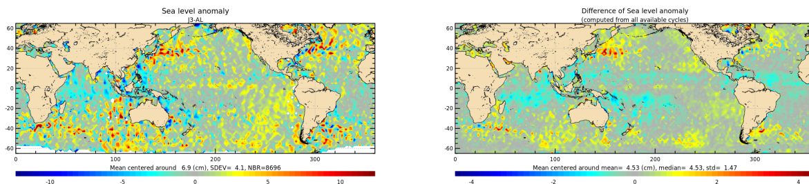
Figure 22: Jason-3 – Saral/AltiKa SLA differences for cycle 145 (left) and averaged over the whole Saral/AltiKa period (right).
