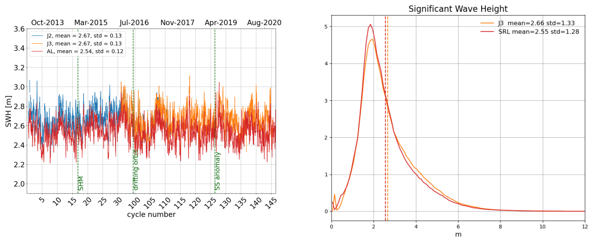
Figure 7: Daily monitoring of significant wave height for AltiKa (Ka-band) Jason-2 and Jason-3 (Ku-band) on the left and histogram for cycle 145 on the right (limited to 66° latitude).
