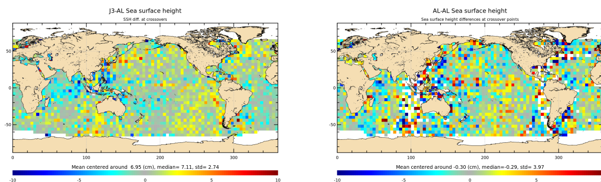
Figure 15: Mean of multi-mission SSH and mono-mission SSH differences at crossovers for cycle 145.
