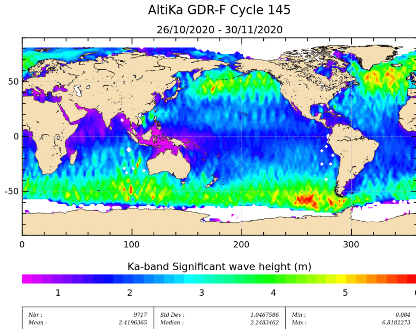
Figure 6: Significant wave height for cycle 145.
