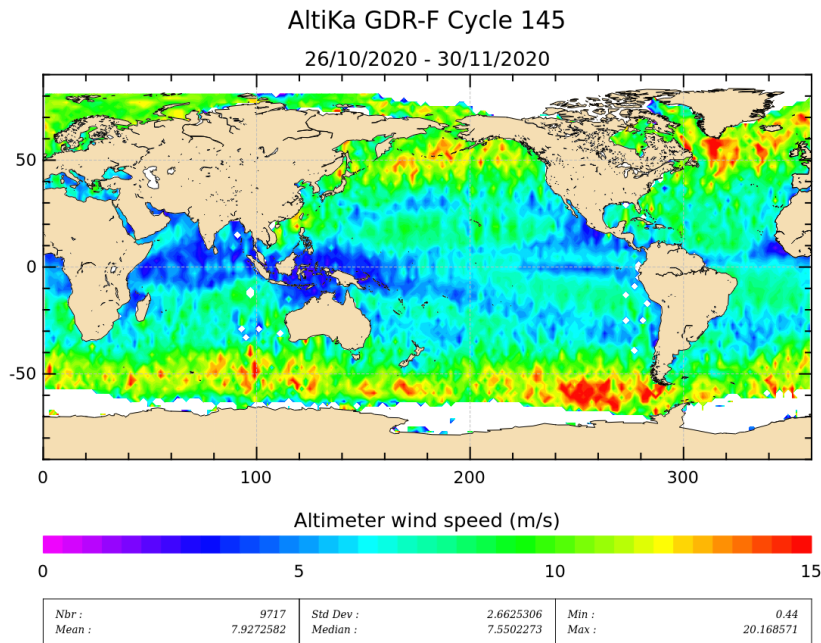
Figure 10: Altimeter wind speed for cycle 145.
