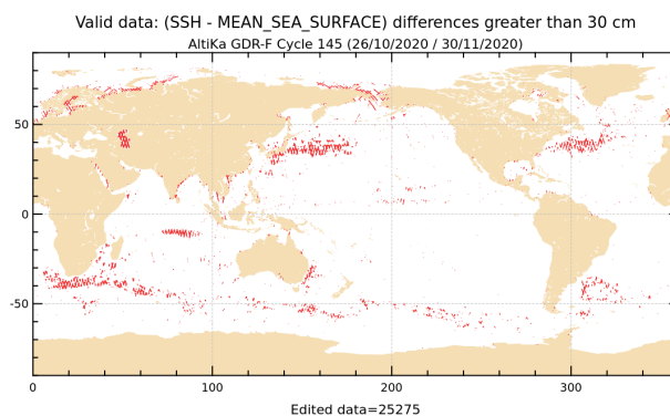
Figure 21: SLA higher than 30 cm for cycle 145.
