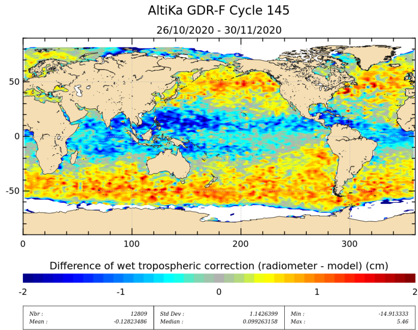
Figure 12: Mean of wet troposphere correction difference (Radiometer-ECMWF model) for cycle 145.
