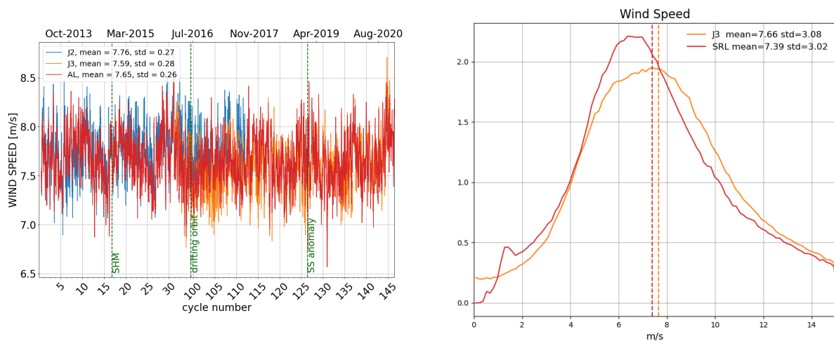
Figure 11: Daily monitoring of altimeter wind speed for Saral/AltiKa, Jason-2 and Jason-3 on the left and histogram for cycle 145 on the right (limited to 66° latitude).
