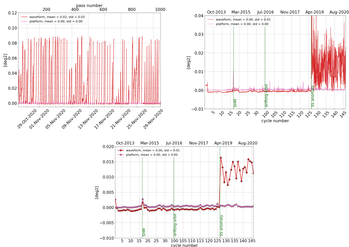
Figure 14: Monitoring per pass for cycle 145 (left), daily monitoring (right) and cyclic monitoring (bottom) of SARAL/AltiKa's mispointing angle: comparison between the one derived from waveform retracking and the one measured by platform startrackers.
