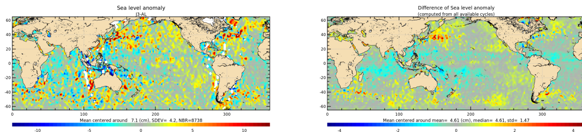
Figure 22: Jason-3 – Saral/AltiKa SLA differences for cycle 147 (left) and averaged over the whole Saral/AltiKa period (right).
