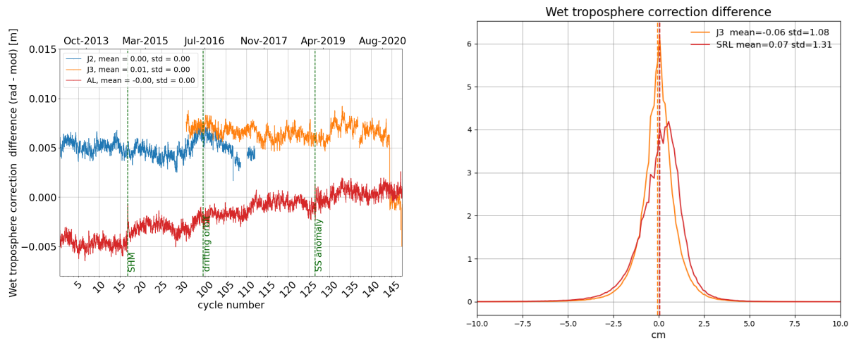
Figure 13: Daily monitoring of wet troposphere differences (Radiometer-ECMWF model) for Saral/AltiKa Jason-2 and Jason-3 (left) and histogram on the right (limited to 66° latitude) for cycle 147 .
