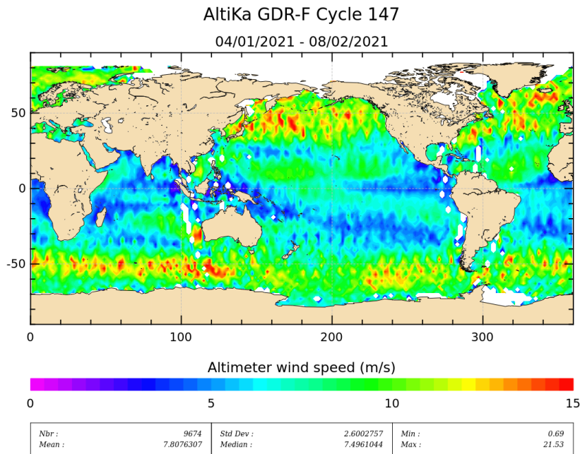
Figure 10: Altimeter wind speed for cycle 147.
