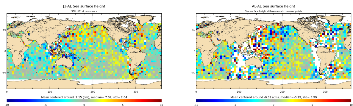
Figure 15: Mean of multi-mission SSH and mono-mission SSH differences at crossovers for cycle 147.
