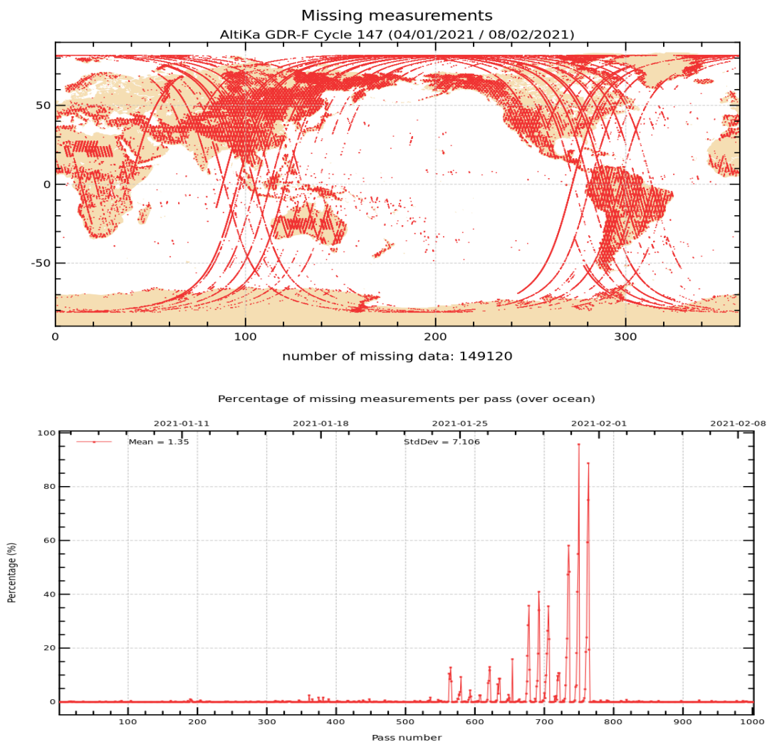
Figure 1: Map of missing measurements for cycle 147 on top. Monitoring of percentage of missing ocean measurements per pass on bottom.
