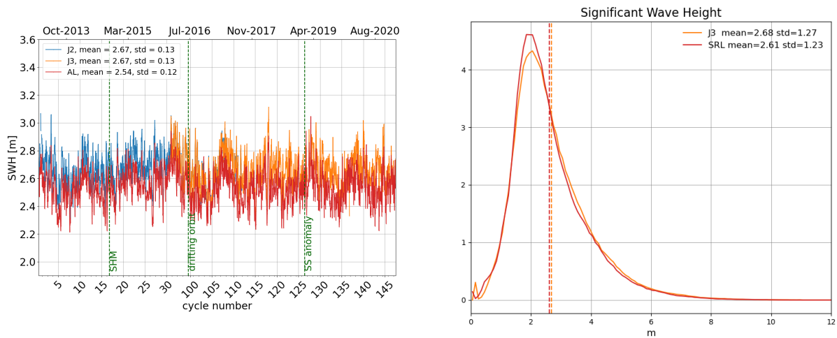
Figure 7: Daily monitoring of significant wave height for AltiKa (Ka-band) Jason-2 and Jason-3 (Ku-band) on the left and histogram for cycle 147 on the right (limited to 66° latitude).
