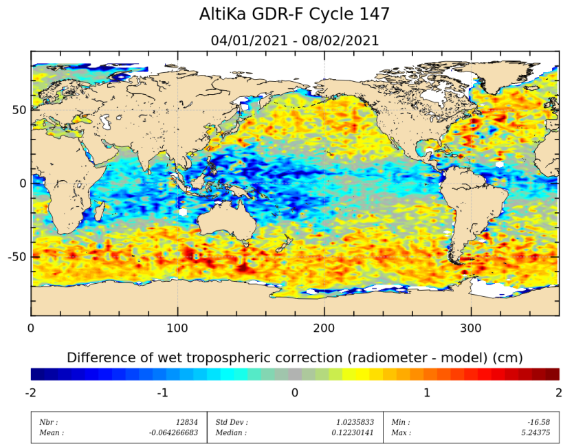
Figure 12: Mean of wet troposphere correction difference (Radiometer-ECMWF model) for cycle 147.
