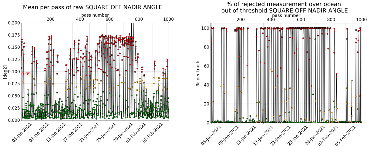
Figure 3: [left] Mispointing cycle 147, [right] Percentage of rejected measurement by threshold on square off-nadir angle.
