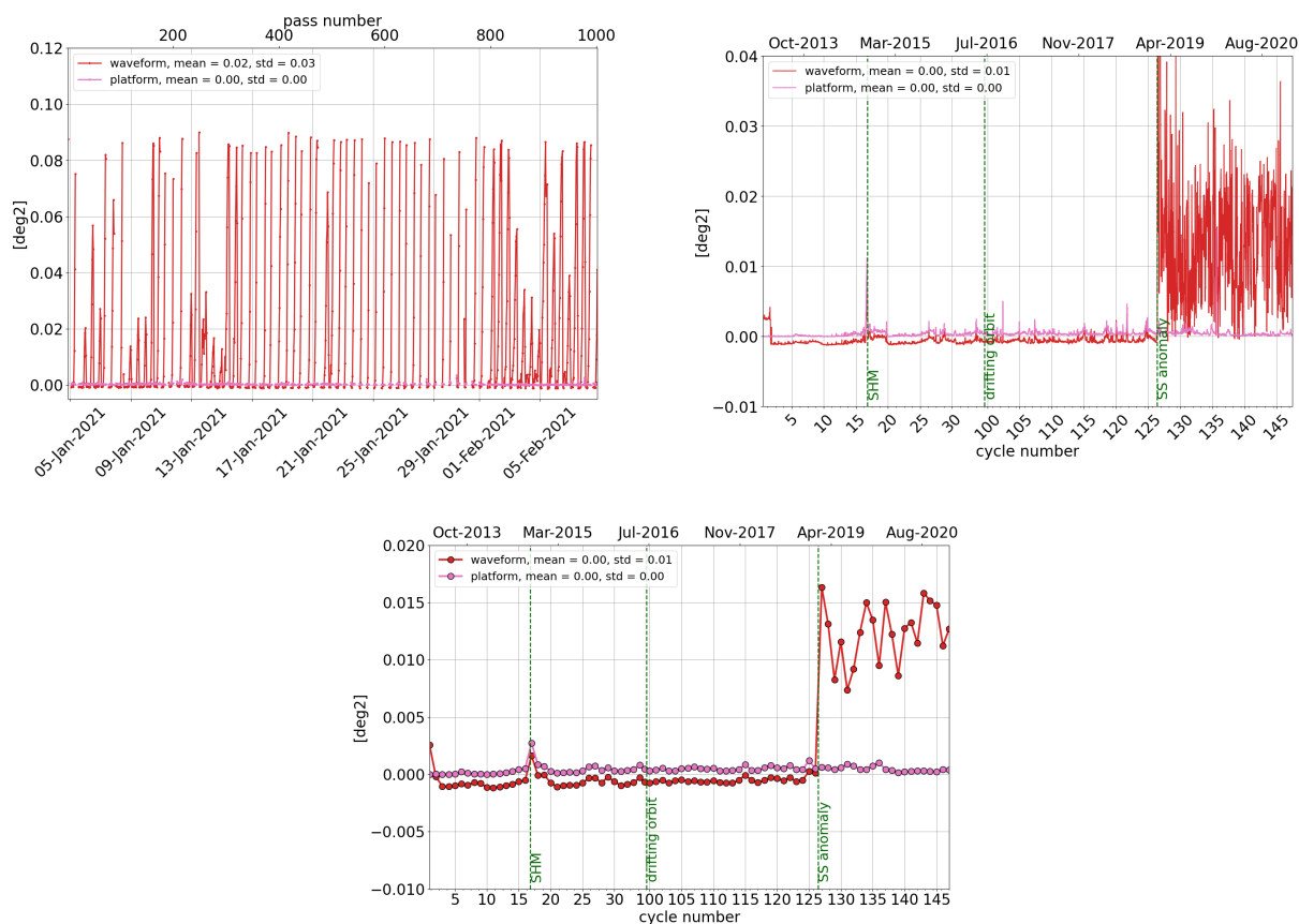
Figure 14: Monitoring per pass for cycle 147 (left), daily monitoring(right) and cyclic monitoring (bottom) of SARAL/AltiKa's mispointing angle: comparison between the one derived from waveform retracking and the one measured by platform startrackers.
