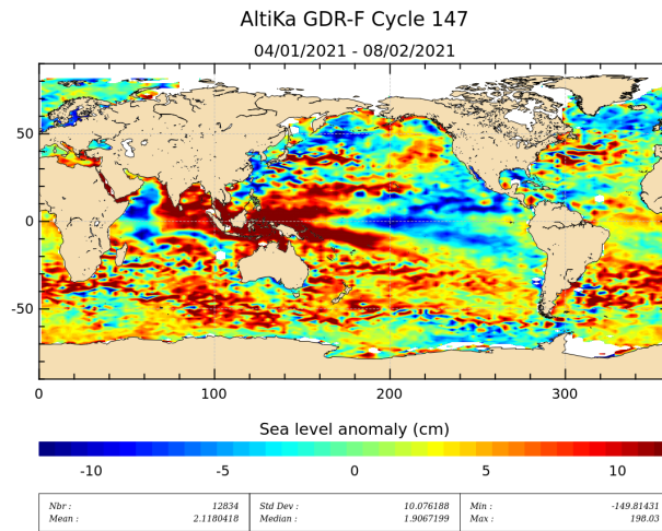
Figure 20: Sea level anomaly relative to MSS for cycle 147.
