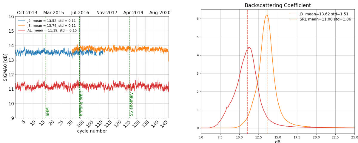
Figure 8: Daily monitoring of backscattering coefficient for Saral/AltiKa, Jason-2 and Jason-3 on the left and histogram for cycle 147 on the right (limited to 66° latitude).
