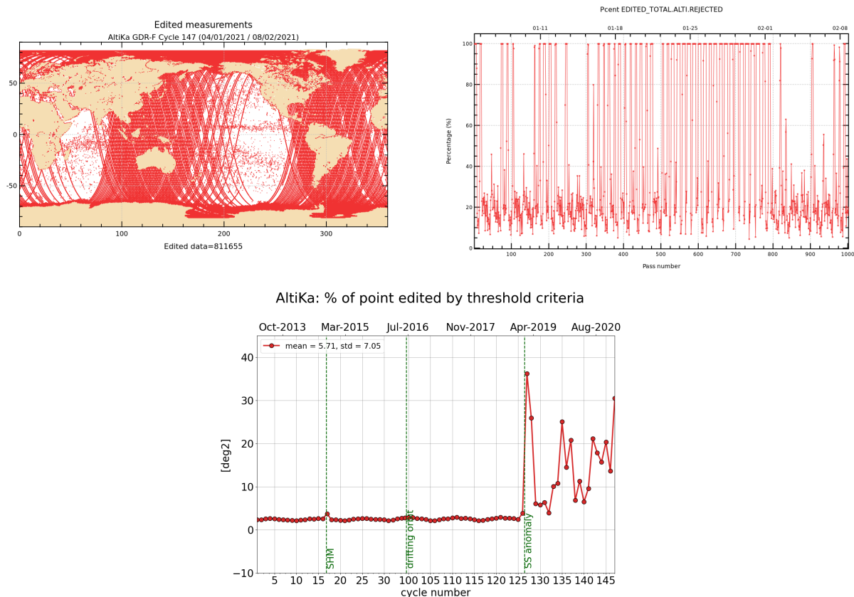
Figure 2: Rejected measurements on thresholds criteria : Cycle 147, map and monitoring of % of rejected measurements per track (top), whole time serie / % of rejected measurements per cycle (bottom).
