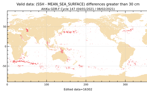
Figure 21: SLA higher than 30 cm for cycle 147.
