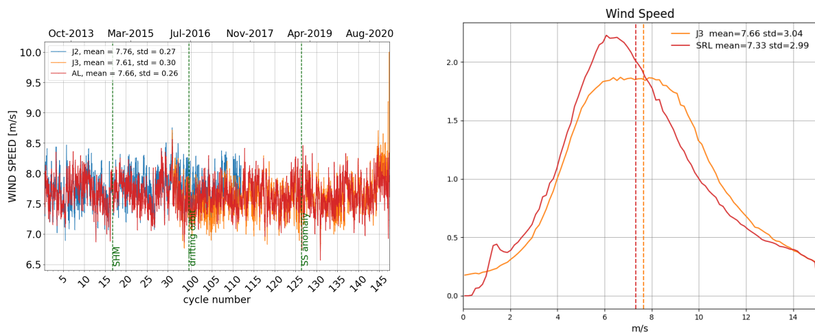
Figure 11: Daily monitoring of altimeter wind speed for Saral/AltiKa, Jason-2 and Jason-3 on the left and histogram for cycle 147 on the right (limited to 66° latitude).
