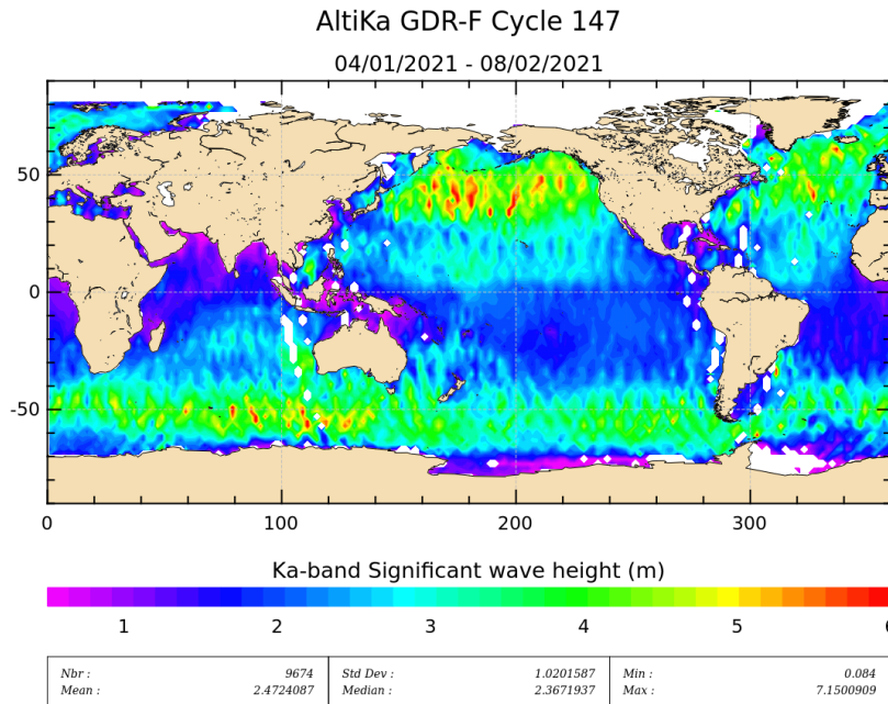
Figure 6: Significant wave height for cycle 147.
